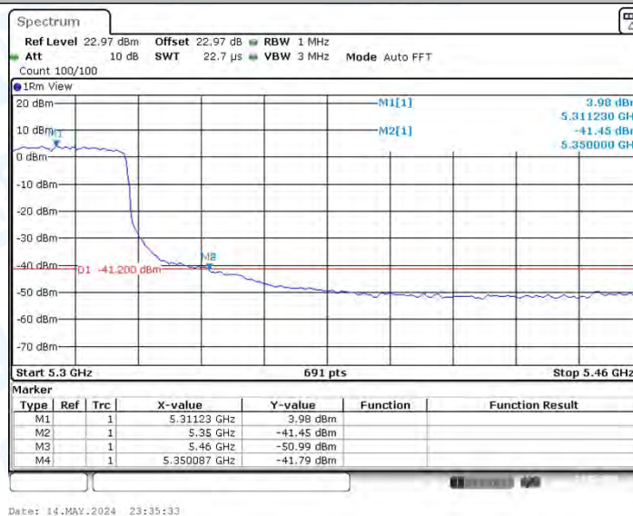
11AX40SISO_Ant1_High_5310_Peak
