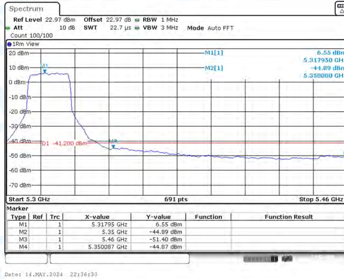
11AX20SISO_Ant1_High_5320_Peak
