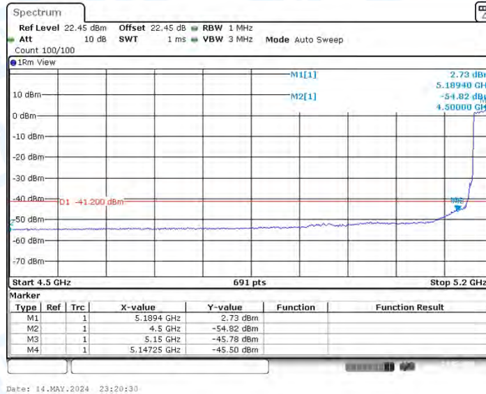
11AX40SISO_Ant1_Low_5190_Peak
