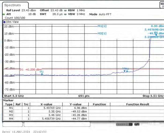
11AX20SISO_Ant1_Low_5500_Peak
