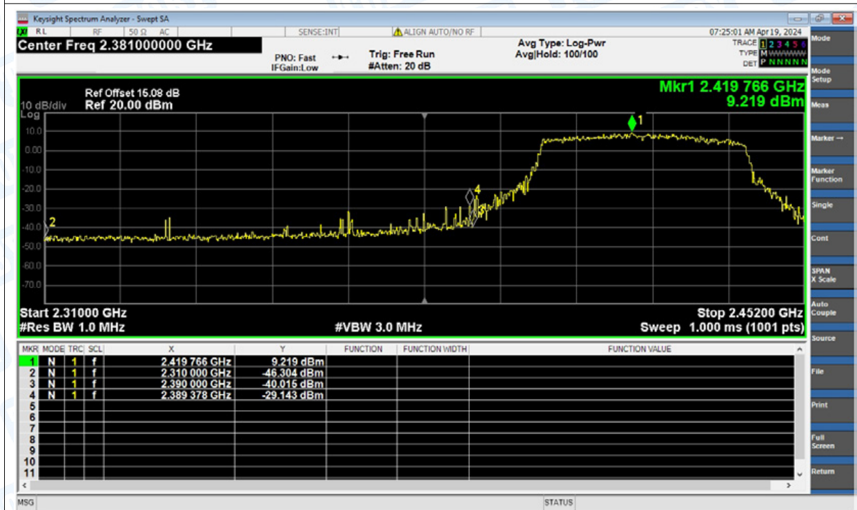
Restrict Band NVNT ax(VHT40) 2422MHz Ant1 Average
