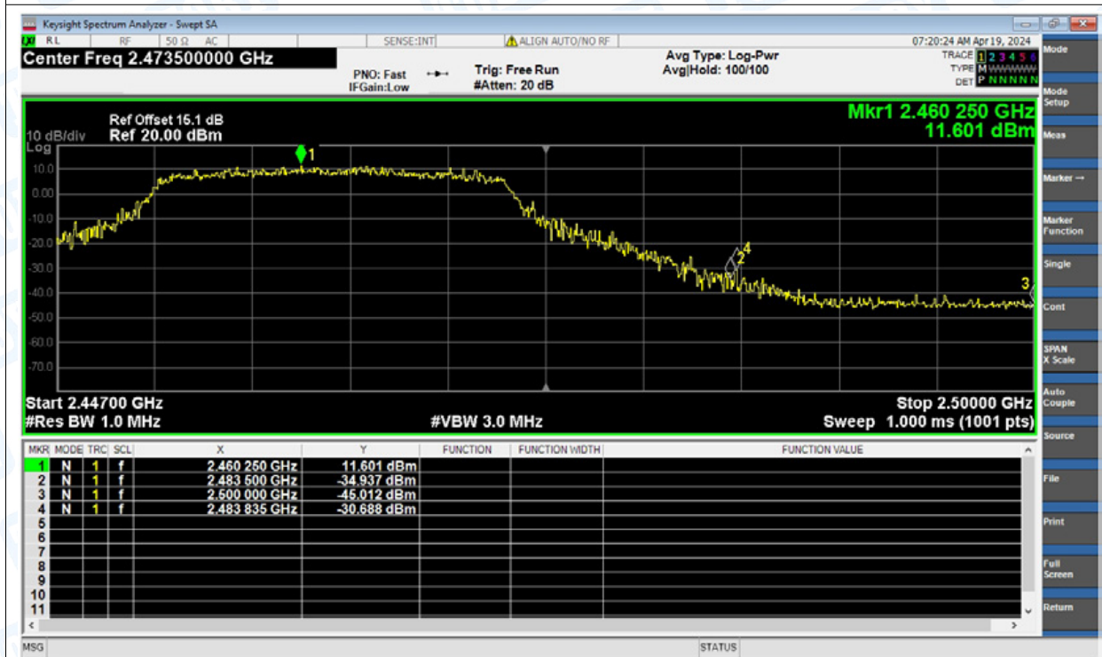
Restrict Band NVNT ax(VHT20) 2462MHz Ant1 Average
