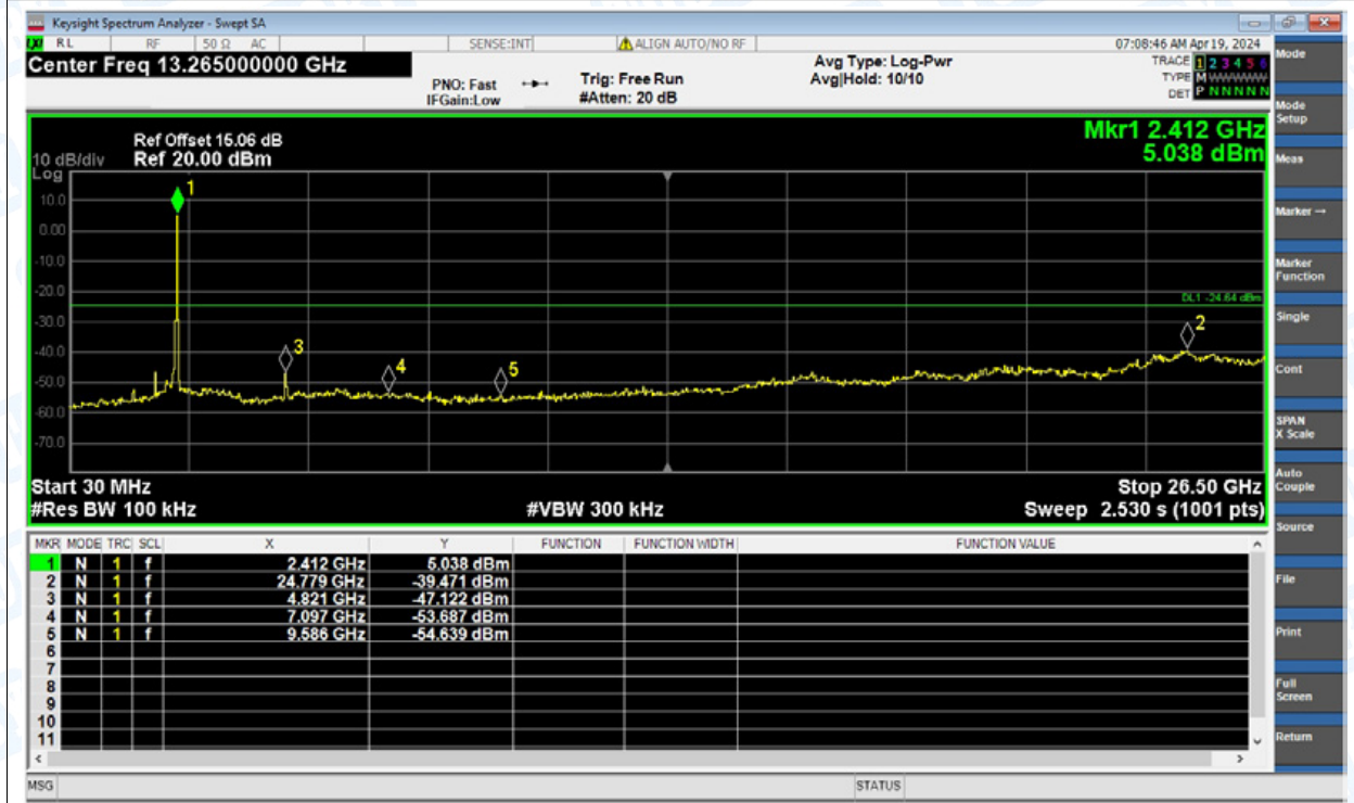
Tx. Spurious NVNT ax(VHT20) 2412MHz Ant1 Emission
