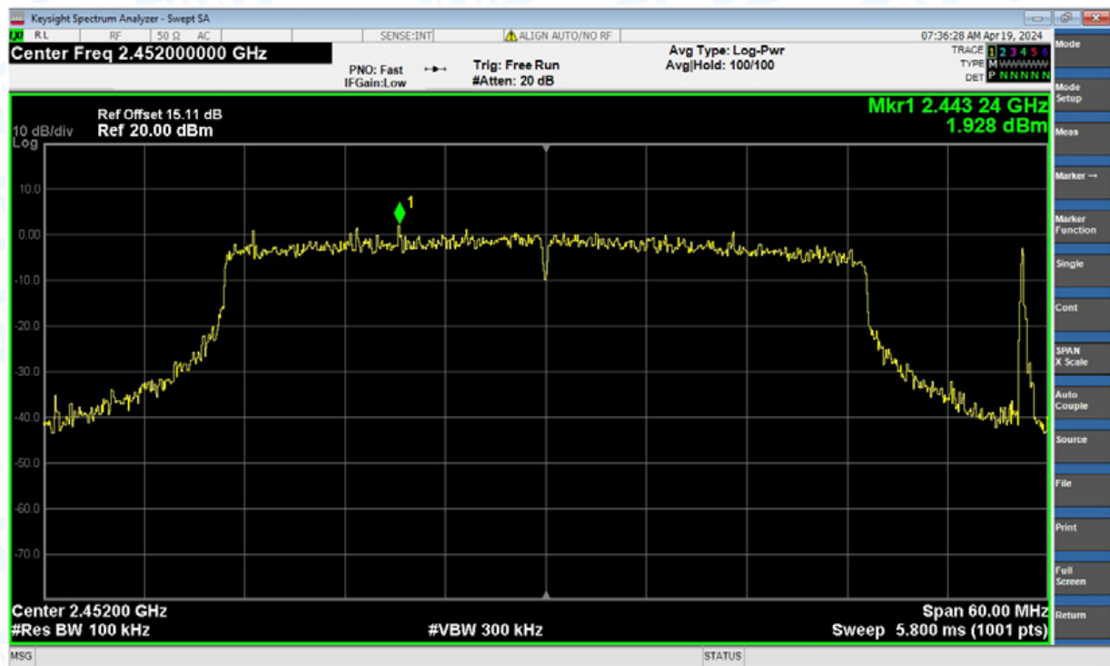
Tx. Spurious NVNT ax(VHT40) 2452MHz Ant1 Emission
