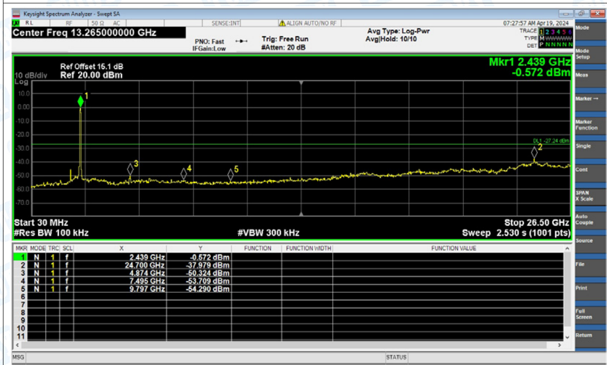
Tx. Spurious NVNT ax(VHT40) 2437MHz Ant1 Emission
