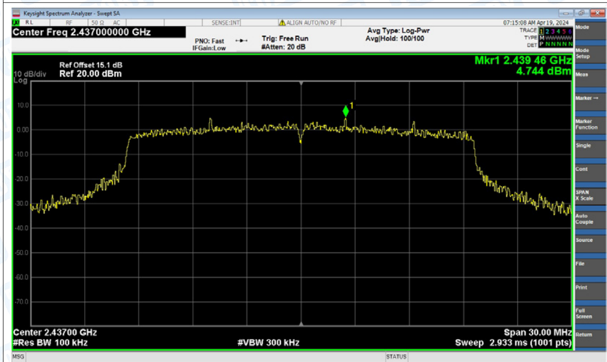
Tx. Spurious NVNT ax(VHT20) 2437MHz Ant1 Emission
