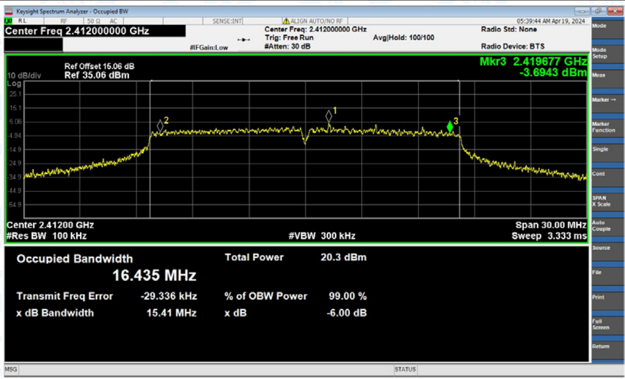
-6dB Bandwidth NVNT g 2412MHz Ant1
