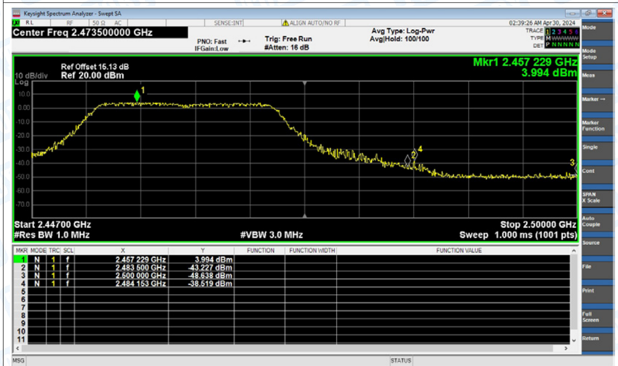
Restrict Band NVNT n(HT20) 2462MHz Ant2 Average
