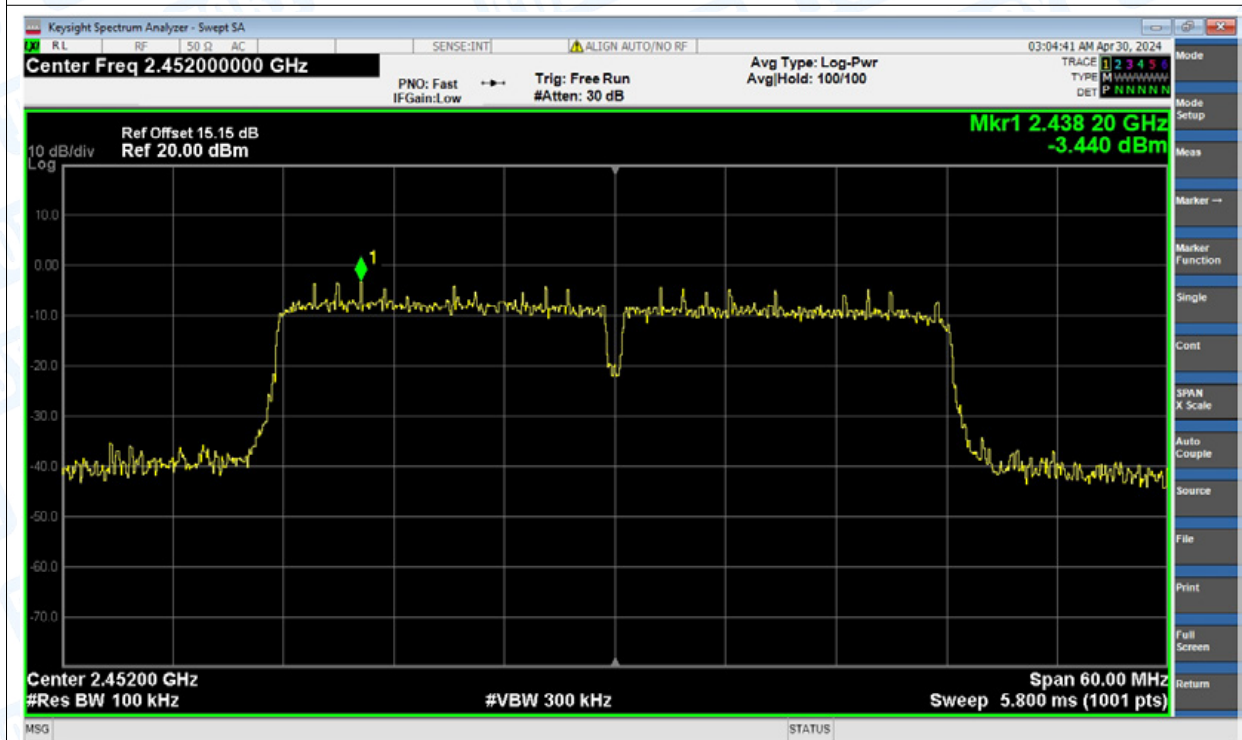
Band Edge NVNT n(HT40) 2452MHz Ant2 Emission
