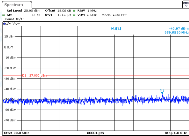
11A-Ant1-5500-30~1000-PASS
