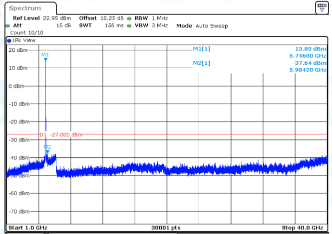
11N20SISO-Ant1-5745-1000~40000-PASS
