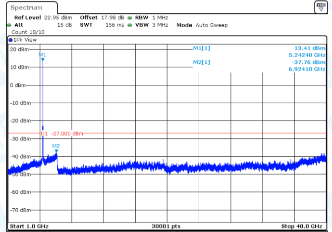
11N20SISO-Ant1-5200-1000~40000-PASS
