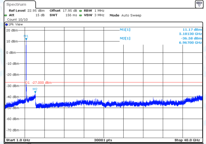
11N20SISO-Ant1-5180-1000~40000-PASS
