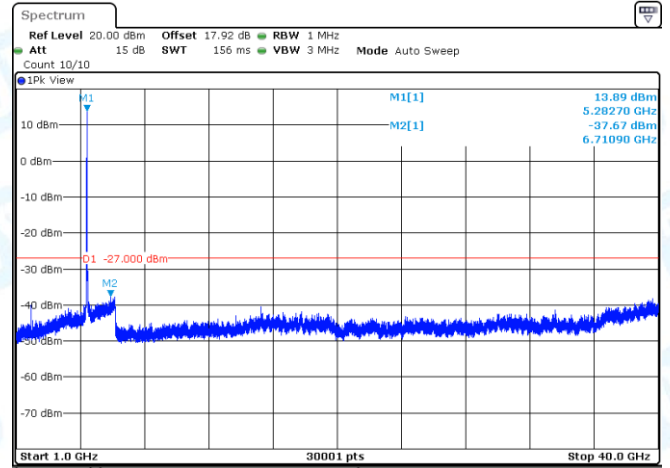
11AC20SISO-Ant1-5260-1000~40000-PASS
