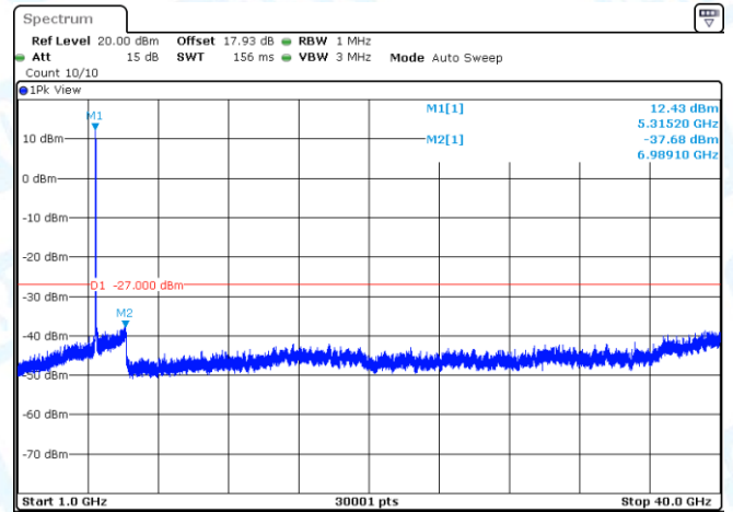
11AX20SISO-Ant1-5280-1000~40000-PASS
