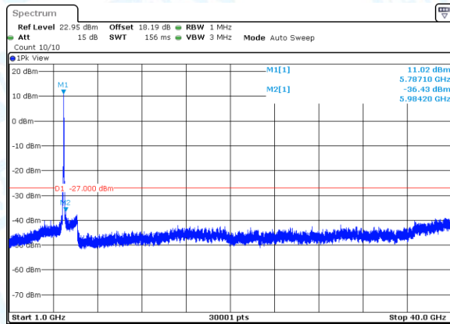
11AC40SISO-Ant1-5755-1000~40000-PASS
