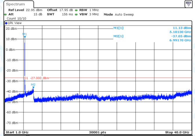
11AC20SISO-Ant1-5180-1000~40000-PASS
