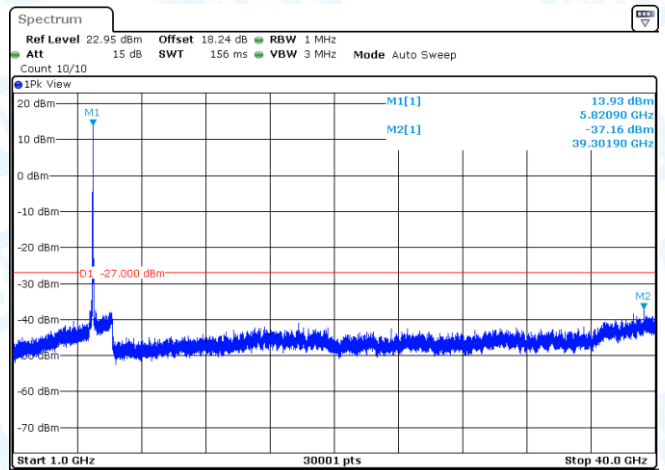
11N20SISO-Ant1-5785-1000~40000-PASS
