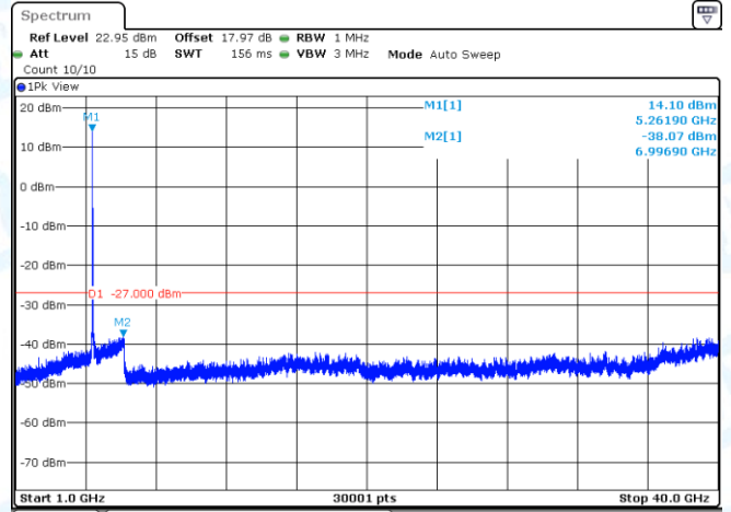
11A-Ant1-5260-1000~40000-PASS
