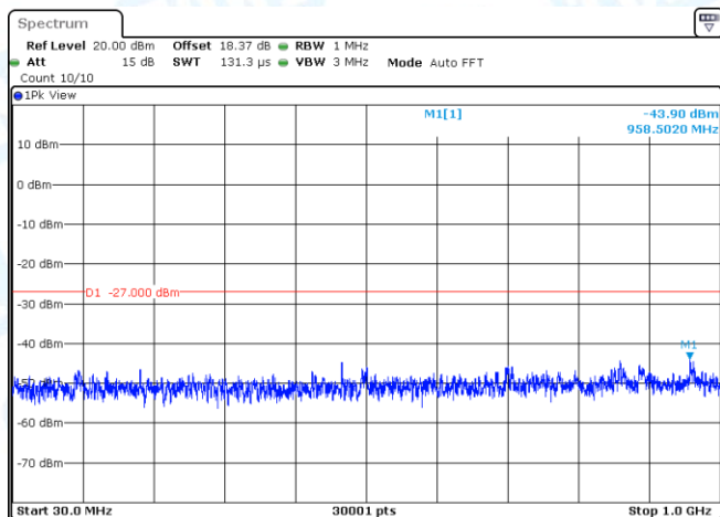
11AC40SISO-Ant1-5670-30~1000-PASS
