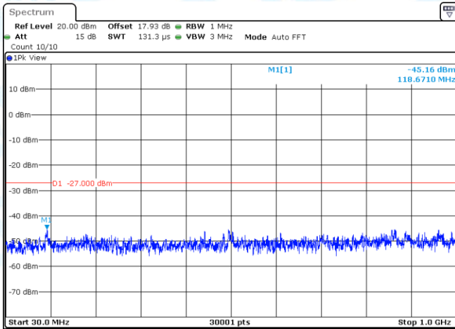
11AC20SISO-Ant1-5280-30~1000-PASS
