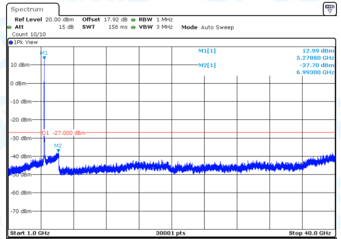
11N20SISO-Ant1-5260-1000~40000-PASS
