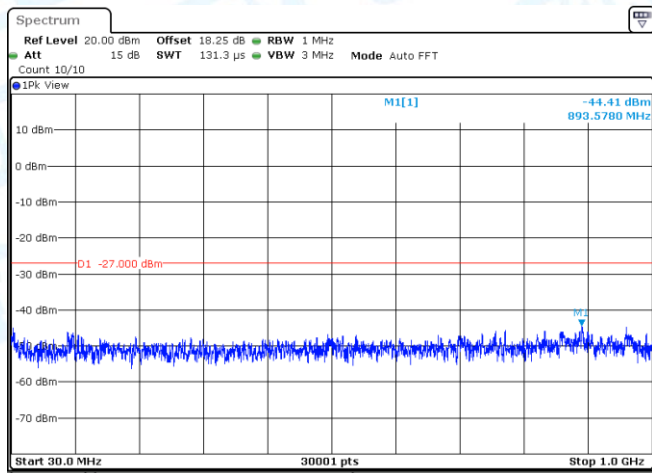
11AC40SISO-Ant1-5670-30~1000-PASS
