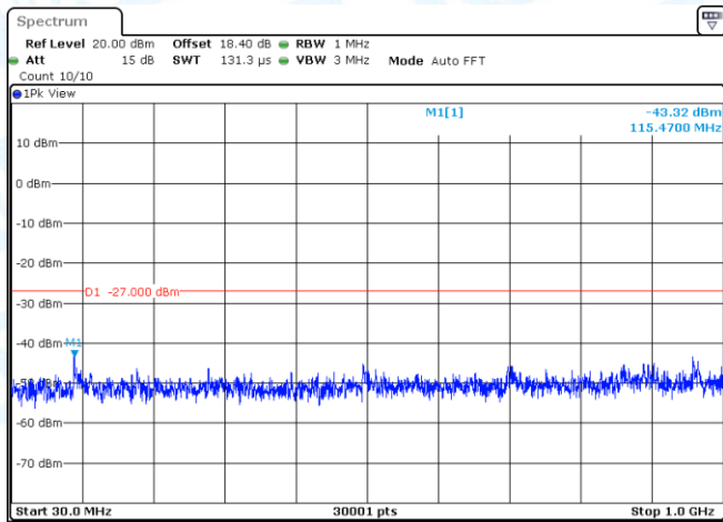
11A-Ant1-5580-30~1000-PASS
