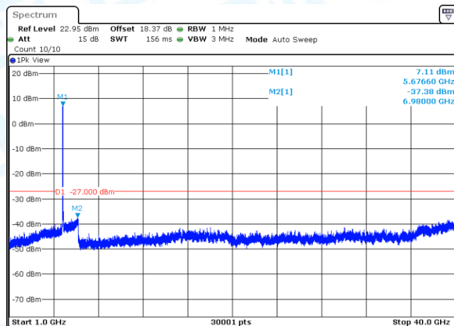
11AC40SISO-Ant1-5670-1000~40000-PASS
