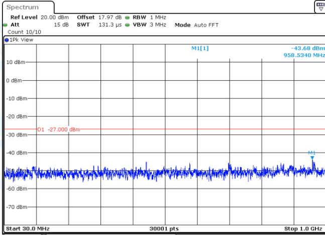
11AC20SISO-Ant1-5260-30~1000-PASS
