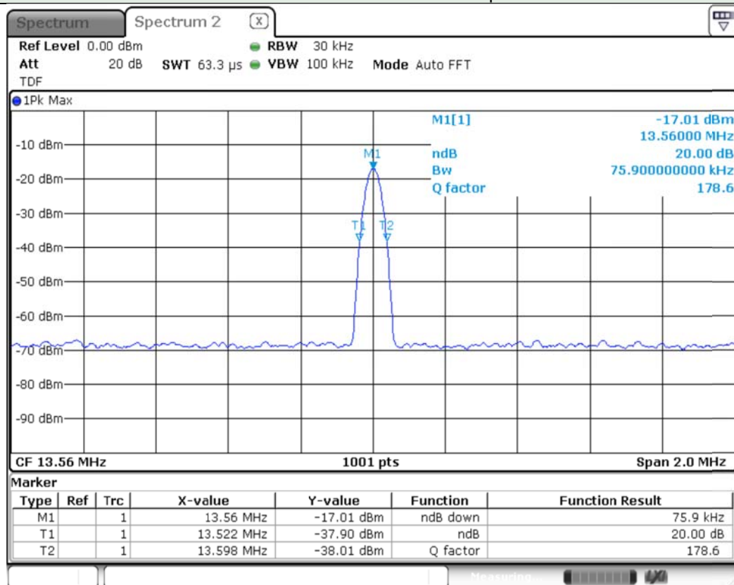
20 dB bandwidth measurement plot
