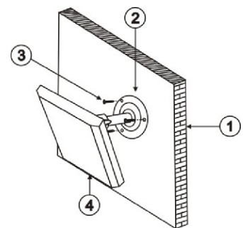
Installation diagram
