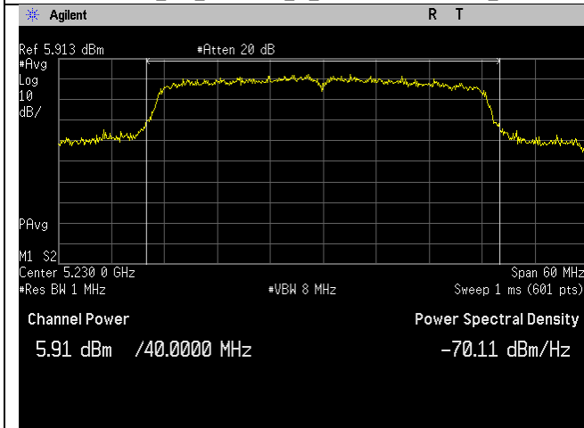
5230MHz_46_40MHz_n_Channel Power_Ant B
