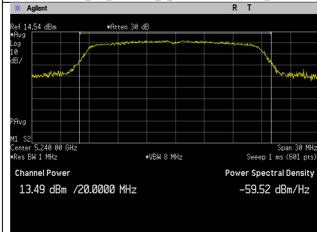
5240MHz_48_20MHz_n_Channel Power_Ant A
