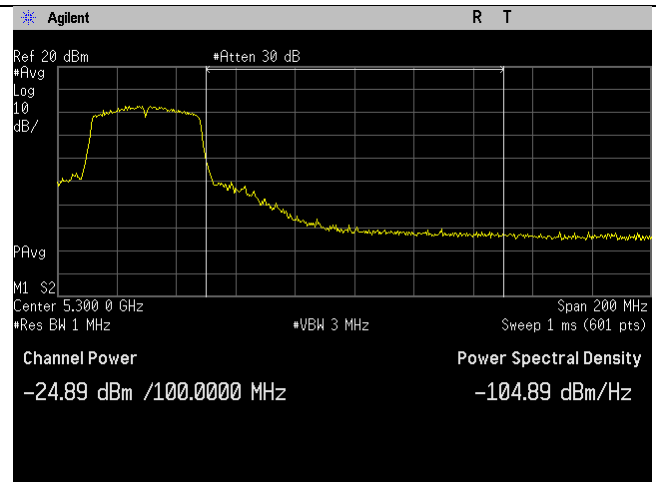
5230MHz_46_40MHz_n_Leakage Power_Ant A
