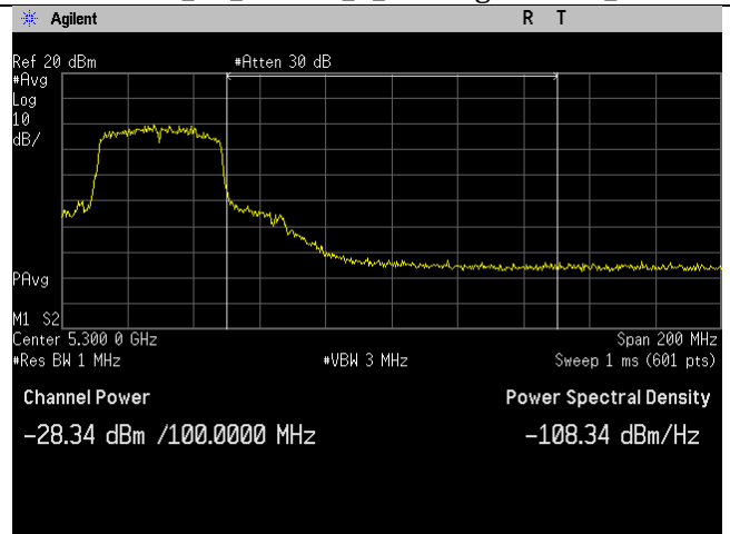
5230MHz_46_40MHz_n_Leakage Power_Ant B
