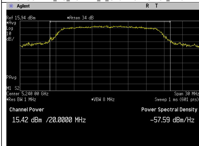
5240MHz_48_20MHz_a_Channel Power_Ant A
