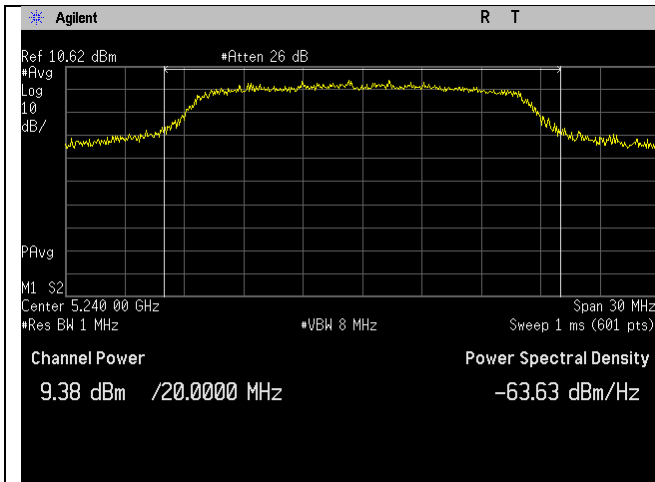
5240MHz_48_20MHz_a_Channel Power_Ant B
