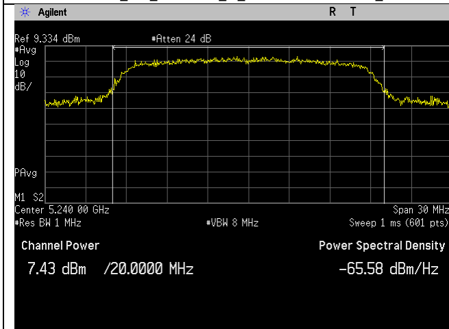
5240MHz_48_20MHz_n_Channel Power_Ant B
