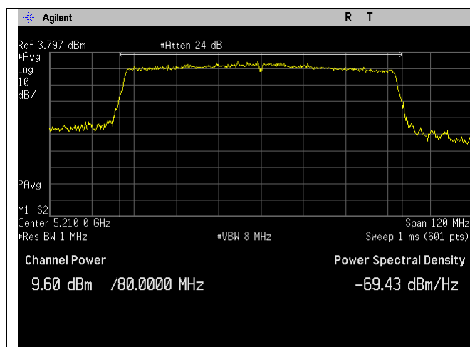
5210MHz_42_80MHz_ac_Channel Power_Ant A
