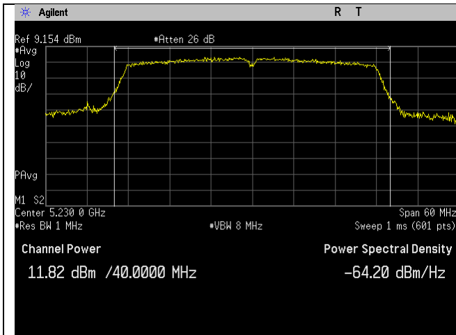
5230MHz_46_40MHz_n_Channel Power_Ant A
