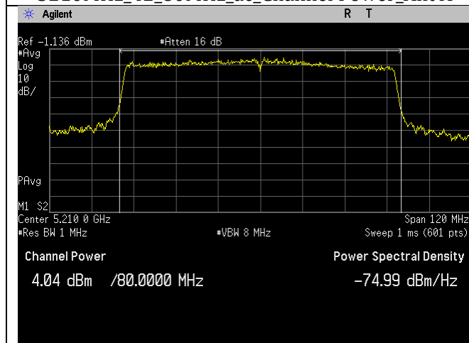
5210MHz_42_80MHz_ac_Channel Power_Ant B
