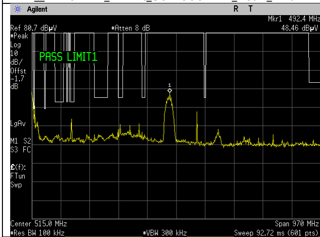
WIFI_2452MHz_40MHz_n-mode_15.209_30-1000MHz_Peak_Ant A
