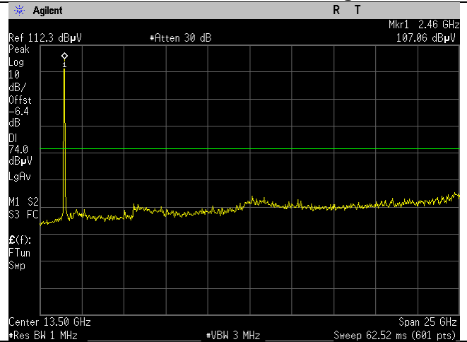
WIFI_2452MHz_40MHz_n-mode_Peak_Ant B
