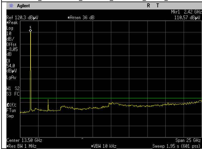
WIFI_2437MHz_20MHz_b-mode_Avg_Ant A
