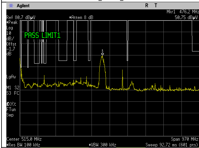
WIFI_2437MHz_40MHz_n-mode_15.209_30- 1000MHz_Peak_Ant A
