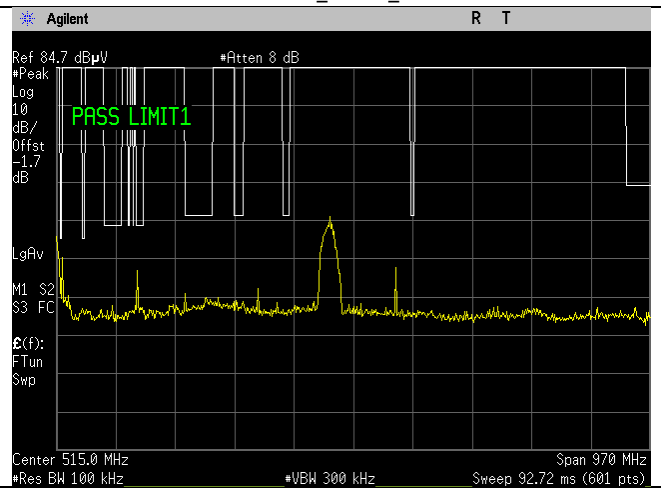
WIFI_2437MHz_40MHz_n-mode_15.209_30- 1000MHz_Peak_Ant B
