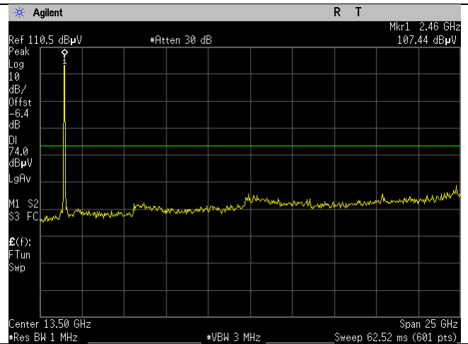
WIFI_2437MHz_40MHz_n-mode_Peak_Ant B
