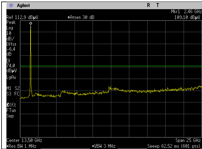
WIFI_2437MHz_40MHz_n-mode_Peak_Ant A
