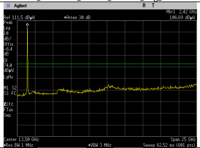
WIFI_2422MHz_40MHz_n-mode_Peak_Ant B
