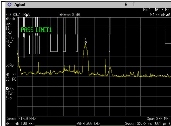
WIFI_2422MHz_40MHz_n-mode_15.209_30-1000MHz_Peak_Ant A
