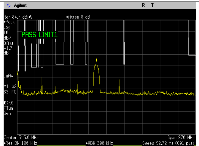
WIFI_2422MHz_40MHz_n-mode_15.209_30-1000MHz_Peak_Ant B
