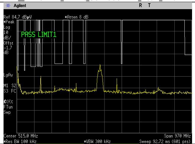
WIFI_2452MHz_40MHz_n-mode_15.209_30-1000MHz_Peak_Ant B
