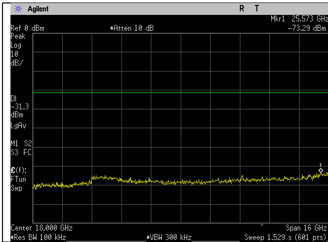
WIFI_2462MHz_20MHz_n-mode_10-26GHz_Ant A
