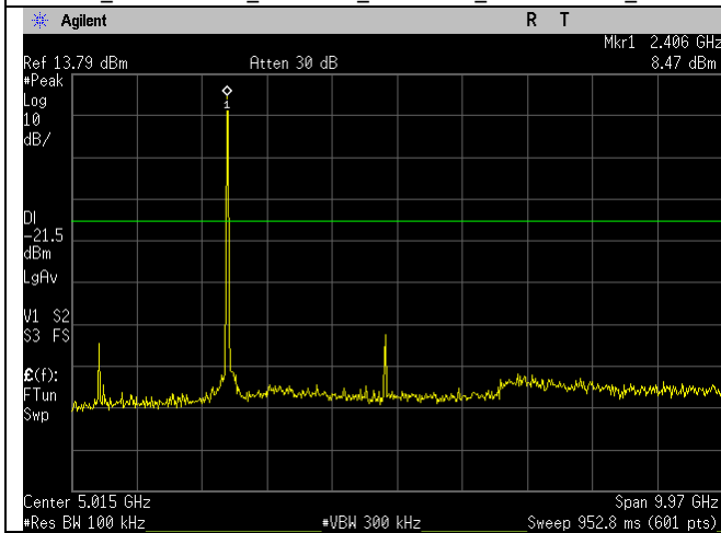
WIFI_2412MHz_20MHz_b-mode_30MHz-10GHz_Ant A
