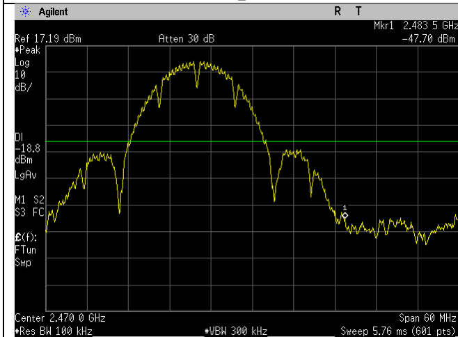
WIFI_2462MHz_20MHz_b-mode_Upper Band Edge_Ant A
