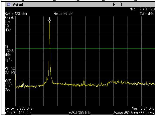
WIFI_2452MHz_40MHz_n-mode_30MHz- 10GHz_Ant A
