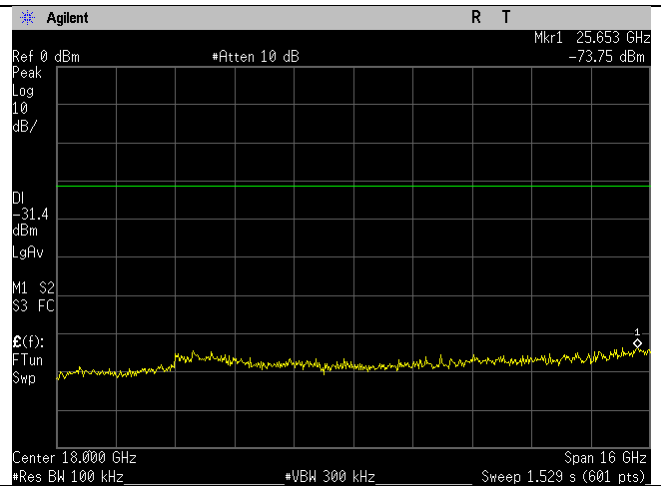
WIFI_2462MHz_20MHz_n-mode_10-26GHz_Ant B
