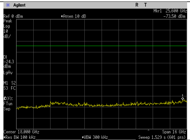
WIFI_2412MHz_20MHz_b-mode_10-26GHz_Ant B
