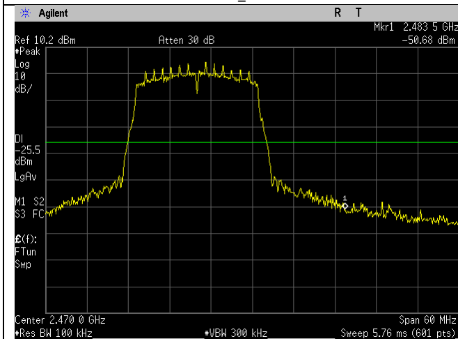
WIFI_2462MHz_20MHz_n-mode_Upper Band_Edge_Ant A
