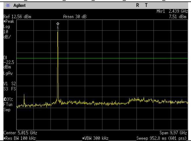
WIFI_2437MHz_20MHz_b-mode_30MHz- 10GHz_Ant B
