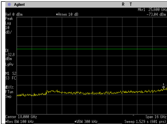
WIFI_2452MHz_40MHz_n-mode_10-26GHz_Ant A
