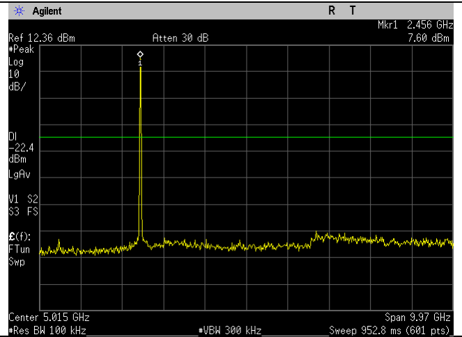
WIFI_2462MHz_20MHz_b-mode_30MHz-10GHz_Ant B
