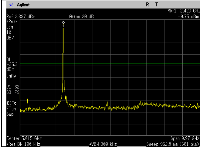
WIFI_2422MHz_40MHz_n-mode_30MHz-10GHz_Ant A
