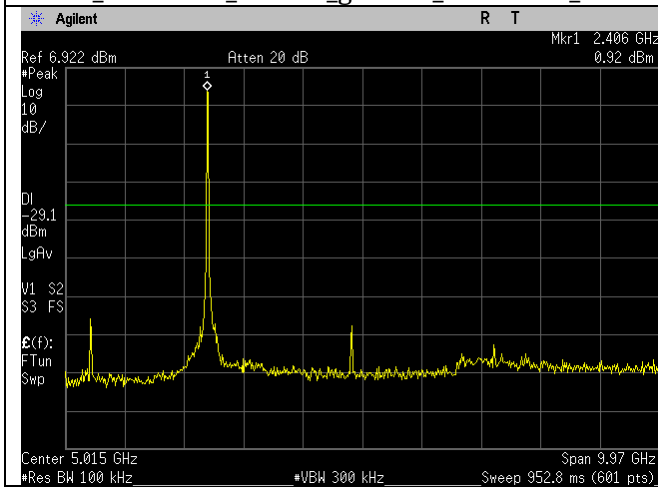
WIFI_2412MHz_20MHz_g-mode_30MHz-10GHz_Ant A
