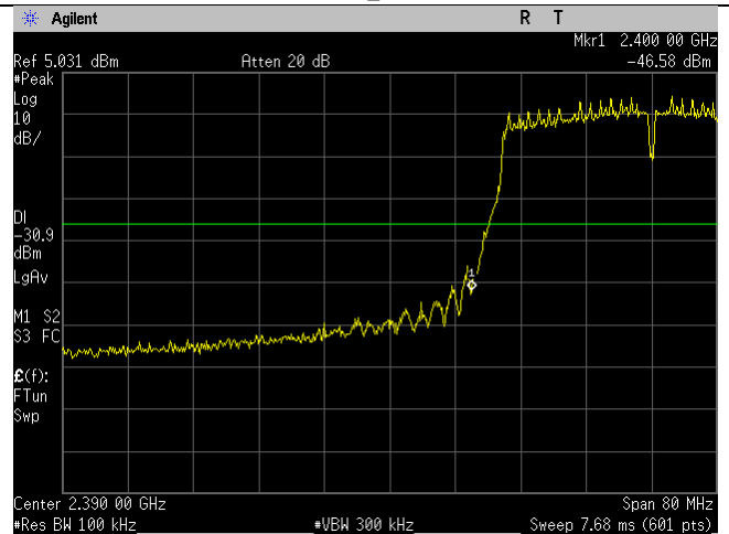
WIFI_2422MHz_40MHz_n-mode_Lower Band Edge_Ant B
