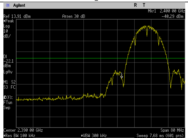
WIFI_2412MHz_20MHz_b-mode_Lower Band Edge_Ant B
