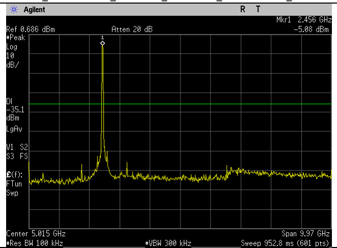
WIFI_2452MHz_40MHz_n-mode_30MHz- 10GHz_Ant B
