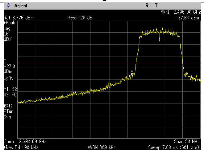
WIFI_2412MHz_20MHz_n-mode_Lower Band Edge_Ant B
