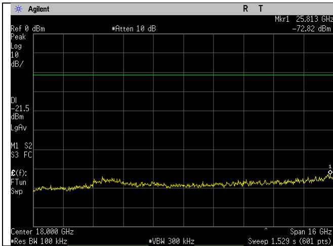
WIFI_2412MHz_20MHz_b-mode_10-26GHz_Ant A
