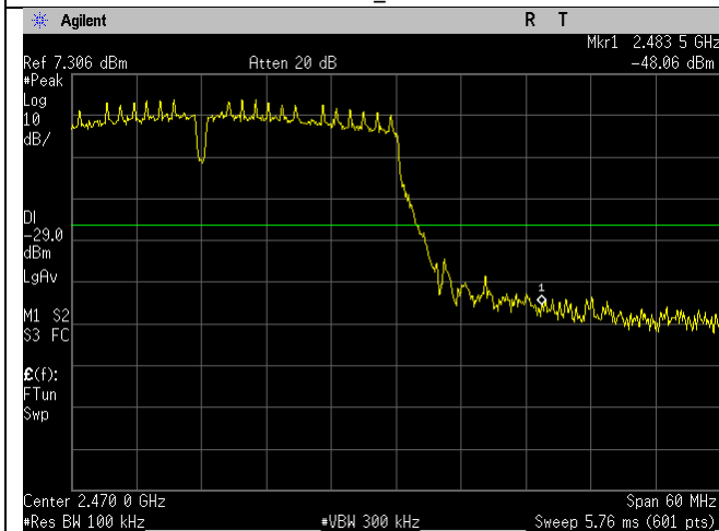
WIFI_2452MHz_40MHz_n-mode_Upper Band Edge_Ant A
