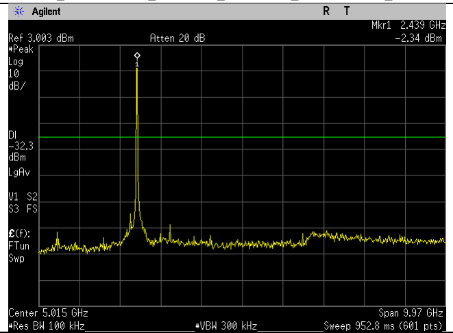
WIFI_2437MHz_20MHz_n-mode_30MHz- 10GHz_Ant B
