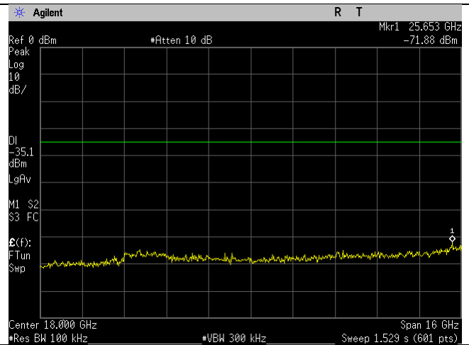
WIFI_2452MHz_40MHz_n-mode_10-26GHz_Ant B
