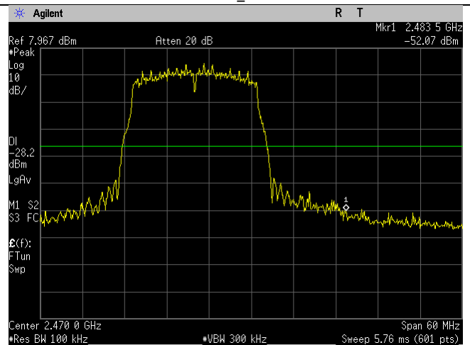
WIFI_2462MHz_20MHz_n-mode_Upper Band_Edge_Ant B
