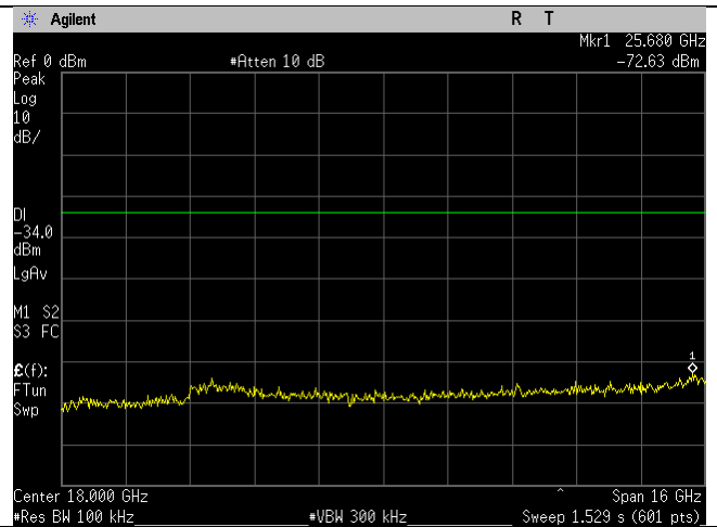
WIFI_2422MHz_40MHz_n-mode_10-26GHz_Ant B
