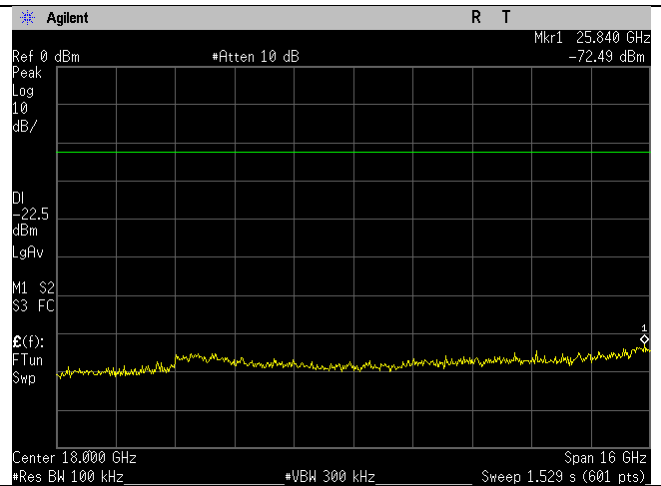
WIFI_2437MHz_20MHz_b-mode_10-26GHz_Ant B
