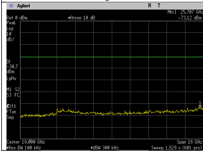
WIFI_2437MHz_20MHz_n-mode_10-26GHz_Ant A
