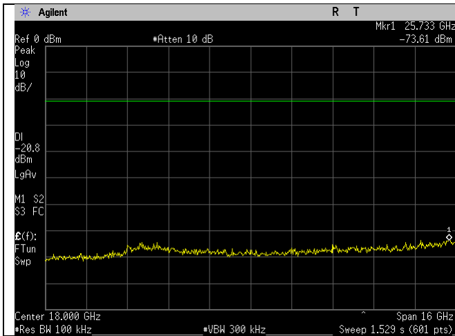
WIFI_2437MHz_20MHz_b-mode_10-26GHz_Ant A
