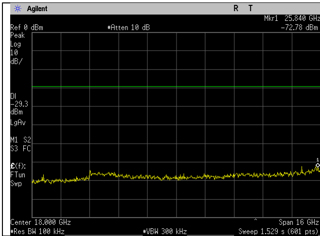
WIFI_2412MHz_20MHz_n-mode_10-26GHz_Ant A
