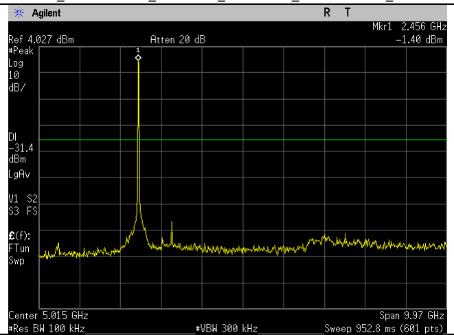
WIFI_2462MHz_20MHz_n-mode_30MHz-10GHz_Ant B
