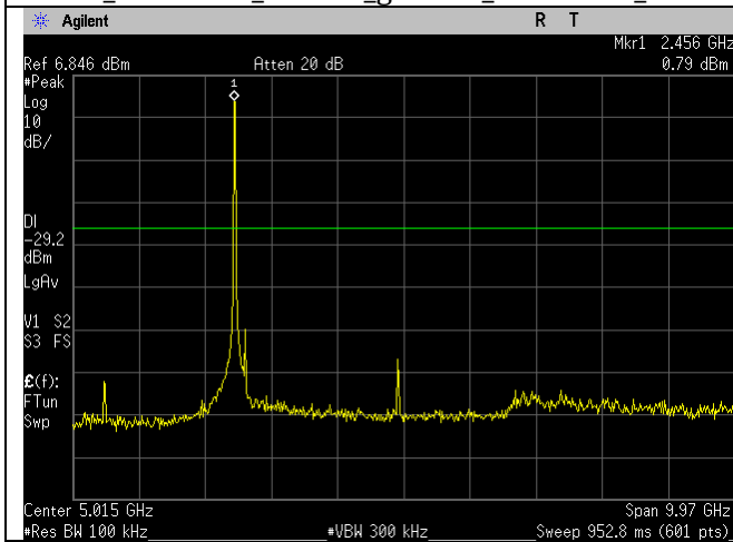
WIFI_2462MHz_20MHz_g-mode_30MHz-10GHz_Ant A
