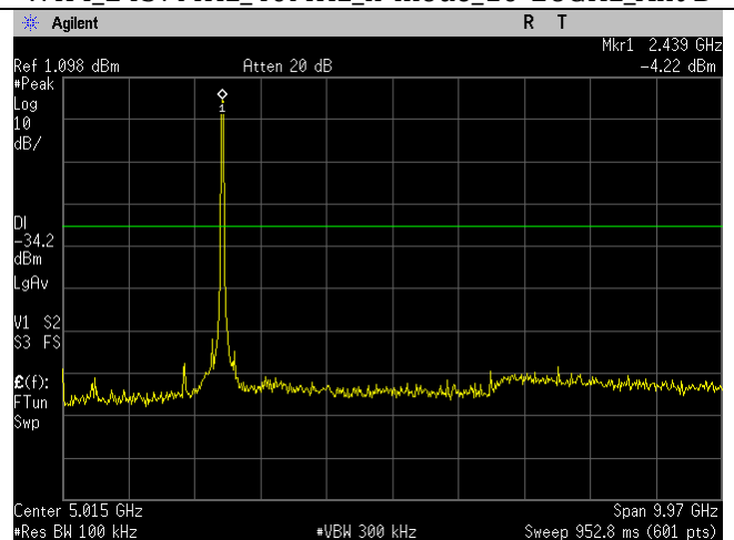
WIFI_2437MHz_40MHz_n-mode_30MHz-10GHz_Ant B
