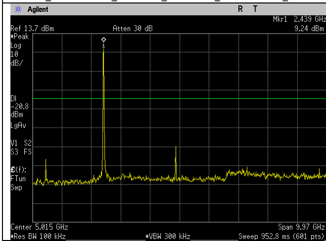
WIFI_2437MHz_20MHz_b-mode_30MHz- 10GHz_Ant A
