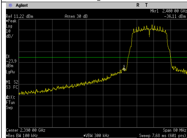
WIFI_2412MHz_20MHz_g-mode_Lower Band Edge_Ant A
