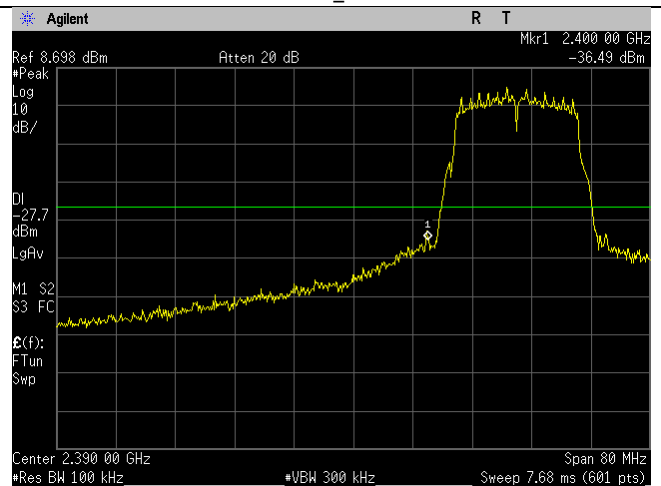
WIFI_2412MHz_20MHz_g-mode_Lower Band Edge_Ant B
