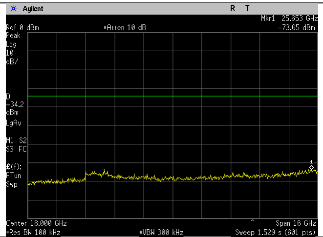
WIFI_2437MHz_40MHz_n-mode_10-26GHz_Ant B
