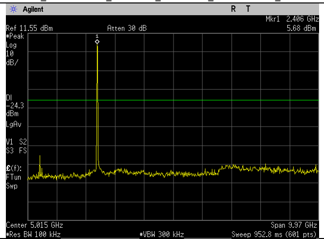
WIFI_2412MHz_20MHz_b-mode_30MHz-10GHz_Ant B
