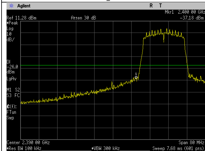
WIFI_2412MHz_20MHz_n-mode_Lower Band Edge_Ant A
