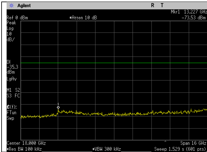
WIFI_2422MHz_40MHz_n-mode_10-26GHz_Ant A
