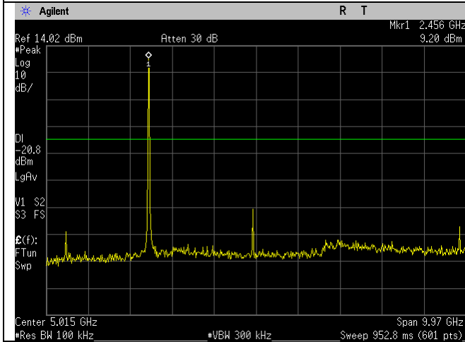
WIFI_2462MHz_20MHz_b-mode_30MHz-10GHz_Ant A
