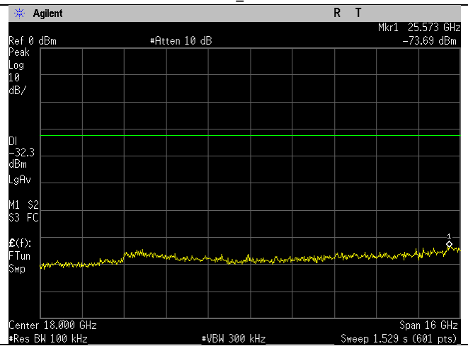
WIFI_2437MHz_20MHz_n-mode_10-26GHz_Ant B
