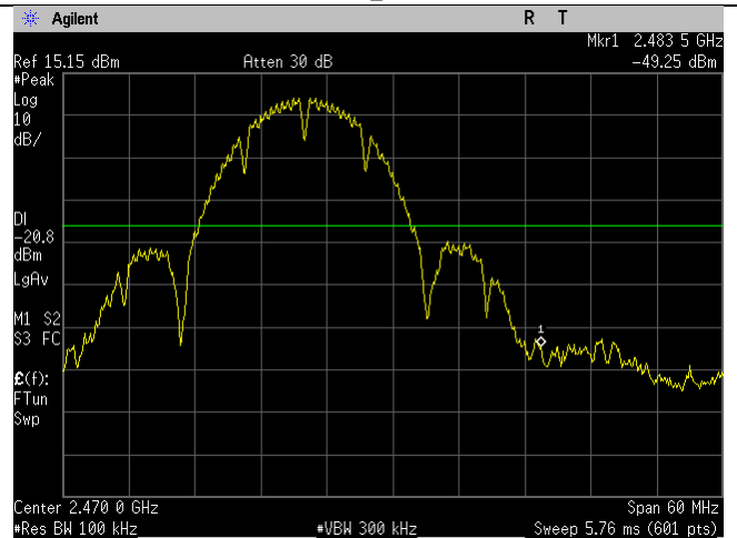
WIFI_2462MHz_20MHz_b-mode_Upper Band Edge_Ant B
