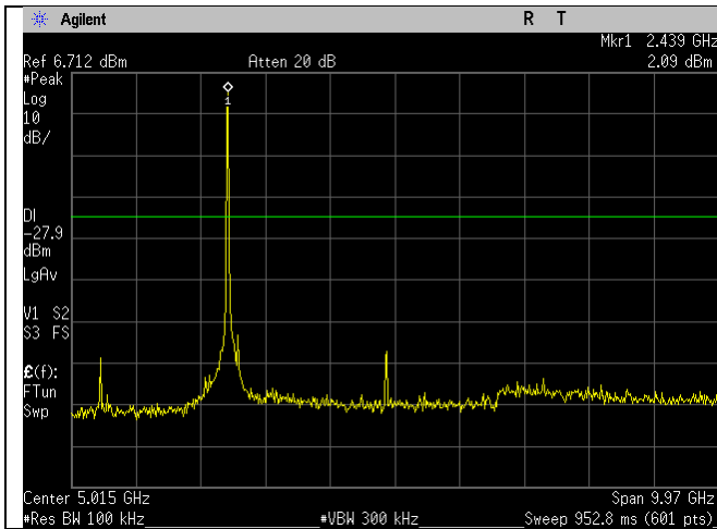
WIFI_2437MHz_20MHz_g-mode_30MHz- 10GHz_Ant A
