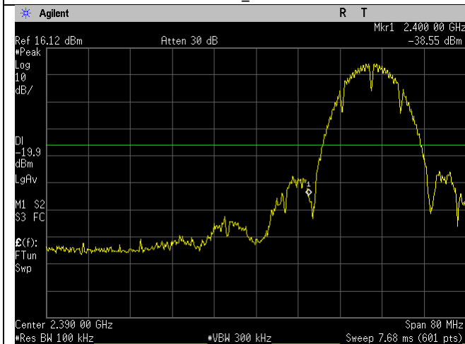
WIFI_2412MHz_20MHz_b-mode_Lower Band Edge_Ant A
