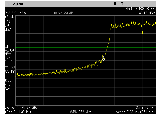
WIFI_2422MHz_40MHz_n-mode_Lower Band Edge_Ant A
