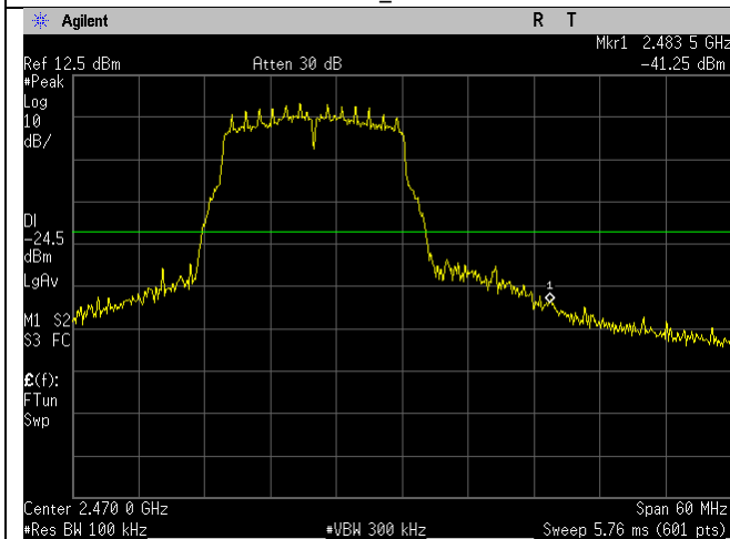
WIFI_2462MHz_20MHz_g-mode_Upper Band Edge_Ant A
