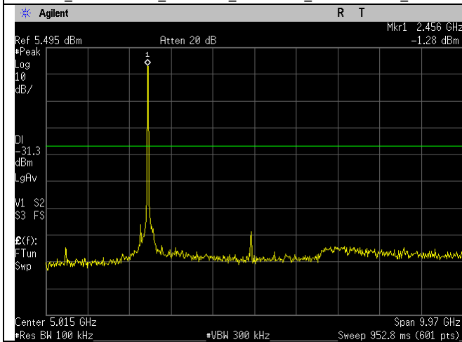
WIFI_2462MHz_20MHz_n-mode_30MHz-10GHz_Ant A
