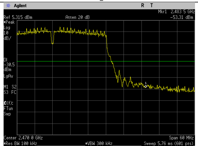
WIFI_2452MHz_40MHz_n-mode_Upper Band Edge_Ant B
