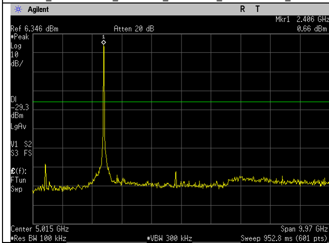
WIFI_2412MHz_20MHz_n-mode_30MHz-10GHz_Ant A
