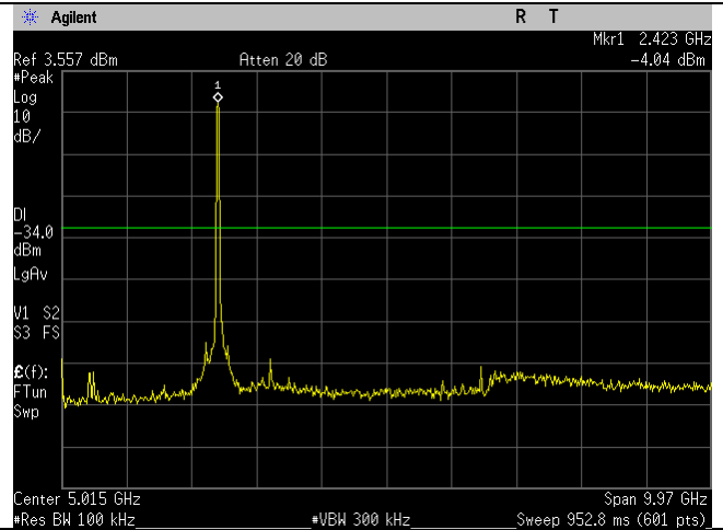
WIFI_2422MHz_40MHz_n-mode_30MHz-10GHz_Ant B
