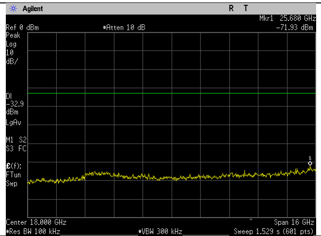
WIFI_2412MHz_20MHz_n-mode_10-26GHz_Ant B
