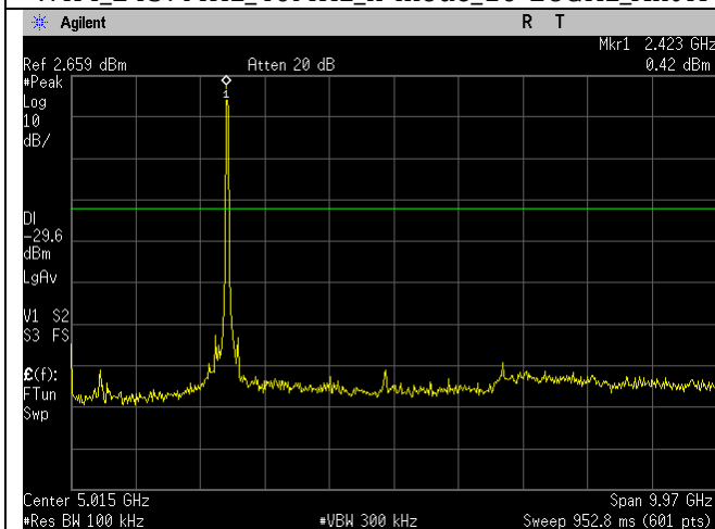
WIFI_2437MHz_40MHz_n-mode_30MHz-10GHz_Ant A
