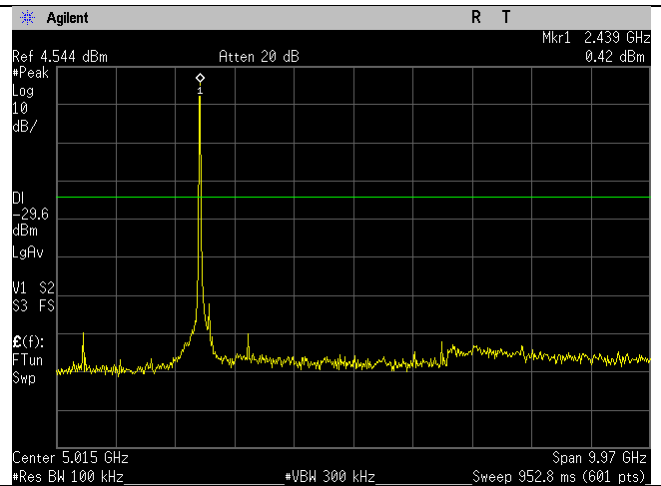
WIFI_2437MHz_20MHz_g-mode_30MHz- 10GHz_Ant B
