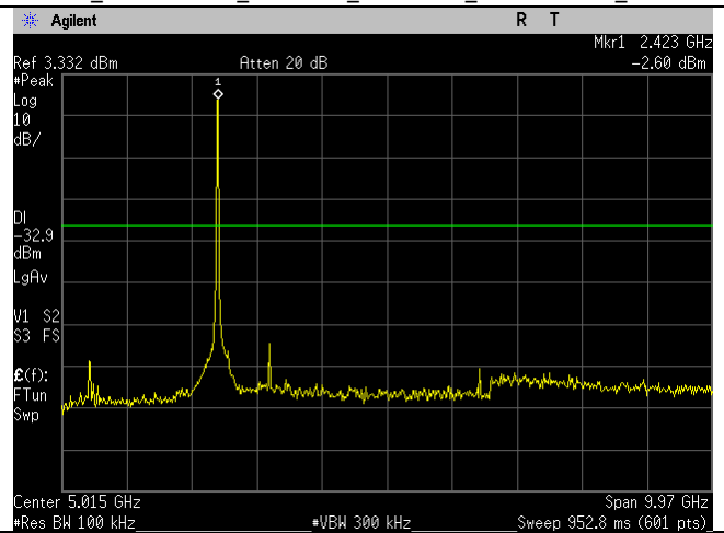
WIFI_2412MHz_20MHz_n-mode_30MHz-10GHz_Ant B
