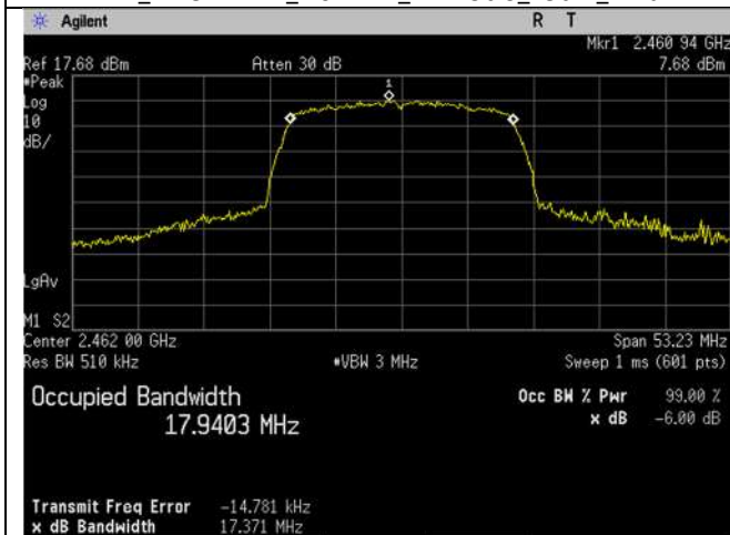
WIFI_2462MHz_20MHz_n-mode_99 percent_Ant A
