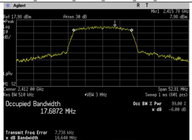
WIFI_2412MHz_20MHz_n-mode_99 percent_Ant B
