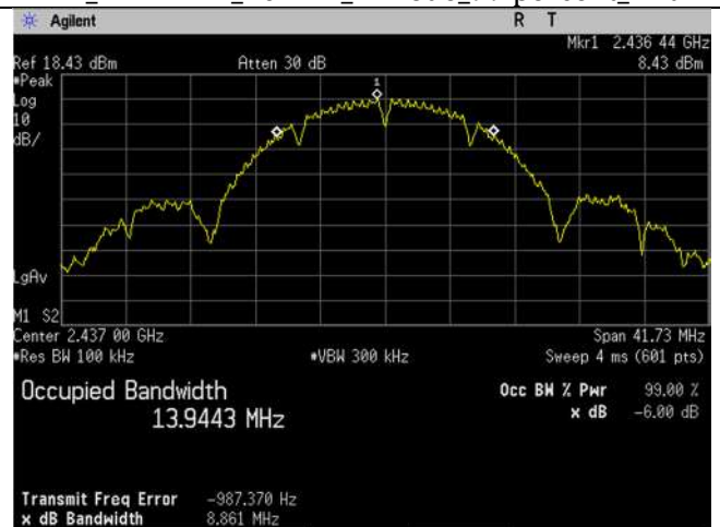
WIFI_2437MHz_20MHz_b-mode -6dB Ant B
