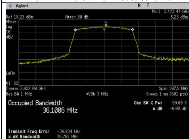
WIFI_2422MHz_40MHz_n-mode_99 percent Ant A
