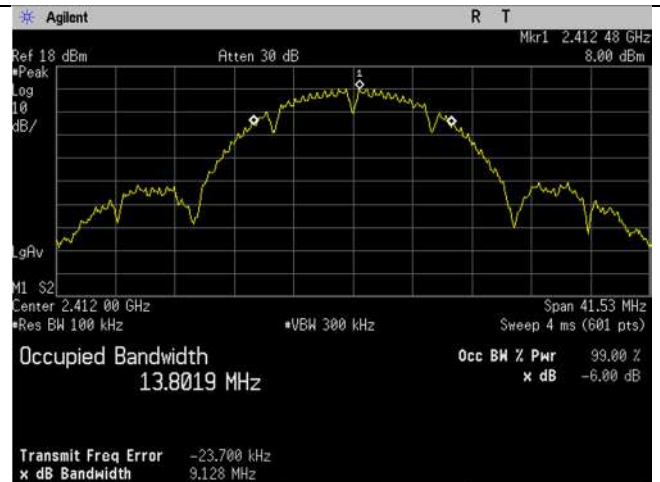
WIFI_2412MHz_20MHz_b-mode -6dB Ant B
