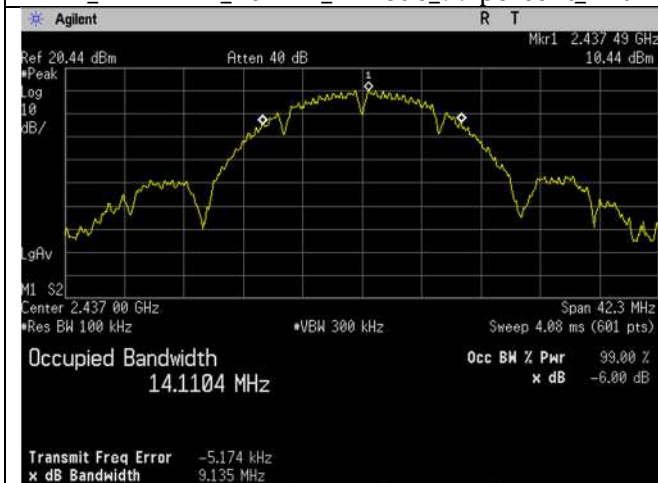
WIFI_2437MHz_20MHz_b-mode -6dB Ant A
