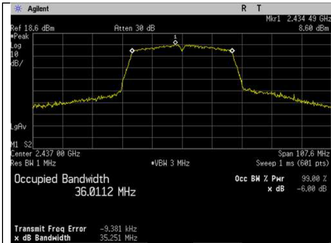
WIFI_2437MHz_40MHz_n-mode_99 percent_Ant A
