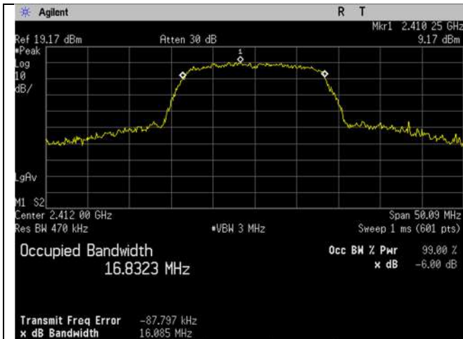
WIFI_2412MHz_20MHz_g-mode_99 percent_Ant A
