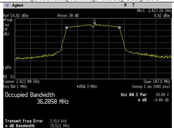
WIFI_2422MHz_40MHz_n-mode_99 percent Ant B
