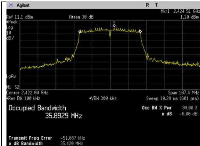
WIFI_2422MHz_40MHz_n-mode -6dB Ant A
