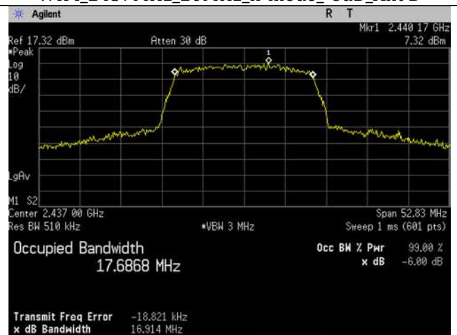
WIFI_2437MHz_20MHz_n-mode_99 percent Ant B
