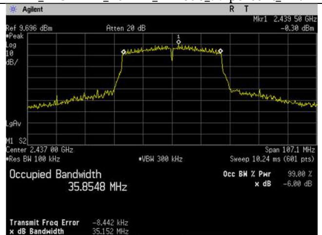
WIFI_2437MHz_40MHz_n-mode -6dB Ant B
