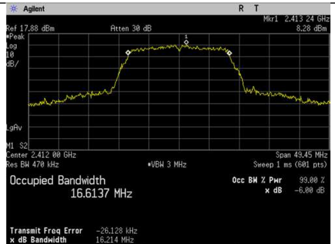
WIFI_2412MHz_20MHz_g-mode_99 percent_Ant B
