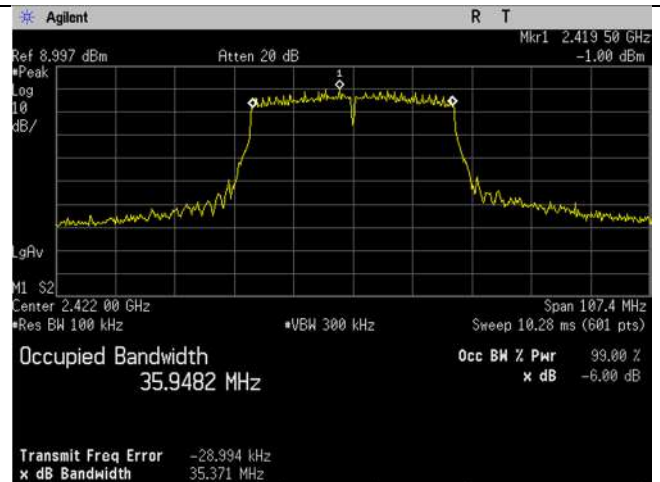
WIFI_2422MHz_40MHz_n-mode -6dB Ant B
