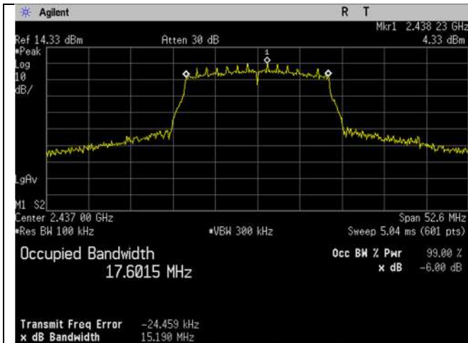
WIFI_2437MHz_20MHz_n-mode -6dB Ant A
