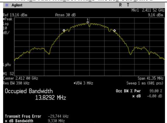
WIFI_2412MHz_20MHz_b-mode_99 percent Ant B
