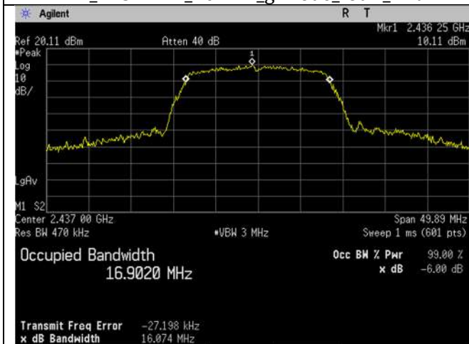
WIFI_2437MHz_20MHz_g-mode_99 percent_Ant A
