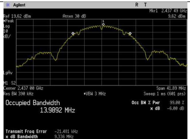
WIFI_2437MHz_20MHz_b-mode_99 percent_Ant B
