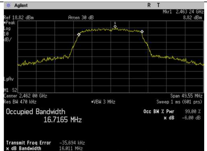
WIFI_2462MHz_20MHz_g-mode_99 percent_Ant B
