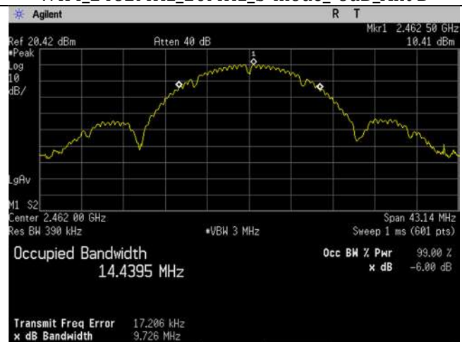
WIFI_2462MHz_20MHz_b-mode_99 percent Ant B
