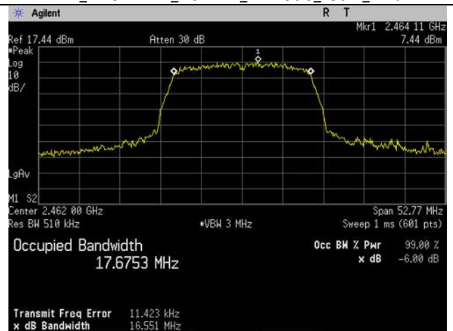
WIFI_2462MHz_20MHz_n-mode_99 percent_Ant B
