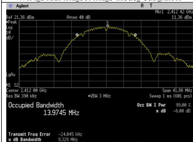
WIFI_2412MHz_20MHz_b-mode_99 percent Ant A
