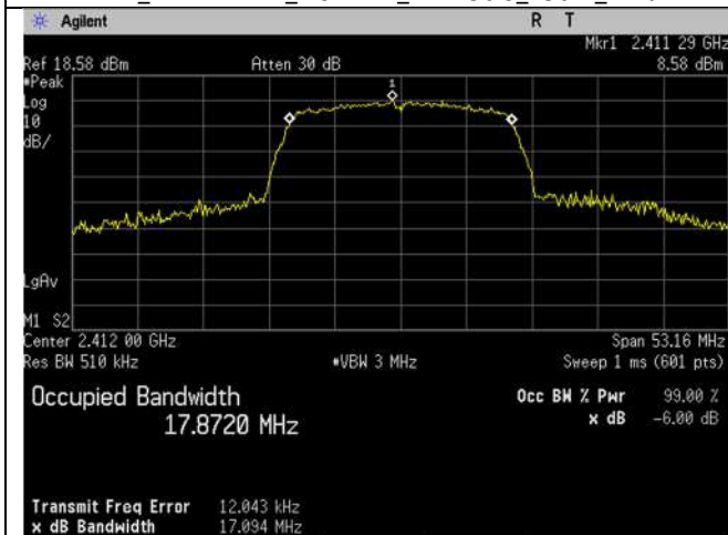
WIFI_2412MHz_20MHz_n-mode_99 percent_Ant A
