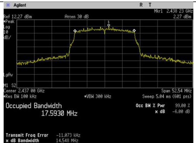
WIFI_2437MHz_20MHz_n-mode -6dB Ant B
