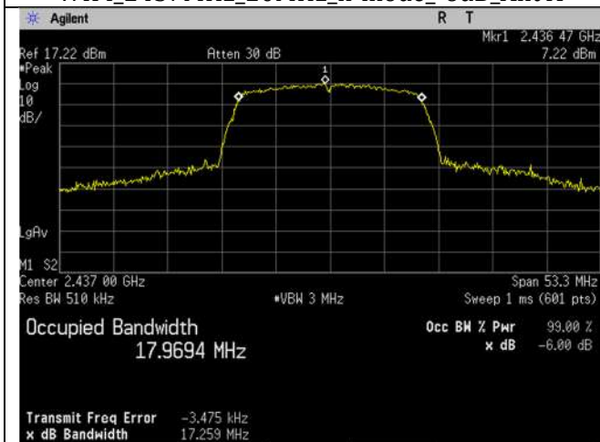
WIFI_2437MHz_20MHz_n-mode_99 percent Ant A
