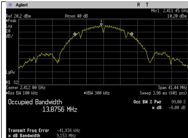
WIFI_2412MHz_20MHz_b-mode -6dB Ant A
