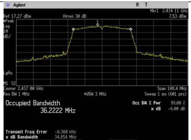
WIFI_2437MHz_40MHz_n-mode_99 percent_Ant B
