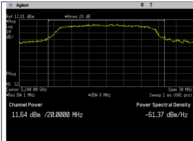
5240MHz_a-mode_Channel Power_Ant B
