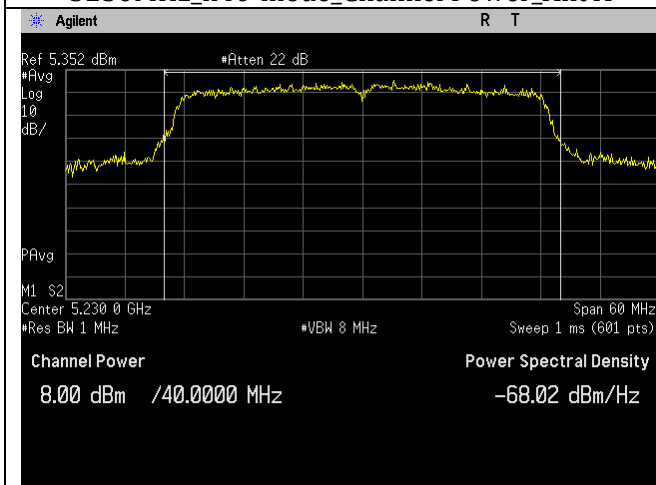
5230MHz_n40-mode_Channel Power_Ant B
