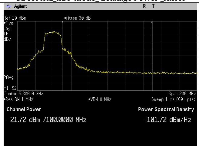
5240MHz_n20-mode_Leakage Power_Ant B
