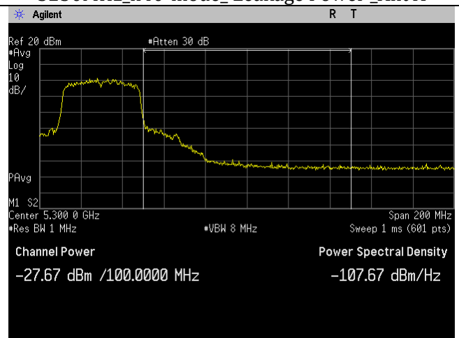
5230MHz_n40-mode_Leakage Power_Ant B
