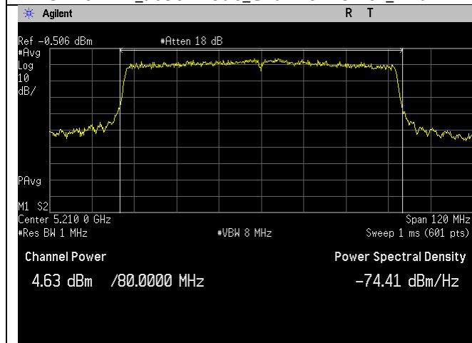
5210MHz_ac80-mode_Channel Power_Ant B
