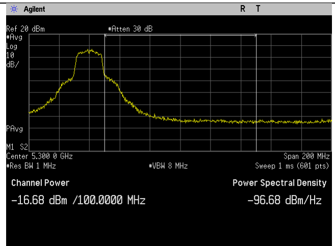
5240MHz_a-mode_Leakage Power_Ant B
