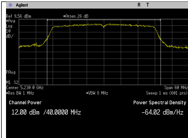
5230MHz_n40-mode_Channel Power_Ant A
