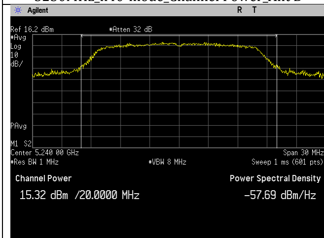
5240MHz_a-mode_Channel Power_Ant A
