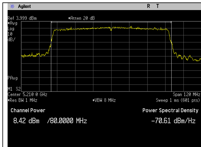
5210MHz_ac80-mode_Channel Power_Ant A
