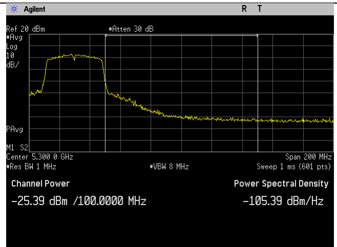
5230MHz_n40-mode_Leakage Power_Ant A
