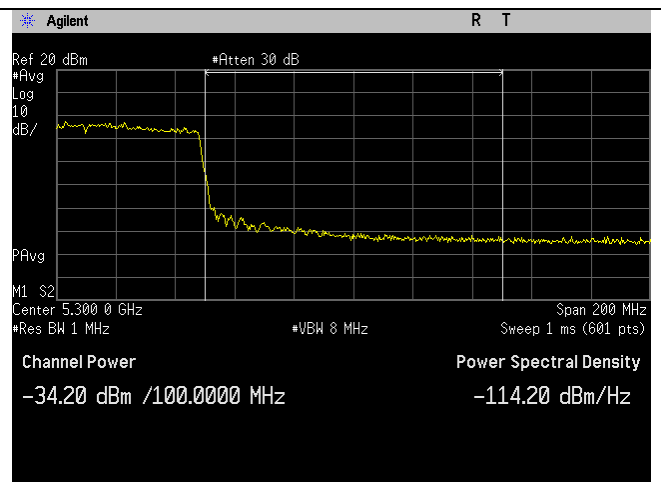
5210MHz_ac80-mode_Leakage Power_Ant A
