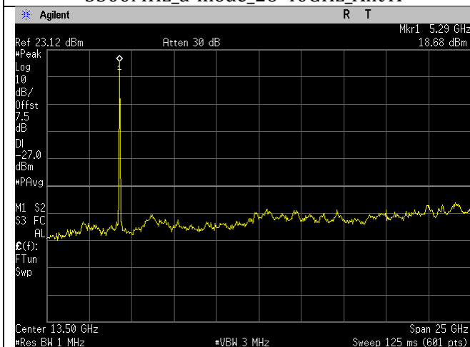
5300MHz_n20-mode_1-26GHz_Ant A
