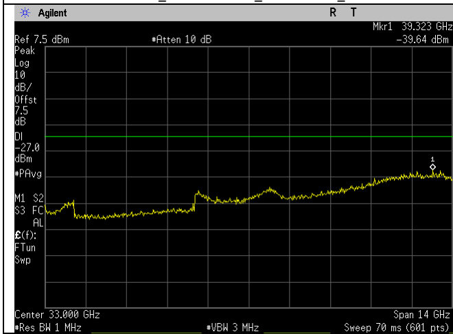
5260MHz_n20-mode_26-40GHz_Ant A
