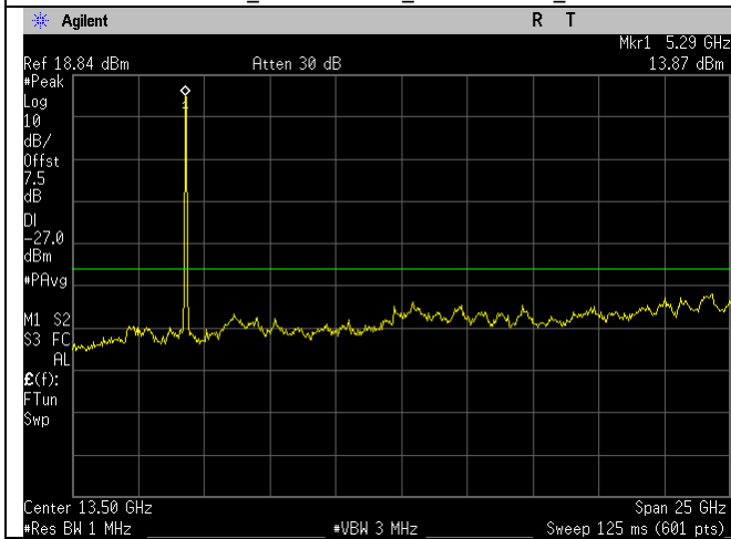
5310MHz_n40-mode_1-26GHz_Ant A
