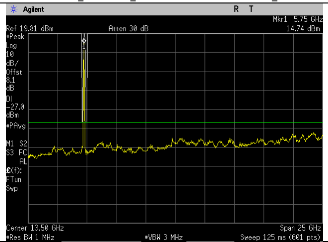
5745MHz_n20-mode_1-26GHz_Ant B
