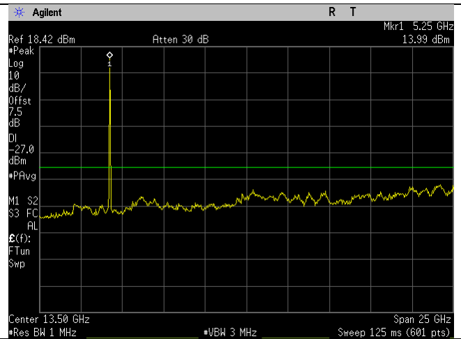
5260MHz_n20-mode_1-26GHz_Ant B
