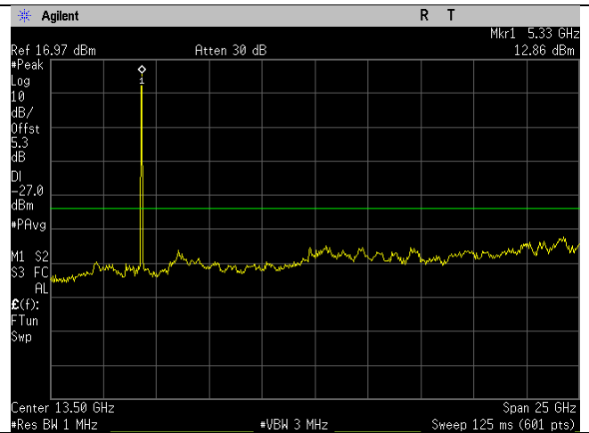
5320MHz_a-mode_1-26GHz_Ant B
