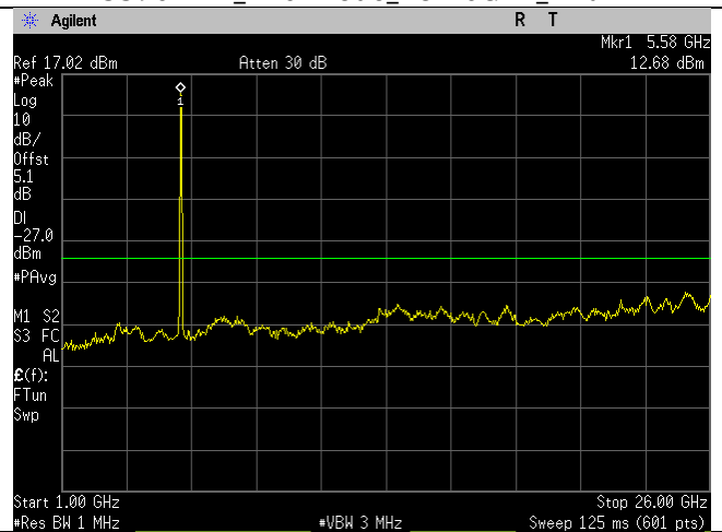
5600MHz_a-mode_1-26GHz_Ant B
