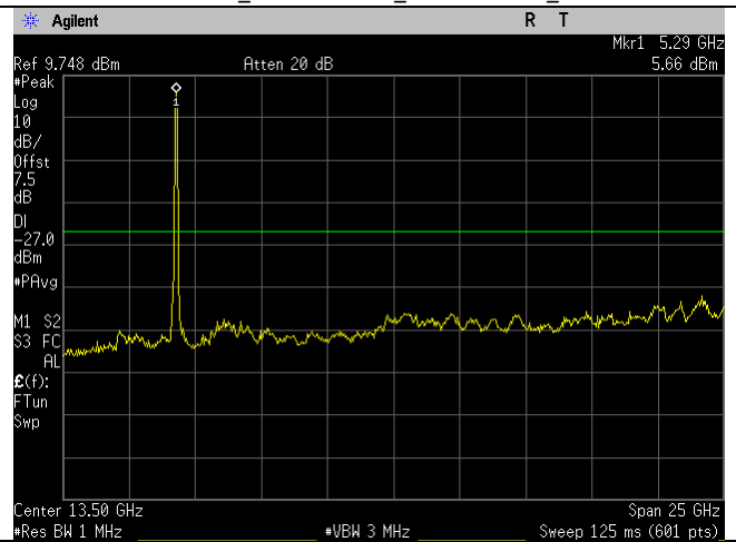
5290MHz_ac80-mode_1-26GHz_Ant B
