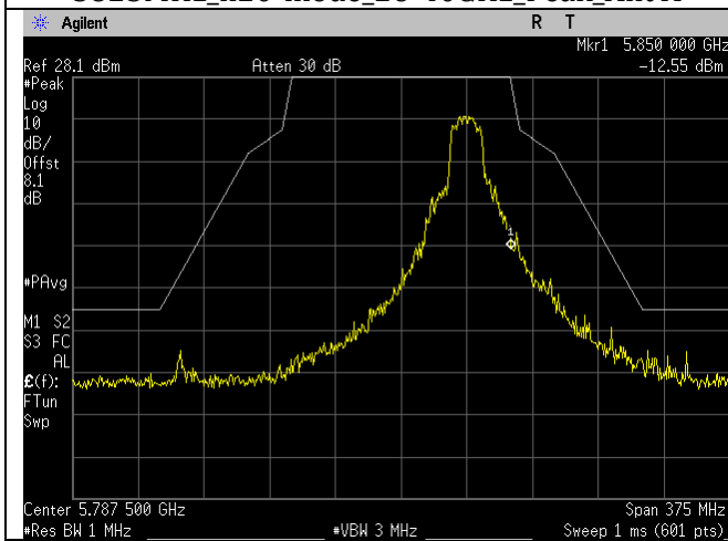
5825MHz_n20-mode_Upper Emission Mask_Ant A
