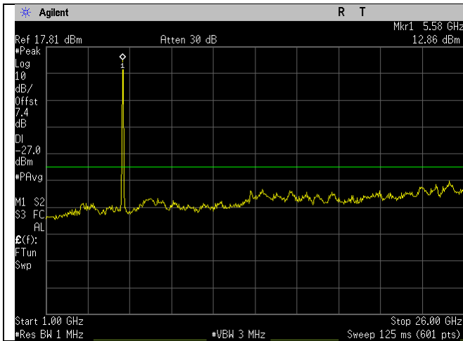
5590MHz_n40-mode_1-26GHz_Ant A
