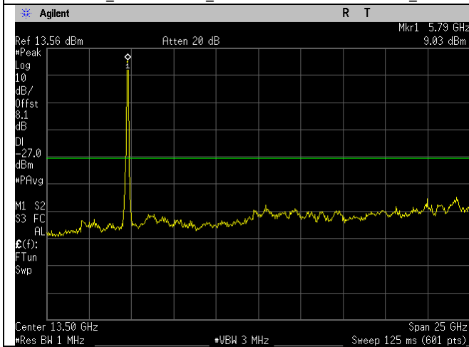
5755MHz_ac80-mode_1-26GHz_Ant A
