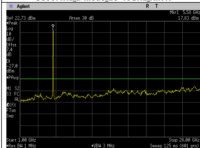
5600MHz_n20-mode_1-26GHz_Ant A
