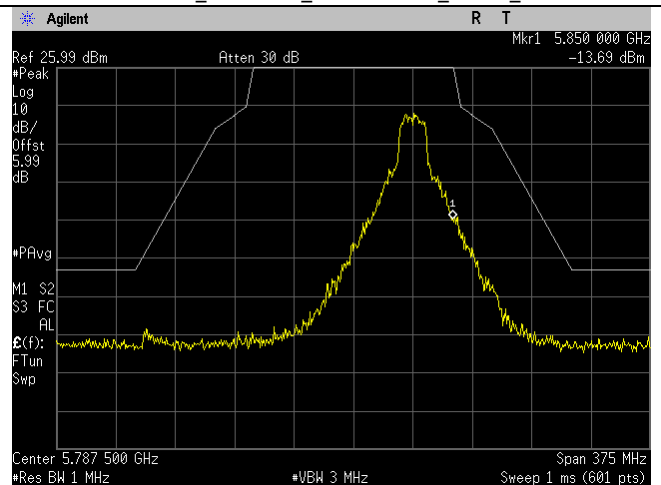
5825MHz_a-mode_Upper Emission Mask_Ant B
