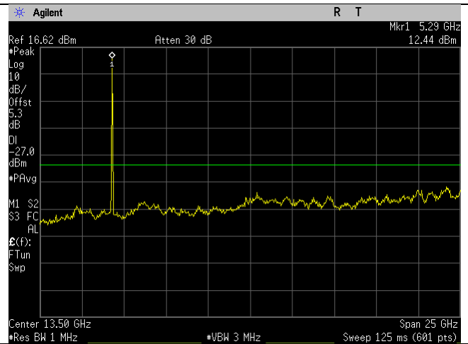
5300MHz_a-mode_1-26GHz_Ant B
