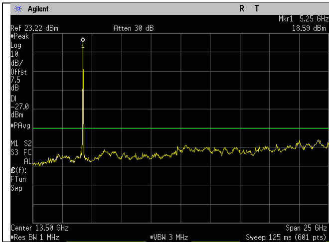
5260MHz_n20-mode_1-26GHz_Ant A
