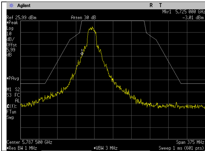
5745MHz_a-mode_Lower Emission Mask_Ant A
