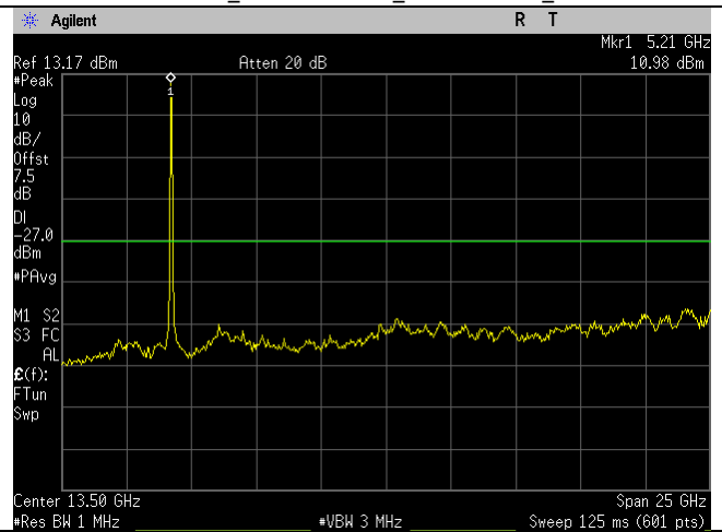
5230MHz_n40-mode_1-26GHz Ant B
