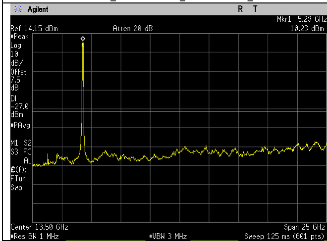
5290MHz_ac80-mode_1-26GHz_Ant A
