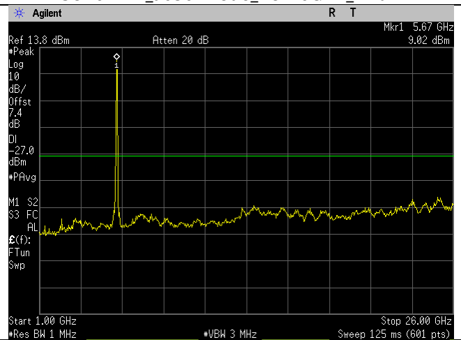
5670MHz_n40-mode_1-26GHz_Ant B
