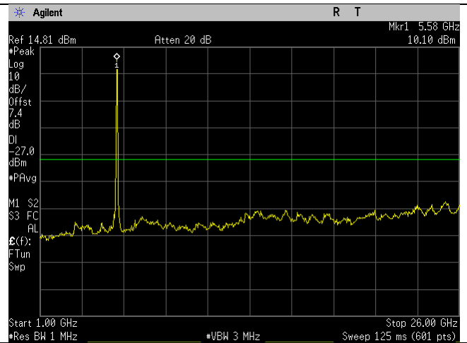
5590MHz_n40-mode_1-26GHz_Ant B
