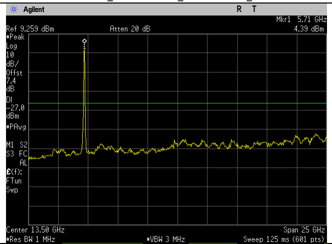
5690MHz_ac80-mode_1-26GHz_Ant B
