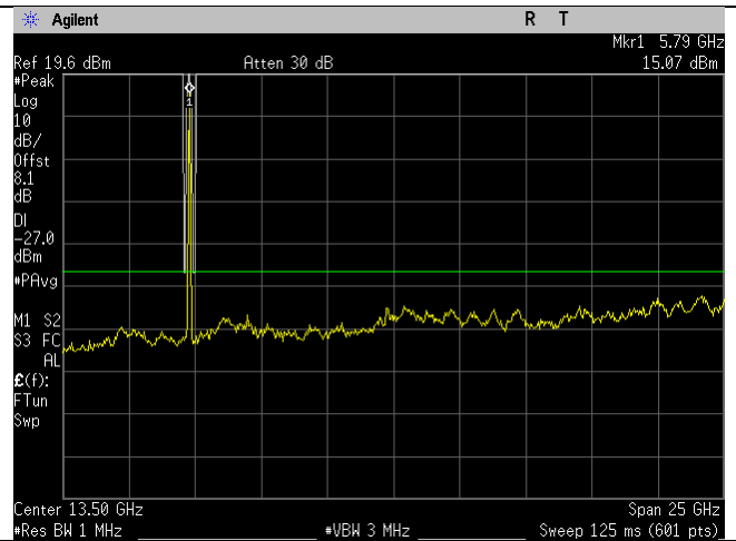
5785MHz_n20-mode_1-26GHz_Ant B
