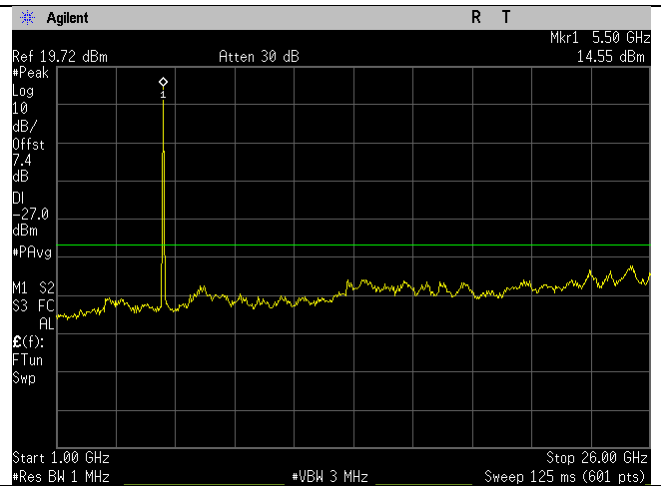
5500MHz_n20-mode_1-26GHz_Ant B
