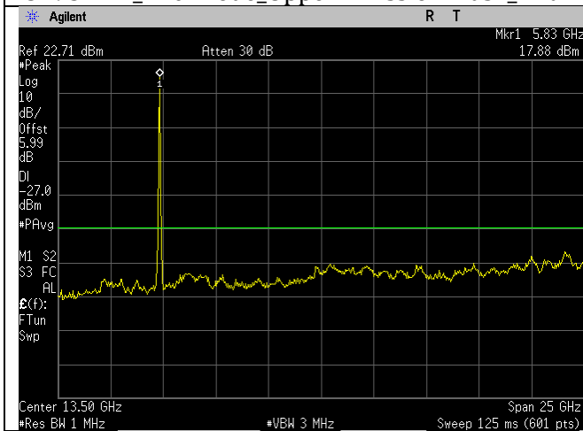
5825MHz_a-mode_1-26GHz_Ant A
