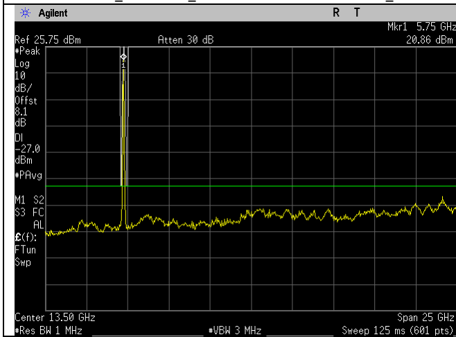
5745MHz_n20-mode_1-26GHz_Ant A
