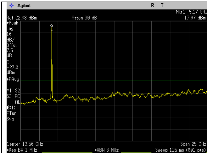
5180MHz_n20-mode_1-26GHz_Ant A
