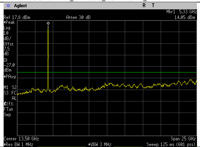
5320MHz_n20-mode_1-26GHz_Ant B
