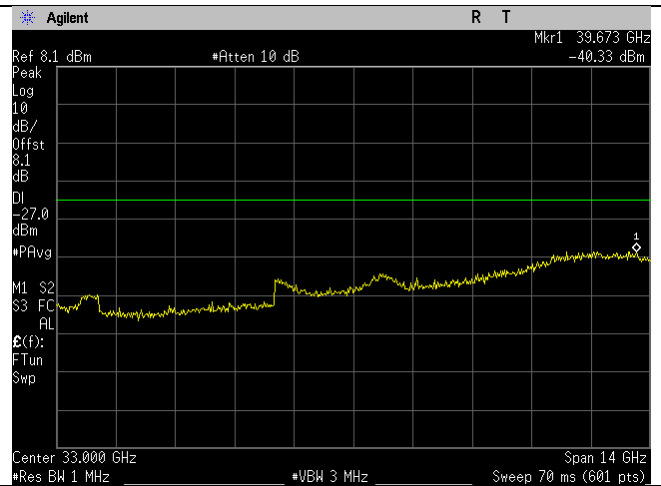
5795MHz_n40-mode_26-40GHz_Peak_Ant B
