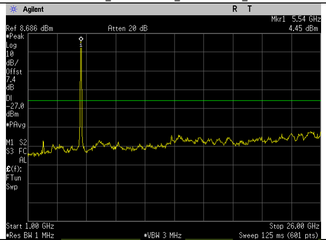
5530MHz_ac80-mode_1-26GHz_Ant B
