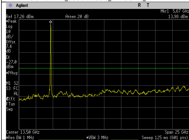
5670MHz_n40-mode_1-26GHz_Ant A
