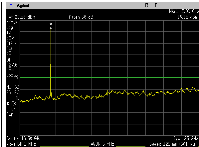
5320MHz_a-mode_1-26GHz_Ant A
