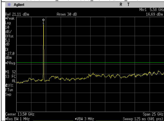
5600MHz_a-mode_1-26GHz_Ant A
