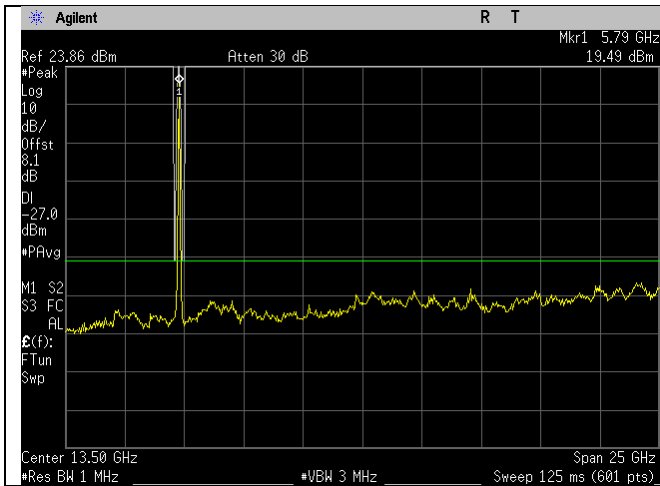
5785MHz_n20-mode_1-26GHz_Ant A
