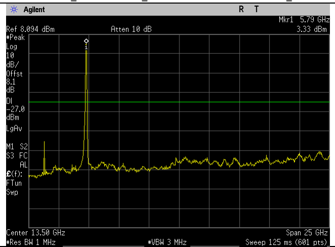
5755MHz_ac80-mode_1-26GHz_Ant B
