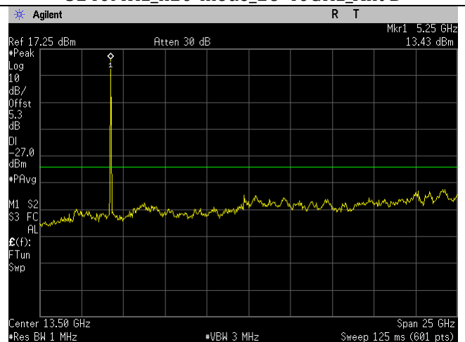
5260MHz_a-mode_1-26GHz_Ant B
