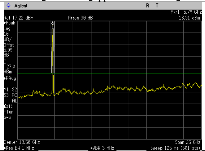
5785MHz_a-mode_1-26GHz_Ant B
