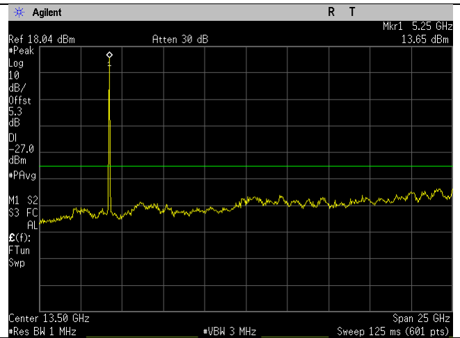
5240MHz_a-mode_1-26GHz_Ant B
