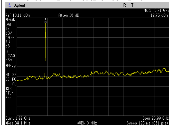
5710MHz_n40-mode_1-26GHz_Ant A
