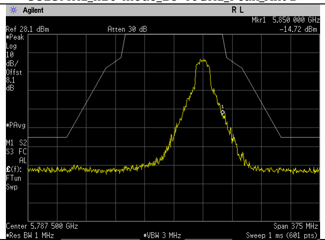
5825MHz_n20-mode_Upper Emission Mask_Ant B
