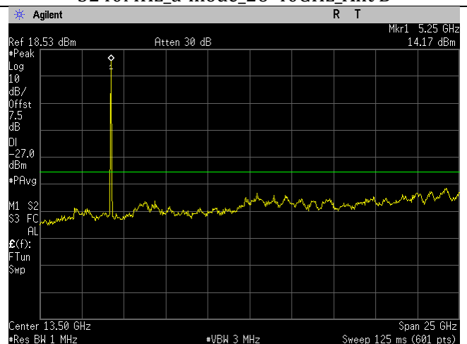
5240MHz_n20-mode_1-26GHz_Ant B
