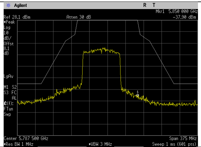
5775MHz_ac80-mode_Upper Emission Mask Ant B
