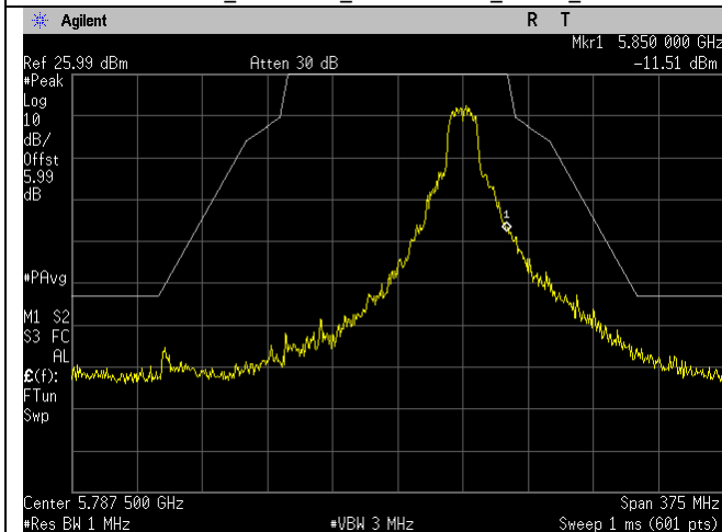
5825MHz_a-mode_Upper Emission Mask_Ant A
