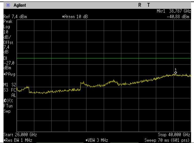
5670MHz_n40-mode_26-40GHz_Ant B
