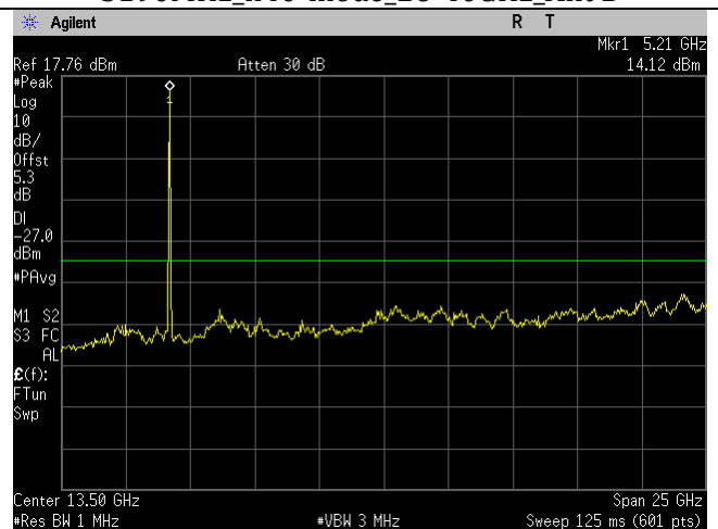
5200MHz_a-mode_1-26GHz_Ant B
