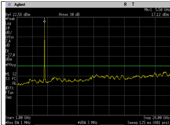
5500MHz_n20-mode_1-26GHz_Ant A
