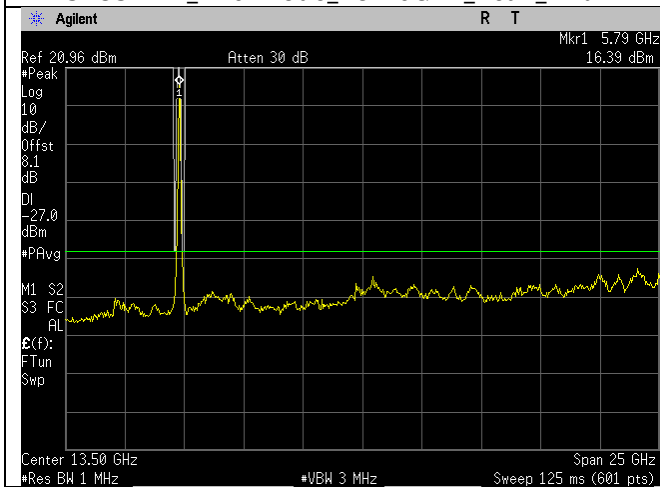
5795MHz_n40-mode_1-26GHz_Ant A
