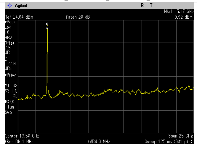
5190MHz_n40-mode_1-26GHz_Ant B
