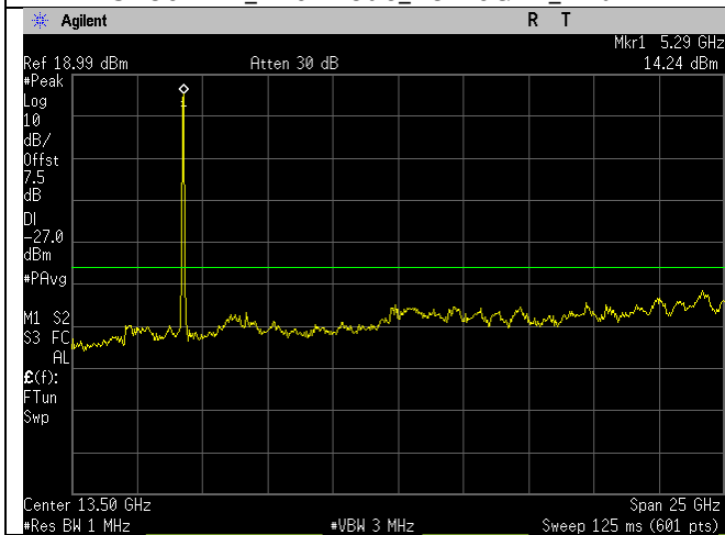
5270MHz_n40-mode_1-26GHz_Ant A
