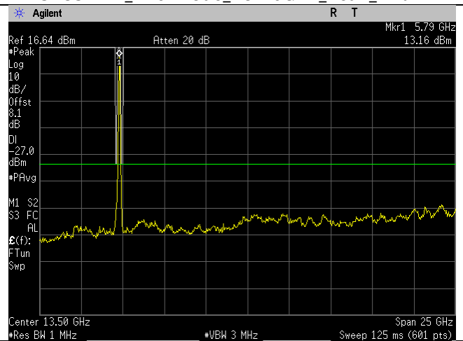
5795MHz_n40-mode_1-26GHz_Ant B
