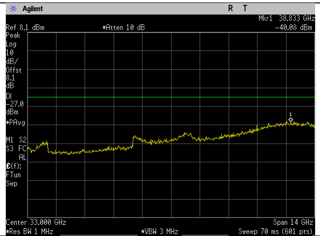
5825MHz_n20-mode_26-40GHz_Peak_Ant B
