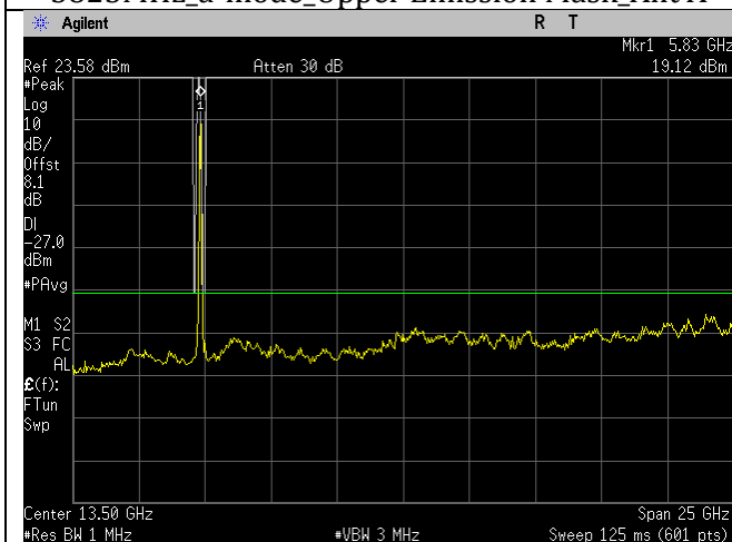
5825MHz_n20-mode_1-26GHz_Ant A
