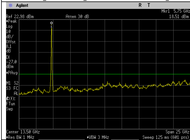
5755MHz_n40-mode_1-26GHz_Ant A
