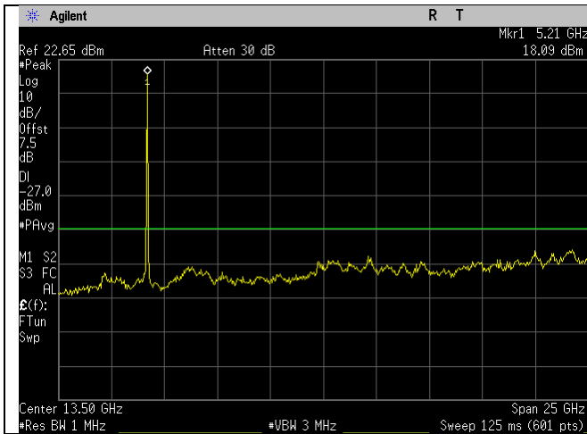
5200MHz_n20-mode_1-26GHz_Ant A
