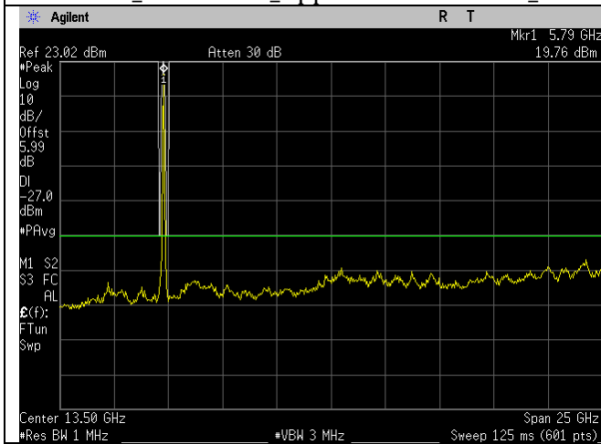
5785MHz_a-mode_1-26GHz_Ant A
