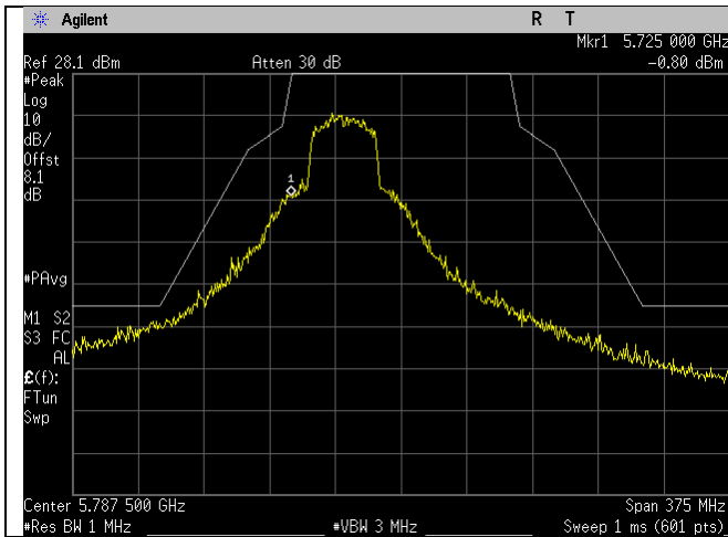
5755MHz_n40-mode_Lower Emission Mask_Ant A
