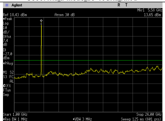
5600MHz_n20-mode_1-26GHz_Ant B
