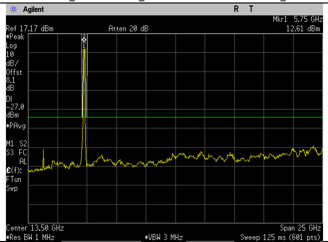
5755MHz_n40-mode_1-26GHz_Ant B
