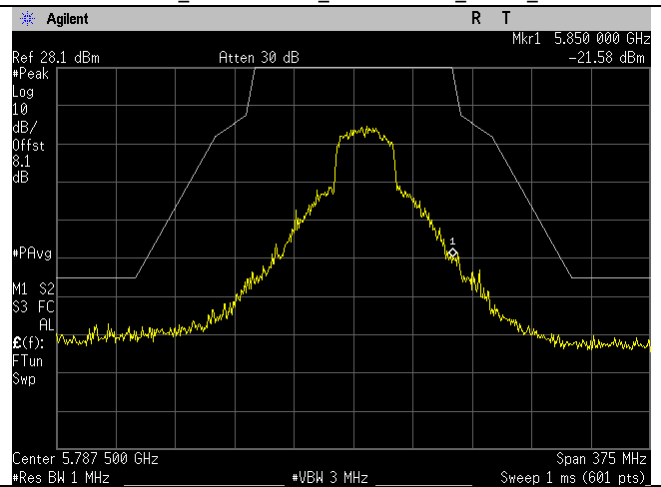
5795MHz_n40-mode_Upper Emission Mask_Ant B
