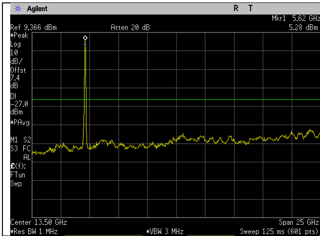
5610MHz_ac80-mode_1-26GHz_Ant B
