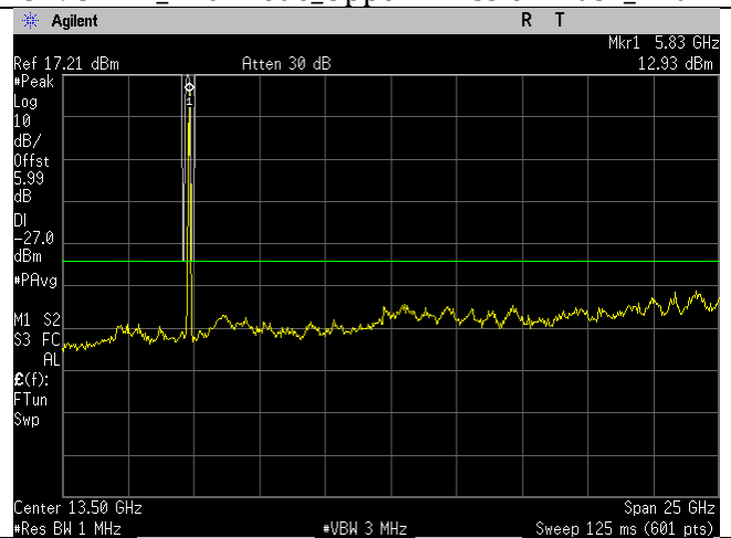
5825MHz_a-mode_1-26GHz_Ant B
