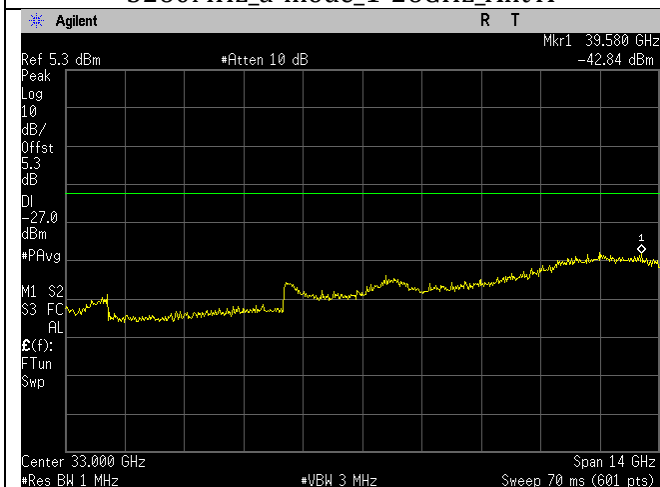
5260MHz_a-mode_26-40GHz_Ant A
