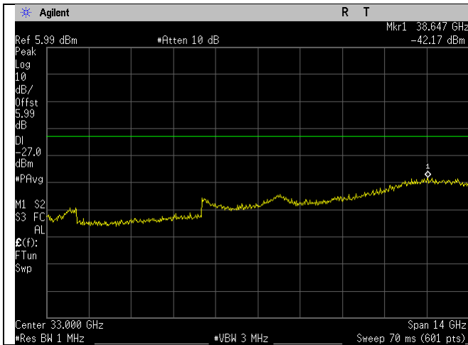
5825MHz_a-mode_26-40GHz_Peak_Ant A
