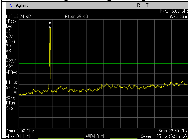
5610MHz_ac80-mode_1-26GHz_Ant A
