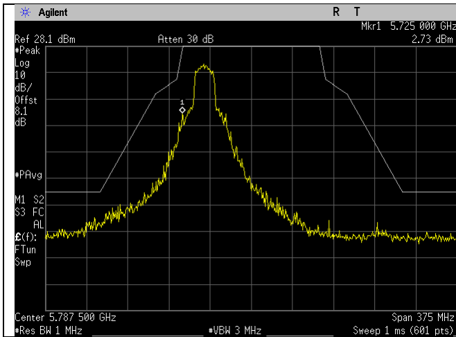
5745MHz_n20-mode_Lower Emission Mask_Ant A
