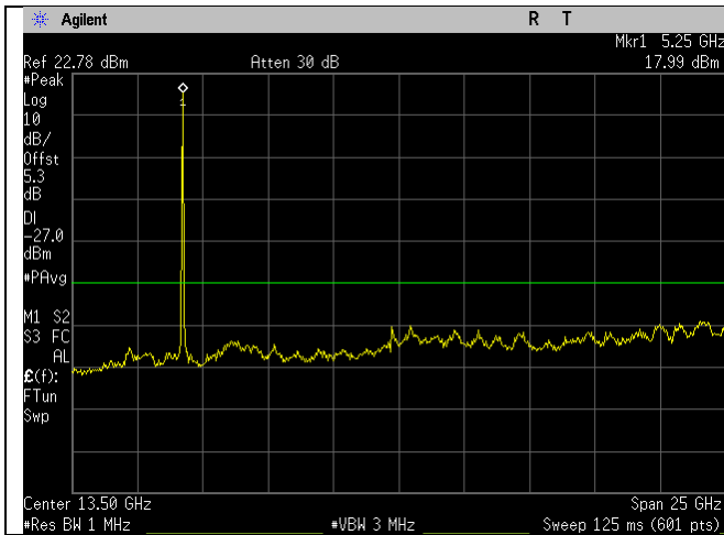
5240MHz_a-mode_1-26GHz_Ant A
