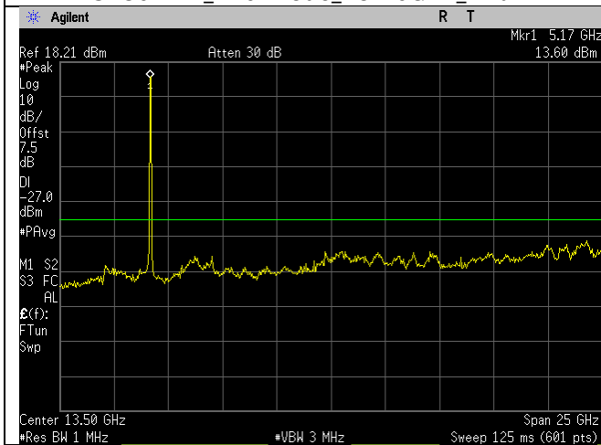
5190MHz_n40-mode_1-26GHz_Ant A
