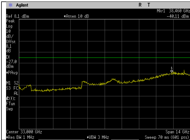
5795MHz_n40-mode_26-40GHz_Peak_Ant A
