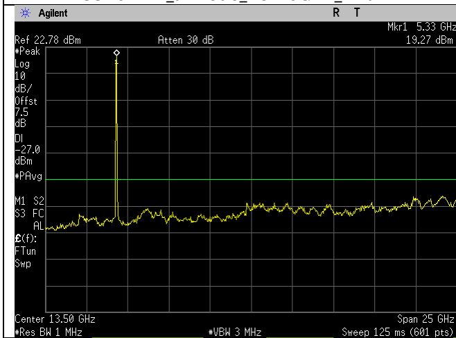
5320MHz_n20-mode_1-26GHz_Ant A
