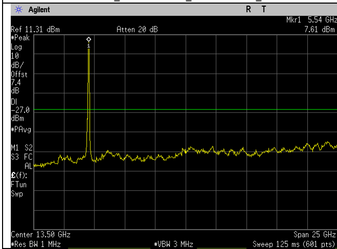
5530MHz_ac80-mode_1-26GHz_Ant A
