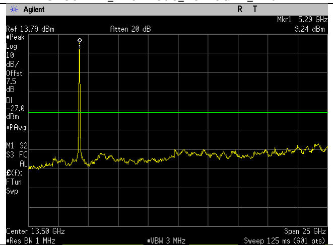
5270MHz_n40-mode_1-26GHz_Ant B
