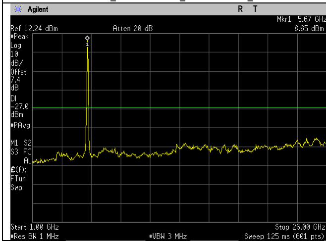
5690MHz_ac80-mode_1-26GHz_Ant A
