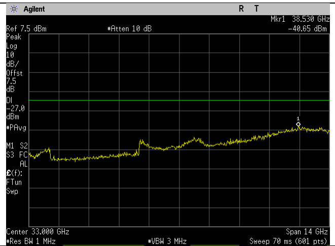
5240MHz_n20-mode_26-40GHz_Ant B
