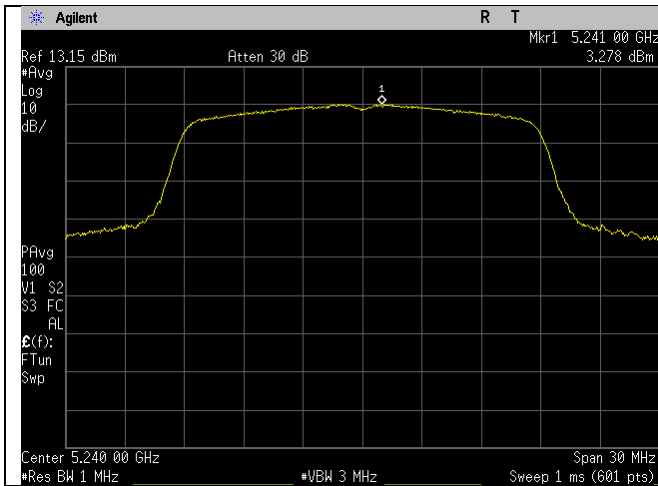
5240MHzCh_48_n20-mode_Ant A
