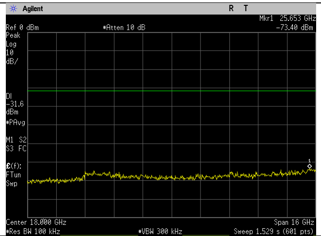
WIFI_2412MHz_g-mode_10-26GHz_Ant B
