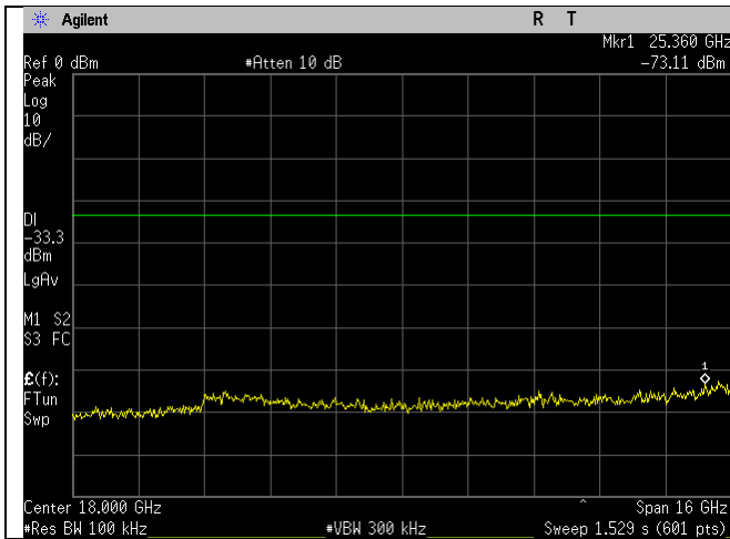
WIFI_2462MHz_n20-mode_10-26GHz_Ant A
