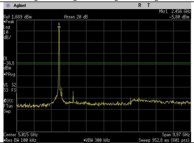
WIFI_2452MHz_n40-mode_30MHz-10GHz_Ant B
