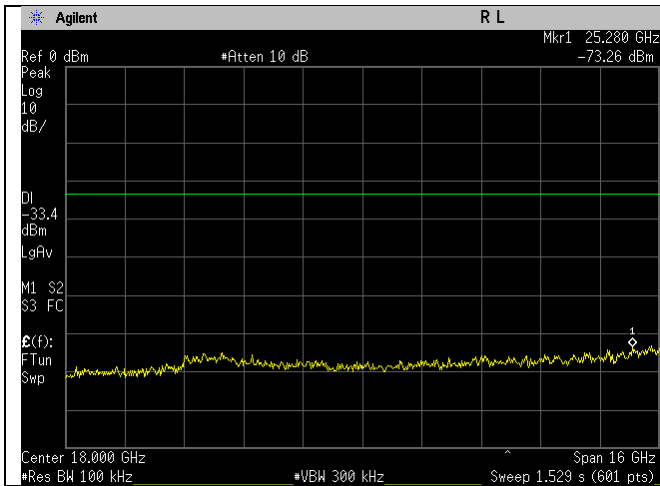
WIFI_2437MHz_n40-mode_10-26GHz_Ant A
