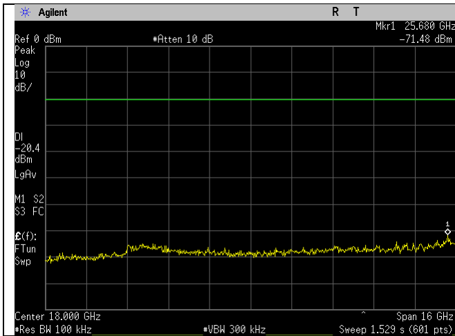
WIFI_2437MHz_b-mode_10-26GHz_Ant A
