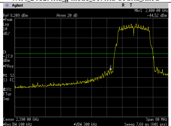
WIFI_2412MHz_g-mode_Lower Band Edge_Ant B
