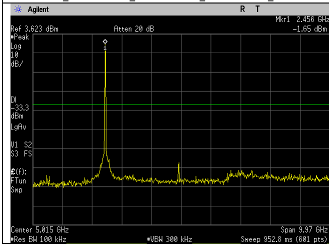
WIFI_2462MHz_n20-mode_30MHz-10GHz_Ant A
