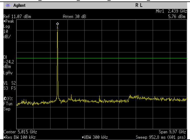
WIFI_2437MHz_b-mode_30MHz-10GHz_Ant B
