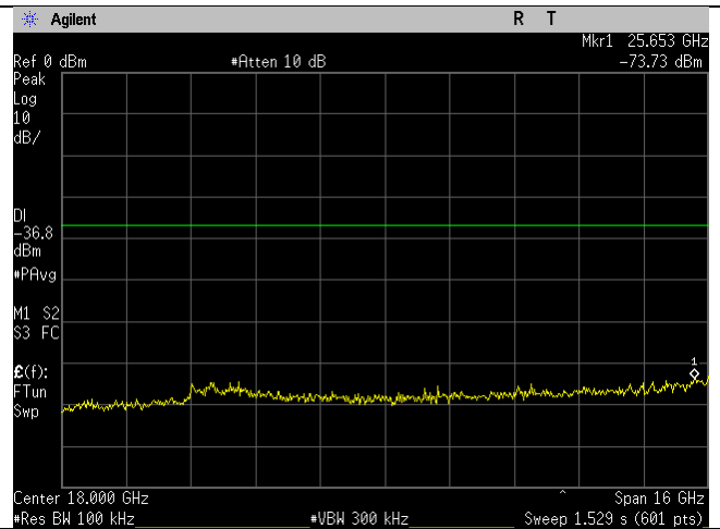
WIFI_2452MHz_n40-mode_10-26GHz_Ant B
