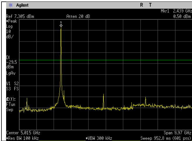
WIFI_2437MHz_g-mode_30MHz-10GHz_Ant A
