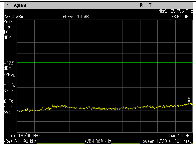
WIFI_2422MHz_n40-mode_10-26GHz_Ant B
