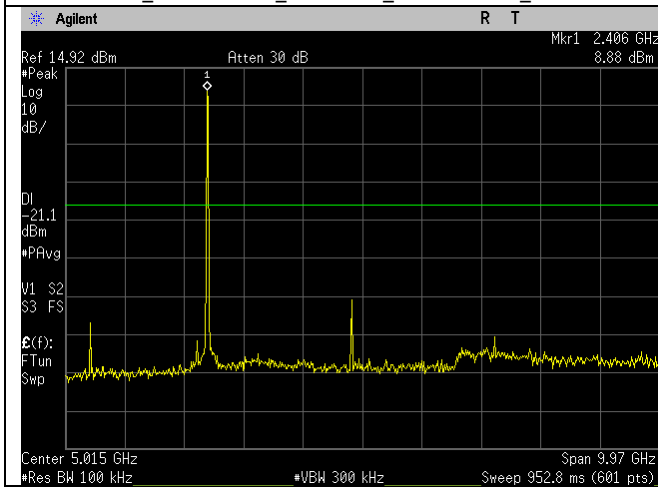
WIFI_2412MHz_b-mode_30MHz-10GHz_Ant A
