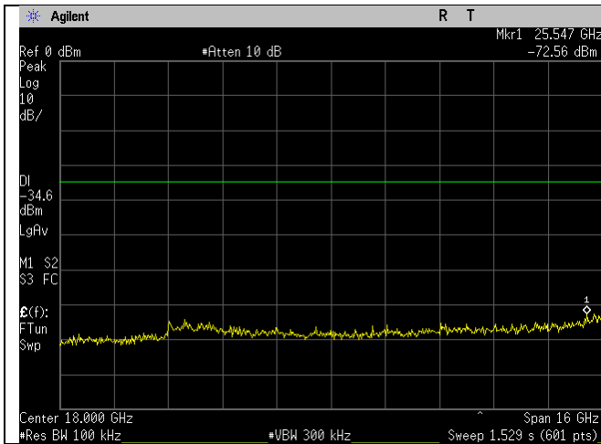
WIFI_2452MHz_n40-mode_10-26GHz_Ant A
