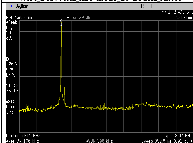
WIFI_2437MHz_n20-mode_30MHz-10GHz_Ant A
