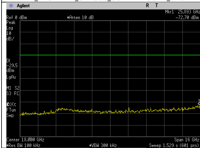
WIFI_2437MHz_g-mode_10-26GHz_Ant A
