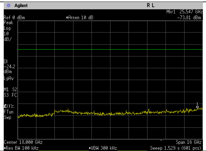
WIFI_2437MHz_b-mode_10-26GHz_Ant B
