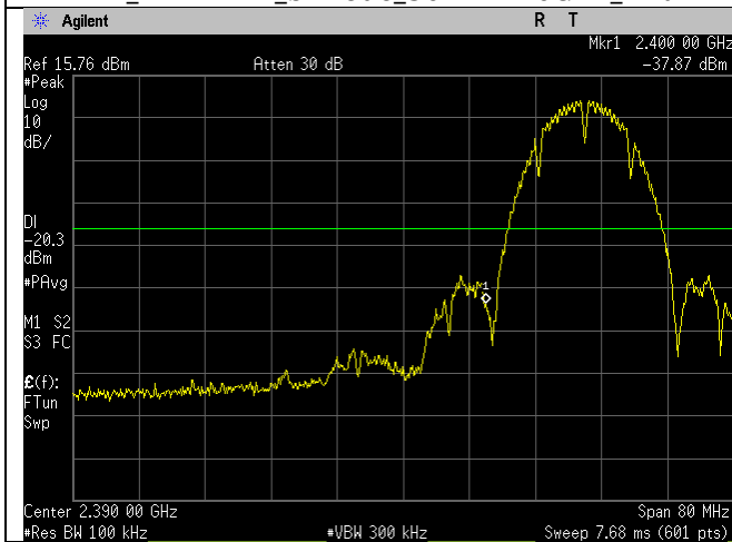
WIFI_2412MHz_b-mode_Lower Band Edge_Ant A
