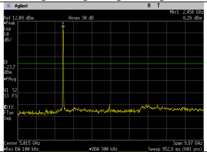
WIFI_2462MHz_b-mode_30MHz-10GHz Ant B
