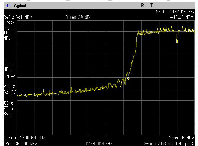
WIFI_2422MHz_n40-mode_Lower Band Edge_Ant
