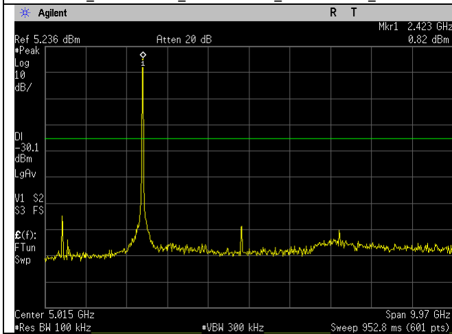
WIFI_2412MHz_n20-mode_30MHz-10GHz_Ant A
