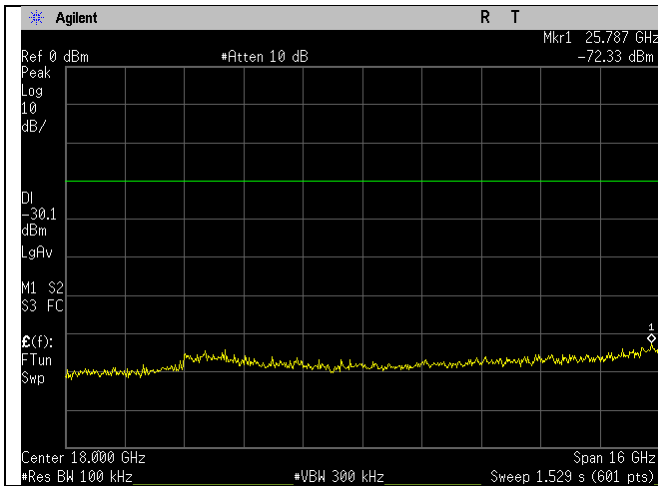
WIFI_2412MHz_n20-mode_10-26GHz_Ant A
