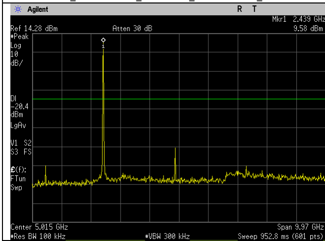
WIFI_2437MHz_b-mode_30MHz-10GHz_Ant A
