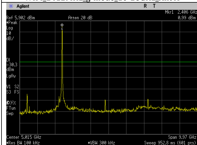
WIFI_2412MHz_g-mode_30MHz-10GHz_Ant A
