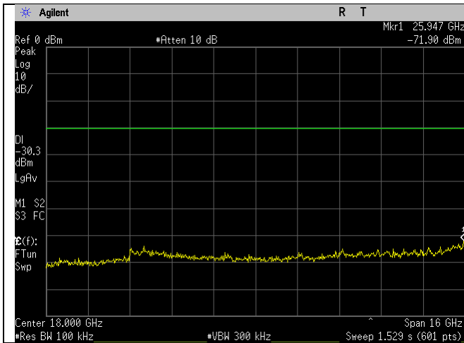
WIFI_2412MHz_g-mode_10-26GHz_Ant A
