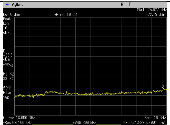
WIFI_2437MHz_n40-mode_10-26GHz_Ant B
