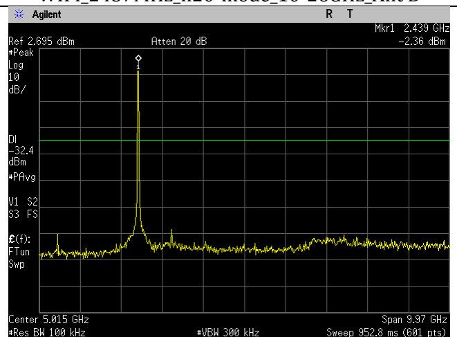
WIFI_2437MHz_n20-mode_30MHz-10GHz_Ant B
