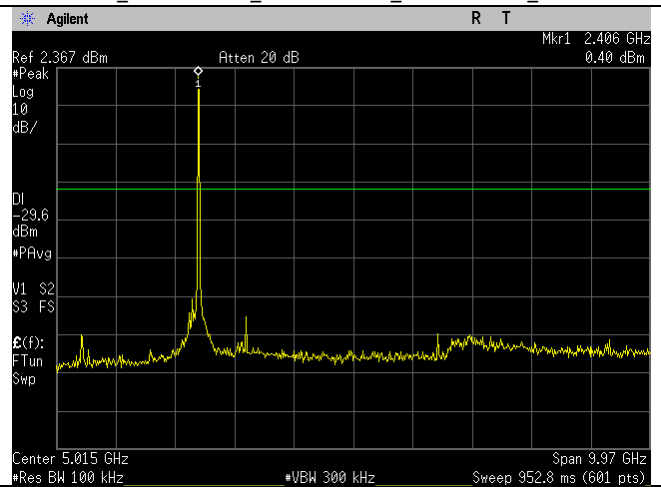
WIFI_2412MHz_n20-mode_30MHz-10GHz_Ant B
