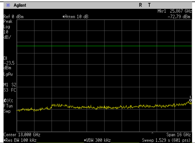
WIFI_2412MHz_b-mode_10-26GHz_Ant B
