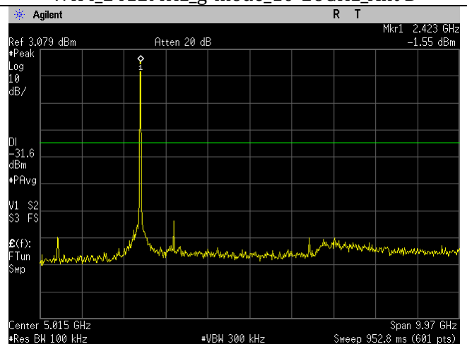
WIFI_2412MHz_g-mode_30MHz-10GHz_Ant B
