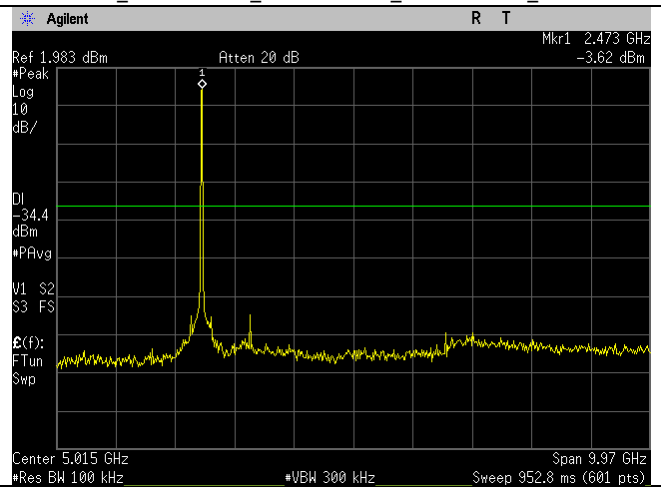
WIFI_2462MHz_n20-mode_30MHz-10GHz_Ant B
