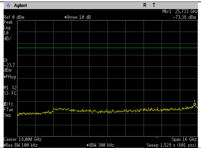
WIFI_2462MHz_b-mode_10-26GHz Ant B
