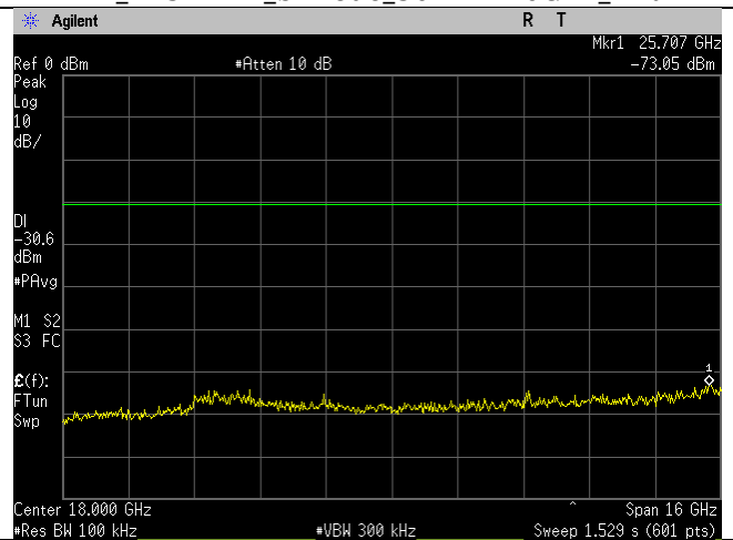
WIFI_2437MHz_g-mode_10-26GHz_Ant B
