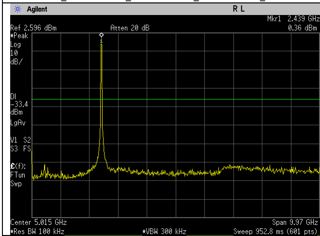
WIFI_2437MHz_n40-mode_30MHz-10GHz_Ant A
