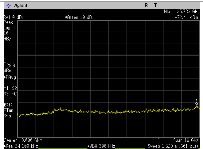
WIFI_2412MHz_n20-mode_10-26GHz_Ant B
