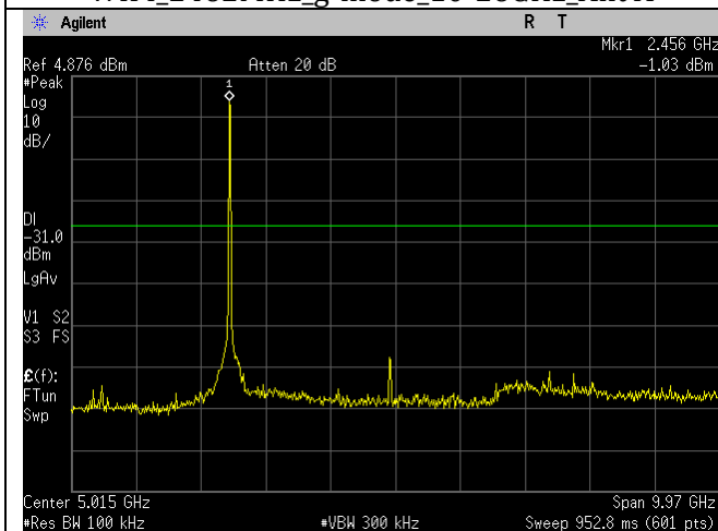
WIFI_2462MHz_g-mode_30MHz-10GHz_Ant A
