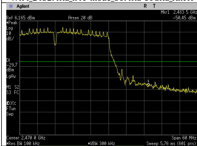
WIFI_2452MHz_n40-mode_Upper Band Edge_Ant
