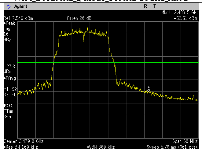
WIFI_2462MHz_g-mode_Upper Band_Edge_Ant B
