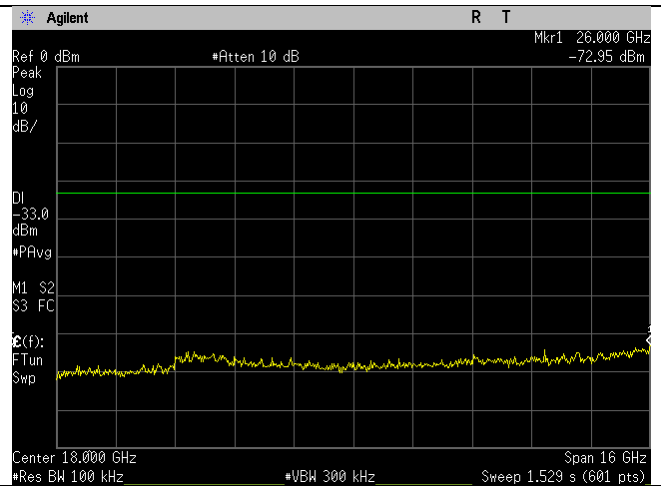
WIFI_2462MHz_g-mode_10-26GHz_Ant B
