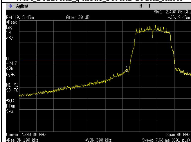
WIFI_2412MHz_g-mode_Lower Band Edge_Ant A
