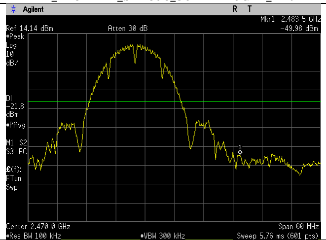
WIFI_2462MHz_b-mode_Upper Band Edge Ant B
