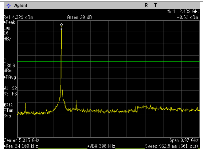
WIFI_2437MHz_g-mode_30MHz-10GHz_Ant B
