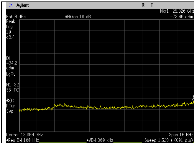
WIFI_2422MHz_n40-mode_10-26GHz_Ant A
