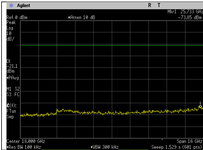
WIFI_2412MHz_b-mode_10-26GHz_Ant A
