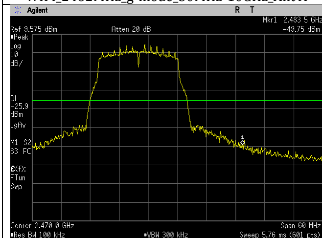
WIFI_2462MHz_g-mode_Upper Band_Edge_Ant A
