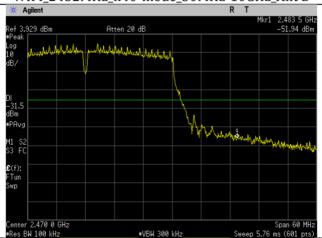
WIFI_2452MHz_n40-mode_Upper Band Edge_Ant
