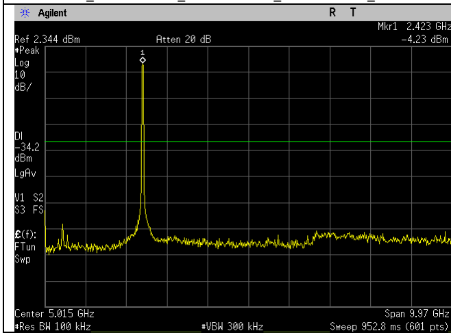
WIFI_2422MHz_n40-mode_30MHz-10GHz_Ant A
