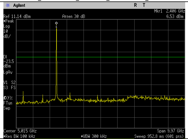
WIFI_2412MHz_b-mode_30MHz-10GHz_Ant B
