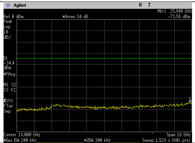
WIFI_2462MHz_n20-mode_10-26GHz_Ant B
