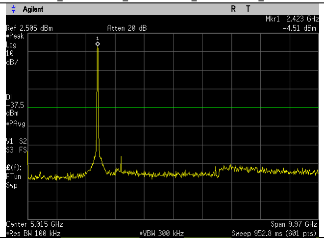
WIFI_2422MHz_n40-mode_30MHz-10GHz_Ant B
