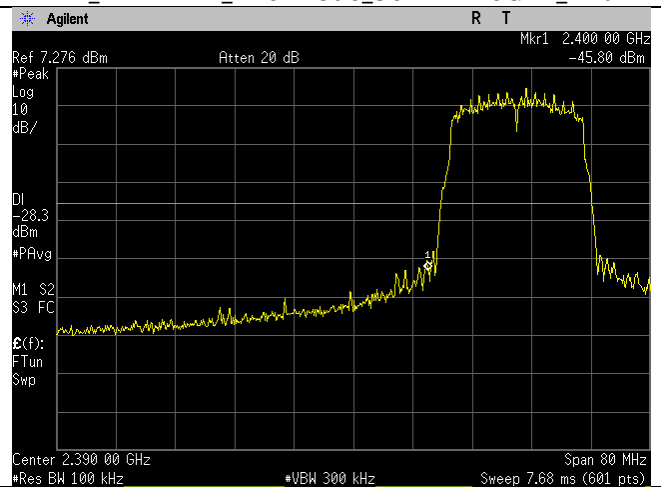
WIFI_2412MHz_n20-mode_Lower Band Edge_Ant
