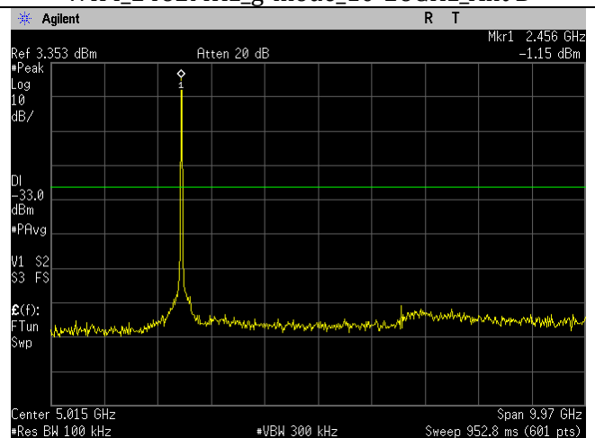
WIFI_2462MHz_g-mode_30MHz-10GHz_Ant B
