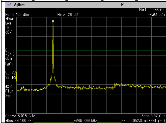
WIFI_2452MHz_n40-mode_30MHz-10GHz_Ant A
