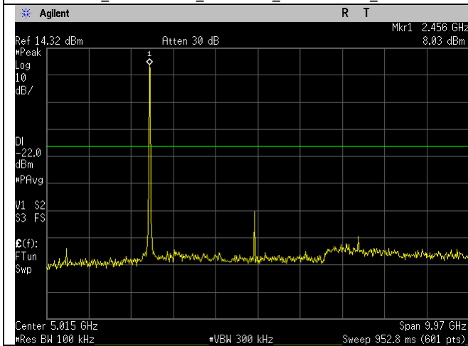
WIFI_2462MHz_b-mode_30MHz-10GHz Ant A
