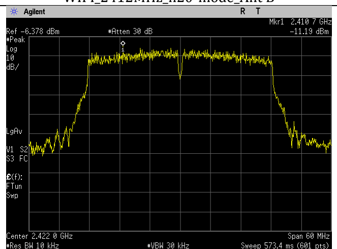
WIFI_2422MHz_n40-mode_Ant B
