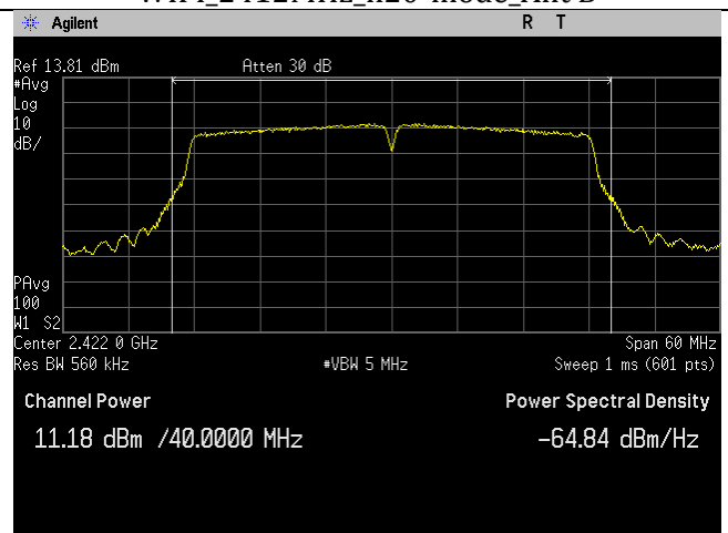
WIFI_2422MHz_n40-mode_Ant B
