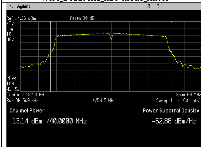
WIFI_2422MHz_n40-mode_Ant A
