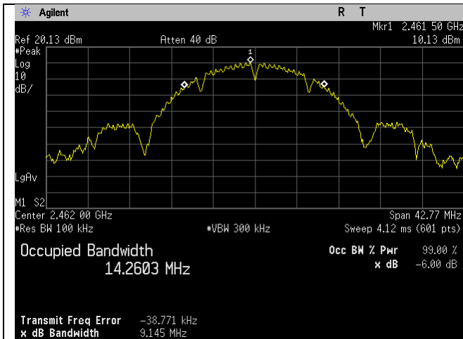
WIFI_2462MHz_b-mode_-6dB_Ant A
