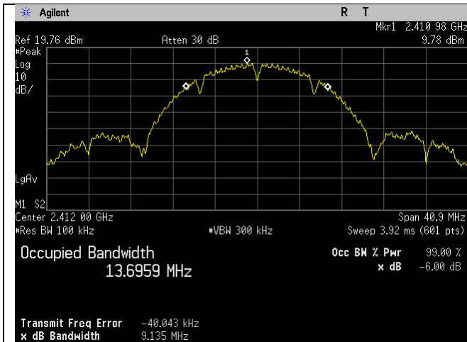
WIFI_2412MHz_b-mode_-6dB_Ant A
