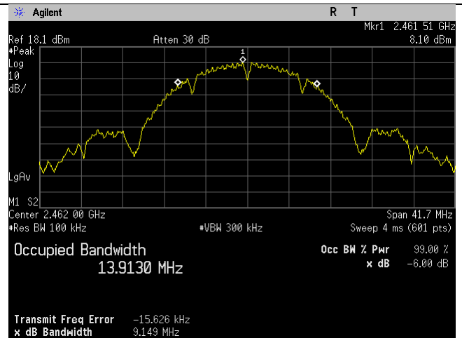
WIFI_2462MHz_b-mode_-6dB_Ant B
