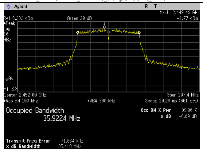
WIFI_2452MHz_n40-mode_-6dB_Ant B
