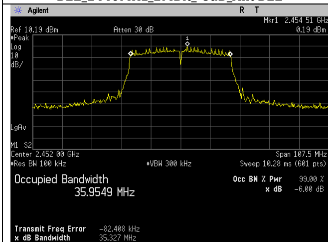
WIFI_2452MHz_n40-mode_-6dB_Ant A
