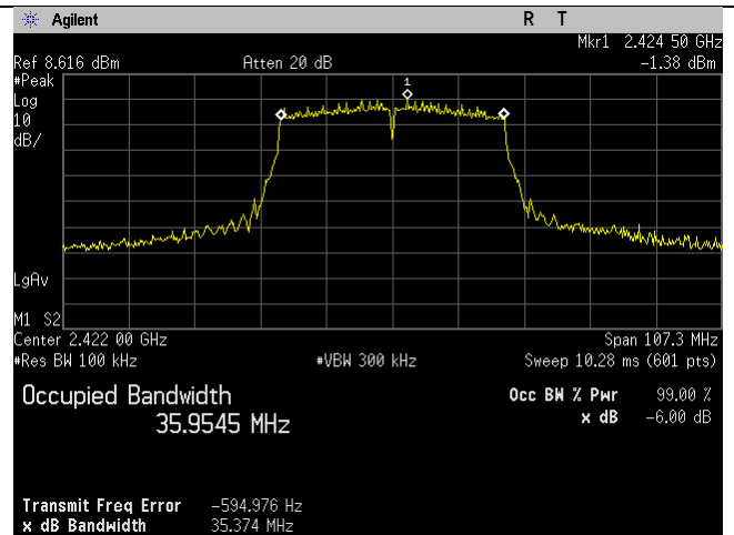
WIFI_2422MHz_n40-mode_-6dB_Ant B
