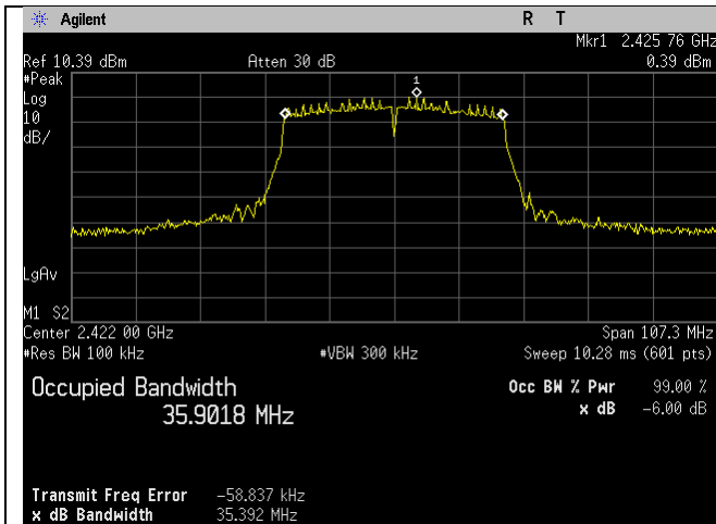
WIFI_2422MHz_n40-mode_-6dB_Ant A
