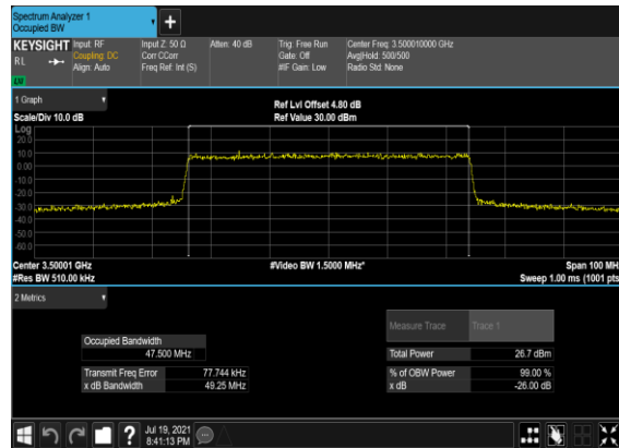
B2_N77(50M)_CP-OFDM_16 QAM_Outer_Full_Mid_CH
