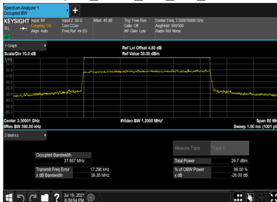
B2_N77(40M)_CP-OFDM_64 QAM_Outer_Full_Mid_CH
