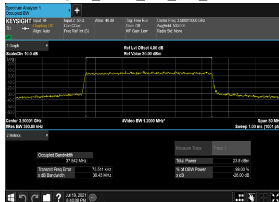
B2_N77(40M)_CP-OFDM_256 QAM_Outer_Full_Mid_CH
