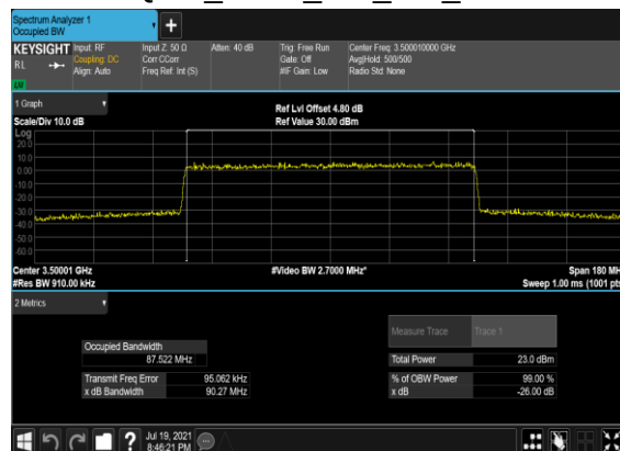
B2_N77(90M)_CP-OFDM_256 QAM_Outer_Full_Mid_CH
