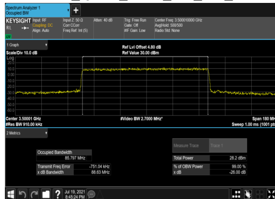
B2_N77(90M)_DFT-s- OFDM_QPSK_Outer_Full_Mid_CH
