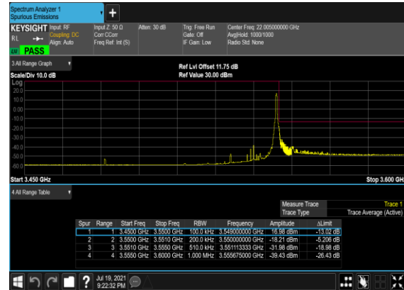
B2_N77(20M)_DFT-s- OFDM_QPSK_Edge_1RB_Right_High_CH
