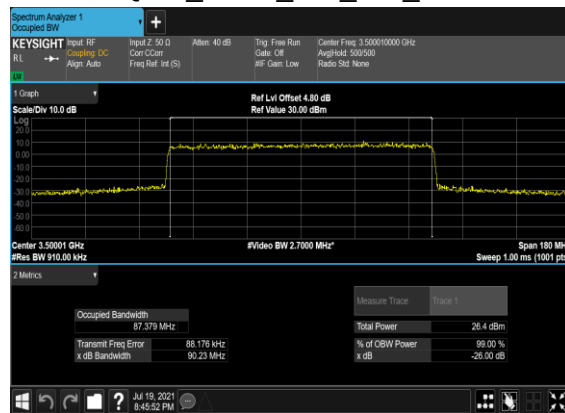
B2_N77(90M)_CP-OFDM_16 QAM_Outer_Full_Mid_CH
