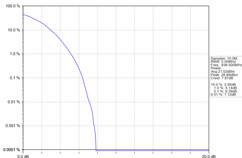
B26_5MHz_64QAM_MCH_836.5MHz_RB_25_0_NTNV
