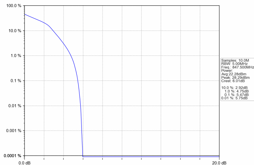
B26_3MHz_16QAM_HCH_847.5MHz_RB_15_0_NTNV
