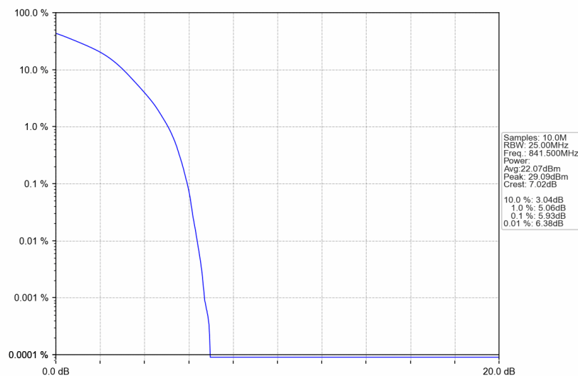
B26_15MHz_16QAM_HCH_841.5MHz_RB_75_0_NTNV
