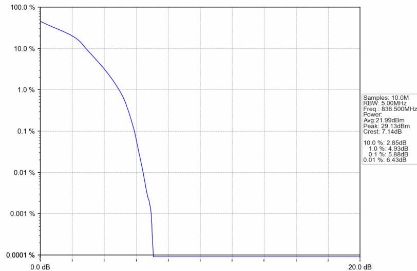
B26_5MHz_16QAM_MCH_836.5MHz_RB_25_0_NTNV
