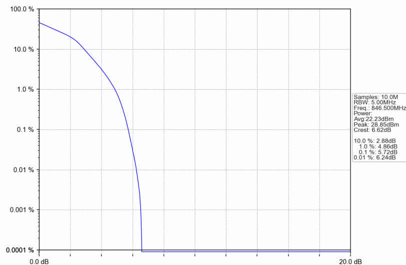
B26_5MHz_16QAM_HCH_846.5MHz_RB_25_0_NTNV
