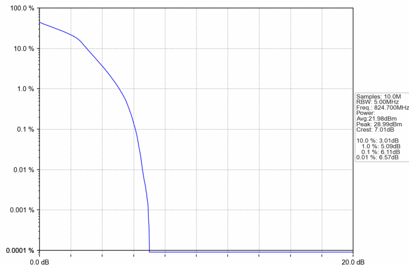
B26_1.4MHz_16QAM_LCH_824.7MHz_RB_6_0_NTNV
