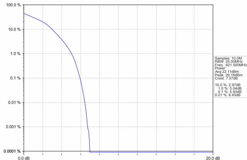
B26_15MHz_16QAM_LCH_821.5MHz_RB_75_0_NTNV
