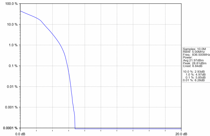
B26_3MHz_16QAM_MCH_836.5MHz_RB_15_0_NTNV
