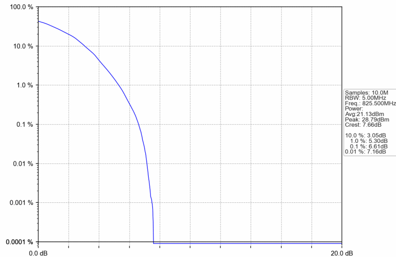
B26_3MHz_64QAM_LCH_825.5MHz_RB_15_0_NTNV
