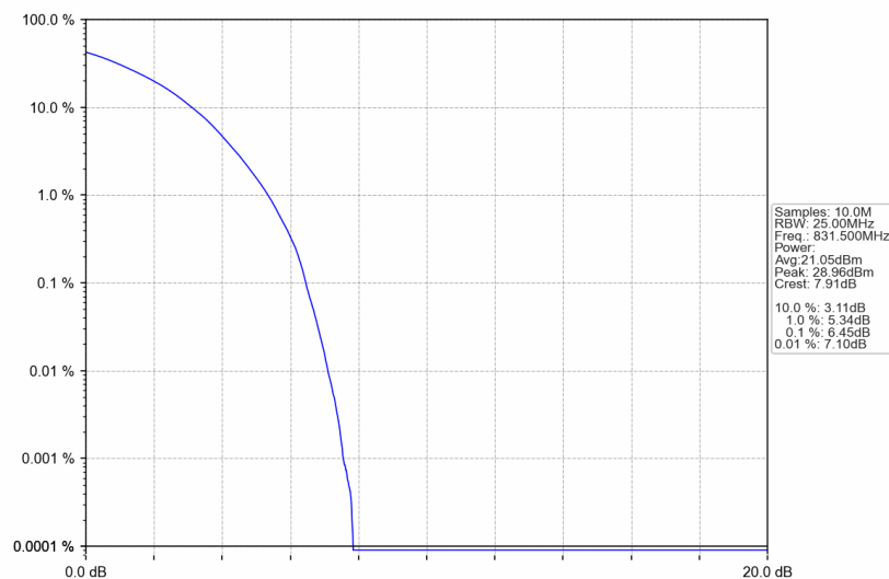
B26_15MHz_64QAM_MCH_831.5MHz_RB_75_0_NTNV
