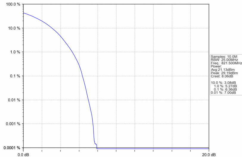
B26_15MHz_64QAM_LCH_821.5MHz_RB_75_0_NTNV
