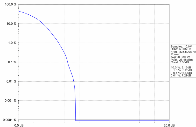
B26_1.4MHz_64QAM_MCH_836.5MHz_RB_6_0_NTNV
