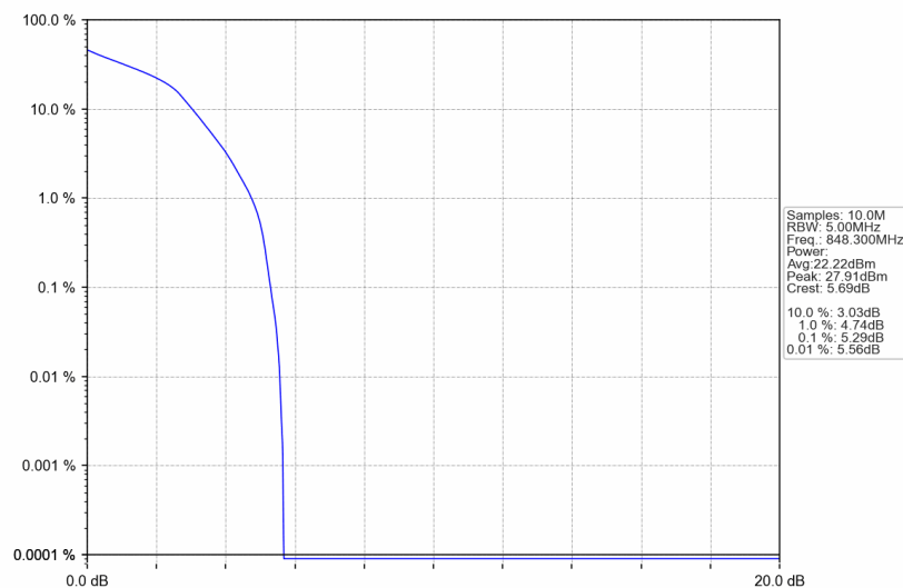
B26_1.4MHz_16QAM_HCH_848.3MHz_RB_6_0_NTNV
