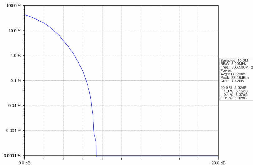
B26_3MHz_64QAM_MCH_836.5MHz_RB_15_0_NTNV
