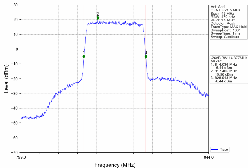
B26_15MHz_16QAM_LCH_821.5MHz_RB_75_0_NTNV
