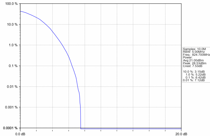
B26_1.4MHz_64QAM_LCH_824.7MHz_RB_6_0_NTNV
