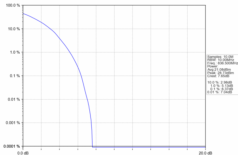
B26_10MHz_64QAM_MCH_836.5MHz_RB_50_0_NTNV
