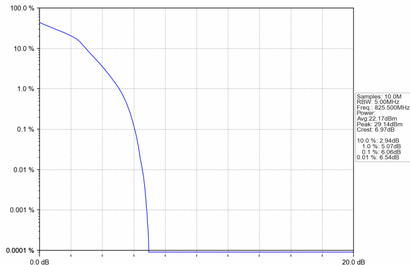
B26_3MHz_16QAM_LCH_825.5MHz_RB_15_0_NTNV
