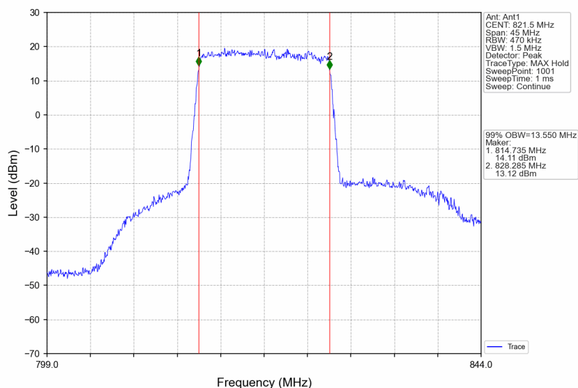
B26_15MHz_16QAM_LCH_821.5MHz_RB_75_0_NTNV
