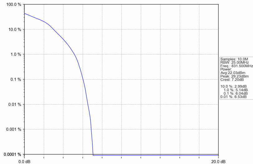
B26_15MHz_16QAM_MCH_831.5MHz_RB_75_0_NTNV
