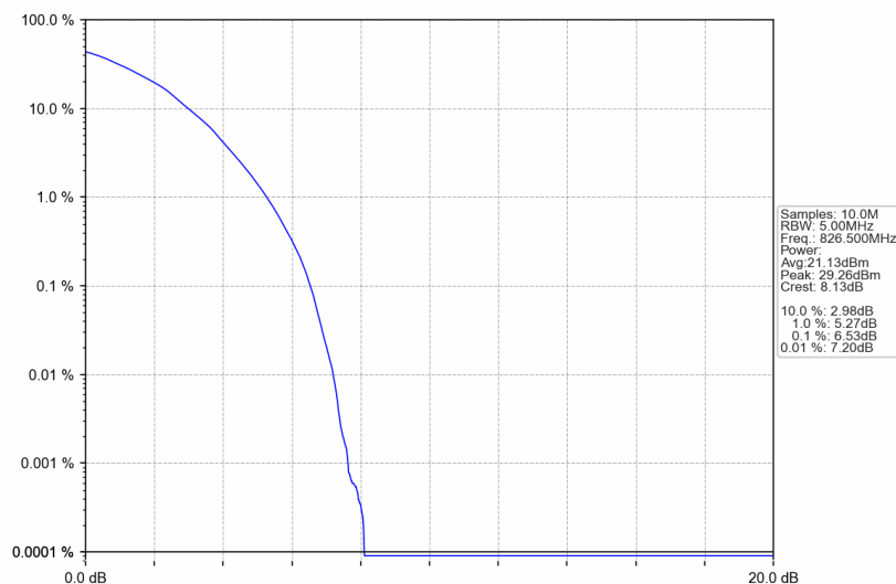
B26_5MHz_64QAM_LCH_826.5MHz_RB_25_0_NTNV
