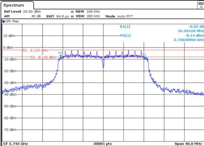
6dB Bandwidth
