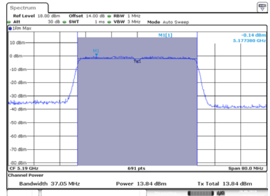
ANT 2(802.11N40)
