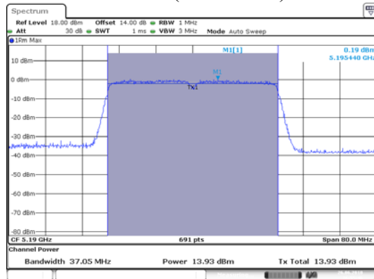
ANT 1(802.11N40)
