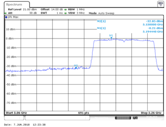
ANT 2(11AC80)
