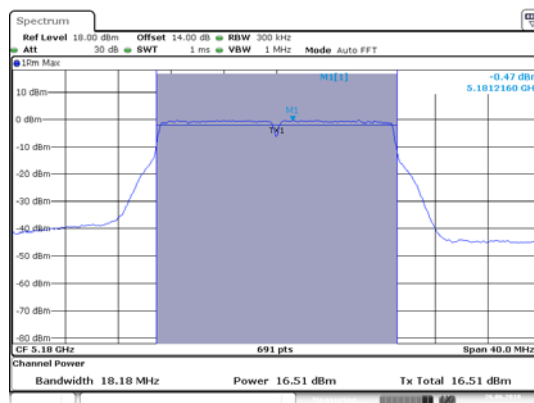
ANT 2(802.11 N20)
