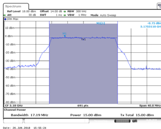
ANT 2(802.11A)
