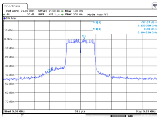
ANT 2(11N40)
