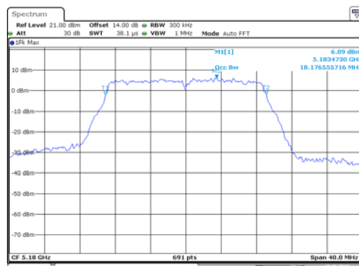
ANT 2(11N20)
