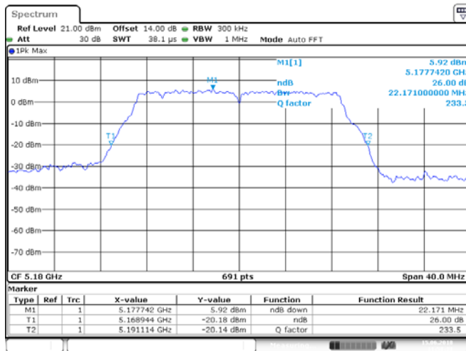
ANT 1(11N20)
