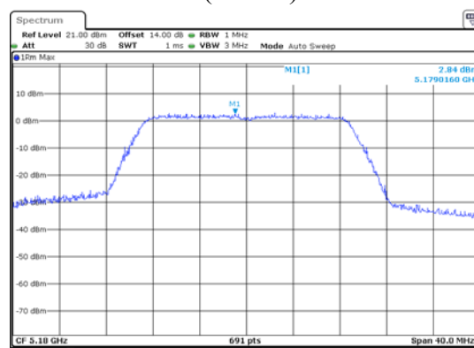
ANT 2(11N20)
