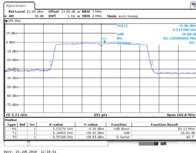
ANT 2(802.11ac80)
