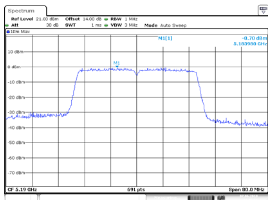
ANT 1(11AC40)
