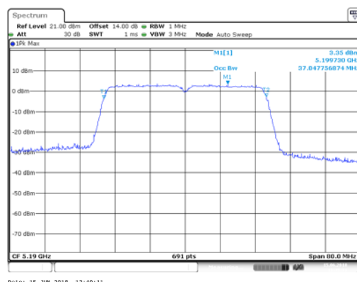
ANT 2(11N40)
