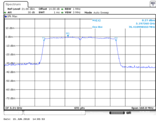
ANT 2(11AC80)
