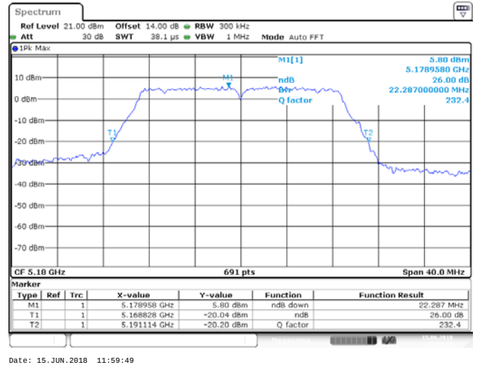
ANT 2(802.11ac20)
