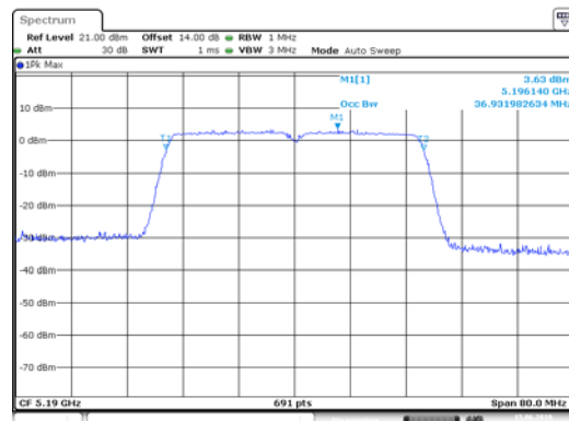
ANT 2(11AC40)
