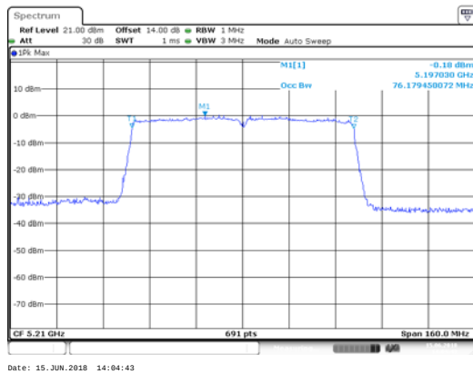
ANT 1(11AC80)
