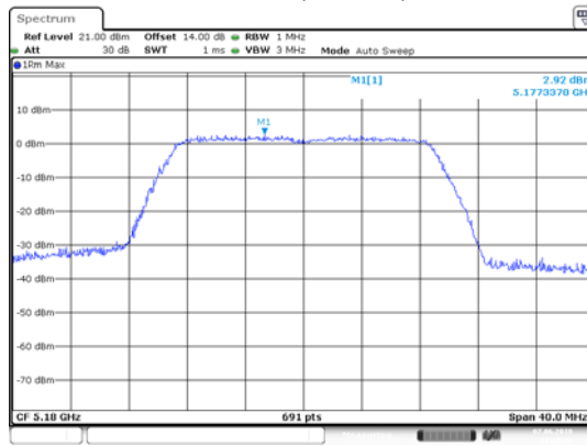
ANT 2(11N20)
