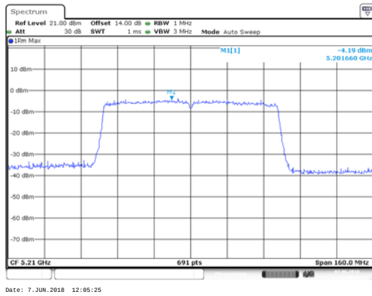
ANT 1(11AC80)
