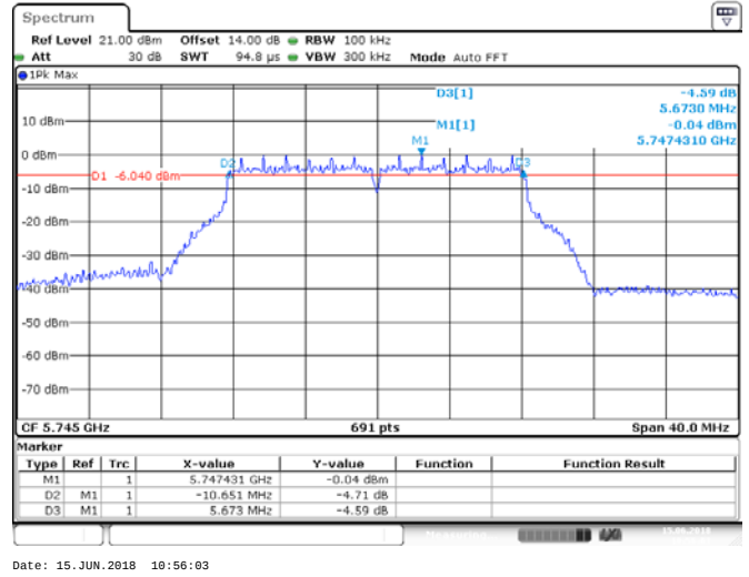
ANT 2(802.11A)
