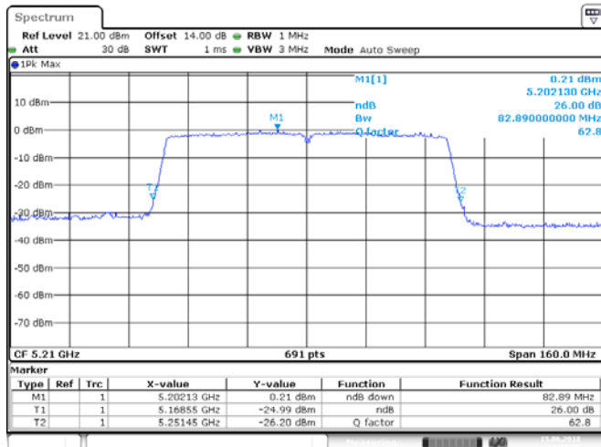
ANT 1(802.11ac80)
