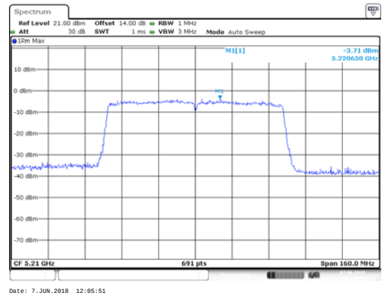
ANT 2(11AC80)
