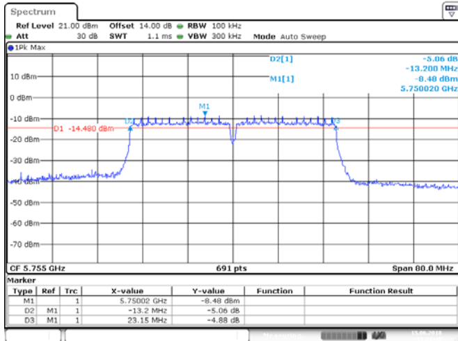
ANT 1(802.11ac40)
