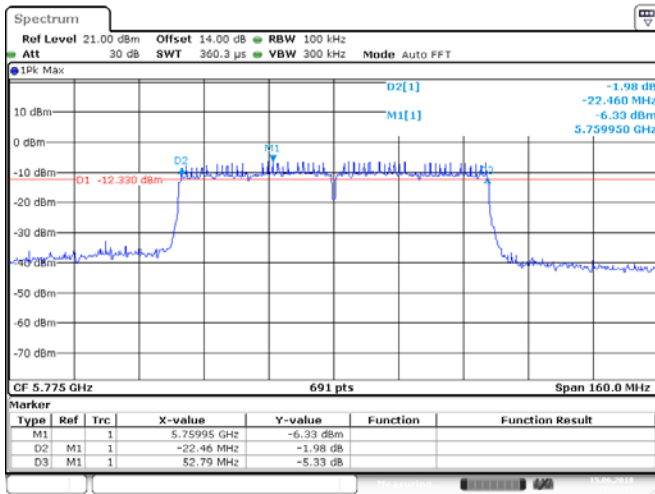
ANT 1(802.11ac80)
