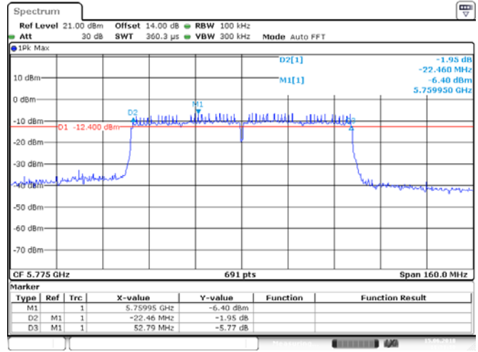
ANT 2(802.11ac80)
