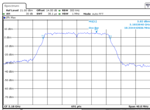
ANT 1(11N20)
