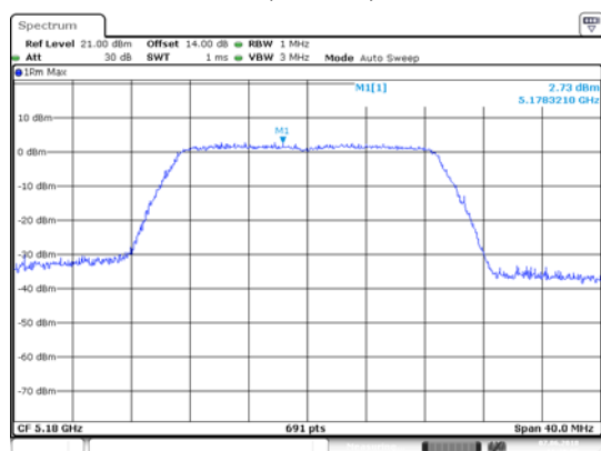
ANT 1(11N20)
