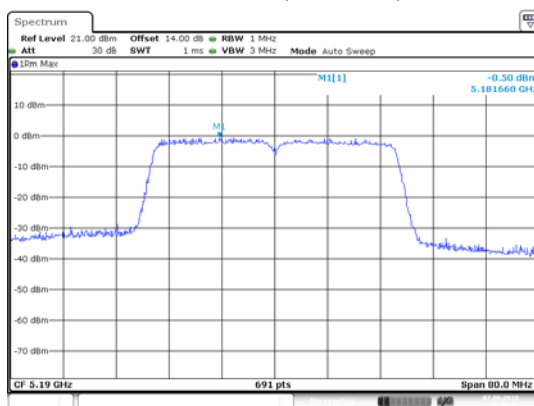
ANT 2(11AC40)
