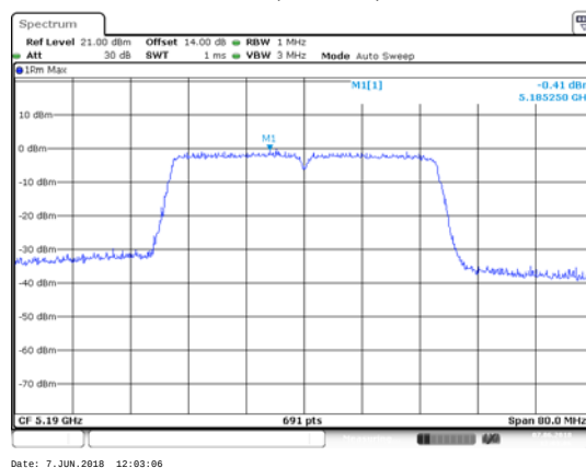
ANT 2(11N40)
