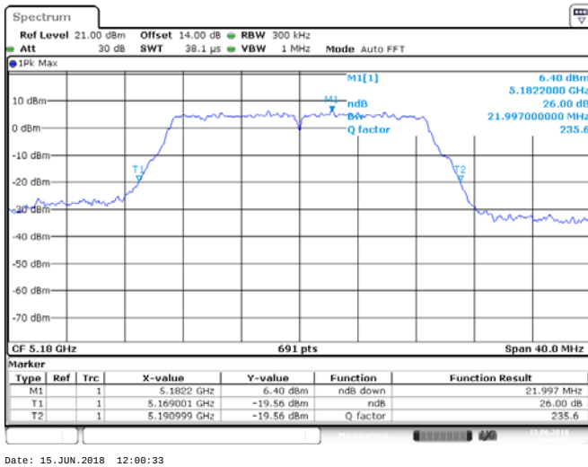
ANT 1(802.11ac20)
