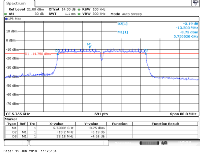
ANT 2(802.11ac40)
