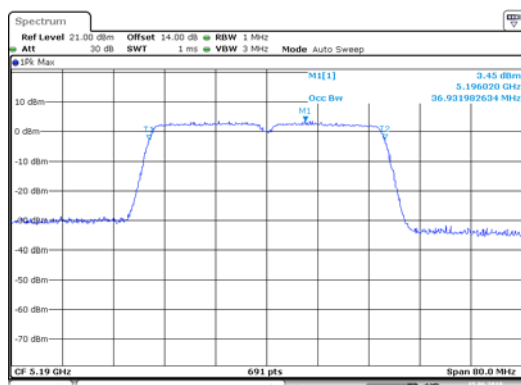
ANT 1(11AC40)
