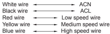
Fig. 2 Connection Wires of IT-AF-SMT
