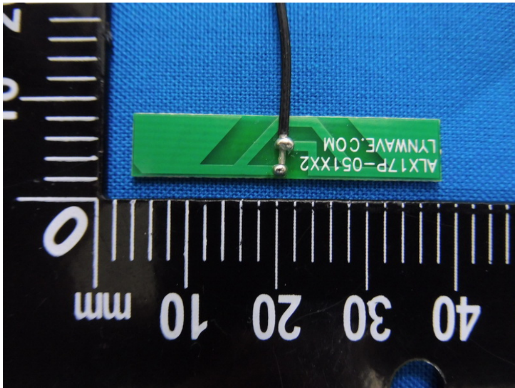
WIFI Antenna – Top View
