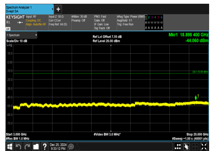
Band66-20MHz-16QAM-132072-100RB#0-3000~20000-P
