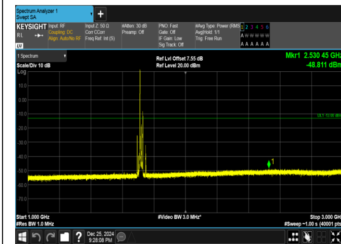
Band66-20MHz-16QAM-132072-1RB#0-1000~3000-PASS
