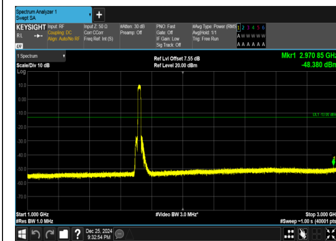
Band66-20MHz-16QAM-132072-100RB#0-1000~3000-PA
