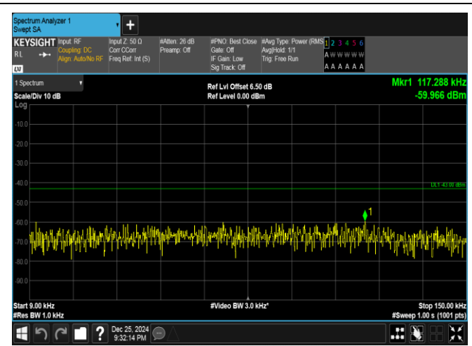
Band66-20MHz-16QAM-132072-100RB#0-0.009~0.15-PA
