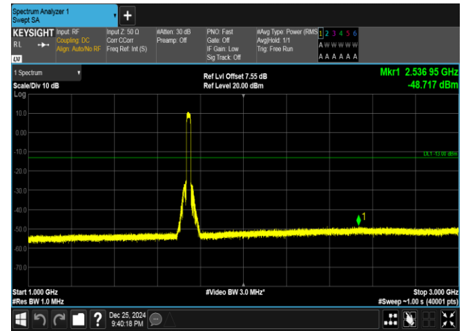
Band66-20MHz-16QAM-132322-100RB#0-1000~3000-PA SS
