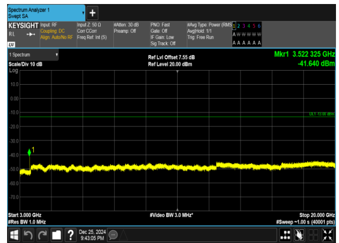
Band66-20MHz-16QAM-132572-1RB#0-3000~20000-PASS
