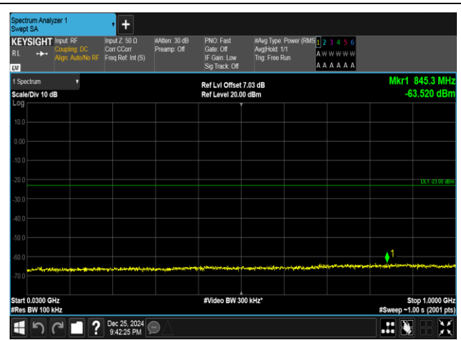
Band66-20MHz-16QAM-132572-1RB#0-30~1000-PASS
