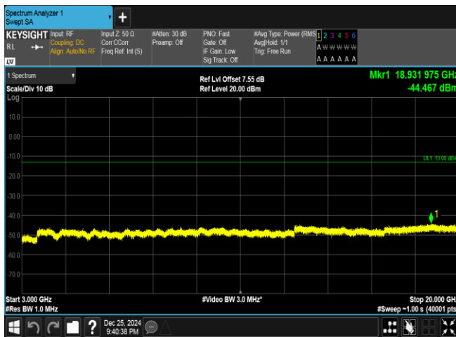
Band66-20MHz-16QAM-132322-100RB#0-3000~20000-P ASS
