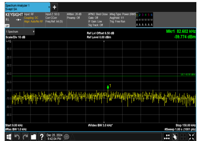
Band66-20MHz-16QAM-132572-1RB#0-0.009~0.15-PASS
