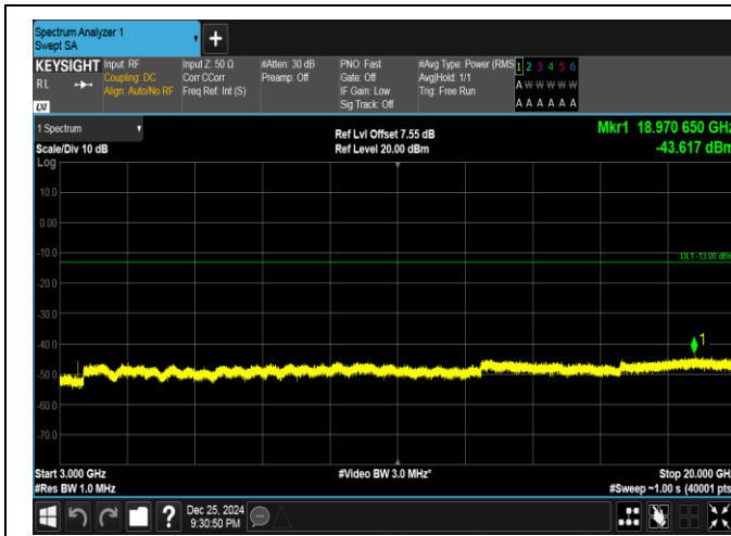
Band66-20MHz-16QAM-132072-1RB#99-3000~20000-PA
