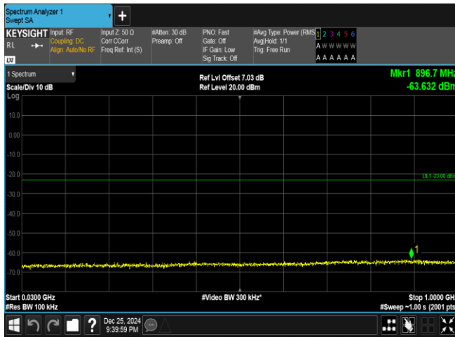
Band66-20MHz-16QAM-132322-100RB#0-30~1000-PASS SS
