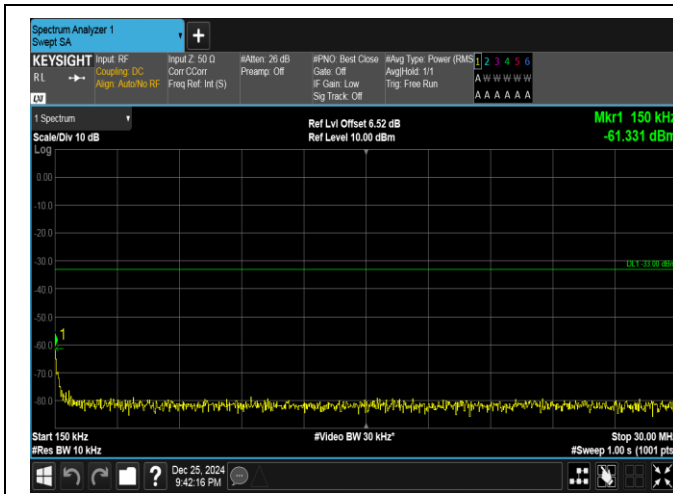
Band66-20MHz-16QAM-132572-1RB#0-0.15~30-PASS
