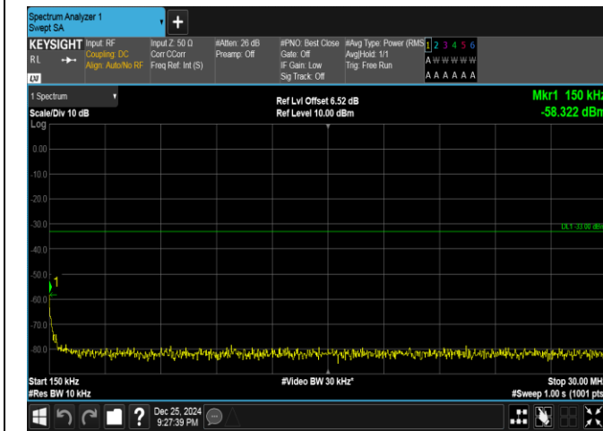
Band66-20MHz-16QAM-132072-1RB#0-0.15~30-PASS
