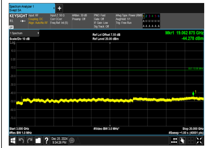
Band66-20MHz-QPSK-132322-1RB#0-3000~20000-PASS
