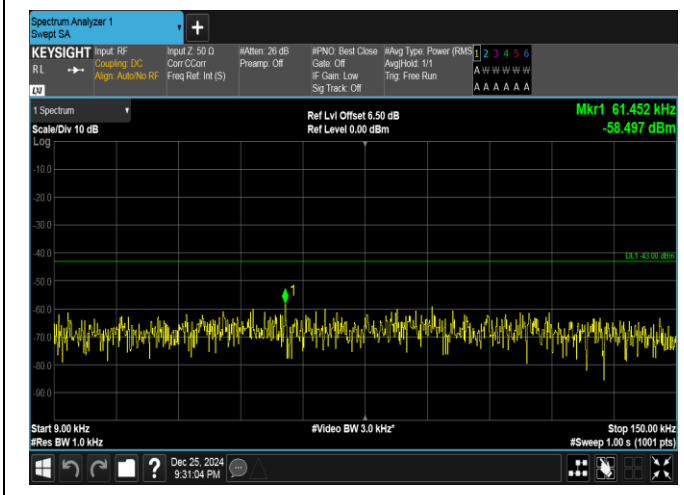
Band66-20MHz-QPSK-132072-100RB#0-0.009~0.15-PASS
