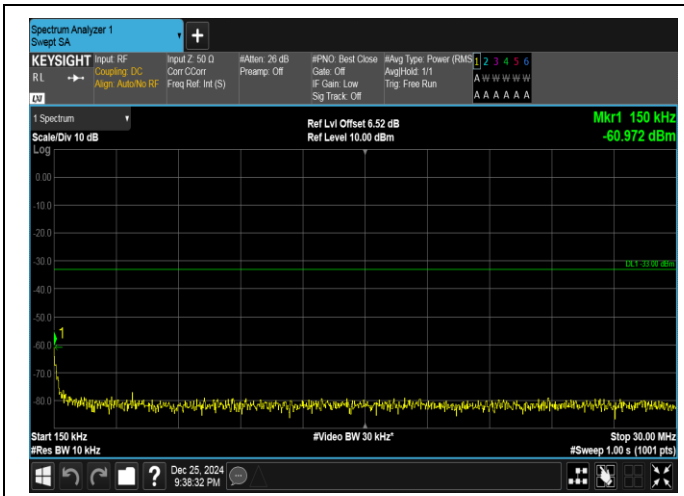
Band66-20MHz-QPSK-132322-100RB#0-0.15~30-PASS
