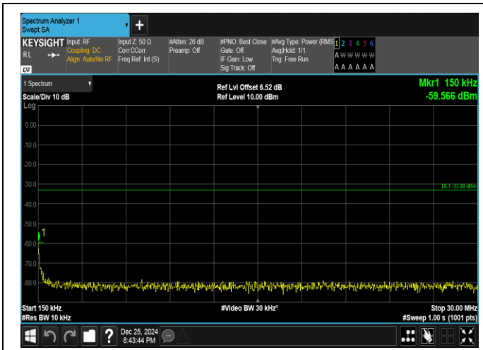
Band66-15MHz-16QAM-132322-1RB#74-0.15~30-PASS
