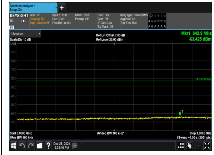
Band66-20MHz-QPSK-132322-1RB#0-30~1000-PASS
