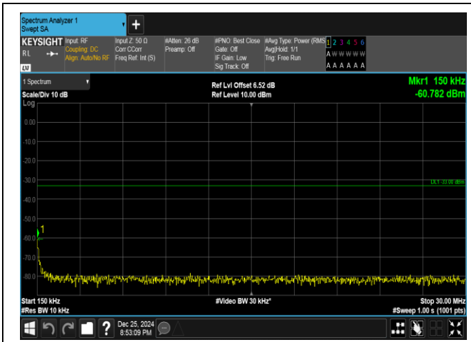
Band66-15MHz-16QAM-132597-75RB#0-0.15~30-PASS
