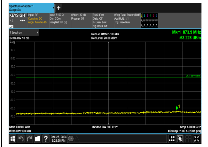
Band66-20MHz-QPSK-132072-1RB#99-30~1000-PASS
