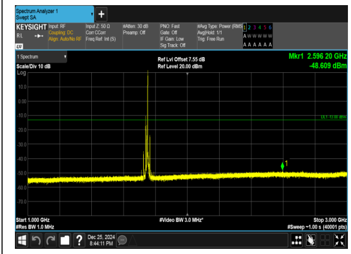
Band66-15MHz-16QAM-132322-1RB#74-1000~3000-PAS
