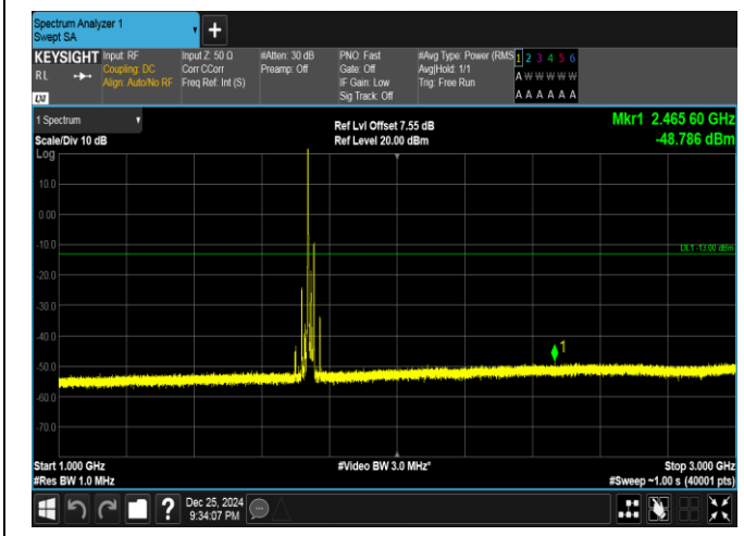
Band66-20MHz-QPSK-132322-1RB#0-1000~3000-PASS
