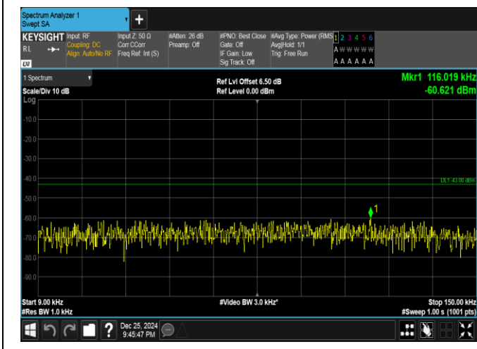
Band66-20MHz-QPSK-132572-100RB#0-0.009~0.15-PASS
