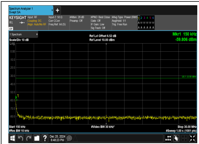
Band66-15MHz-16QAM-132597-1RB#0-0.15~30-PASS
