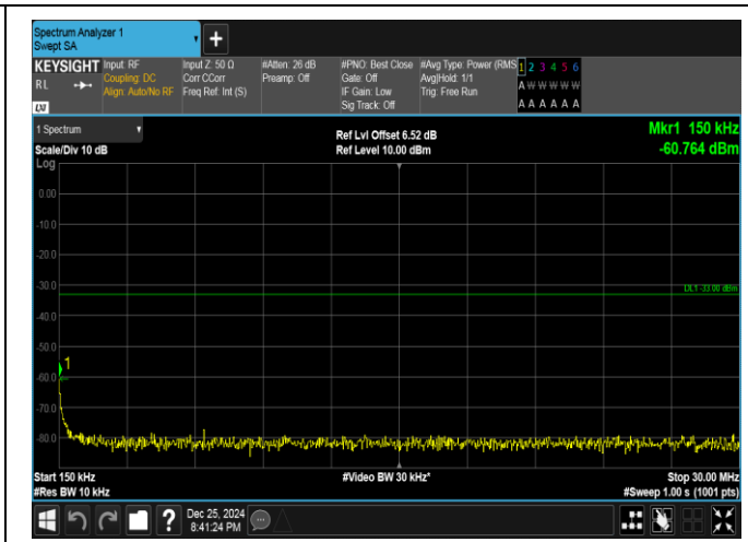
Band66-15MHz-16QAM-132322-1RB#0-0.15~30-PASS
