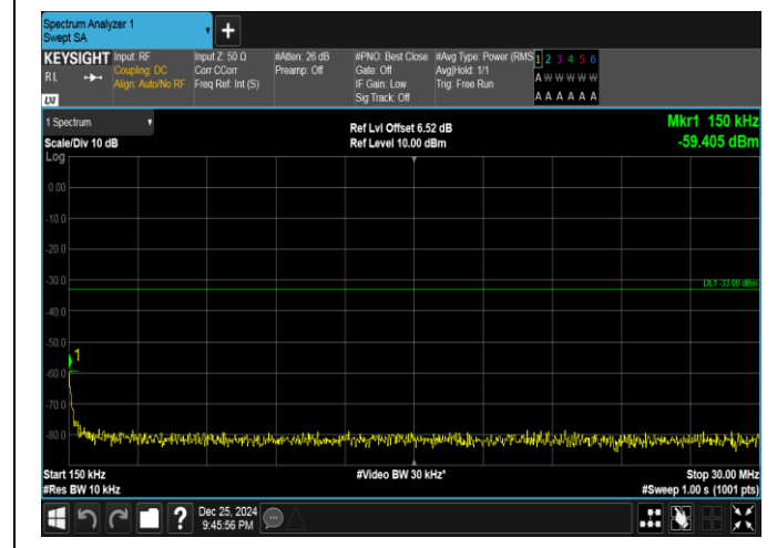
Band66-20MHz-QPSK-132572-100RB#0-0.15~30-PASS
