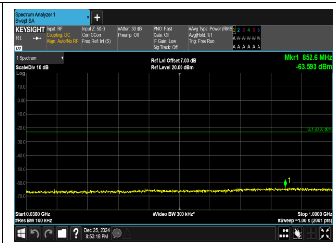
Band66-15MHz-16QAM-132597-75RB#0-30~1000-PASS
