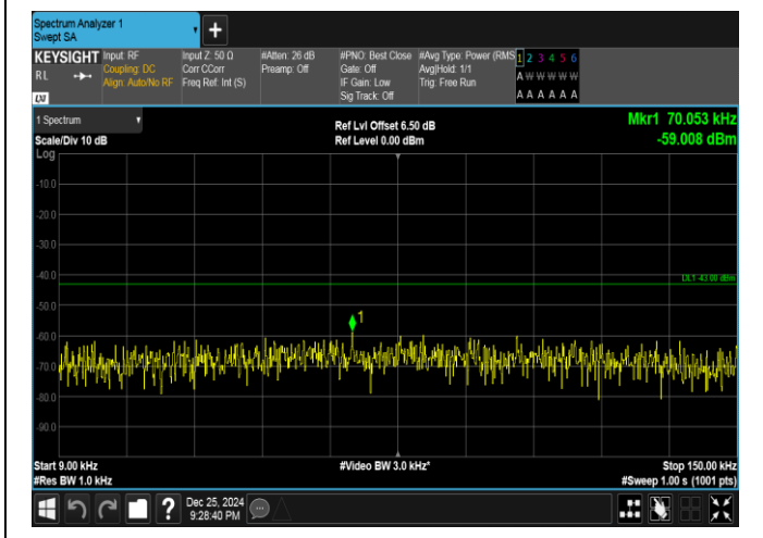
Band66-20MHz-QPSK-132072-1RB#99-0.009~0.15-PASS
