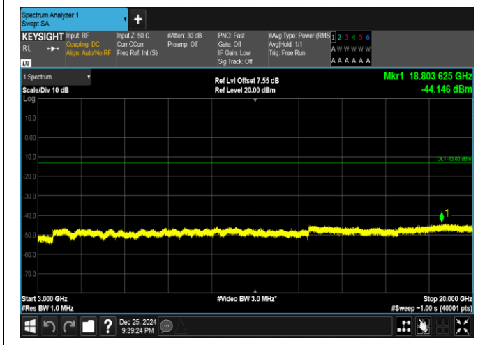
Band66-20MHz-QPSK-132322-100RB#0-3000~20000-PASS
