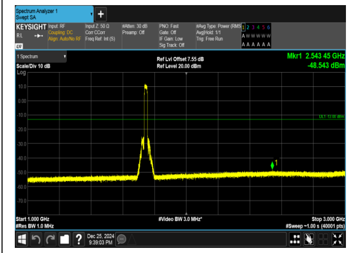
Band66-20MHz-QPSK-132322-100RB#0-1000~3000-PASS
