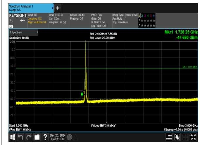
Band66-15MHz-16QAM-132597-1RB#0-1000~3000-PASS
