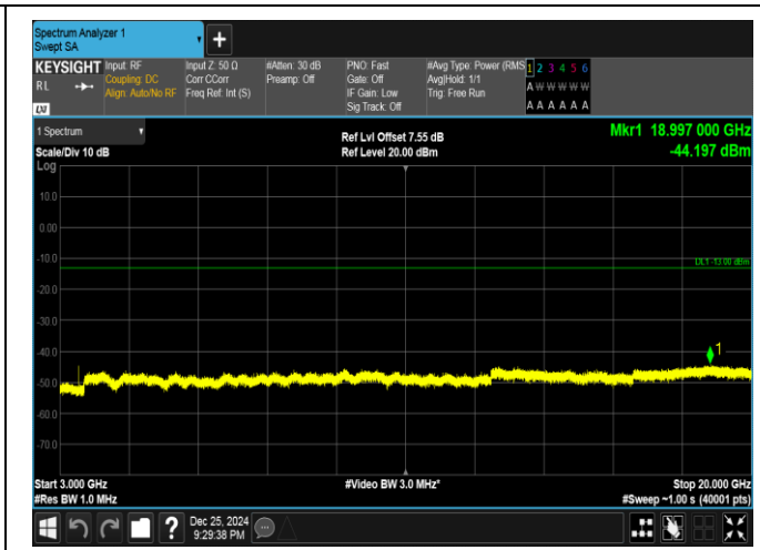
Band66-20MHz-QPSK-132072-1RB#99-3000~20000-PASS
