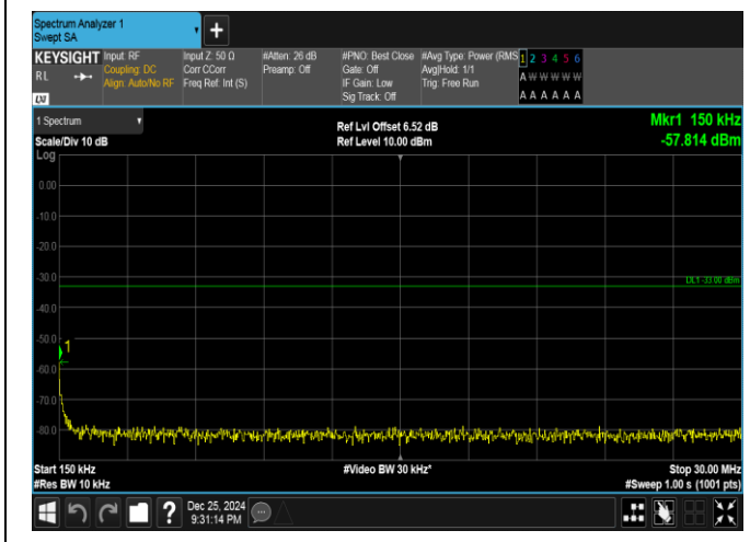
Band66-20MHz-QPSK-132072-100RB#0-0.15~30-PASS
