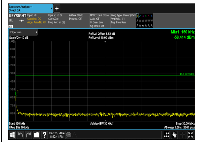
Band66-15MHz-16QAM-132597-1RB#74-0.15~30-PASS
