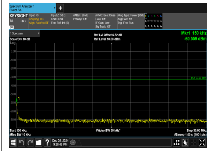
Band66-20MHz-QPSK-132072-1RB#99-0.15~30-PASS
