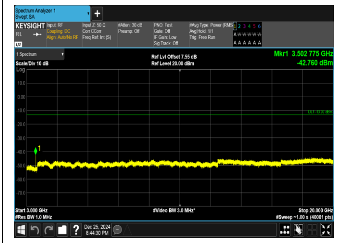
Band66-15MHz-16QAM-132322-1RB#74-3000~20000-PA
