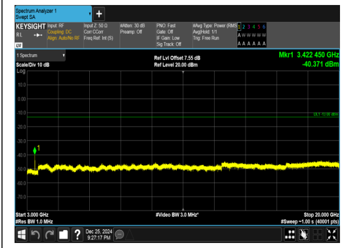
Band66-20MHz-QPSK-132072-1RB#0-3000~20000-PASS
