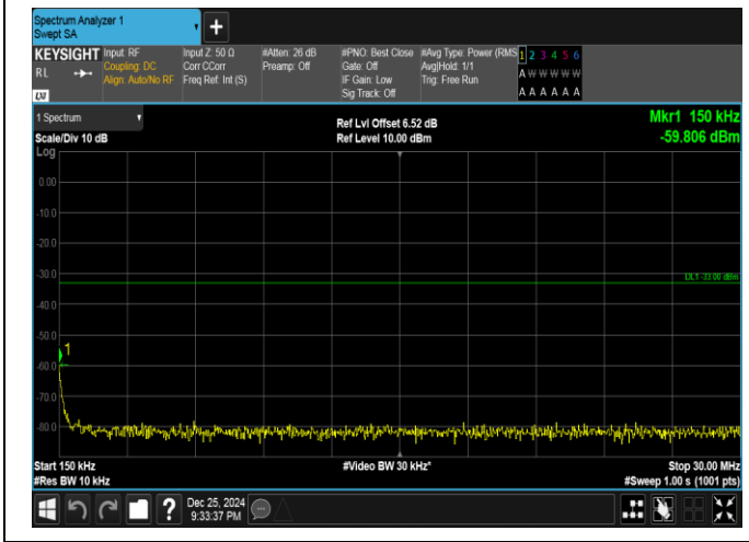
Band66-20MHz-QPSK-132322-1RB#0-0.15~30-PASS
