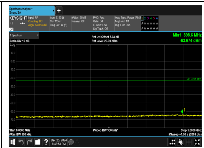
Band66-15MHz-16QAM-132322-1RB#74-30~1000-PASS
