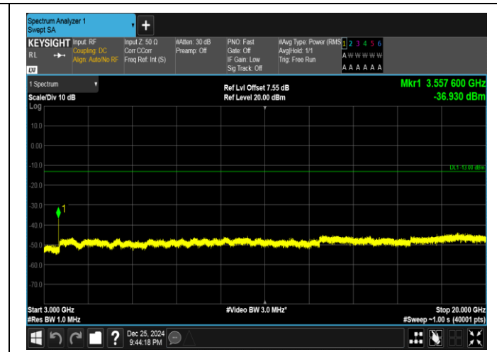
Band66-20MHz-QPSK-132572-1RB#99-3000~20000-PASS
