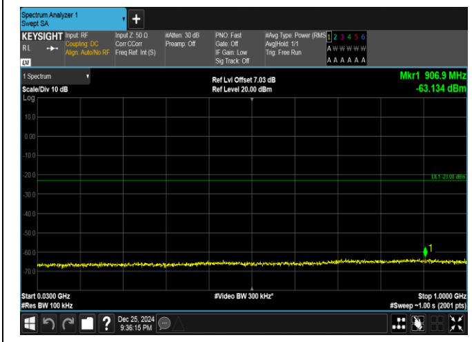
Band66-20MHz-QPSK-132322-1RB#99-30~1000-PASS
