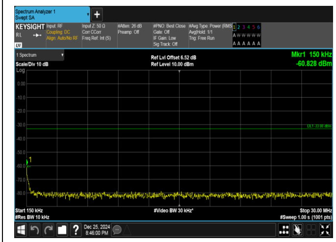
Band66-15MHz-16QAM-132322-75RB#0-0.15~30-PASS
