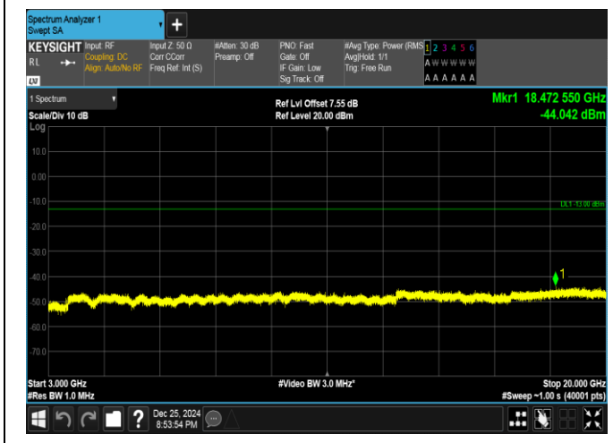
Band66-15MHz-16QAM-132597-75RB#0-3000~20000-PASS
