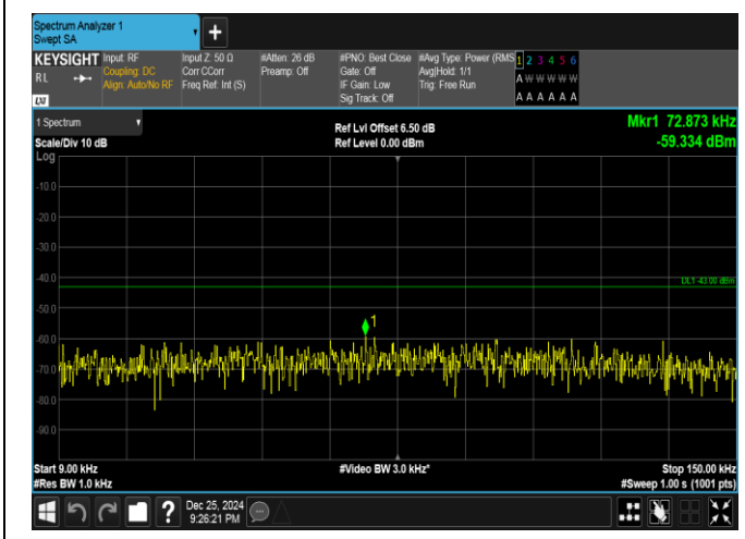
Band66-20MHz-QPSK-132072-1RB#0-0.009~0.15-PASS
