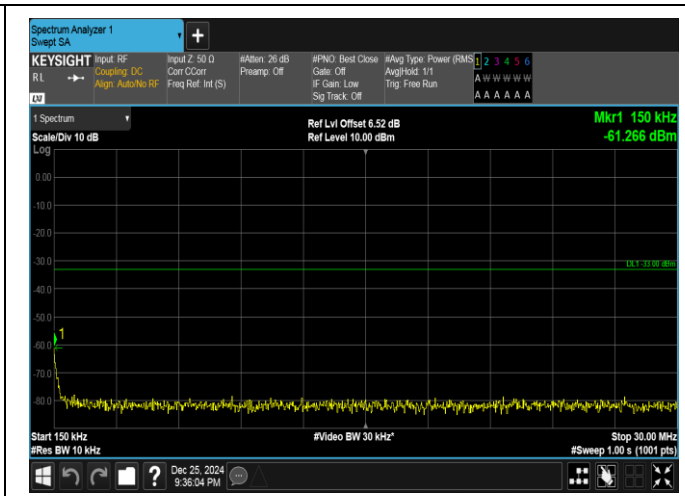
Band66-20MHz-QPSK-132322-1RB#99-0.15~30-PASS
