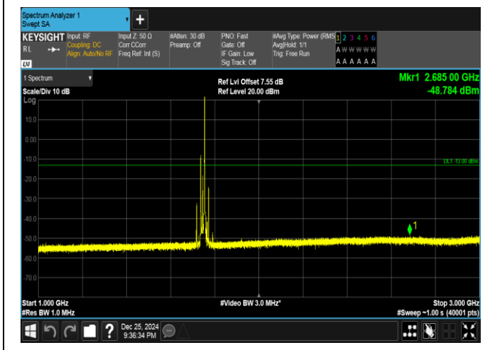
Band66-20MHz-QPSK-132322-1RB#99-1000~3000-PASS
