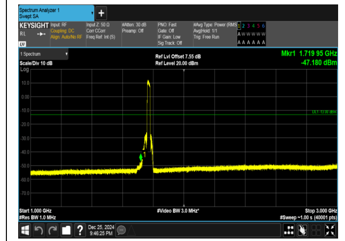
Band66-20MHz-QPSK-132572-100RB#0-1000~3000-PASS
