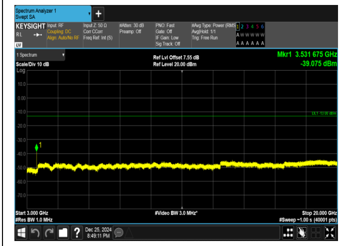
Band66-15MHz-16QAM-132597-1RB#0-3000~20000-PASS
