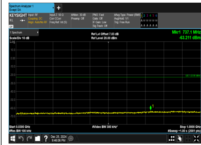
Band66-20MHz-QPSK-132572-100RB#0-30~1000-PASS
