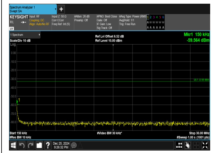
Band66-20MHz-QPSK-132072-1RB#0-0.15~30-PASS
