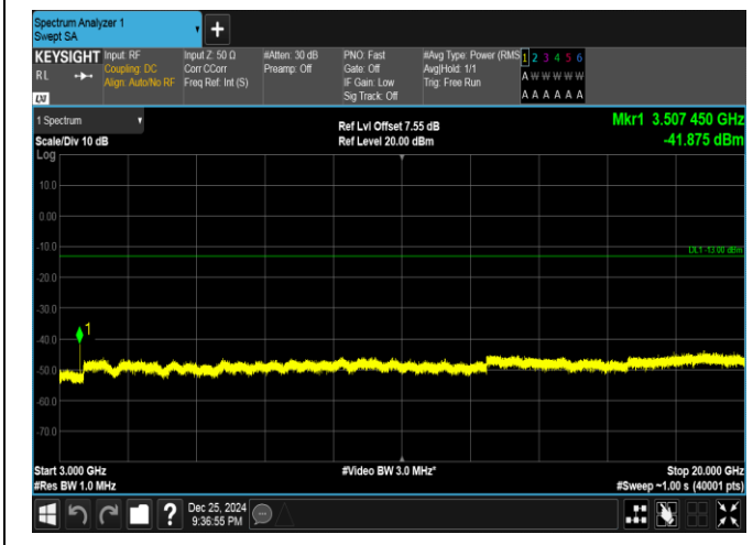
Band66-20MHz-QPSK-132322-1RB#99-3000~20000-PASS
