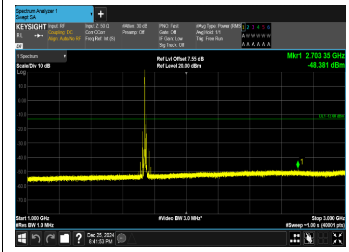
Band66-15MHz-16QAM-132322-1RB#0-1000~3000-PASS
