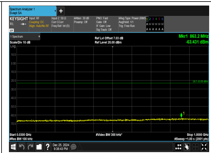
Band66-20MHz-QPSK-132322-100RB#0-30~1000-PASS
