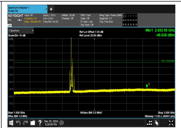
Band66-20MHz-QPSK-132072-1RB#0-1000~3000-PASS
