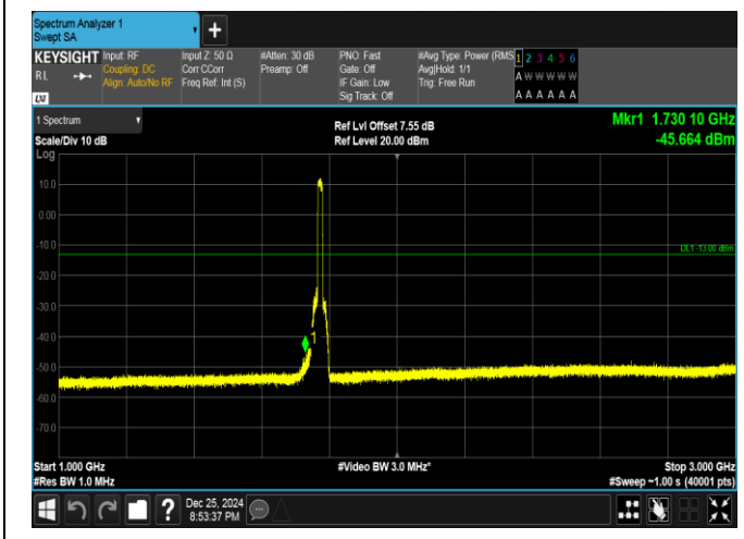
Band66-15MHz-16QAM-132597-75RB#0-1000~3000-PASS
