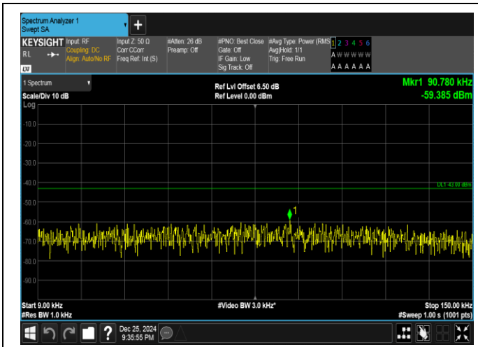
Band66-20MHz-QPSK-132322-1RB#99-0.009~0.15-PASS
