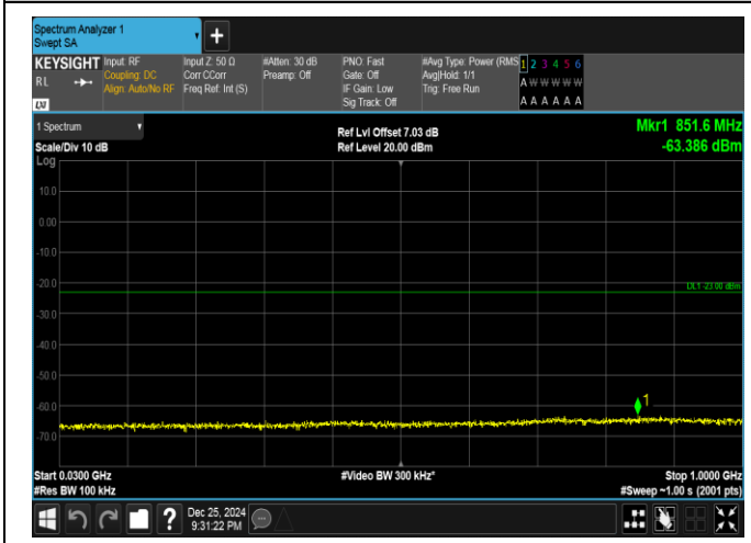
Band66-20MHz-QPSK-132072-100RB#0-30~1000-PASS
