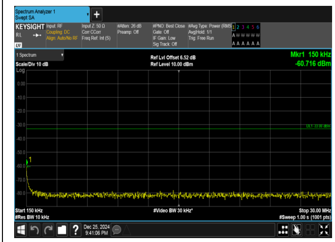
Band66-20MHz-QPSK-132572-1RB#0-0.15~30-PASS
