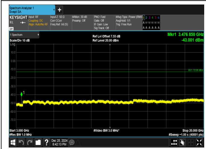
Band66-15MHz-16QAM-132322-1RB#0-3000~20000-PAS
