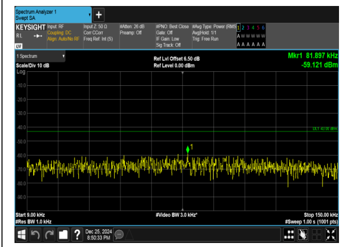
Band66-15MHz-16QAM-132597-1RB#74-0.009~0.15-PASS
