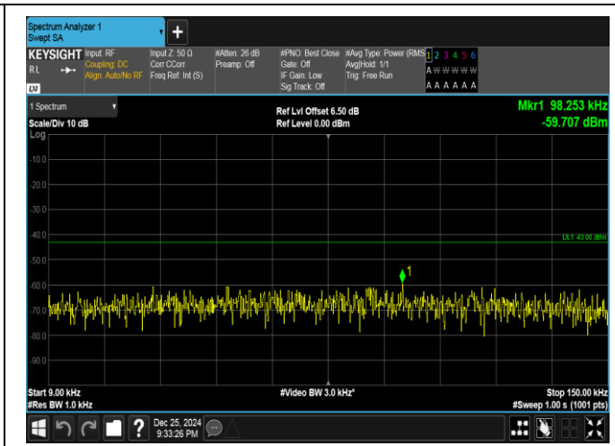
Band66-20MHz-QPSK-132322-1RB#0-0.009~0.15-PASS
