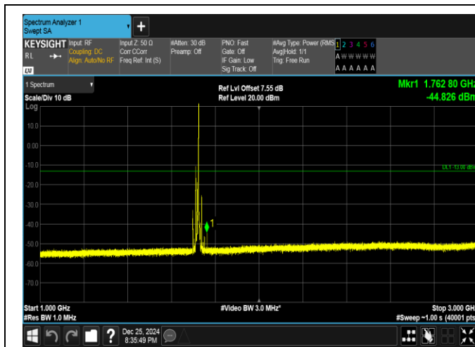
Band66-15MHz-QPSK-132047-1RB#74-1000~3000-PASS
