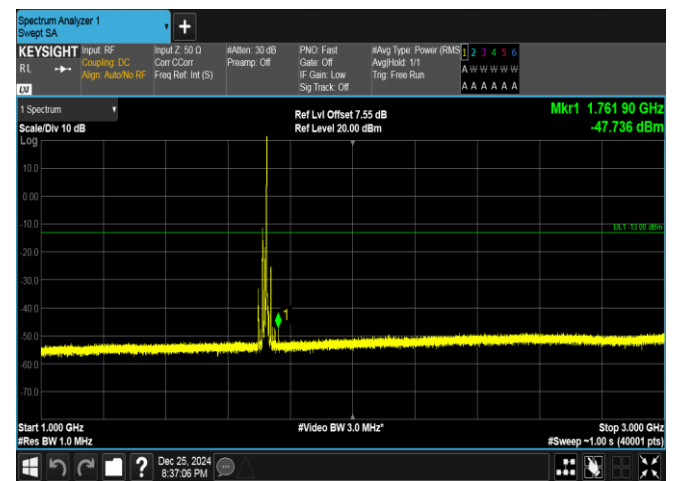
Band66-15MHz-16QAM-132047-1RB#74-1000~3000-PAS S
