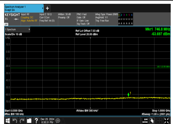
Band66-15MHz-QPSK-132047-1RB#74-30~1000-PASS
