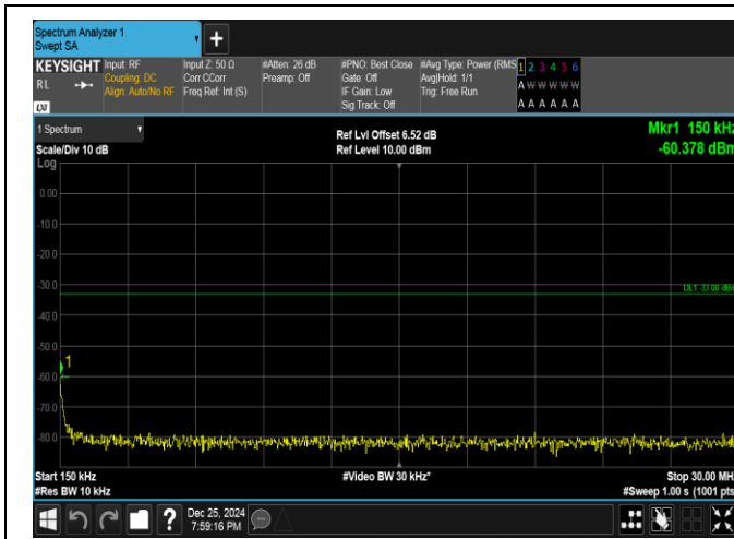
Band66-10MHz-16QAM-132622-50RB#0-0.15~30-PASS
