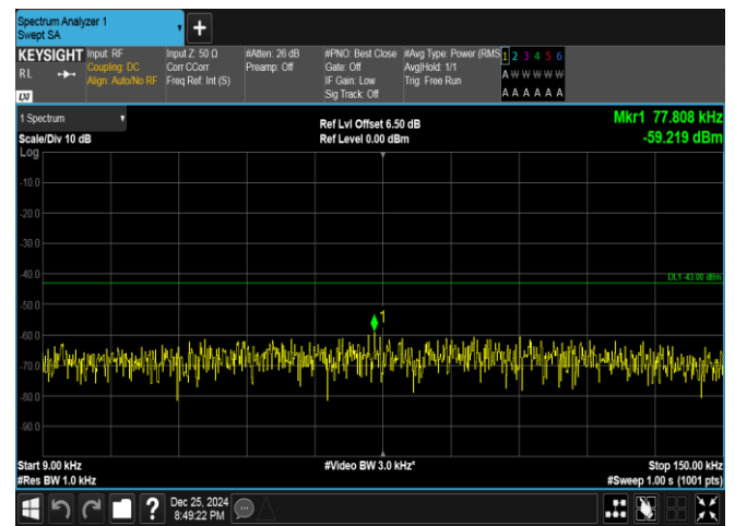
Band66-15MHz-QPSK-132597-1RB#74-0.009~0.15-PASS
