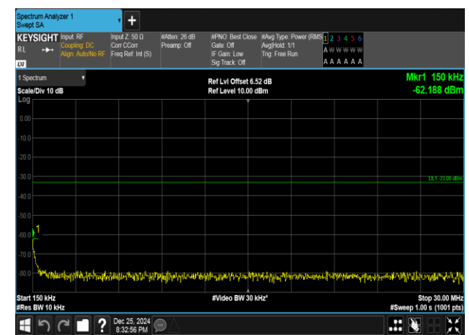
Band66-15MHz-QPSK-132047-1RB#0-0.15~30-PASS
