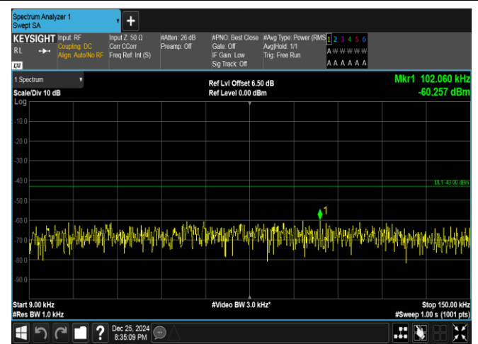
Band66-15MHz-QPSK-132047-1RB#74-0.009~0.15-PASS
