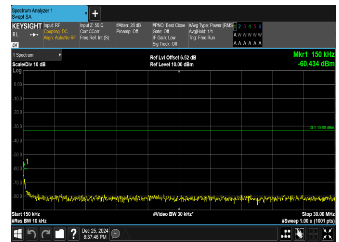
Band66-15MHz-QPSK-132047-75RB#0-0.15~30-PASS
