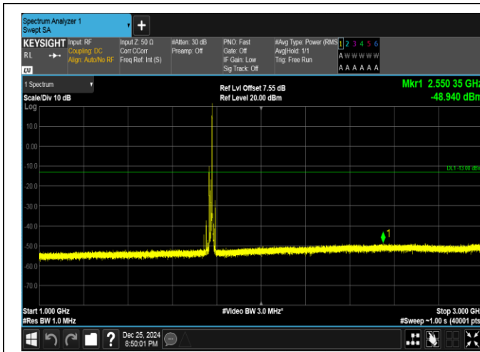
Band66-15MHz-QPSK-132597-1RB#74-1000~3000-PASS
