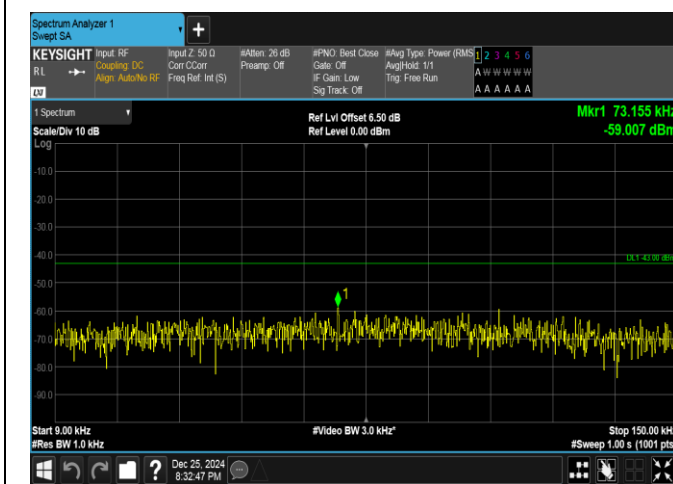
Band66-15MHz-QPSK-132047-1RB#0-0.009~0.15-PASS
