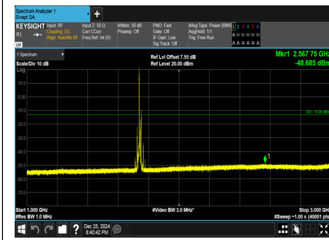
Band66-15MHz-QPSK-132322-1RB#0-1000~3000-PASS
