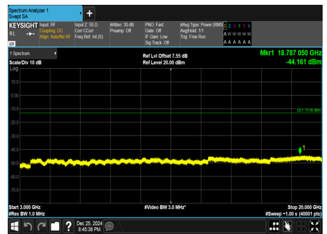
Band66-15MHz-QPSK-132322-75RB#0-3000~20000-PASS
