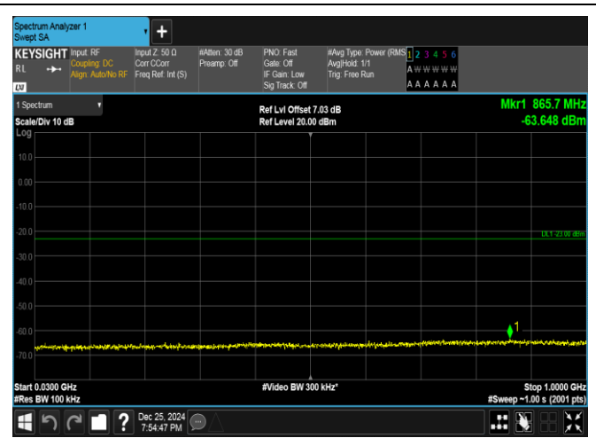
Band66-10MHz-16QAM-132622-1RB#0-30~1000-PASS
