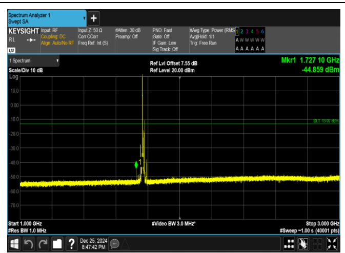
Band66-15MHz-QPSK-132597-1RB#0-1000~3000-PASS
