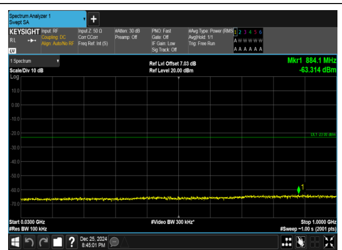
Band66-15MHz-QPSK-132322-75RB#0-30~1000-PASS
