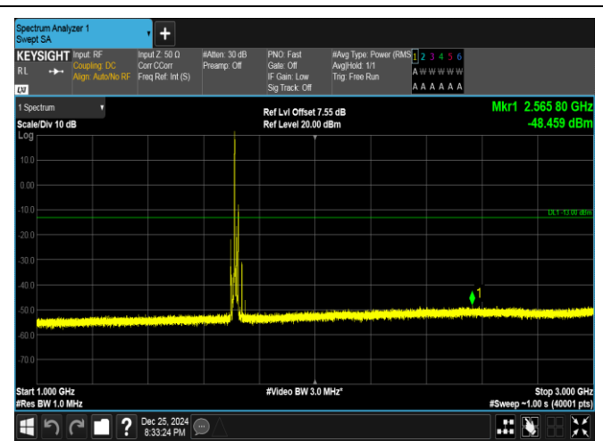
Band66-15MHz-QPSK-132047-1RB#0-1000~3000-PASS
