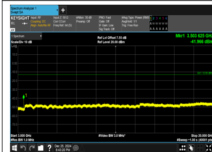
Band66-15MHz-QPSK-132322-1RB#74-3000~20000-PASS
