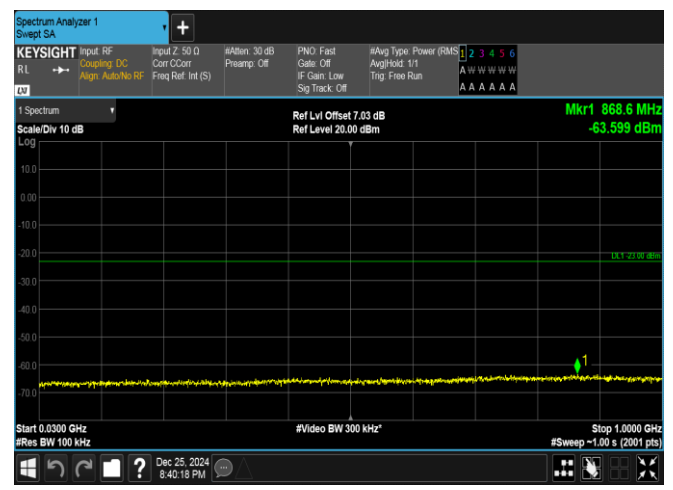
Band66-15MHz-QPSK-132322-1RB#0-30~1000-PASS
