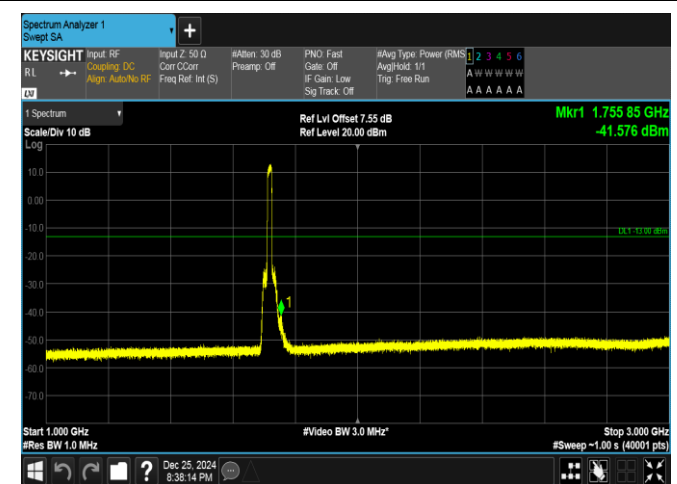
Band66-15MHz-QPSK-132047-75RB#0-1000~3000-PASS
