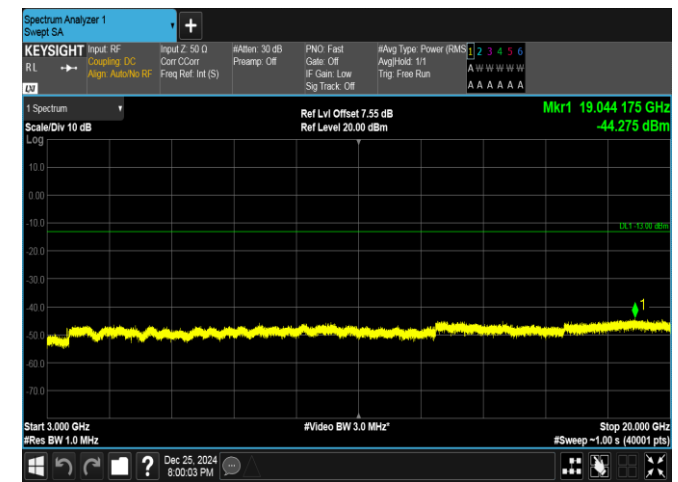
Band66-10MHz-16QAM-132622-50RB#0-3000~20000-PA
