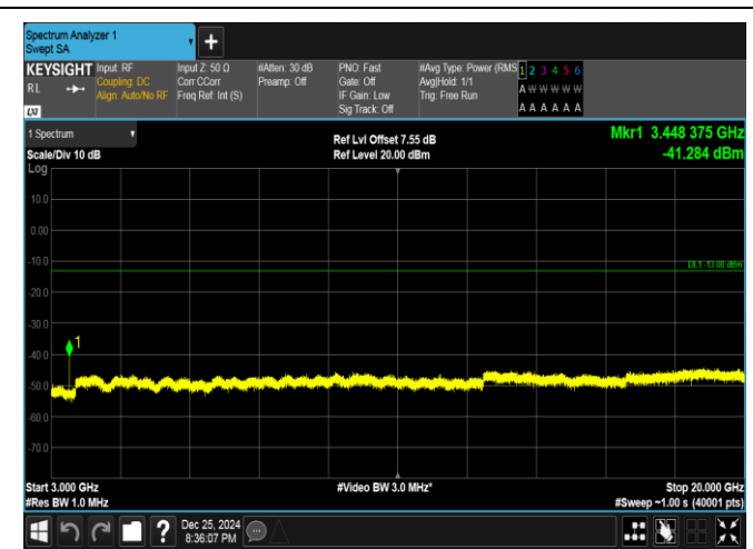
Band66-15MHz-QPSK-132047-1RB#74-3000~20000-PASS
