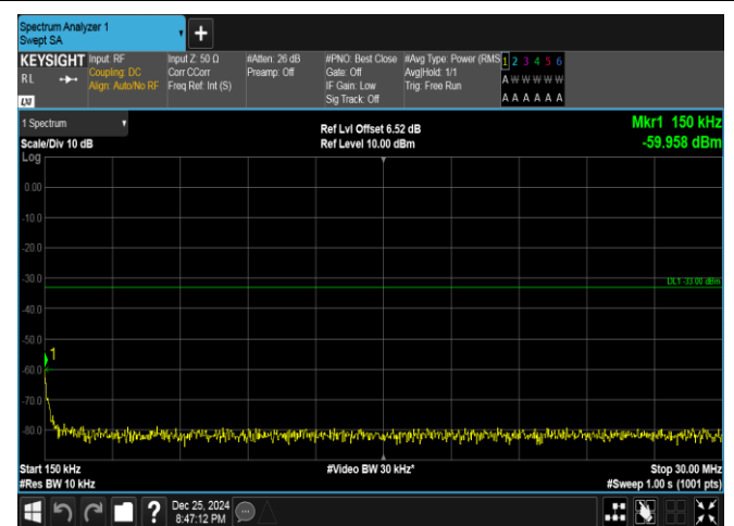
Band66-15MHz-QPSK-132597-1RB#0-0.15~30-PASS
