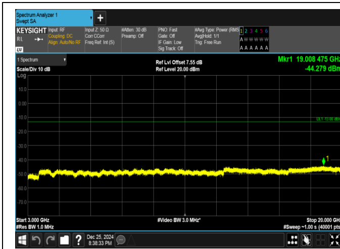
Band66-15MHz-QPSK-132047-75RB#0-3000~20000-PASS
