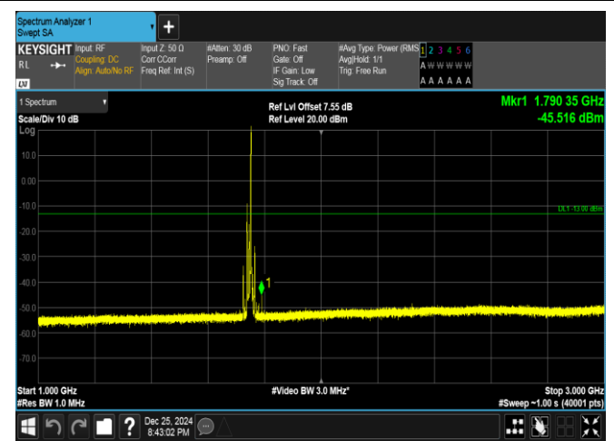
Band66-15MHz-QPSK-132322-1RB#74-1000~3000-PASS
