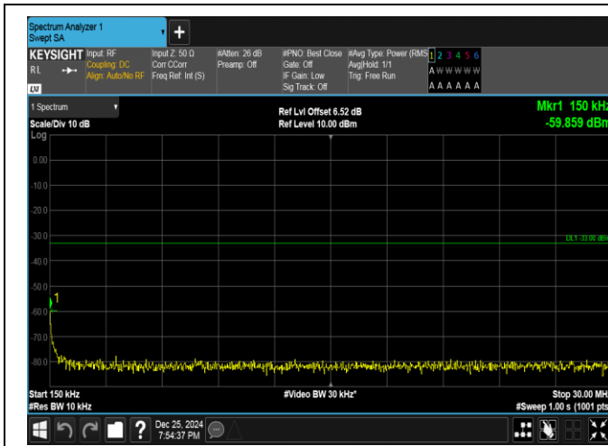
Band66-10MHz-16QAM-132622-1RB#0-0.15~30-PASS
