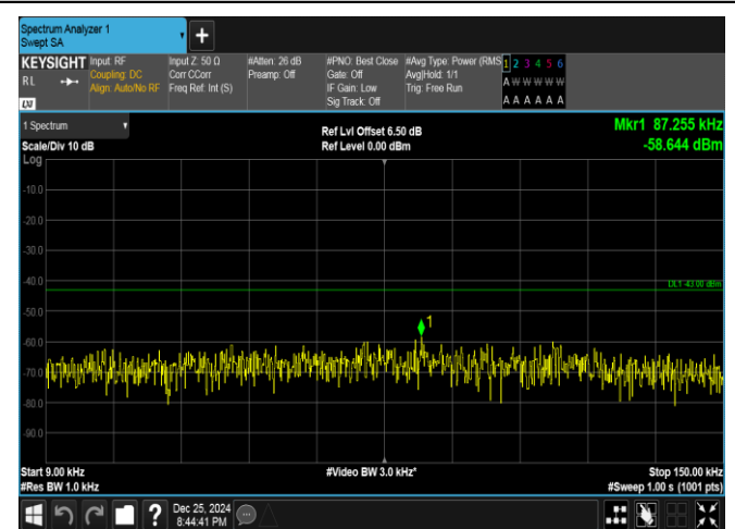
Band66-15MHz-QPSK-132322-75RB#0-0.009~0.15-PASS
