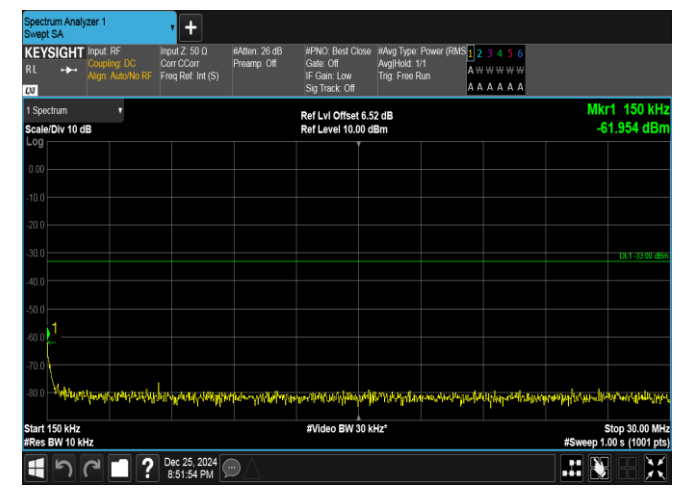
Band66-15MHz-QPSK-132597-75RB#0-0.15~30-PASS
