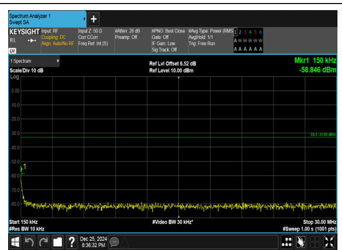
Band66-15MHz-16QAM-132047-1RB#74-0.15~30-PASS
