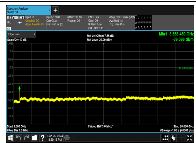
Band66-15MHz-QPSK-132597-1RB#74-3000~20000-PASS
