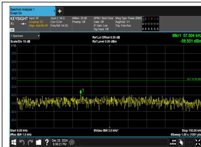
Band66-15MHz-16QAM-132047-1RB#74-0.009~0.15-PAS S
