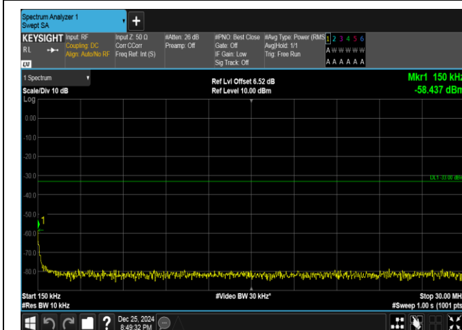
Band66-15MHz-QPSK-132597-1RB#74-0.15~30-PASS
