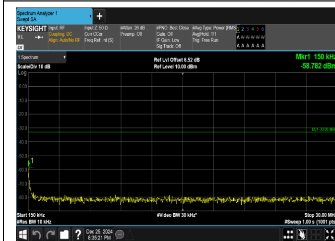
Band66-15MHz-QPSK-132047-1RB#74-0.15~30-PASS
