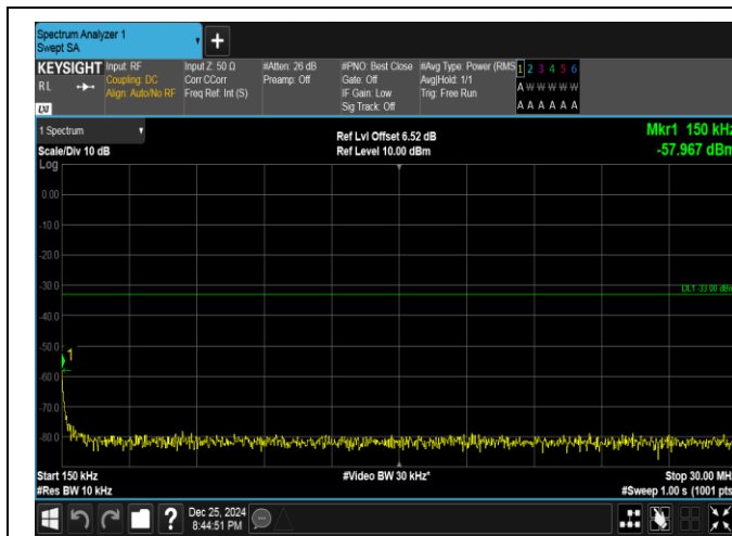
Band66-15MHz-QPSK-132322-75RB#0-0.15~30-PASS
