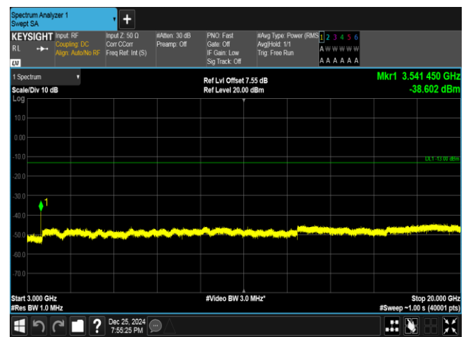
Band66-10MHz-16QAM-132622-1RB#0-3000~20000-PAS S
