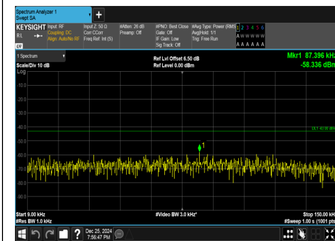
Band66-10MHz-16QAM-132622-1RB#49-0.009~0.15-PAS
