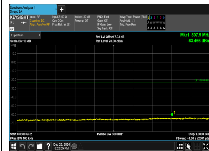
Band66-15MHz-QPSK-132597-75RB#0-30~1000-PASS
