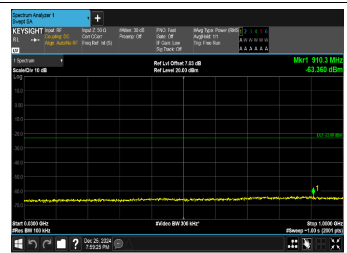
Band66-10MHz-16QAM-132622-50RB#0-30~1000-PASS
