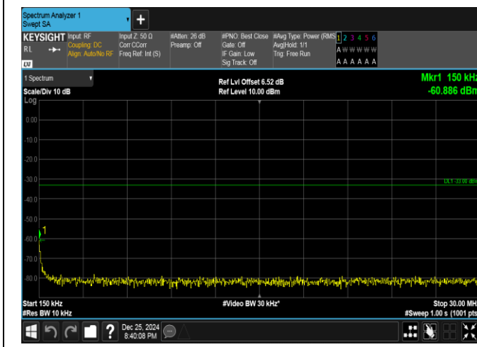
Band66-15MHz-QPSK-132322-1RB#0-0.15~30-PASS
