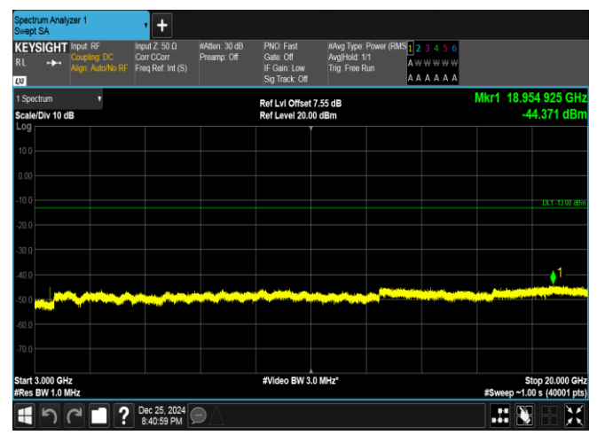
Band66-15MHz-QPSK-132322-1RB#0-3000~20000-PASS
