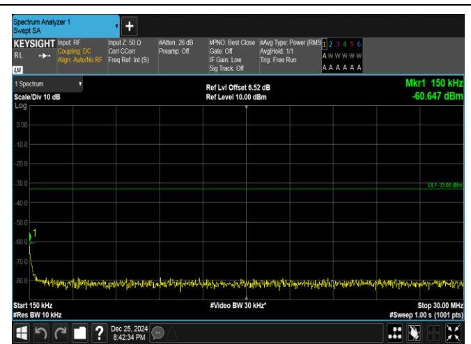
Band66-15MHz-QPSK-132322-1RB#74-0.15~30-PASS
