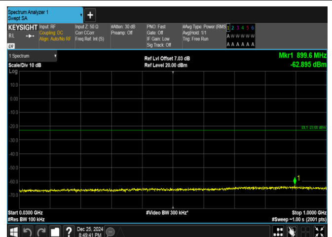
Band66-15MHz-QPSK-132597-1RB#74-30~1000-PASS
