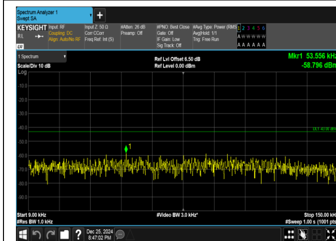
Band66-15MHz-QPSK-132597-1RB#0-0.009~0.15-PASS
