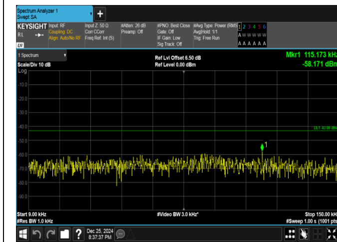
Band66-15MHz-QPSK-132047-75RB#0-0.009~0.15-PASS
