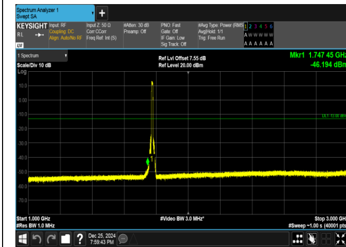
Band66-10MHz-16QAM-132622-50RB#0-1000~3000-PAS
