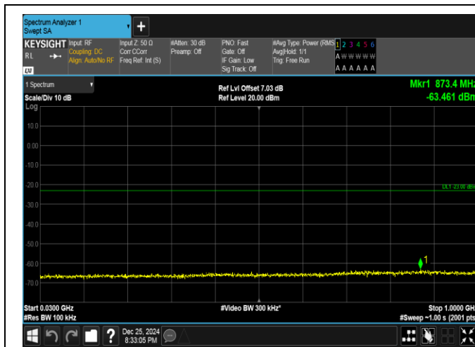
Band66-15MHz-QPSK-132047-1RB#0-30~1000-PASS
