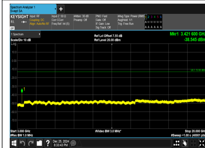
Band66-15MHz-QPSK-132047-1RB#0-3000~20000-PASS
