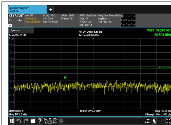
Band66-15MHz-QPSK-132322-1RB#74-0.009~0.15-PASS
