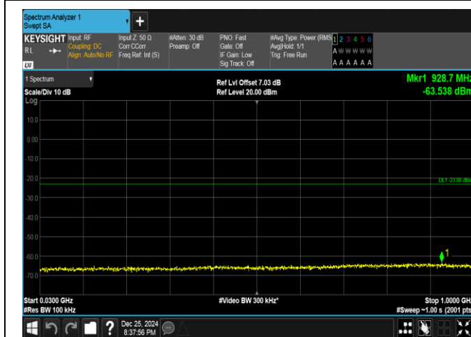
Band66-15MHz-QPSK-132047-75RB#0-30~1000-PASS
