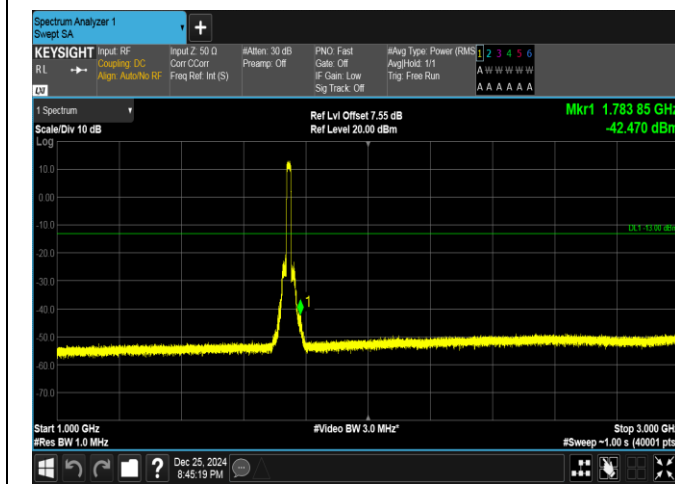
Band66-15MHz-QPSK-132322-75RB#0-1000~3000-PASS
