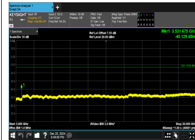
Band66-15MHz-QPSK-132597-1RB#0-3000~20000-PASS
