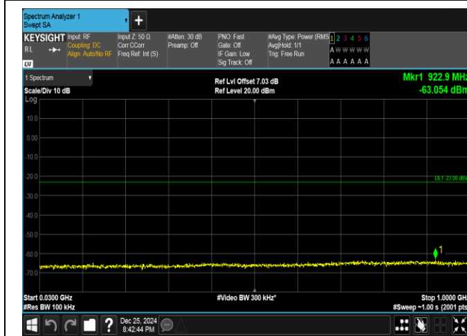
Band66-15MHz-QPSK-132322-1RB#74-30~1000-PASS
