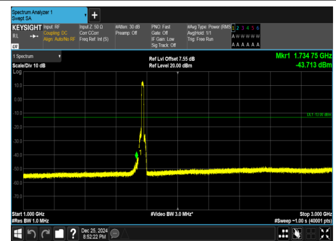
Band66-15MHz-QPSK-132597-75RB#0-1000~3000-PASS
