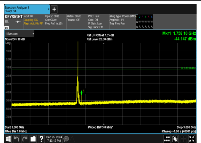
Band66-10MHz-16QAM-132022-1RB#49-1000~3000-PAS S
