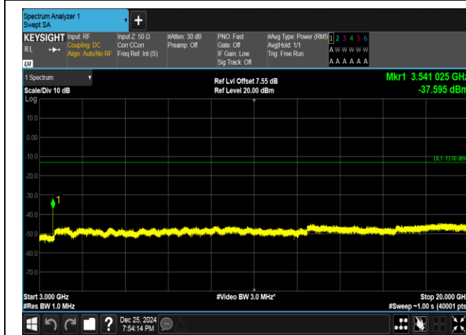
Band66-10MHz-QPSK-132622-1RB#0-3000~20000-PASS
