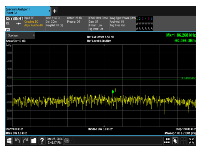
Band66-10MHz-QPSK-132322-1RB#0-0.009~0.15-PASS
