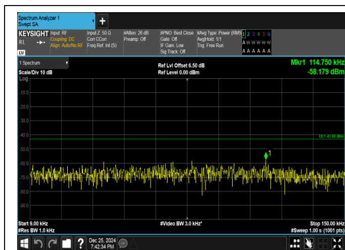
Band66-10MHz-16QAM-132022-1RB#49-0.009~0.15-PAS S
