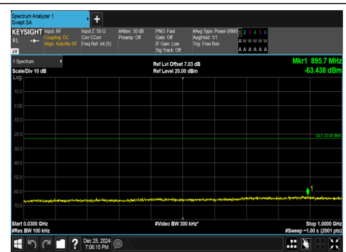
Band66-5MHz-16QAM-132647-25RB#0-30~1000-PASS
