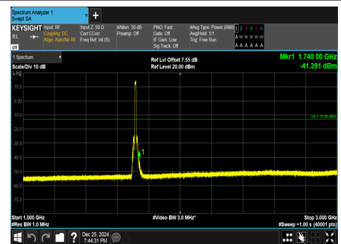
Band66-10MHz-QPSK-132022-50RB#0-1000~3000-PASS
