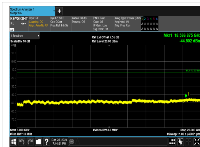
Band66-10MHz-QPSK-132022-50RB#0-3000~20000-PASS
