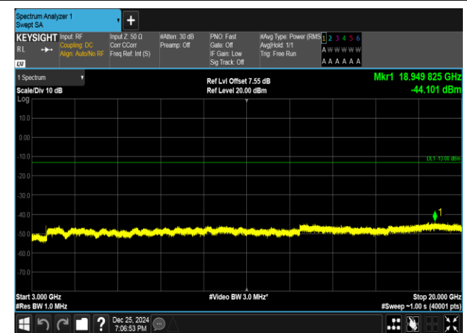
Band66-5MHz-16QAM-132647-25RB#0-3000~20000-PASS
