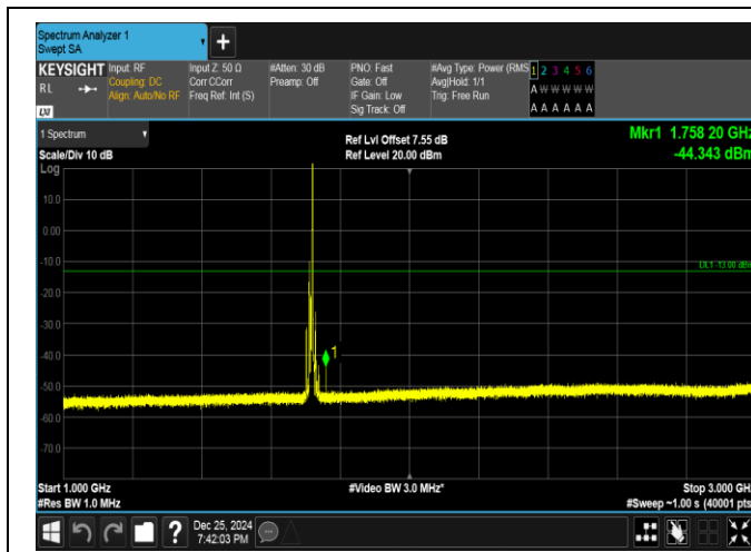
Band66-10MHz-QPSK-132022-1RB#49-1000~3000-PASS
