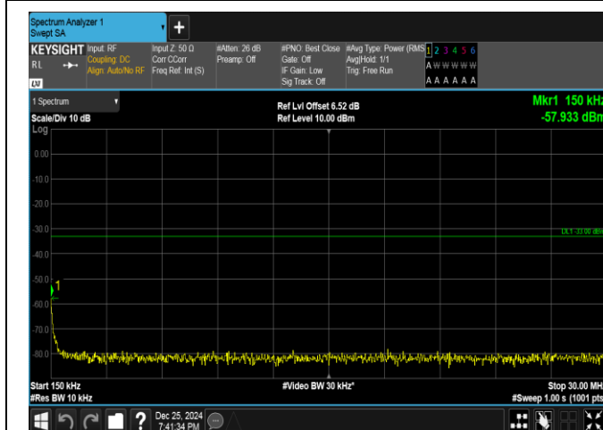
Band66-10MHz-QPSK-132022-1RB#49-0.15~30-PASS
