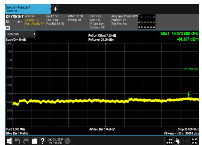
Band66-10MHz-QPSK-132322-1RB#0-3000~20000-PASS
