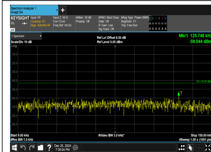
Band66-10MHz-QPSK-132022-1RB#0-0.009~0.15-PASS
