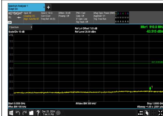
Band66-10MHz-QPSK-132022-50RB#0-30~1000-PASS
