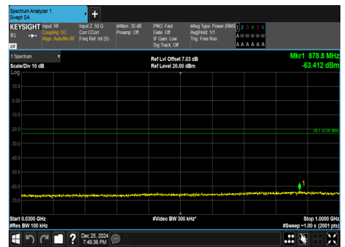
Band66-10MHz-QPSK-132322-1RB#0-30~1000-PASS
