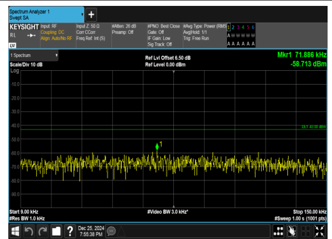
Band66-10MHz-QPSK-132622-1RB#49-0.009~0.15-PASS
