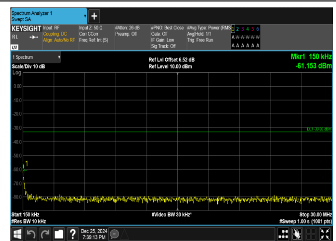
Band66-10MHz-QPSK-132022-1RB#0-0.15~30-PASS
