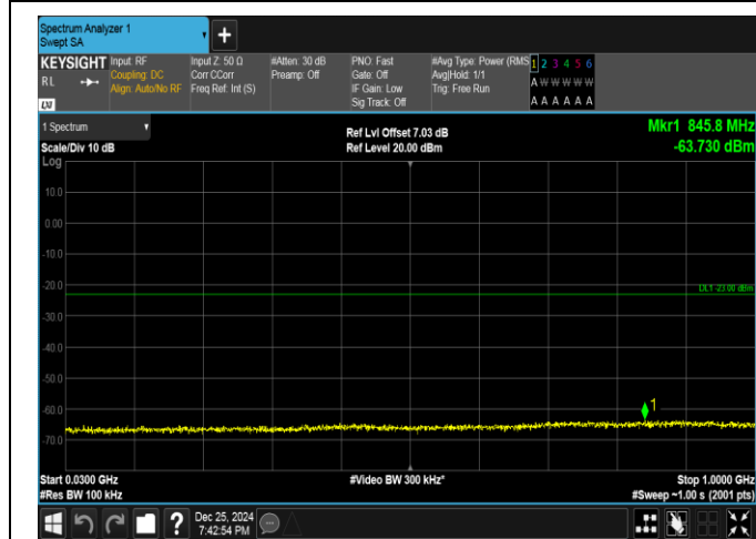
Band66-10MHz-16QAM-132022-1RB#49-30~1000-PASS
