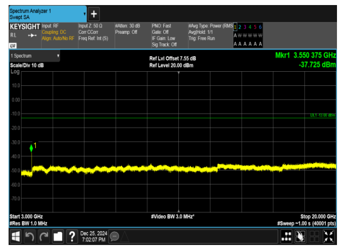
Band66-5MHz-16QAM-132647-1RB#0-3000~20000-PASS
