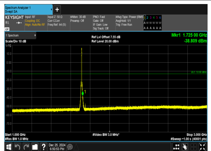
Band66-5MHz-QPSK-131997-25RB#0-1000~3000-PASS
