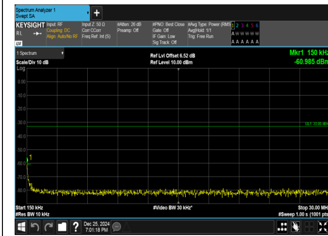
Band66-5MHz-16QAM-132647-1RB#0-0.15~30-PASS
