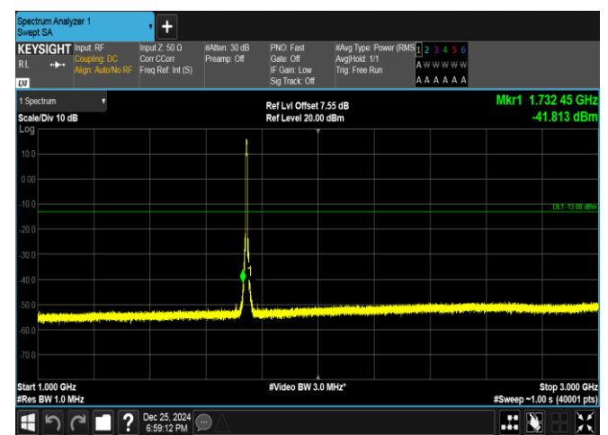
Band66-5MHz-16QAM-132322-25RB#0-1000~3000-PASS
