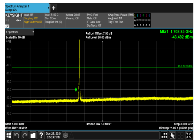
Band66-5MHz-QPSK-132322-1RB#24-1000~3000-PASS
