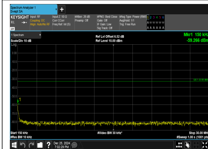
Band66-5MHz-QPSK-132647-1RB#24-0.15~30-PASS
