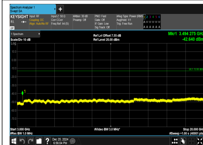
Band66-5MHz-QPSK-132322-1RB#24-3000~20000-PASS
