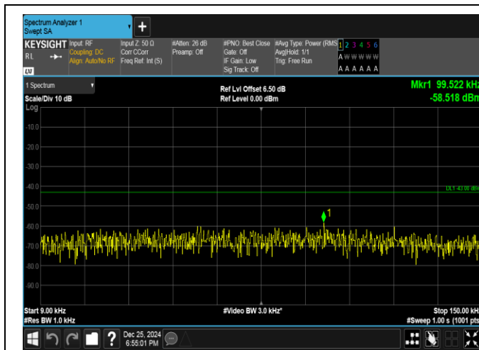
Band66-5MHz-QPSK-132322-1RB#24-0.009~0.15-PASS
