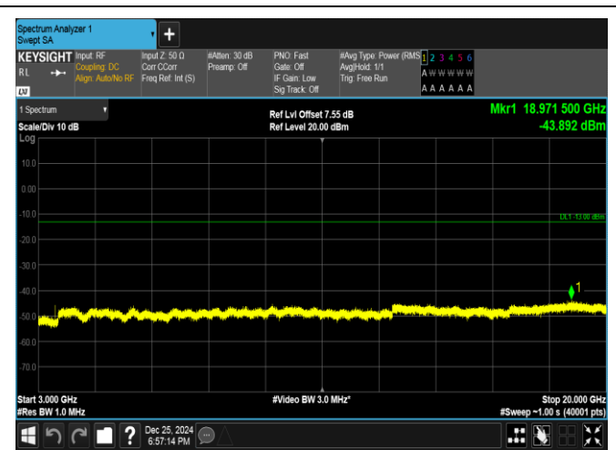
Band66-5MHz-16QAM-132322-1RB#24-3000~20000-PASS
