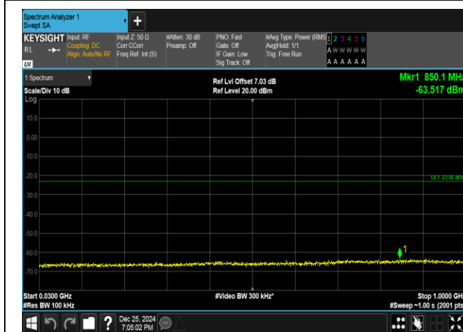
Band66-5MHz-QPSK-132647-25RB#0-30~1000-PASS
