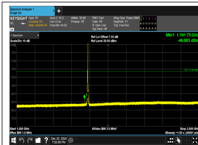
Band66-5MHz-QPSK-132647-1RB#24-1000~3000-PASS
