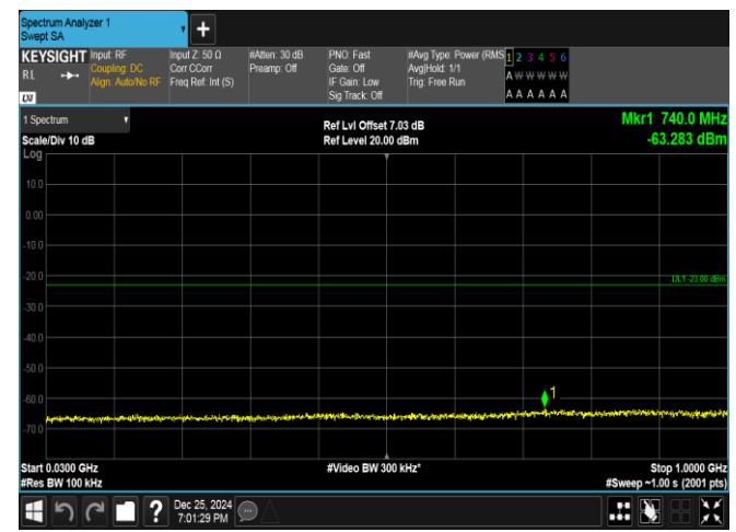
Band66-5MHz-16QAM-132647-1RB#0-30~1000-PASS
