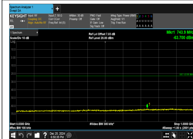
Band66-5MHz-QPSK-131997-25RB#0-30~1000-PASS
