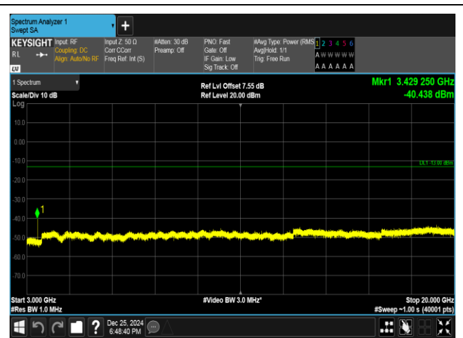
Band66-5MHz-QPSK-131997-1RB#24-3000~20000-PASS
