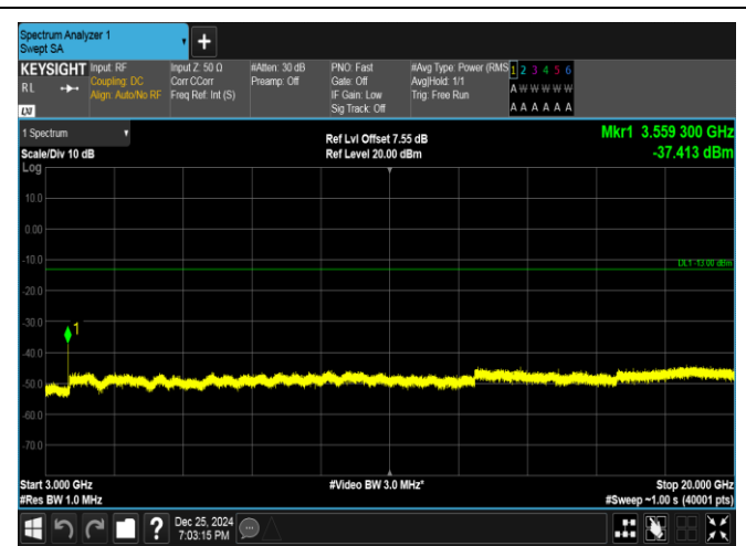
Band66-5MHz-QPSK-132647-1RB#24-3000~20000-PASS
