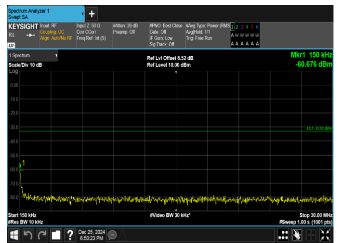
Band66-5MHz-QPSK-131997-25RB#0-0.15~30-PASS
