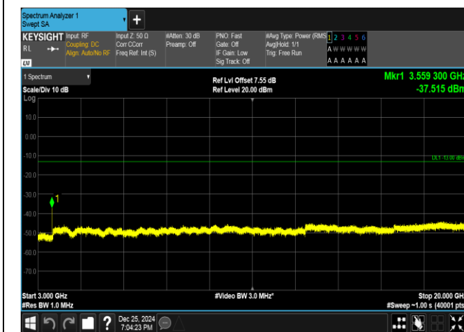
Band66-5MHz-16QAM-132647-1RB#24-3000~20000-PAS
