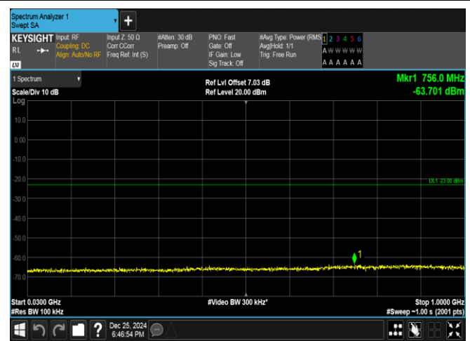
Band66-5MHz-16QAM-131997-1RB#0-30~1000-PASS
