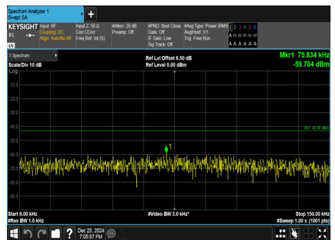
Band66-5MHz-16QAM-132647-25RB#0-0.009~0.15-PASS
