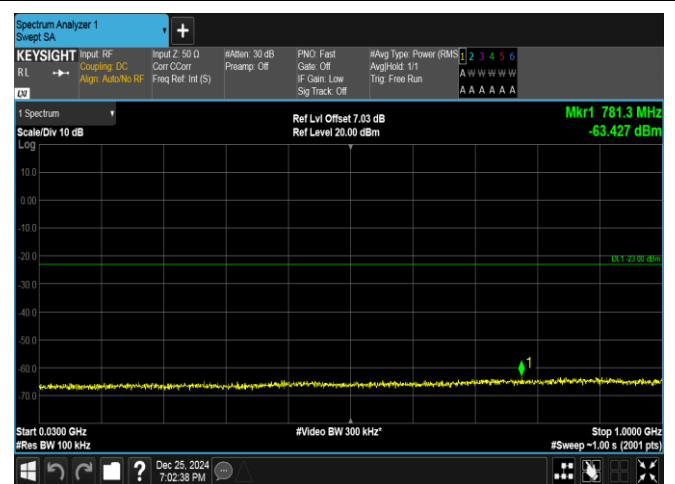
Band66-5MHz-QPSK-132647-1RB#24-30~1000-PASS
