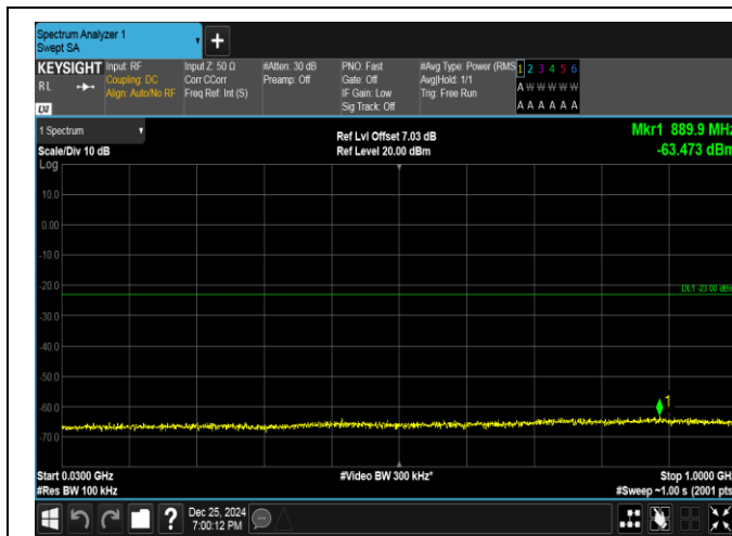
Band66-5MHz-QPSK-132647-1RB#0-30~1000-PASS
