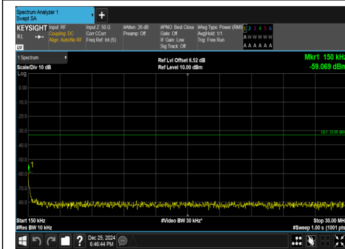
Band66-5MHz-16QAM-131997-1RB#0-0.15~30-PASS
