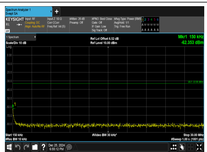
Band66-5MHz-QPSK-132322-1RB#24-0.15~30-PASS
