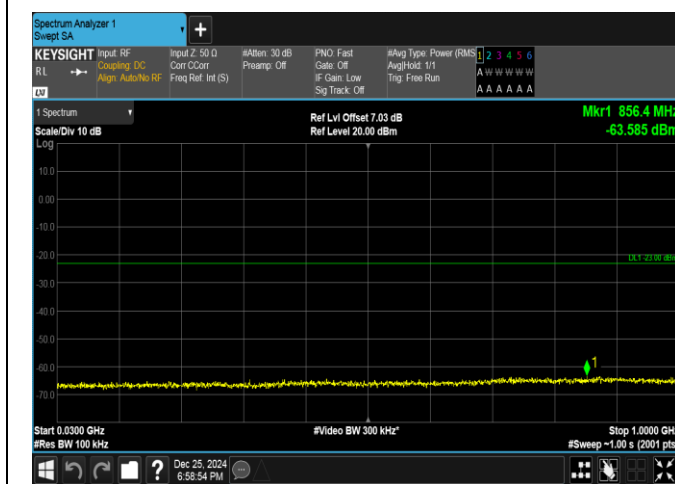
Band66-5MHz-16QAM-132322-25RB#0-30~1000-PASS
