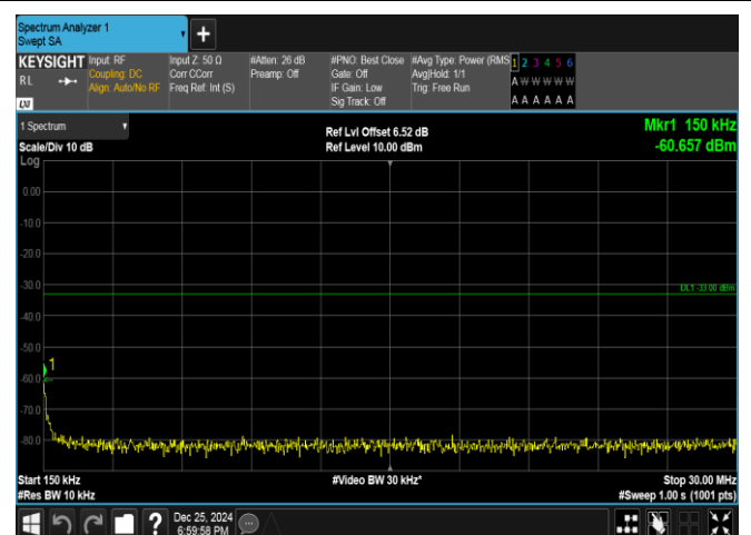
Band66-5MHz-QPSK-132647-1RB#0-0.15~30-PASS
