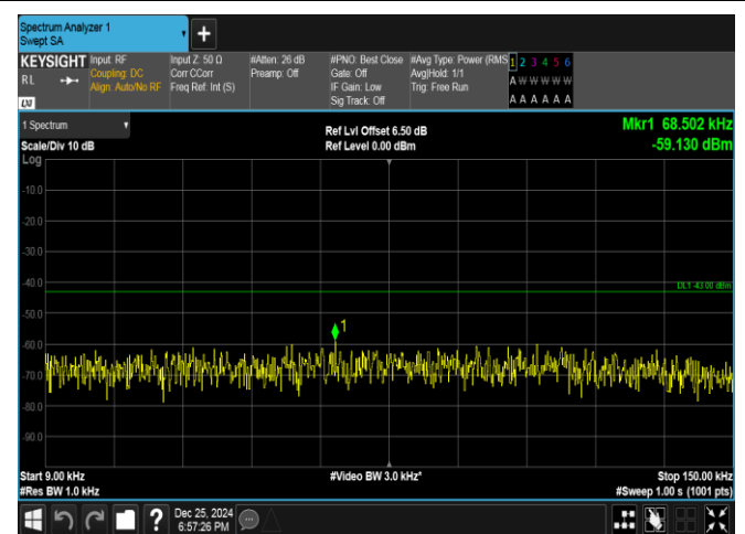
Band66-5MHz-QPSK-132322-25RB#0-0.009~0.15-PASS
