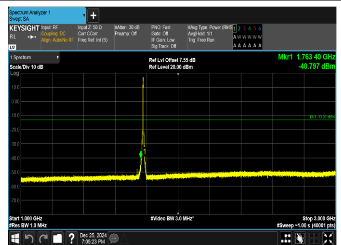
Band66-5MHz-QPSK-132647-25RB#0-1000~3000-PASS
