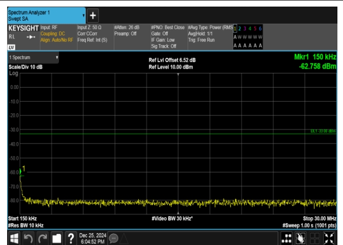
Band66-3MHz-QPSK-132657-1RB#0-0.15~30-PASS
