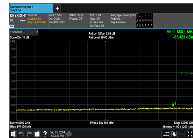
Band66-3MHz-16QAM-132322-15RB#0-30~1000-PASS
