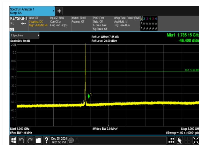
Band66-3MHz-16QAM-132322-1RB#14-1000~3000-PASS
