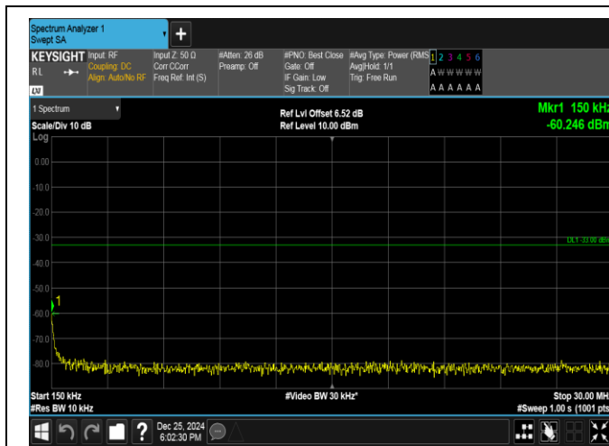
Band66-3MHz-QPSK-132322-15RB#0-0.15~30-PASS
