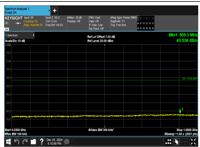
Band66-3MHz-16QAM-132657-15RB#0-30~1000-PASS
