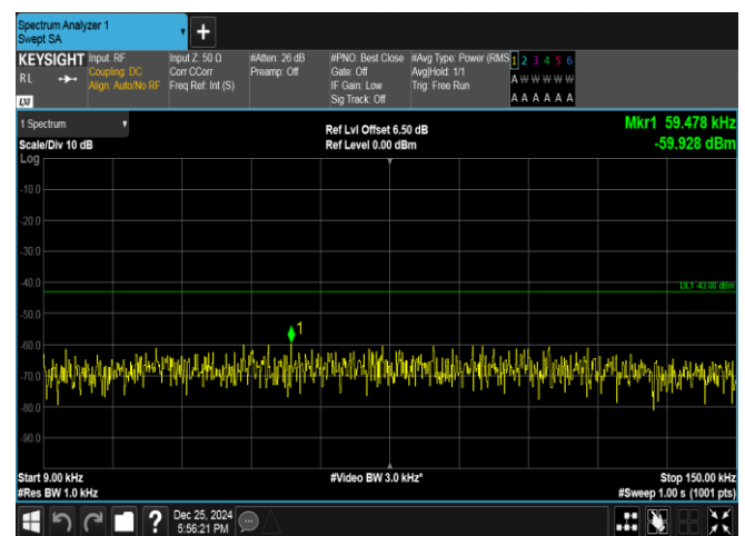
Band66-3MHz-16QAM-131987-15RB#0-0.009~0.15-PASS
