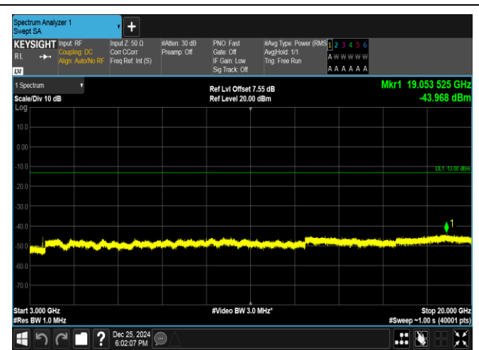
Band66-3MHz-16QAM-132322-1RB#14-3000~20000-PASS
