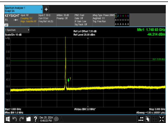
Band66-5MHz-QPSK-131997-1RB#0-1000~3000-PASS
