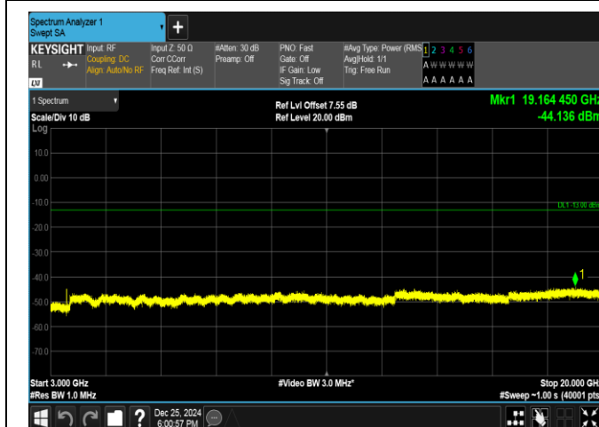
Band66-3MHz-QPSK-132322-1RB#14-3000~20000-PASS
