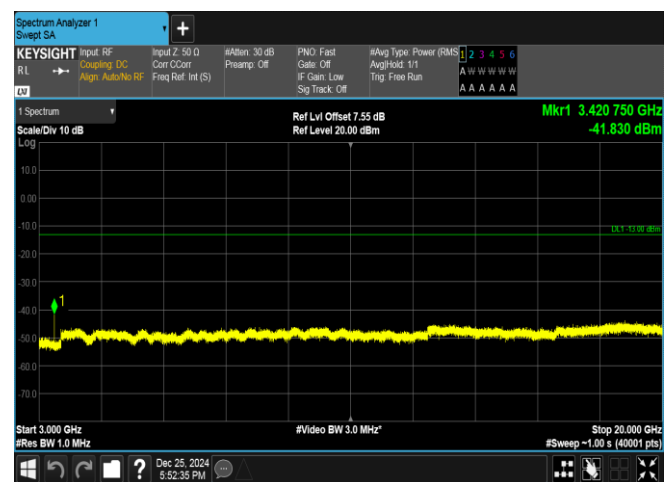
Band66-3MHz-16QAM-131987-1RB#0-3000~20000-PASS
