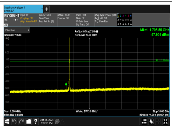
Band66-3MHz-16QAM-132322-1RB#0-1000~3000-PASS
