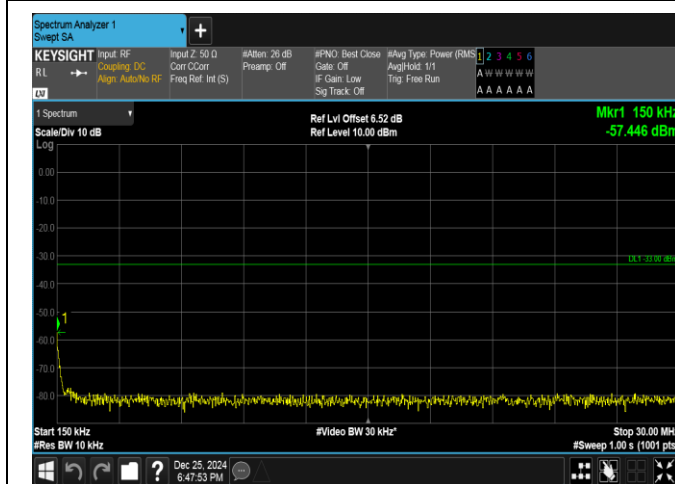
Band66-5MHz-QPSK-131997-1RB#24-0.15~30-PASS
