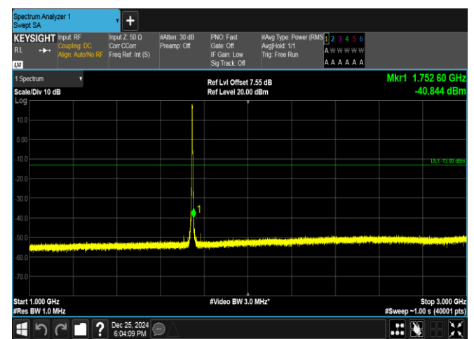
Band66-3MHz-16QAM-132322-15RB#0-1000~3000-PASS
