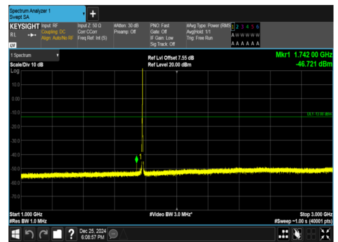
Band66-3MHz-16QAM-132657-1RB#14-1000~3000-PASS
