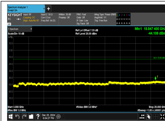
Band66-3MHz-16QAM-132322-15RB#0-3000~20000-PAS
