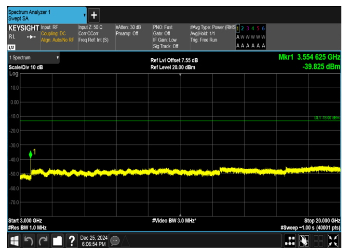
Band66-3MHz-16QAM-132657-1RB#0-3000~20000-PASS
