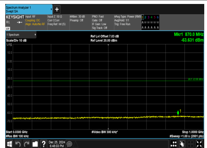
Band66-5MHz-QPSK-131997-1RB#24-30~1000-PASS
