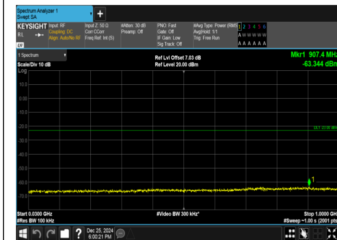
Band66-3MHz-QPSK-132322-1RB#14-30~1000-PASS
