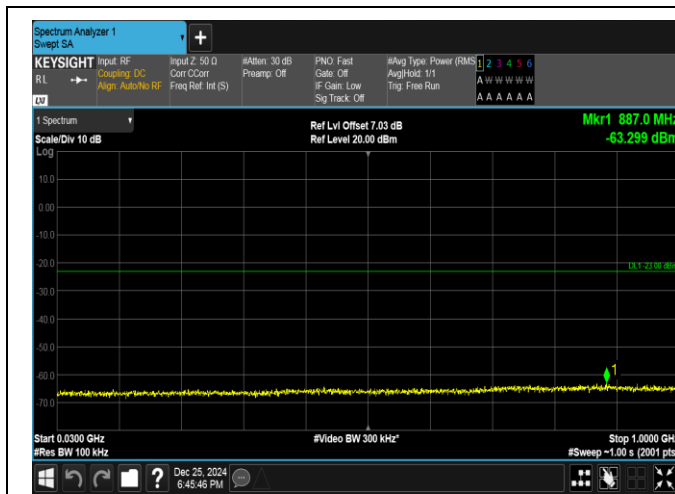
Band66-5MHz-QPSK-131997-1RB#0-30~1000-PASS
