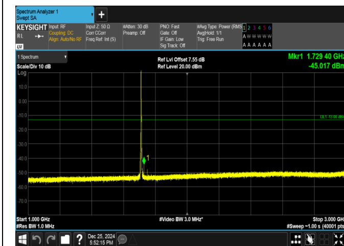
Band66-3MHz-16QAM-131987-1RB#0-1000~3000-PASS
