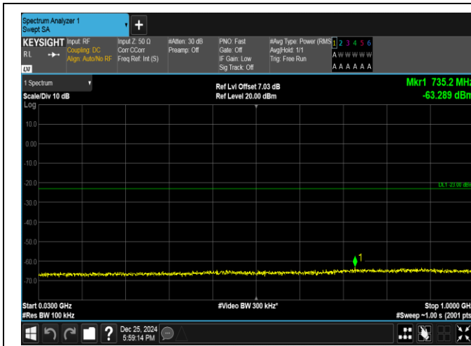
Band66-3MHz-16QAM-132322-1RB#0-30~1000-PASS
