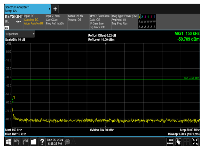
Band66-5MHz-QPSK-131997-1RB#0-0.15~30-PASS
