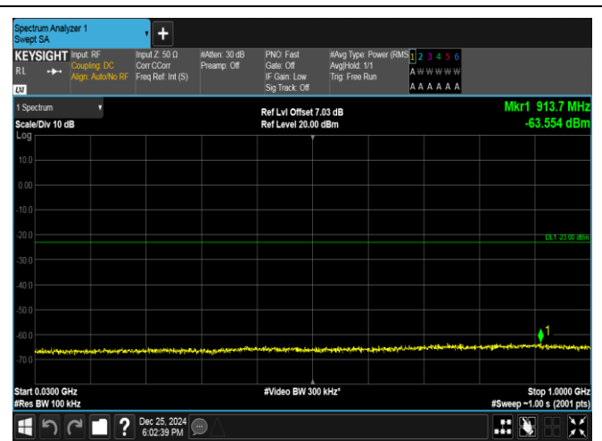
Band66-3MHz-QPSK-132322-15RB#0-30~1000-PASS
