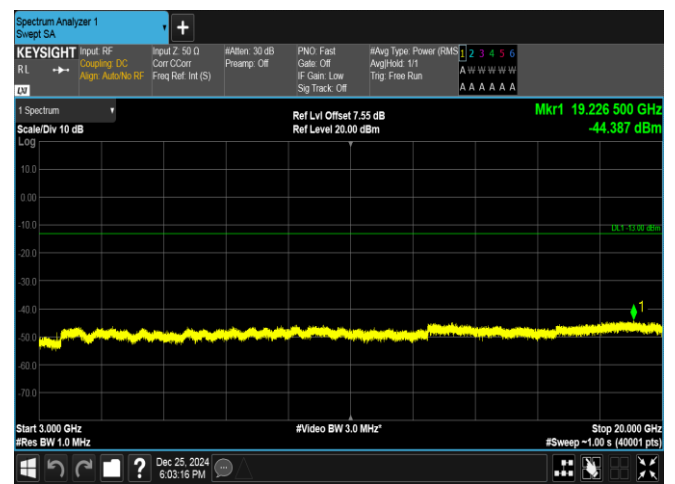
Band66-3MHz-QPSK-132322-15RB#0-3000~20000-PASS
