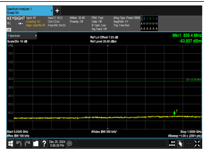
Band66-3MHz-16QAM-131987-15RB#0-30~1000-PASS
