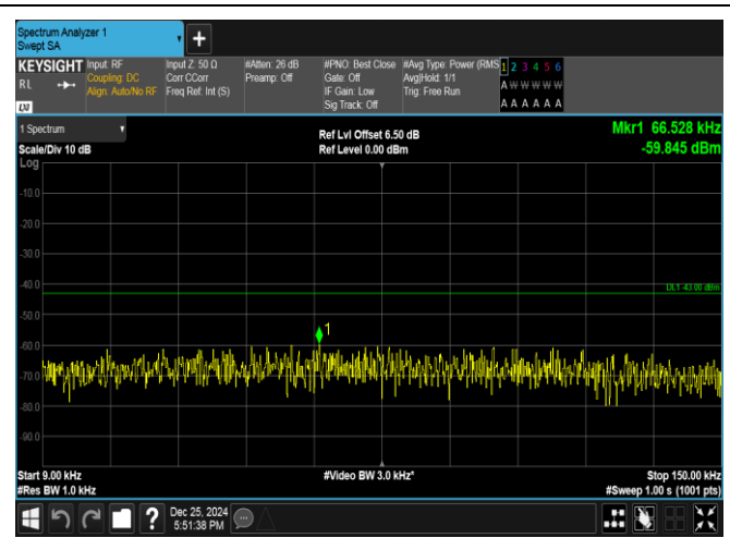
Band66-3MHz-16QAM-131987-1RB#0-0.009~0.15-PASS
