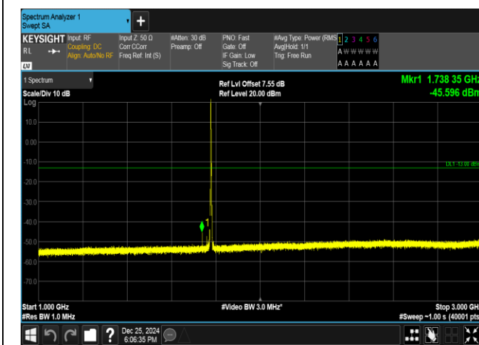
Band66-3MHz-16QAM-132657-1RB#0-1000~3000-PASS
