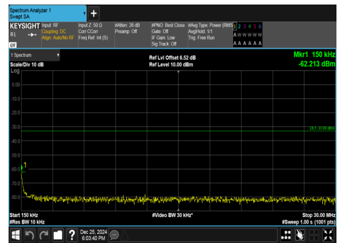
Band66-3MHz-16QAM-132322-15RB#0-0.15~30-PASS
