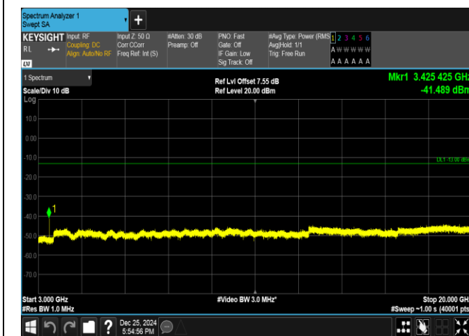
Band66-3MHz-16QAM-131987-1RB#14-3000~20000-PAS
