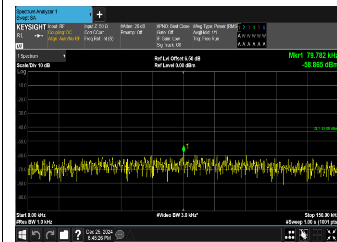
Band66-5MHz-QPSK-131997-1RB#0-0.009~0.15-PASS
