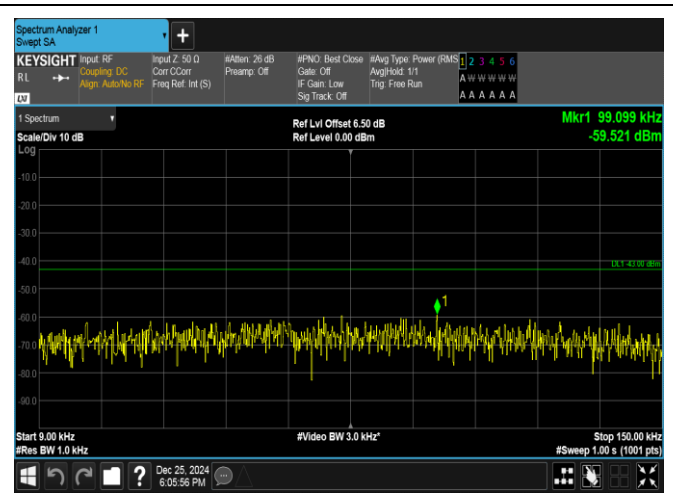
Band66-3MHz-16QAM-132657-1RB#0-0.009~0.15-PASS
