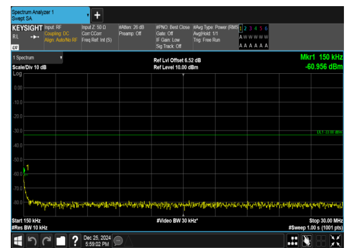
Band66-3MHz-16QAM-132322-1RB#0-0.15~30-PASS
