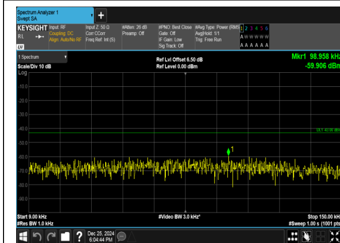
Band66-3MHz-QPSK-132657-1RB#0-0.009~0.15-PASS
