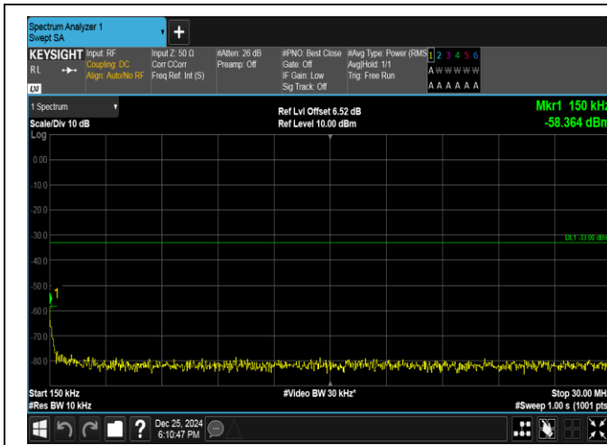
Band66-3MHz-16QAM-132657-15RB#0-0.15~30-PASS
