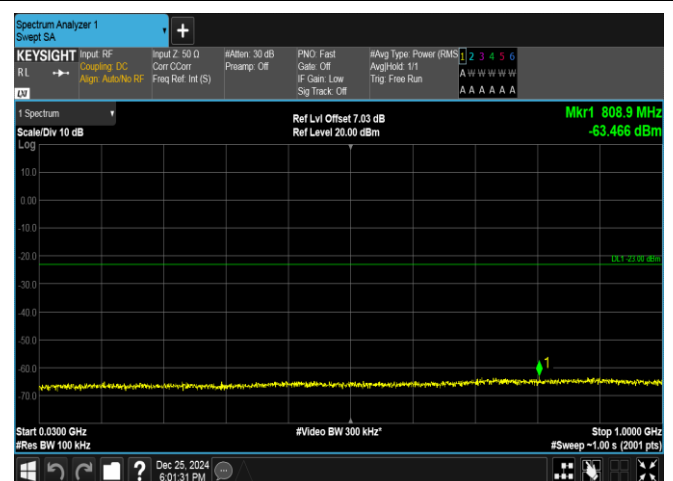
Band66-3MHz-16QAM-132322-1RB#14-30~1000-PASS
