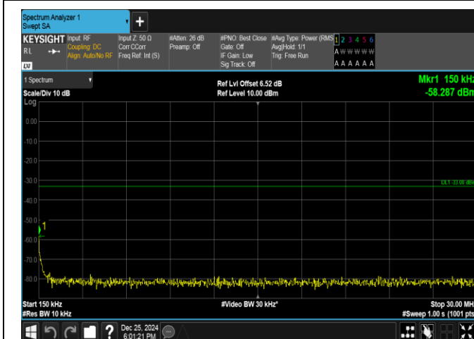
Band66-3MHz-16QAM-132322-1RB#14-0.15~30-PASS
