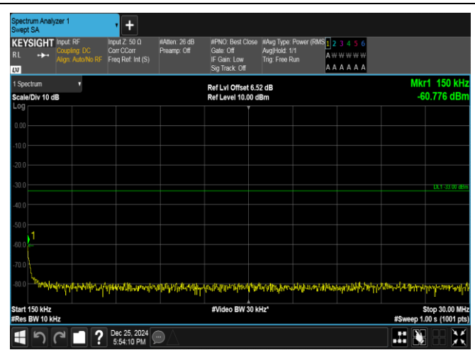
Band66-3MHz-16QAM-131987-1RB#14-0.15~30-PASS
