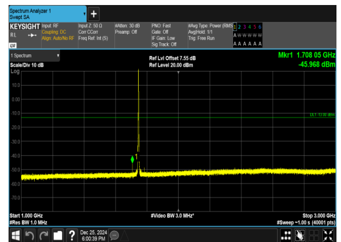
Band66-3MHz-QPSK-132322-1RB#14-1000~3000-PASS
