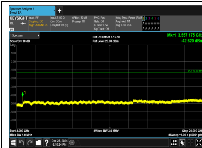
Band66-3MHz-QPSK-132657-15RB#0-3000~20000-PASS
