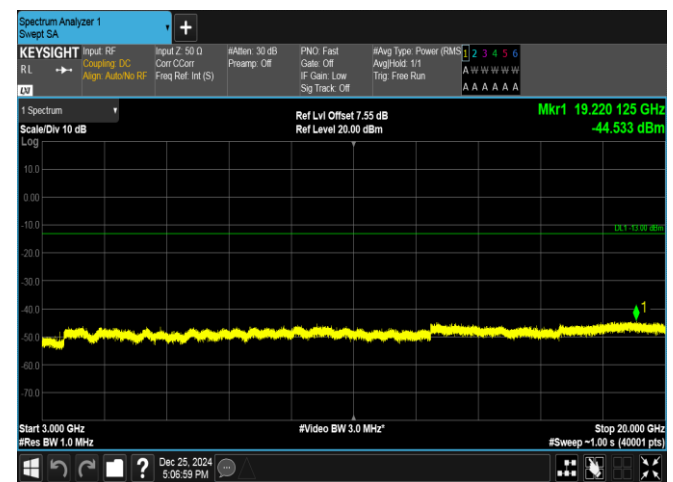
Band66-1.4MHz-16QAM-132322-1RB#5-3000~20000-PA
