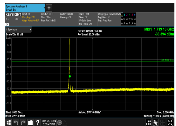
Band66-3MHz-QPSK-131987-15RB#0-1000~3000-PASS
