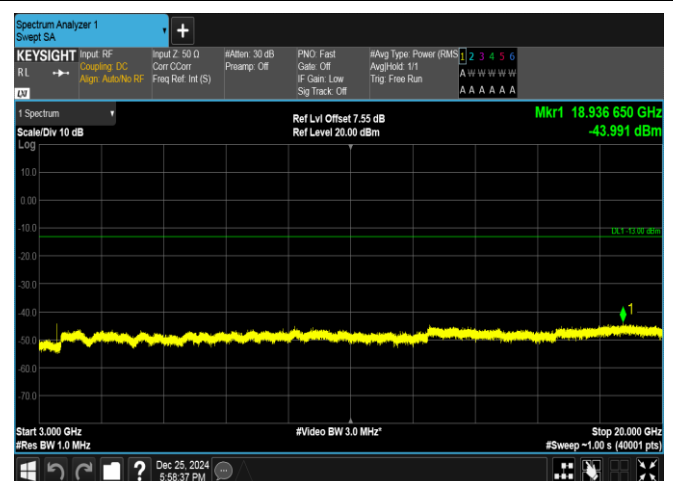
Band66-3MHz-QPSK-132322-1RB#0-3000~20000-PASS
