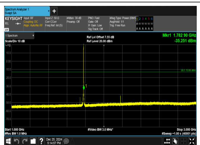
Band66-1.4MHz-QPSK-132665-6RB#0-1000~3000-PASS
