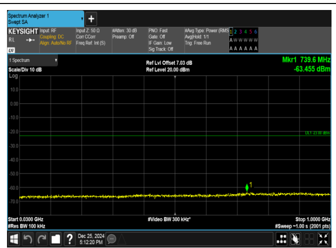
Band66-1.4MHz-QPSK-132665-1RB#5-30~1000-PASS
