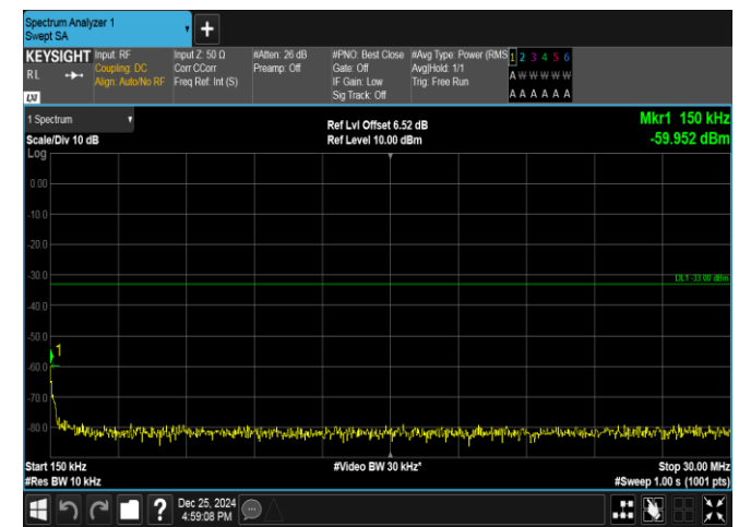
Band66-1.4MHz-16QAM-131979-1RB#5-0.15~30-PASS
