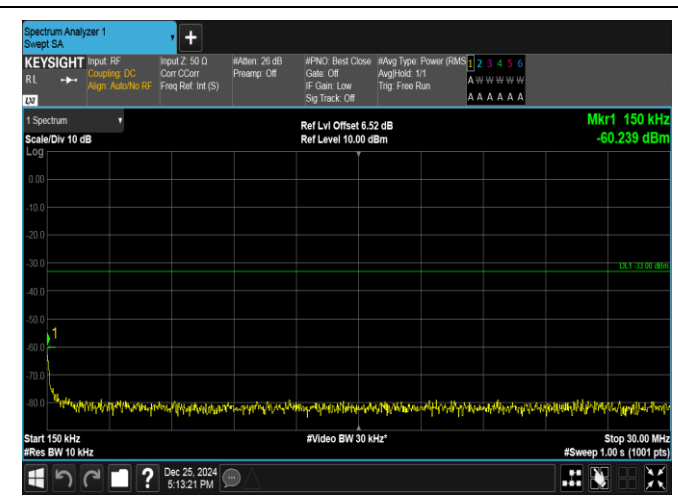
Band66-1.4MHz-16QAM-132665-1RB#5-0.15~30-PASS
