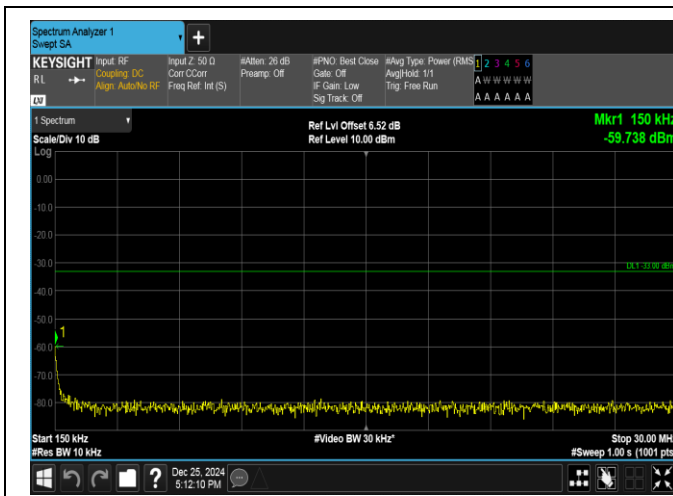
Band66-1.4MHz-QPSK-132665-1RB#5-0.15~30-PASS
