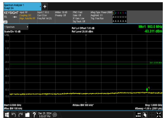
Band66-3MHz-QPSK-131987-1RB#14-30~1000-PASS
