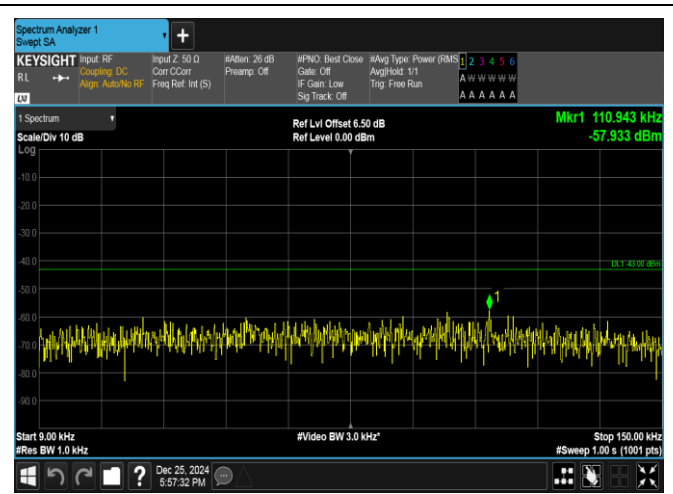
Band66-3MHz-QPSK-132322-1RB#0-0.009~0.15-PASS
