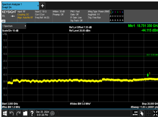
Band66-3MHz-QPSK-131987-1RB#0-3000~20000-PASS
