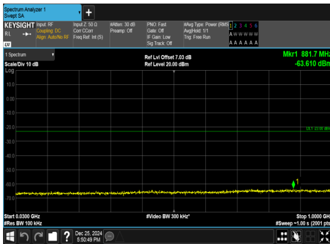
Band66-3MHz-QPSK-131987-1RB#0-30~1000-PASS
