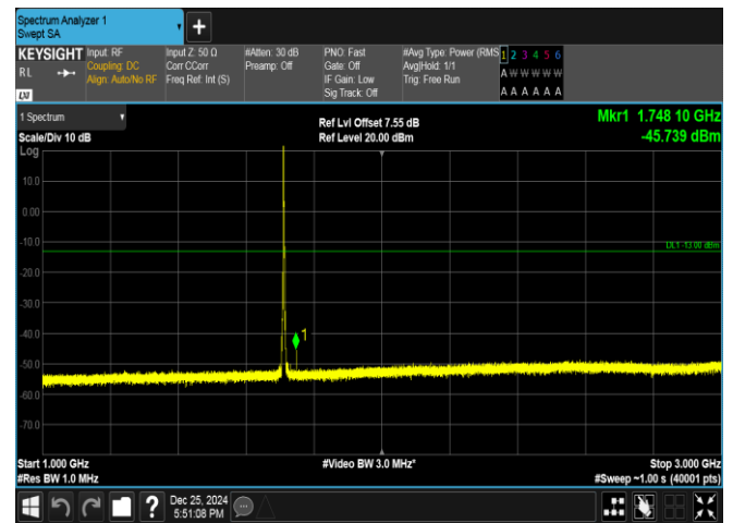
Band66-3MHz-QPSK-131987-1RB#0-1000~3000-PASS
