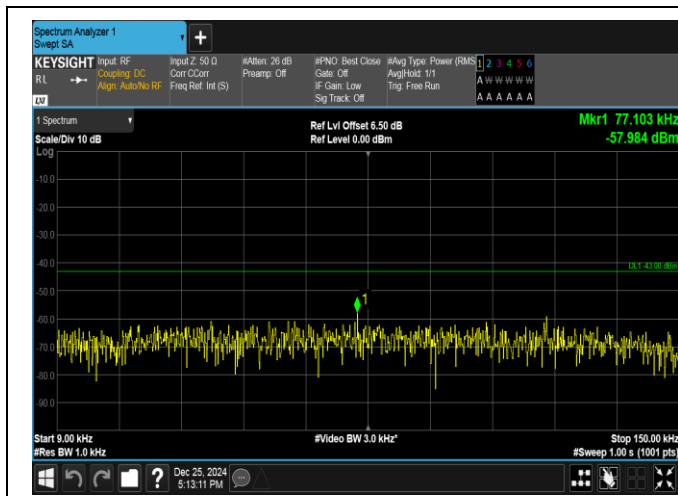
Band66-1.4MHz-16QAM-132665-1RB#5-0.009~0.15-PASS
