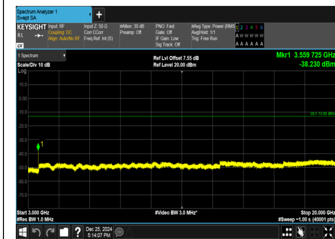
Band66-1.4MHz-16QAM-132665-1RB#5-3000~20000-PASS
