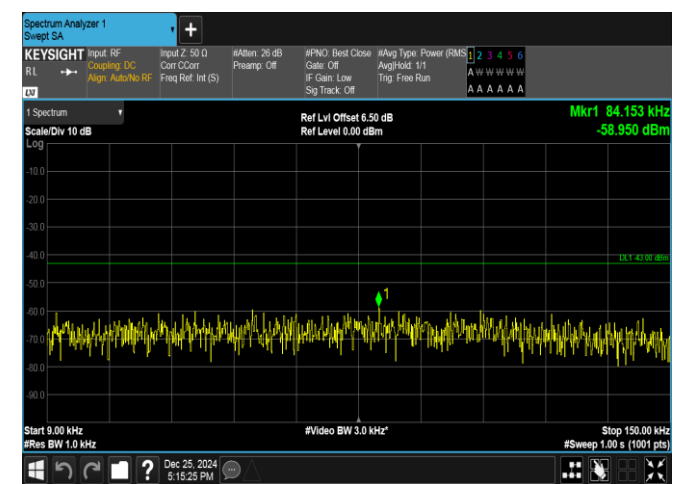
Band66-1.4MHz-16QAM-132665-6RB#0-0.009~0.15-PASS
