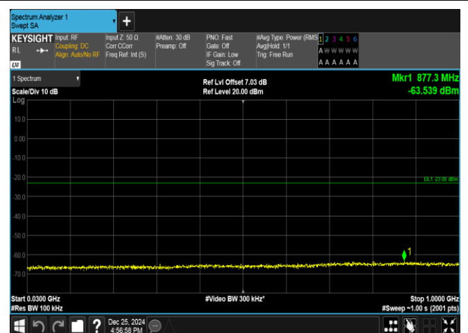
Band66-1.4MHz-16QAM-131979-1RB#0-30~1000-PASS
