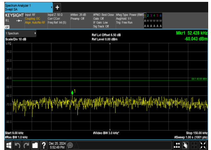
Band66-3MHz-QPSK-131987-1RB#14-0.009~0.15-PASS
