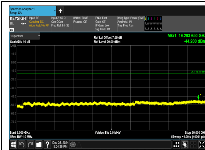
Band66-1.4MHz-16QAM-132322-1RB#0-3000~20000-PA SS
