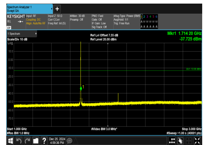
Band66-1.4MHz-16QAM-131979-1RB#5-1000~3000-PAS
