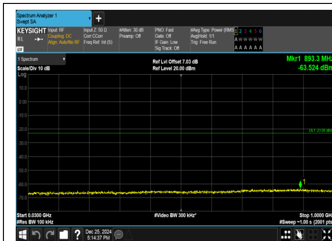
Band66-1.4MHz-QPSK-132665-6RB#0-30~1000-PASS
