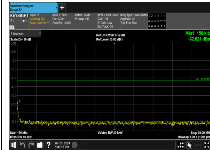
Band66-1.4MHz-16QAM-132322-1RB#5-0.15~30-PASS
