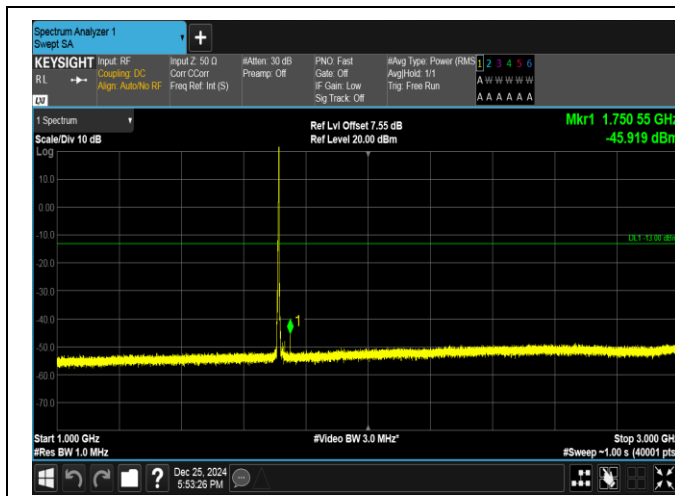
Band66-3MHz-QPSK-131987-1RB#14-1000~3000-PASS
