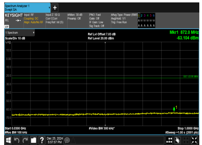
Band66-3MHz-QPSK-132322-1RB#0-30~1000-PASS
