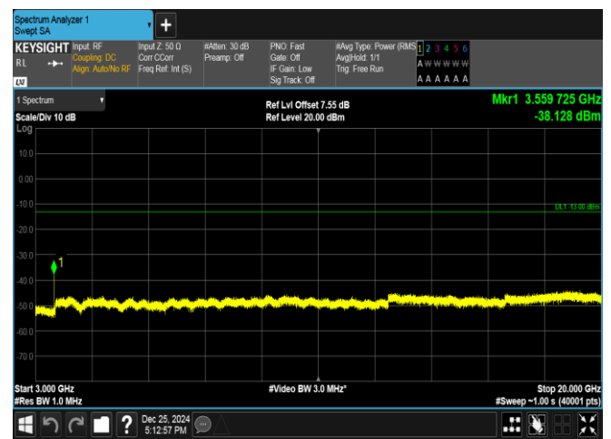
Band66-1.4MHz-QPSK-132665-1RB#5-3000~20000-PASS
