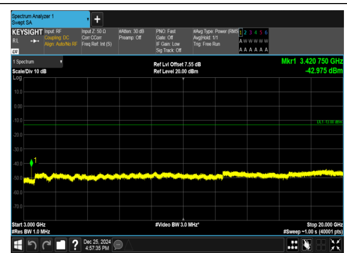
Band66-1.4MHz-16QAM-131979-1RB#0-3000~20000-PA
