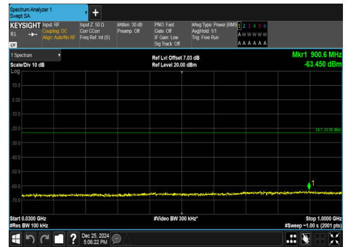
Band66-1.4MHz-16QAM-132322-1RB#5-30~1000-PASS
