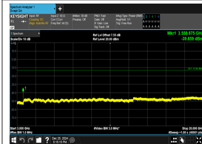
Band66-1.4MHz-QPSK-132665-6RB#0-3000~20000-PASS
