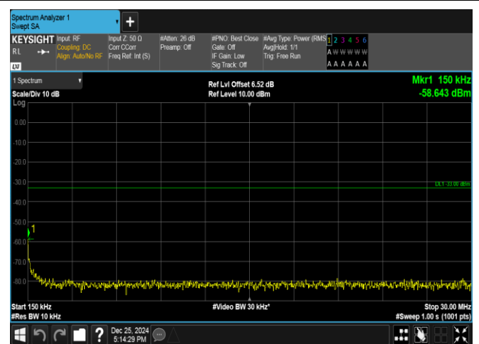
Band66-1.4MHz-QPSK-132665-6RB#0-0.15~30-PASS
