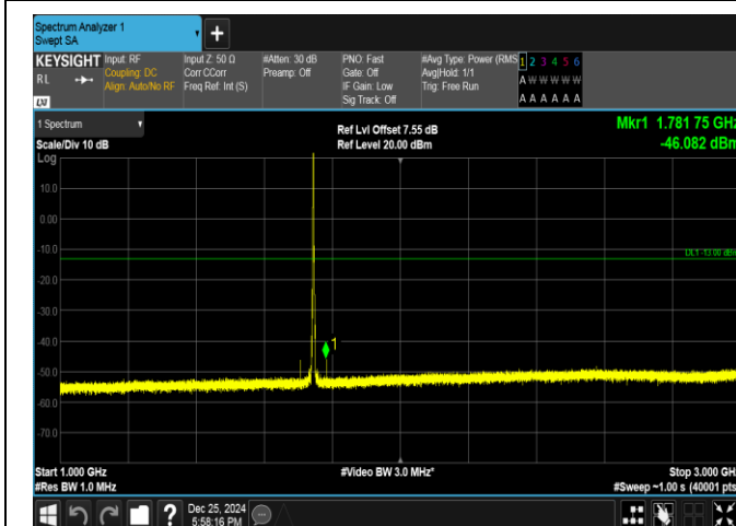
Band66-3MHz-QPSK-132322-1RB#0-1000~3000-PASS
