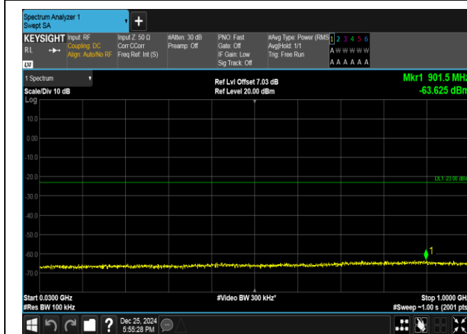
Band66-3MHz-QPSK-131987-15RB#0-30~1000-PASS
