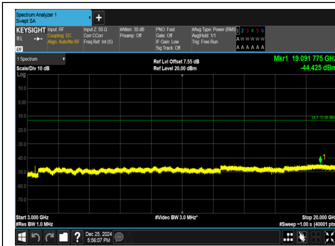
Band66-3MHz-QPSK-131987-15RB#0-3000~20000-PASS
