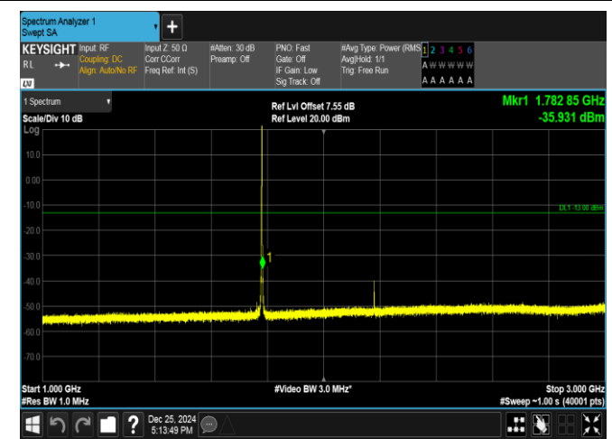
Band66-1.4MHz-16QAM-132665-1RB#5-1000~3000-PASS
