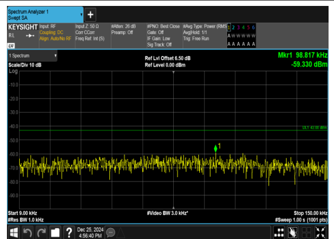
Band66-1.4MHz-16QAM-131979-1RB#0-0.009~0.15-PASS
