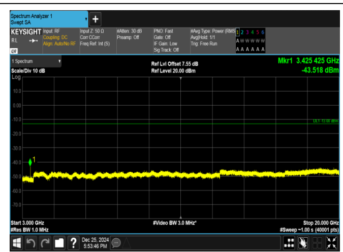
Band66-3MHz-QPSK-131987-1RB#14-3000~20000-PASS
