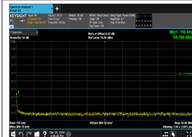
Band66-1.4MHz-16QAM-131979-1RB#0-0.15~30-PASS
