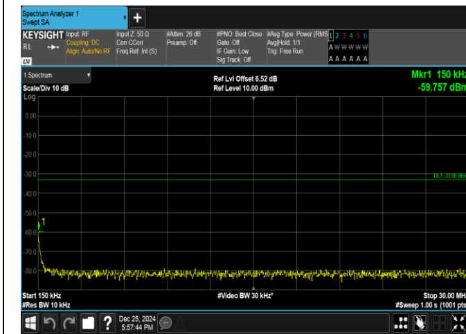
Band66-3MHz-QPSK-132322-1RB#0-0.15~30-PASS
