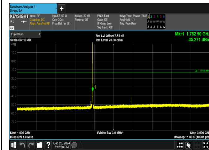
Band66-1.4MHz-QPSK-132665-1RB#5-1000~3000-PASS
