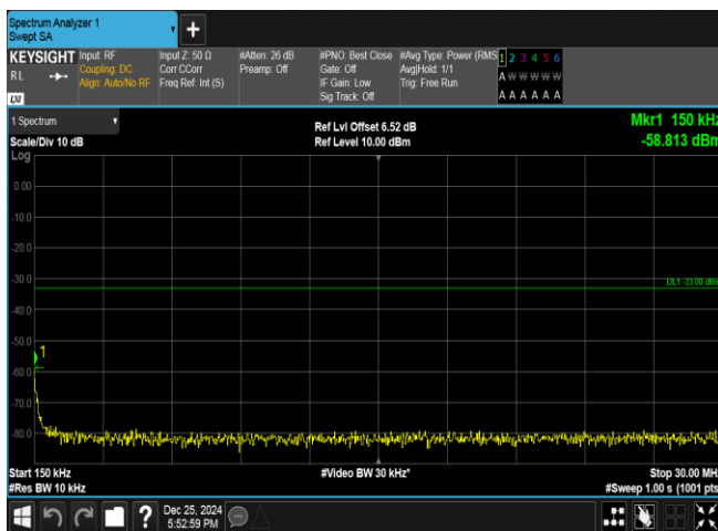
Band66-3MHz-QPSK-131987-1RB#14-0.15~30-PASS
