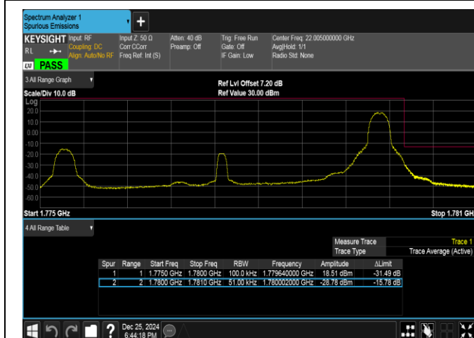
Band66-5MHz-QPSK-132647-1RB#24-PASS
