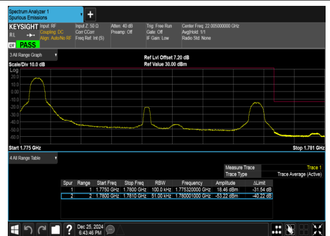
Band66-5MHz-QPSK-132647-1RB#0-PASS
