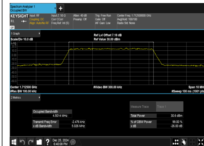
Band66-5MHz-QPSK-131997-25RB#0-PASS
