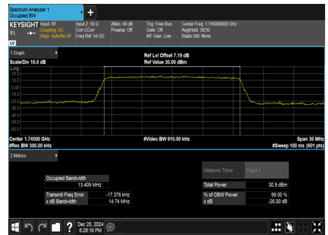
Band66-15MHz-QPSK-132322-75RB#0-PASS
