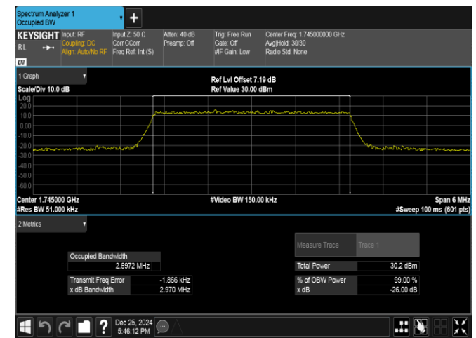
Band66-3MHz-QPSK-132322-15RB#0-PASS
