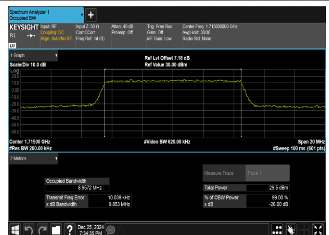
Band66-10MHz-16QAM-132022-50RB#0-PASS
