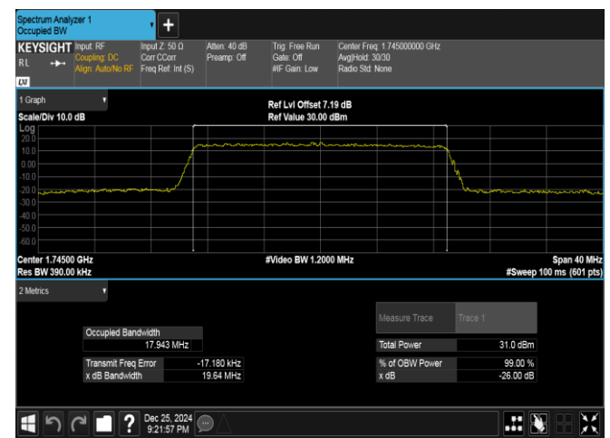
Band66-20MHz-QPSK-132322-100RB#0-PASS
