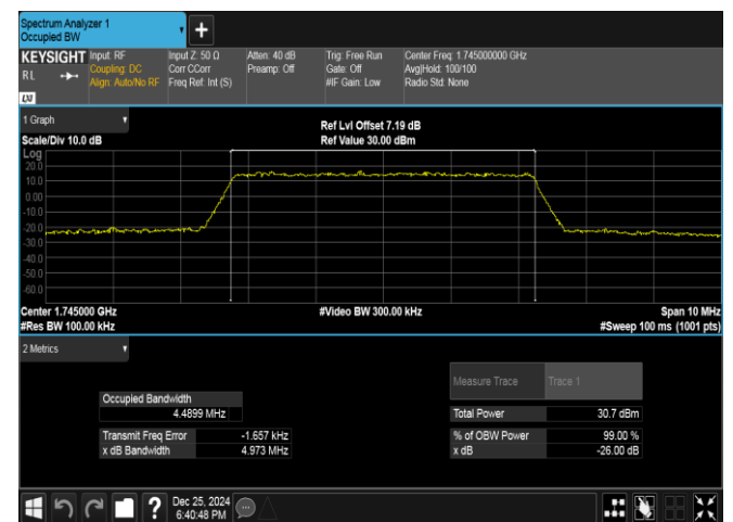
Band66-5MHz-QPSK-132322-25RB#0-PASS
