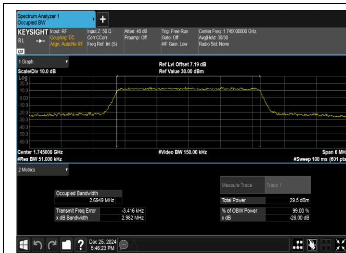
Band66-3MHz-16QAM-132322-15RB#0-PASS
