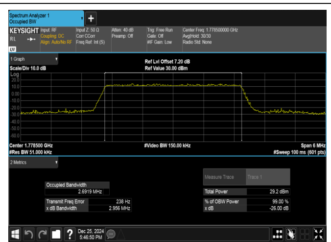
Band66-3MHz-16QAM-132657-15RB#0-PASS
