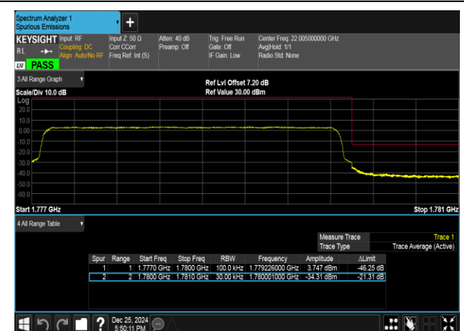
Band66-3MHz-16QAM-132657-15RB#0-PASS
