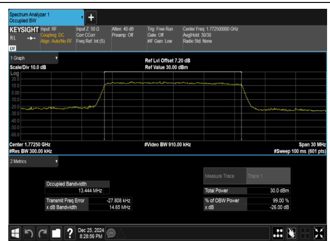
Band66-15MHz-16QAM-132597-75RB#0-PASS
