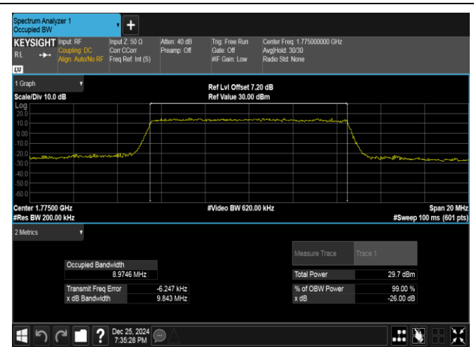
Band66-10MHz-16QAM-132622-50RB#0-PASS
