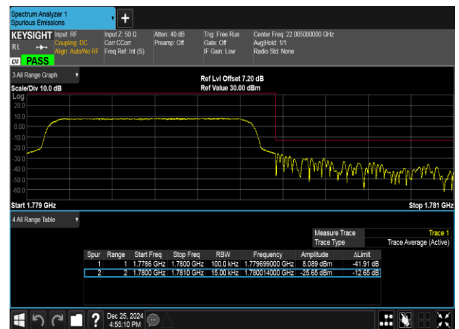
Band66-1.4MHz-16QAM-132665-6RB#0-PASS
