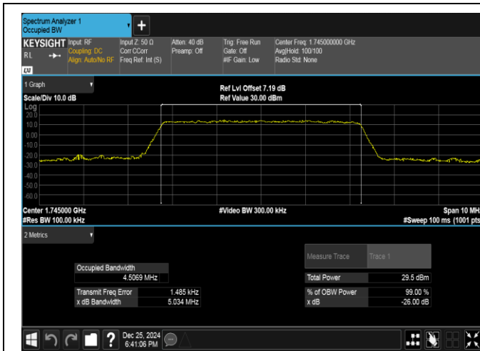
Band66-5MHz-16QAM-132322-25RB#0-PASS
