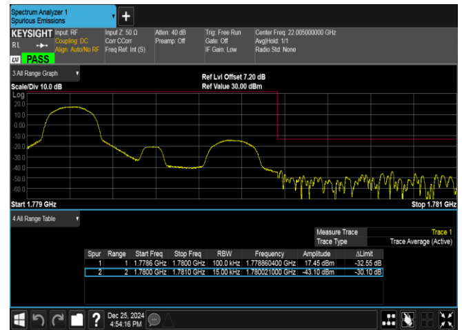
Band66-1.4MHz-16QAM-132665-1RB#0-PASS
