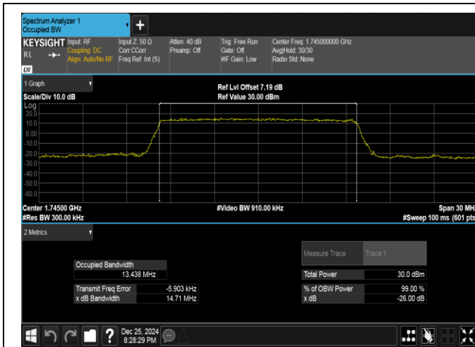
Band66-15MHz-16QAM-132322-75RB#0-PASS
