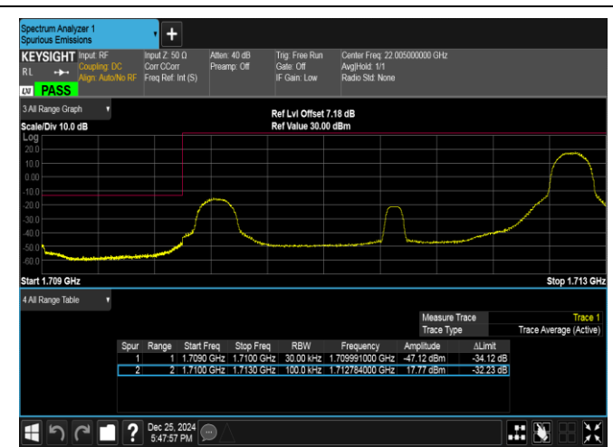
Band66-3MHz-16QAM-131987-1RB#14-PASS
