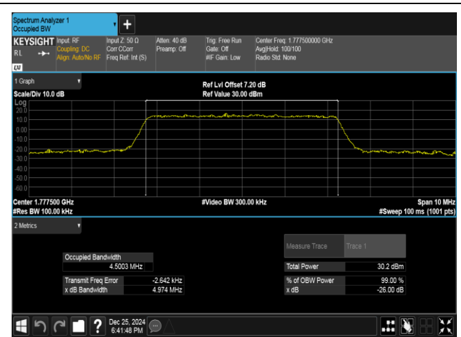
Band66-5MHz-16QAM-132647-25RB#0-PASS
