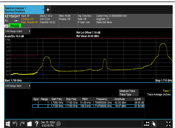
Band66-5MHz-QPSK-131997-1RB#24-PASS
