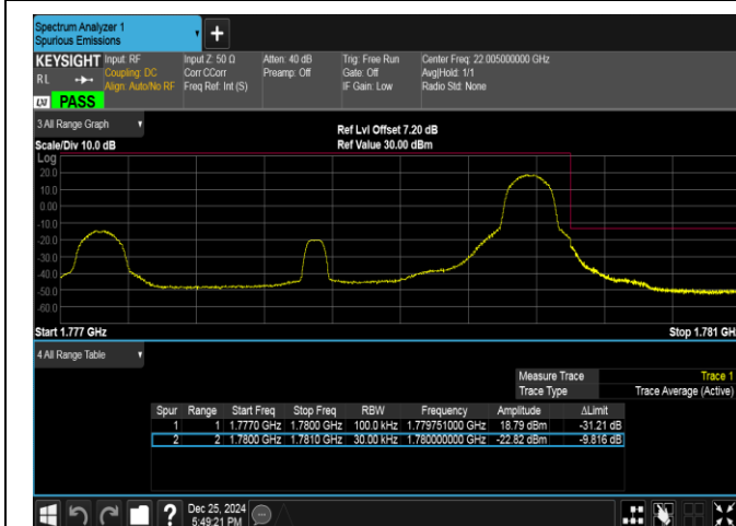
Band66-3MHz-QPSK-132657-1RB#14-PASS
