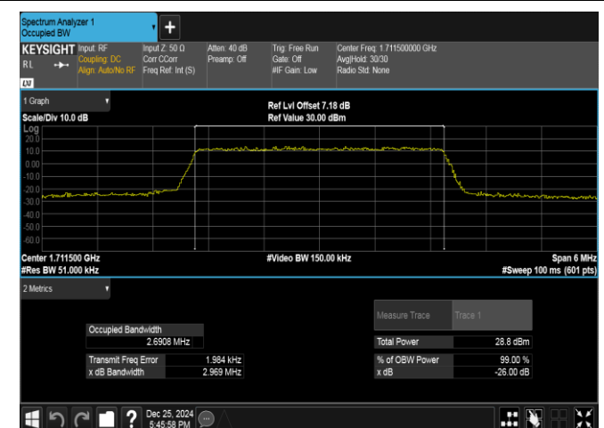
Band66-3MHz-16QAM-131987-15RB#0-PASS
