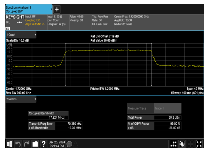
Band66-20MHz-16QAM-132072-100RB#0-PASS
