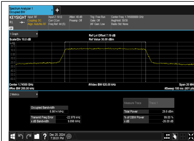
Band66-10MHz-16QAM-132322-50RB#0-PASS
