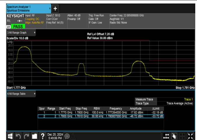
Band66-3MHz-16QAM-132657-1RB#0-PASS
