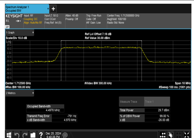
Band66-5MHz-16QAM-131997-25RB#0-PASS
