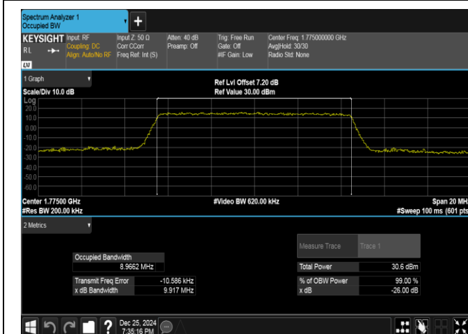
Band66-10MHz-QPSK-132622-50RB#0-PASS
