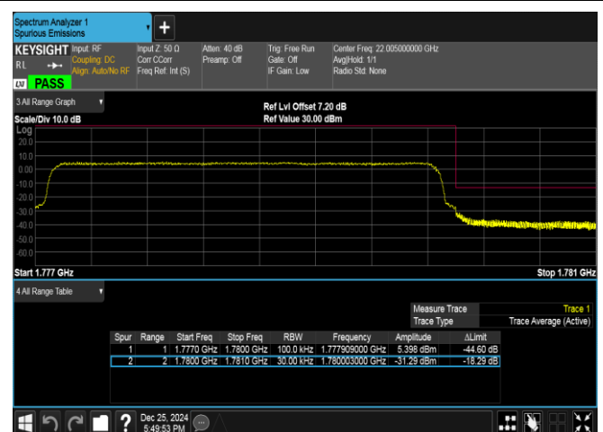
Band66-3MHz-QPSK-132657-15RB#0-PASS
