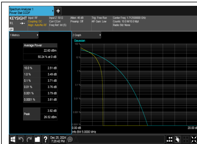
Band66-5MHz-QPSK-131997-1RB#0-PASS
