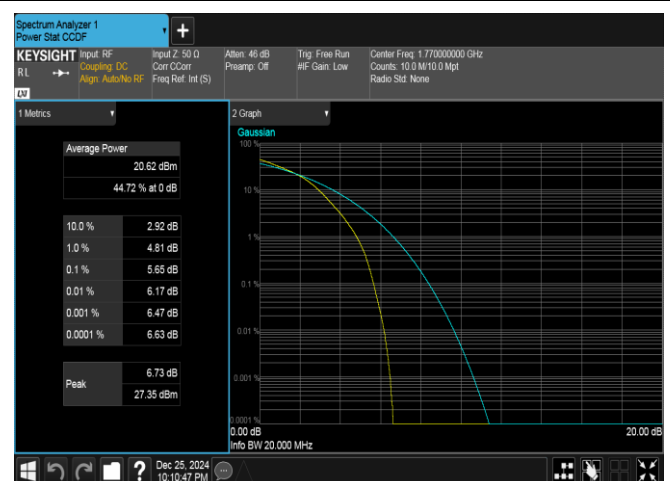
Band66-20MHz-16QAM-132572-100RB#0-PASS
