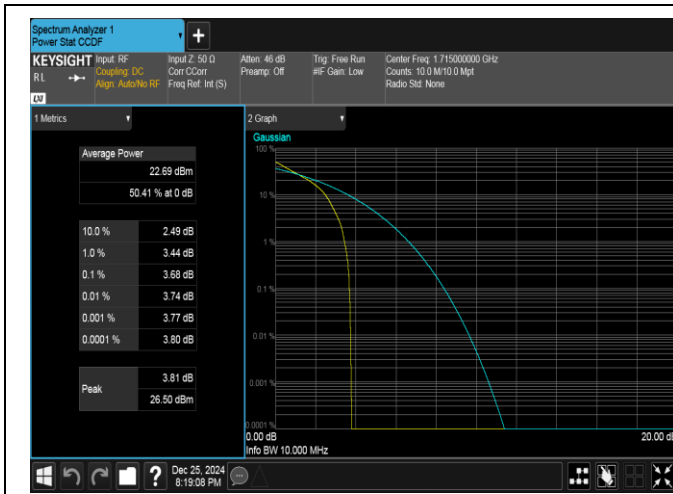
Band66-10MHz-QPSK-132022-1RB#0-PASS
