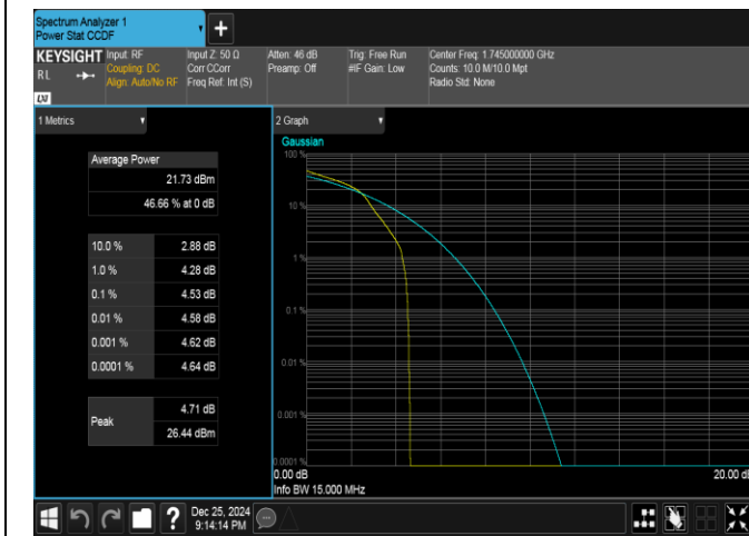
Band66-15MHz-16QAM-132322-1RB#0-PASS
