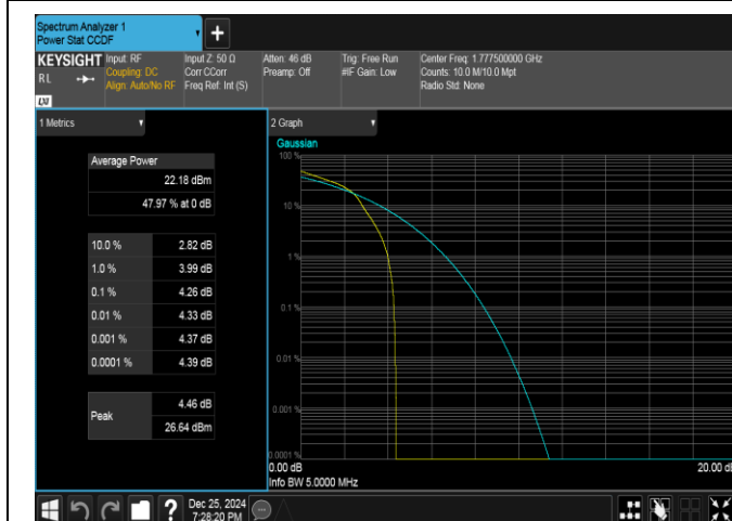
Band66-5MHz-16QAM-132647-1RB#0-PASS
