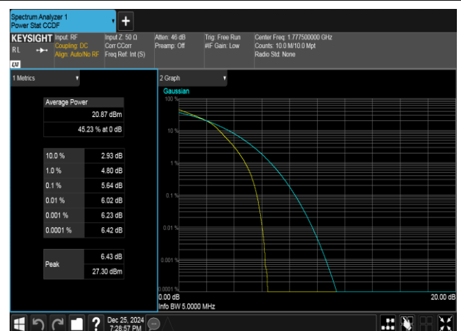
Band66-5MHz-16QAM-132647-25RB#0-PASS
