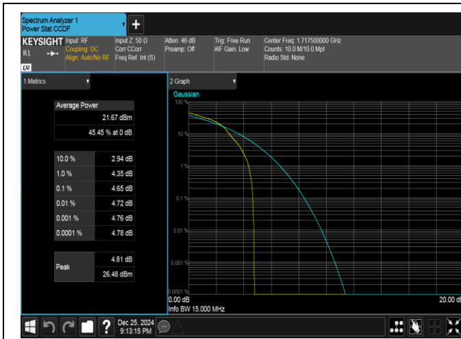
Band66-15MHz-16QAM-132047-1RB#0-PASS
