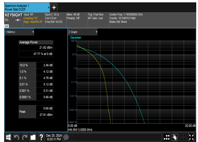
Band66-3MHz-QPSK-132322-15RB#0-PASS
