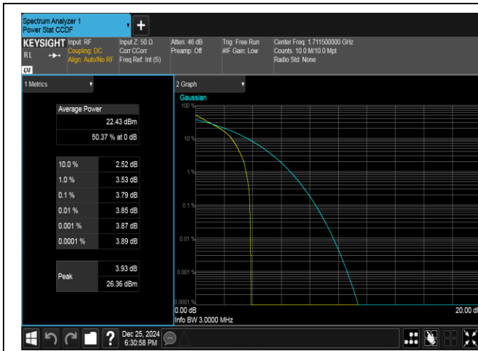
Band66-3MHz-QPSK-131987-1RB#0-PASS
