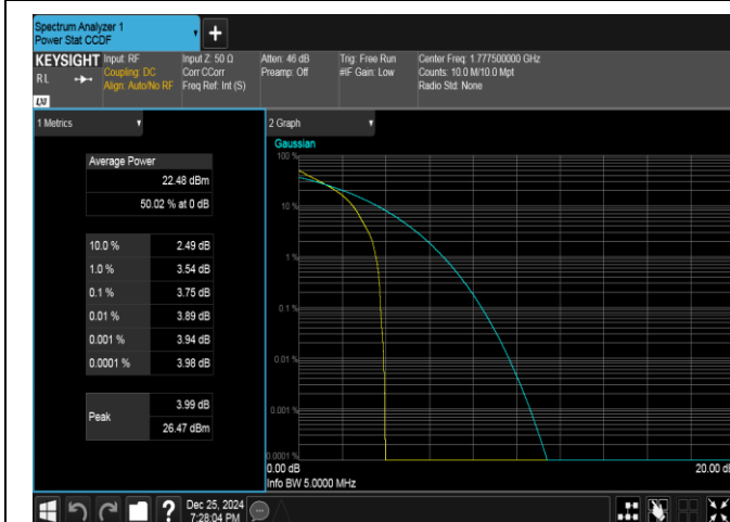
Band66-5MHz-QPSK-132647-1RB#0-PASS
