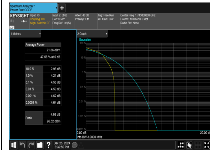
Band66-3MHz-16QAM-132322-1RB#0-PASS
