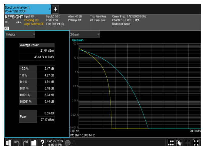
Band66-15MHz-QPSK-132597-75RB#0-PASS
