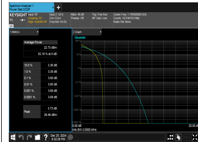
Band66-3MHz-QPSK-132322-1RB#0-PASS
