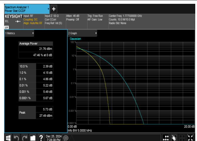
Band66-5MHz-QPSK-132647-25RB#0-PASS
