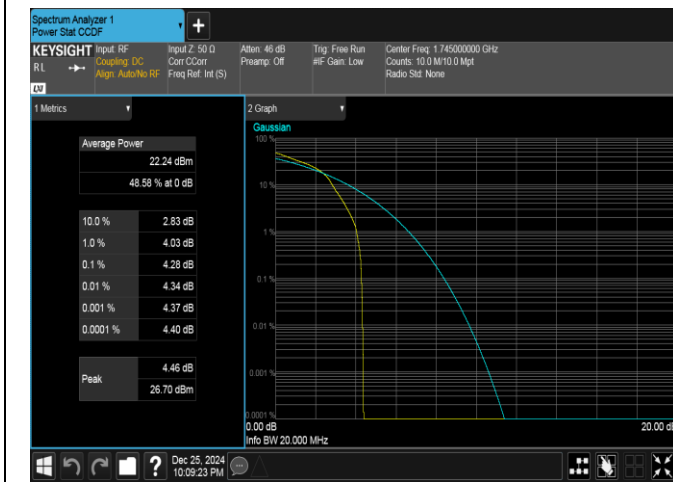
Band66-20MHz-16QAM-132322-1RB#0-PASS
