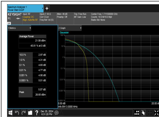
Band66-3MHz-16QAM-131987-1RB#0-PASS
