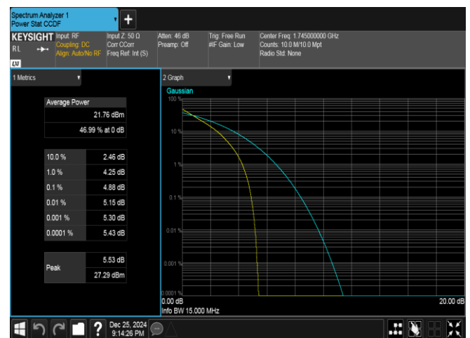
Band66-15MHz-QPSK-132322-75RB#0-PASS
