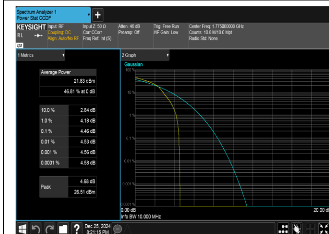
Band66-10MHz-16QAM-132622-1RB#0-PASS
