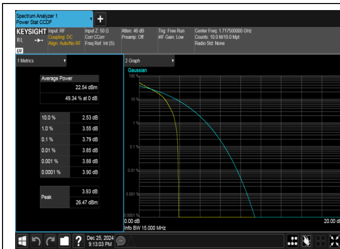
Band66-15MHz-QPSK-132047-1RB#0-PASS
