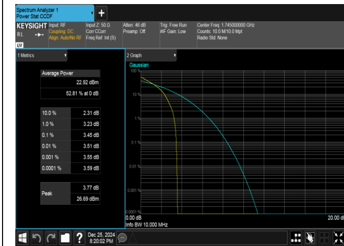
Band66-10MHz-QPSK-132322-1RB#0-PASS
