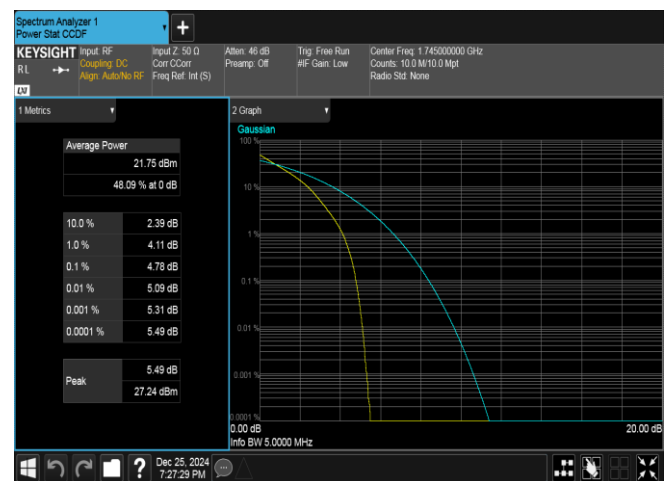
Band66-5MHz-QPSK-132322-25RB#0-PASS
