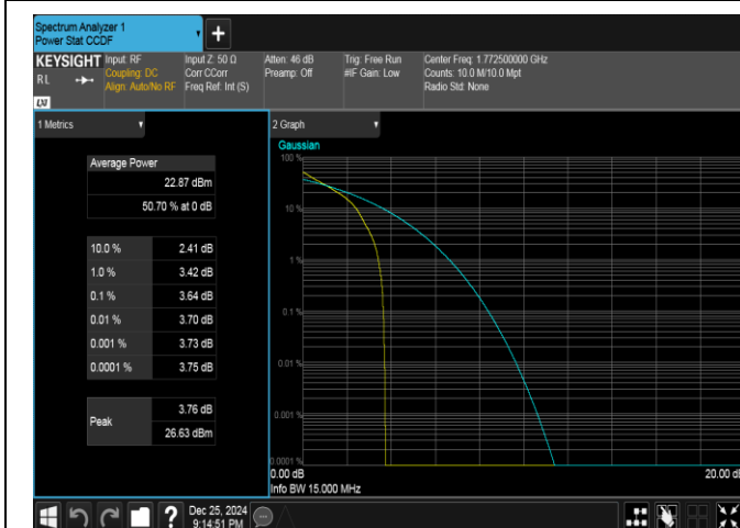
Band66-15MHz-QPSK-132597-1RB#0-PASS
