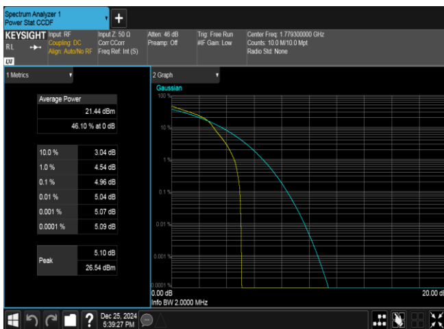
Band66-1.4MHz-16QAM-132665-1RB#0-PASS
