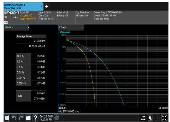
Band66-10MHz-QPSK-132322-50RB#0-PASS
