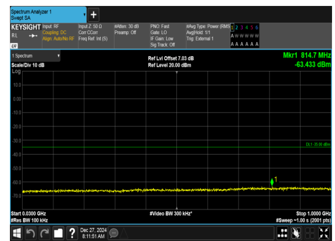
Band41-20MHz-16QAM-39750-1RB#0-30~1000-PASS
