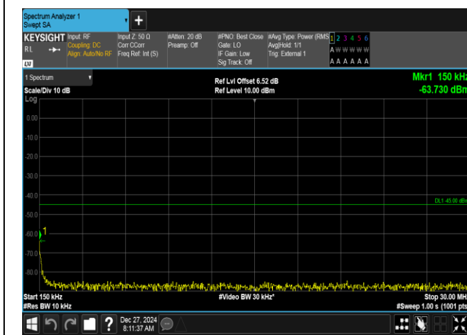
Band41-20MHz-16QAM-39750-1RB#0-0.15~30-PASS
