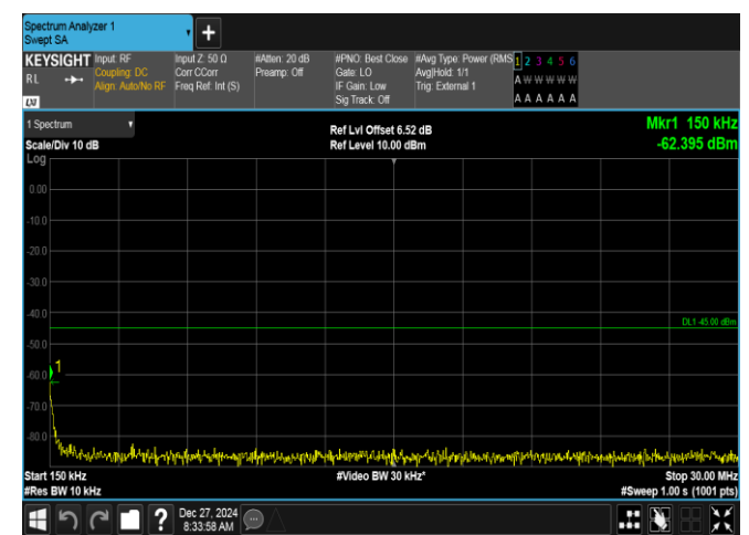
Band41-20MHz-QPSK-41490-100RB#0-0.15~30-PASS
