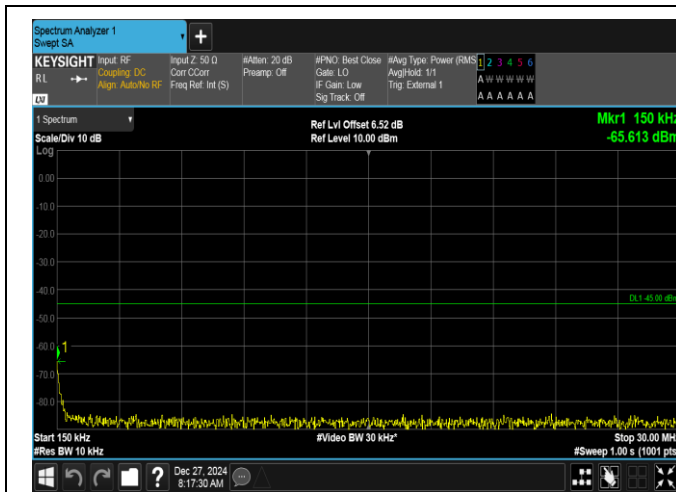
Band41-20MHz-16QAM-39750-100RB#0-0.15~30-PASS
