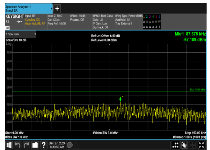
Band41-20MHz-QPSK-41490-1RB#99-0.009~0.15-PASS
