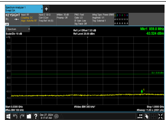
Band41-20MHz-16QAM-39750-100RB#0-30~1000-PASS
