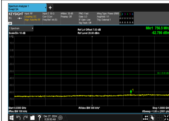
Band41-20MHz-16QAM-40620-100RB#0-30~1000-PASS
