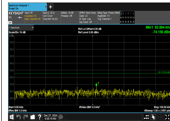
Band41-20MHz-16QAM-40620-100RB#0-0.009~0.15-PASS
