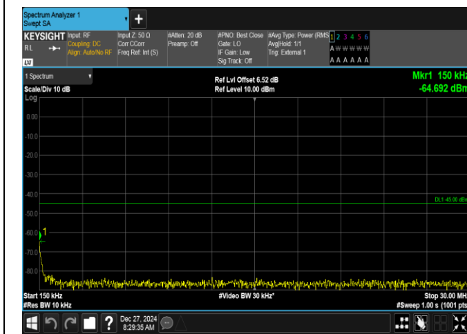
Band41-20MHz-16QAM-41490-1RB#0-0.15~30-PASS
