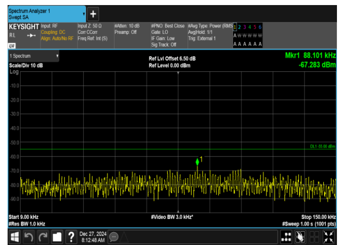
Band41-20MHz-QPSK-39750-1RB#99-0.009~0.15-PASS
