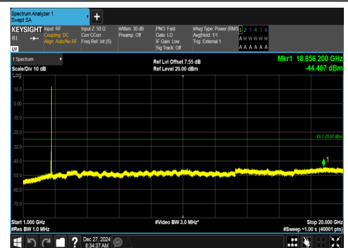
Band41-20MHz-QPSK-41490-100RB#0-1000~20000-PASS
