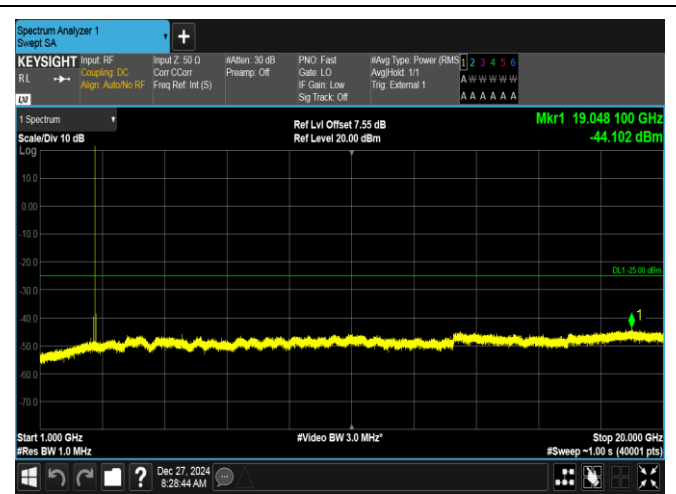
Band41-20MHz-QPSK-41490-1RB#0-1000~20000-PASS
