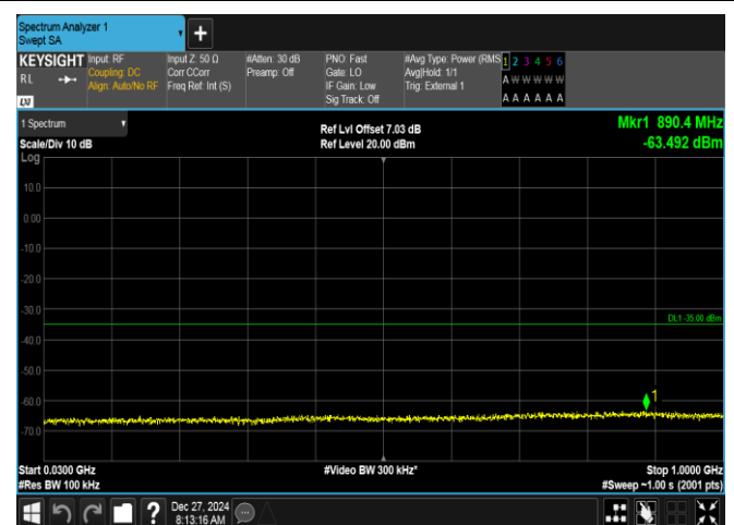
Band41-20MHz-QPSK-39750-1RB#99-30~1000-PASS
