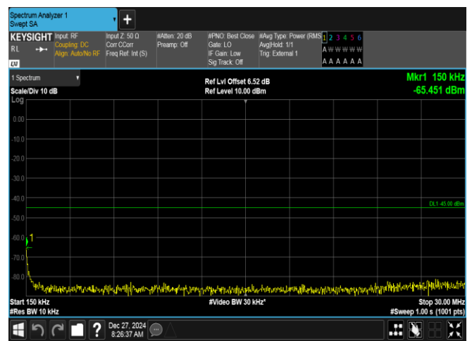
Band41-20MHz-16QAM-40620-100RB#0-0.15~30-PASS
