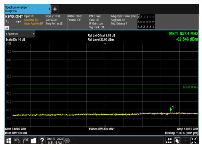
Band41-20MHz-QPSK-41490-1RB#99-30~1000-PASS
