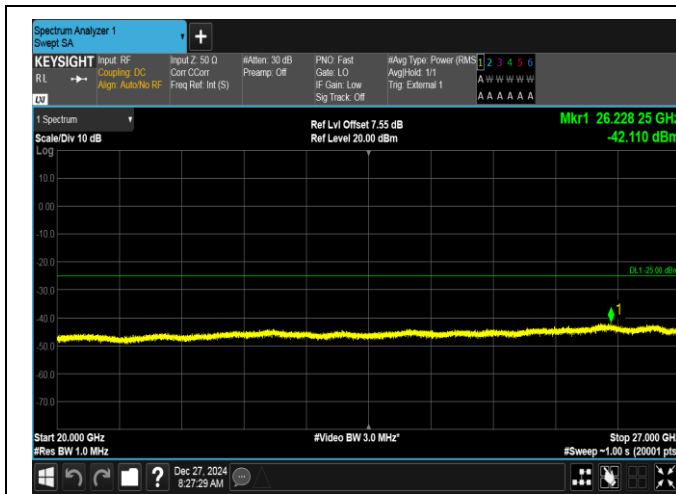
Band41-20MHz-16QAM-40620-100RB#0-20000~27000-PASS
