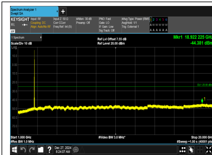
Band41-20MHz-16QAM-40620-1RB#99-1000~20000-PASS
