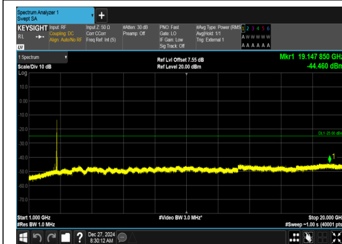
Band41-20MHz-16QAM-41490-1RB#0-1000~20000-PASS
