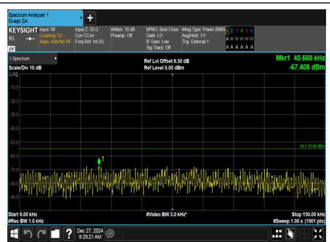
Band41-20MHz-16QAM-41490-1RB#0-0.009~0.15-PASS
