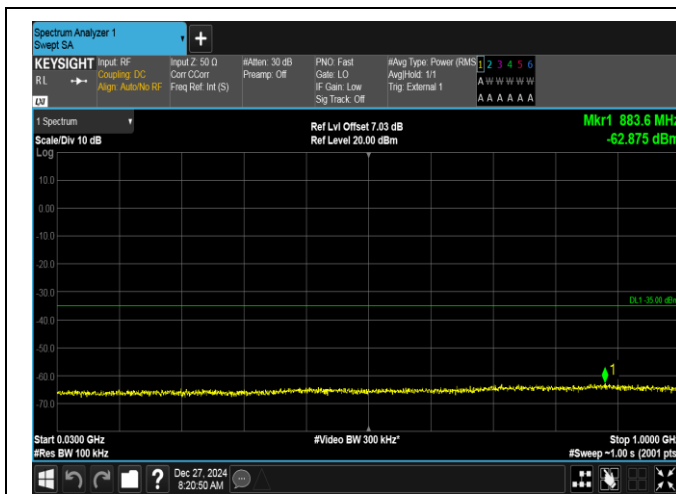
Band41-20MHz-16QAM-40620-1RB#0-30~1000-PASS
