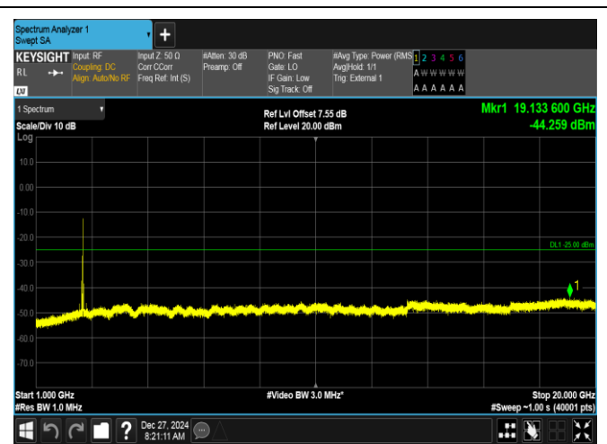
Band41-20MHz-16QAM-40620-1RB#0-1000~20000-PASS
