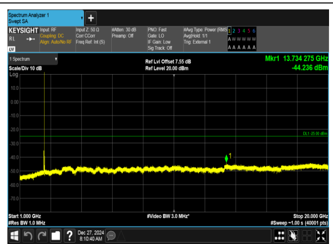
Band41-20MHz-QPSK-39750-1RB#0-1000~20000-PASS
