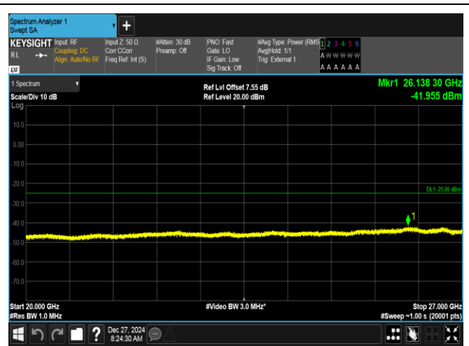
Band41-20MHz-16QAM-40620-1RB#99-20000~27000-PASS
