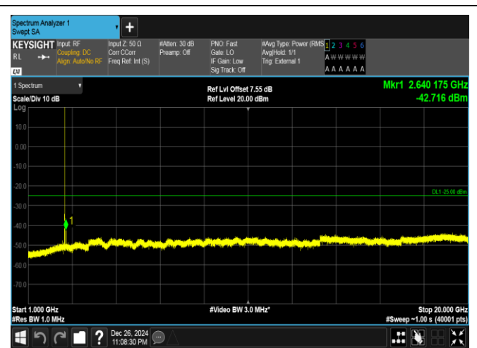
Band41-15MHz-16QAM-40620-1RB#0-1000~20000-PASS
