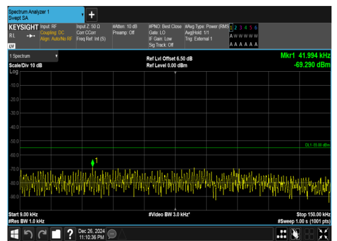
Band41-15MHz-16QAM-40620-1RB#74-0.009~0.15-PASS
