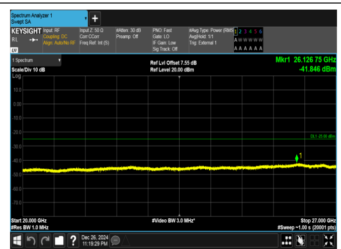
Band41-15MHz-QPSK-41515-1RB#74-20000~27000-PASS
