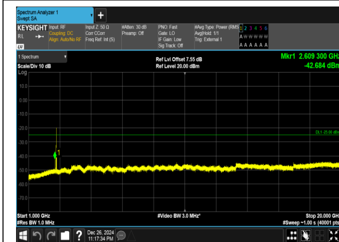
Band41-15MHz-16QAM-41515-1RB#0-1000~20000-PASS
