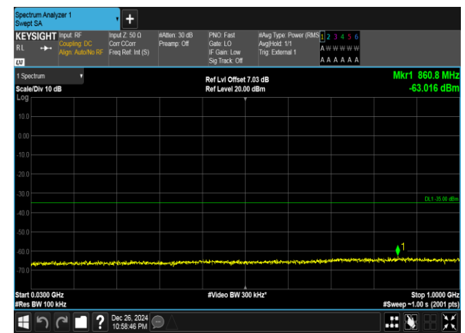
Band41-15MHz-16QAM-39725-1RB#0-30~1000-PASS
