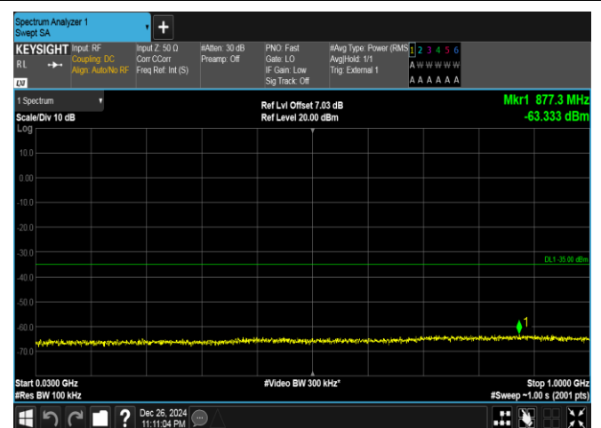
Band41-15MHz-16QAM-40620-1RB#74-30~1000-PASS
