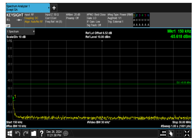
Band41-15MHz-QPSK-41515-75RB#0-0.15~30-PASS
