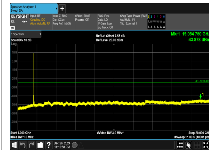
Band41-15MHz-QPSK-40620-75RB#0-1000~20000-PASS
