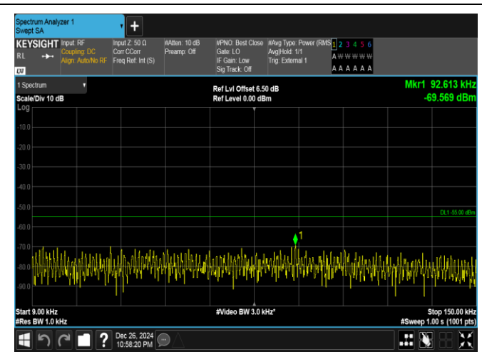
Band41-15MHz-16QAM-39725-1RB#0-0.009~0.15-PASS
