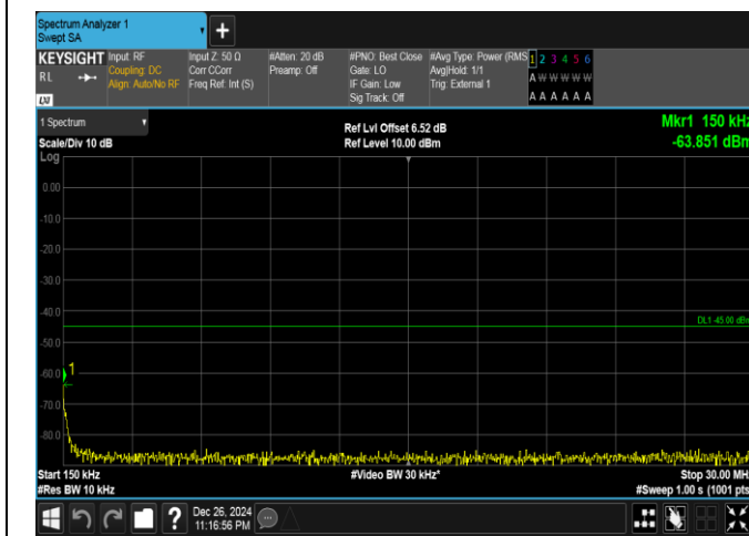
Band41-15MHz-16QAM-41515-1RB#0-0.15~30-PASS
