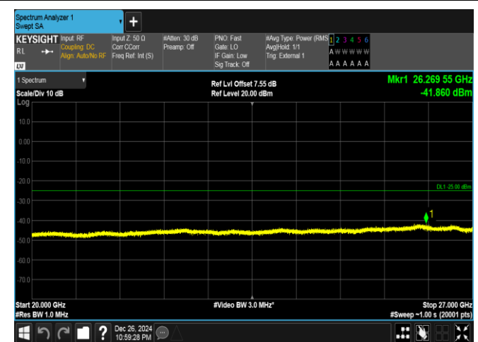
Band41-15MHz-16QAM-39725-1RB#0-20000~27000-PASS
