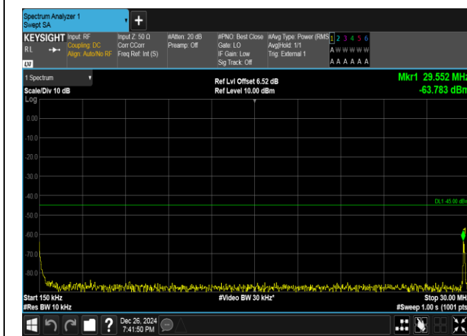
Band41-5MHz-QPSK-40620-1RB#0-0.15~30-PASS
