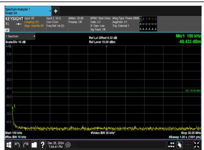
Band41-5MHz-QPSK-40620-1RB#24-0.15~30-PASS
