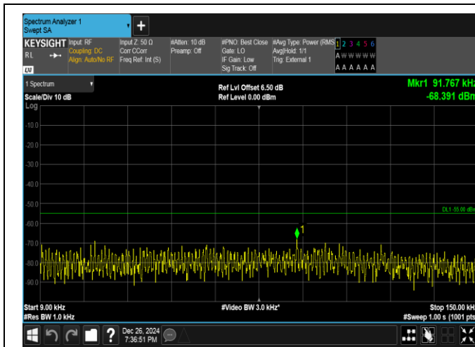
Band41-5MHz-16QAM-39675-1RB#24-0.009~0.15-PASS
