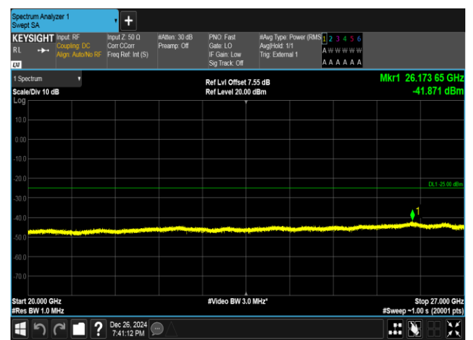
Band41-5MHz-16QAM-39675-25RB#0-20000~27000-PASS
