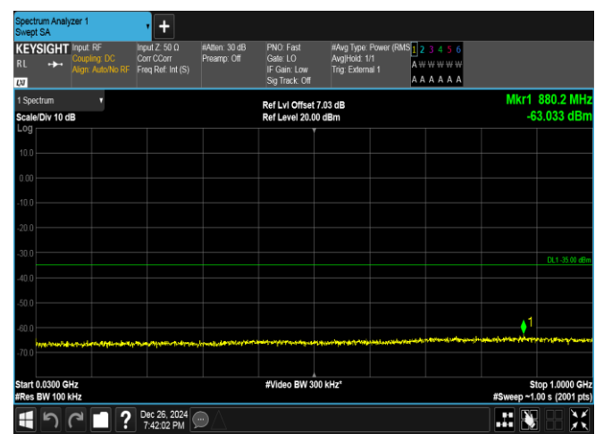
Band41-5MHz-QPSK-40620-1RB#0-30~1000-PASS
