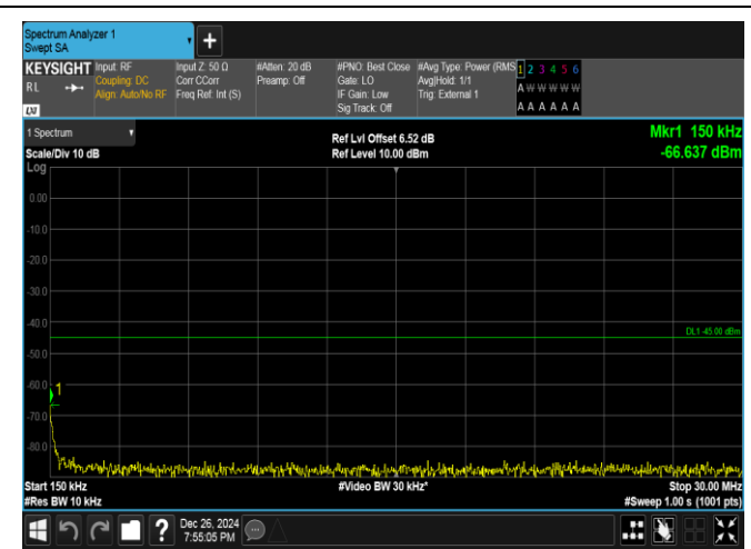
Band41-5MHz-16QAM-41565-1RB#24-0.15~30-PASS
