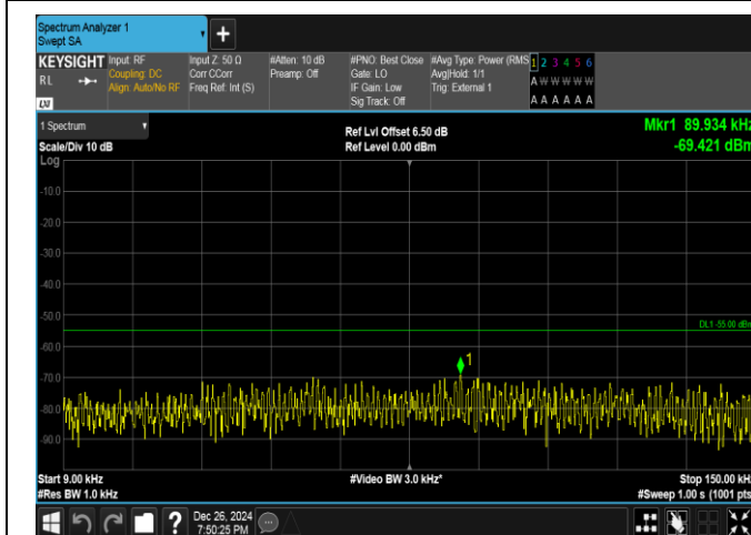
Band41-5MHz-QPSK-41565-1RB#0-0.009~0.15-PASS
