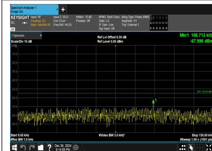
Band41-10MHz-QPSK-39700-1RB#0-0.009~0.15-PASS
