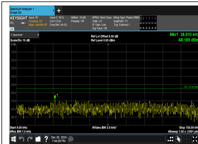
Band41-5MHz-QPSK-40620-1RB#24-0.009~0.15-PASS
