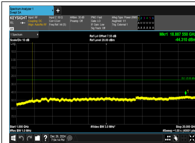
Band41-5MHz-QPSK-41565-1RB#24-1000~20000-PASS
