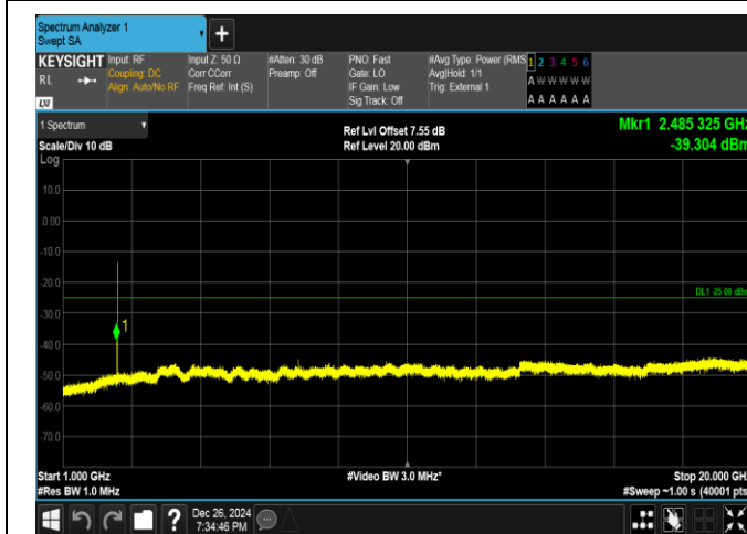
Band41-5MHz-16QAM-39675-1RB#0-1000~20000-PASS
