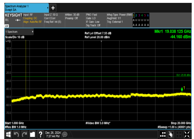
Band41-5MHz-16QAM-39675-1RB#24-1000~20000-PASS
