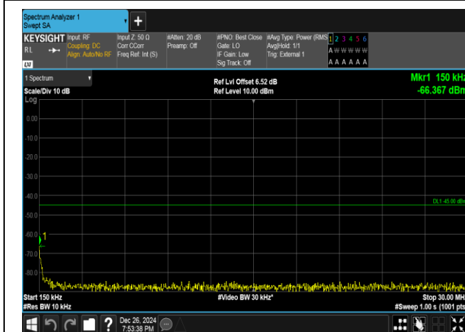
Band41-5MHz-QPSK-41565-1RB#24-0.15~30-PASS
