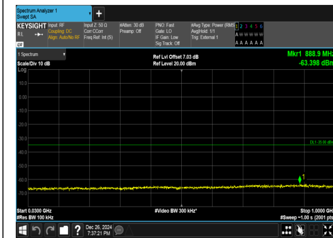
Band41-5MHz-16QAM-39675-1RB#24-30~1000-PASS
