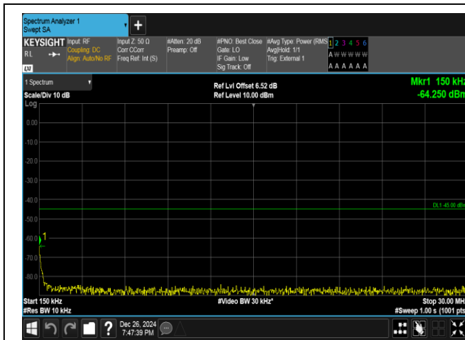
Band41-5MHz-QPSK-40620-25RB#0-0.15~30-PASS
