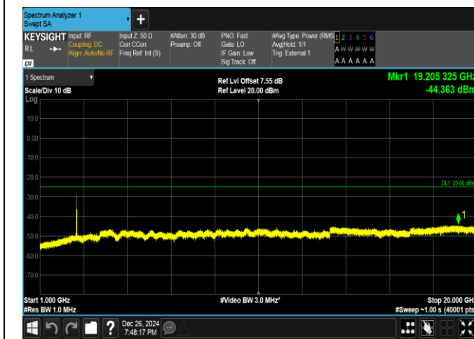
Band41-5MHz-QPSK-40620-25RB#0-1000~20000-PASS
