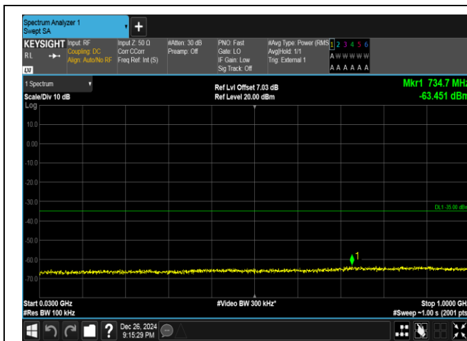
Band41-10MHz-QPSK-39700-1RB#0-30~1000-PASS
