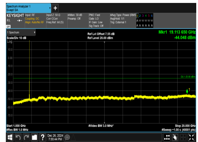
Band41-5MHz-16QAM-41565-1RB#24-1000~20000-PASS
