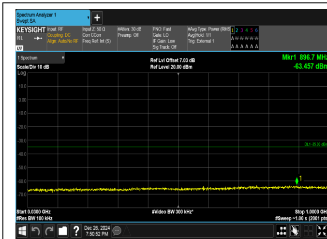
Band41-5MHz-QPSK-41565-1RB#0-30~1000-PASS
