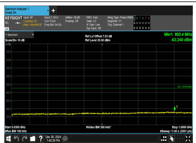
Band41-5MHz-16QAM-39675-25RB#0-30~1000-PASS
