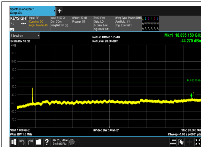
Band41-5MHz-16QAM-40620-1RB#24-1000~20000-PASS
