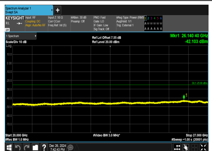
Band41-5MHz-QPSK-40620-1RB#0-20000~27000-PASS
