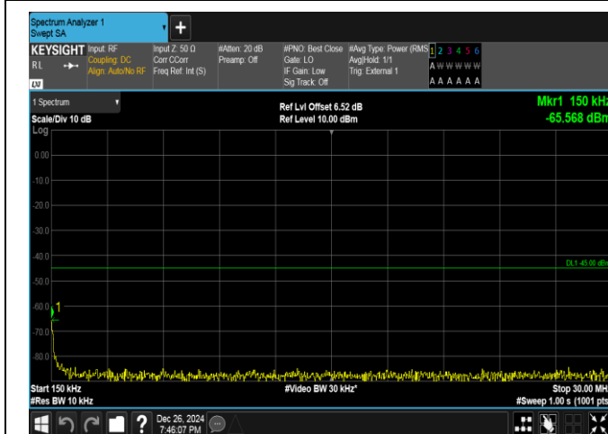
Band41-5MHz-16QAM-40620-1RB#24-0.15~30-PASS
