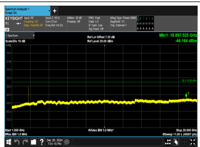
Band41-5MHz-QPSK-41565-1RB#0-1000~20000-PASS
