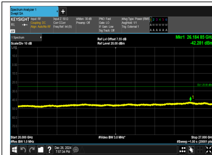
Band41-5MHz-QPSK-41565-25RB#0-20000~27000-PASS
