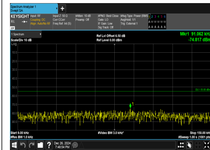
Band41-5MHz-16QAM-40620-25RB#0-0.009~0.15-PASS
