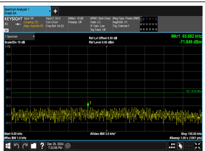
Band41-5MHz-16QAM-39675-1RB#0-0.009~0.15-PASS
