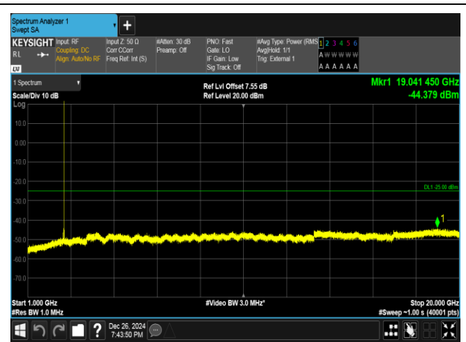
Band41-5MHz-16QAM-40620-1RB#0-1000~20000-PASS
