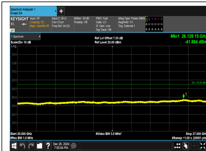
Band41-5MHz-16QAM-40620-25RB#0-20000~27000-PASS
