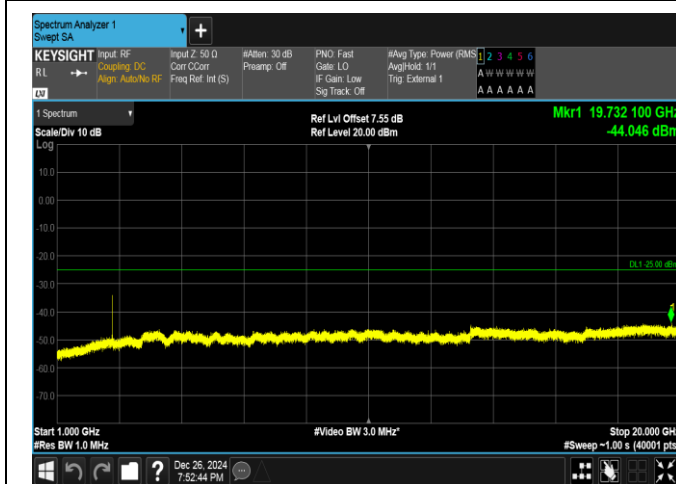
Band41-5MHz-16QAM-41565-1RB#0-1000~20000-PASS
