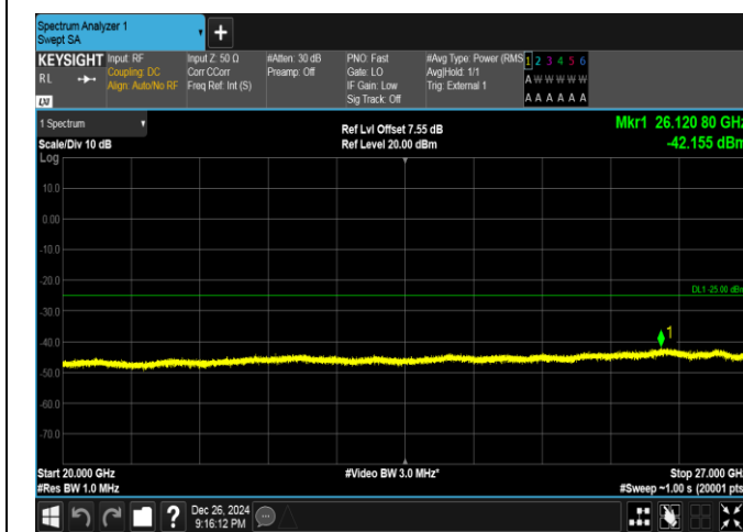
Band41-10MHz-QPSK-39700-1RB#0-20000~27000-PASS
