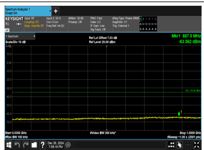
Band41-5MHz-16QAM-41565-25RB#0-30~1000-PASS
