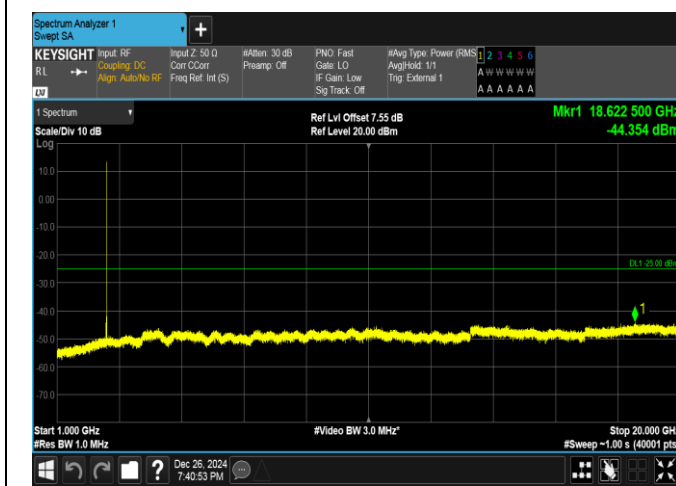
Band41-5MHz-16QAM-39675-25RB#0-1000~20000-PASS
