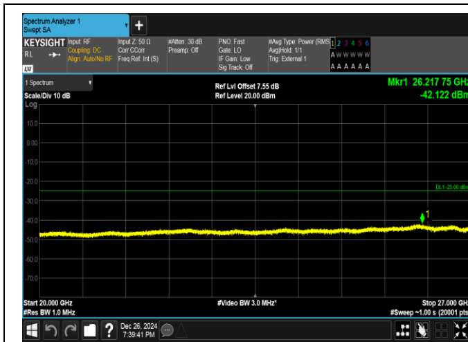
Band41-5MHz-QPSK-39675-25RB#0-20000~27000-PASS
