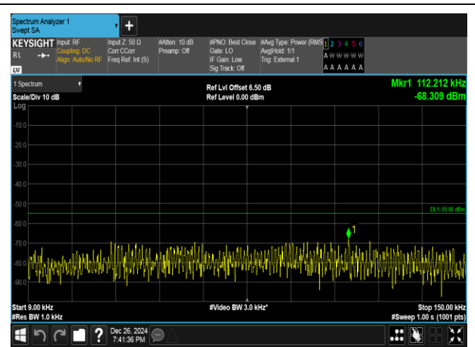
Band41-5MHz-QPSK-40620-1RB#0-0.009~0.15-PASS
