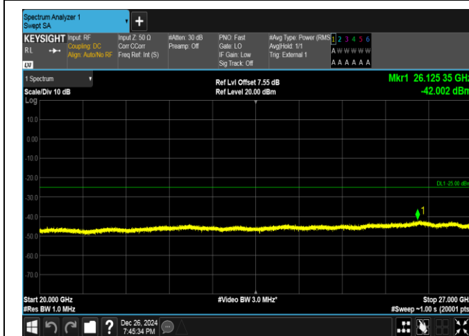
Band41-5MHz-QPSK-40620-1RB#24-20000~27000-PASS
