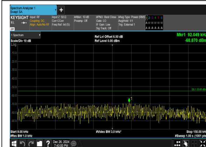
Band41-5MHz-16QAM-40620-1RB#0-0.009~0.15-PASS
