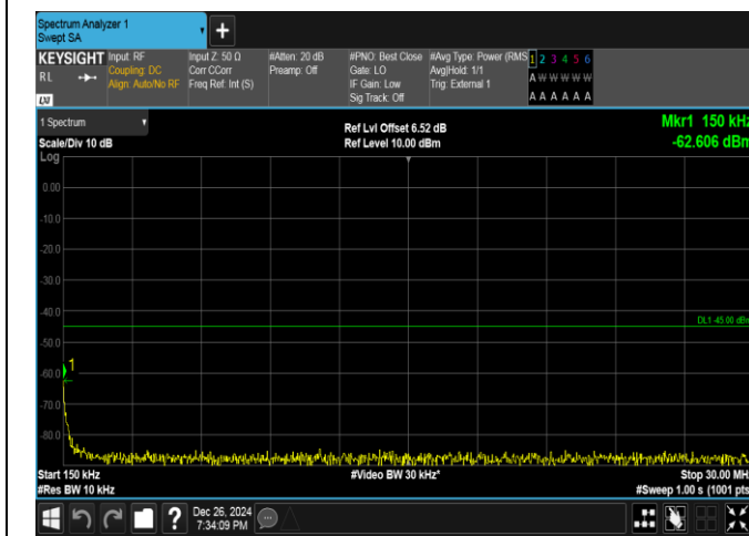
Band41-5MHz-16QAM-39675-1RB#0-0.15~30-PASS
