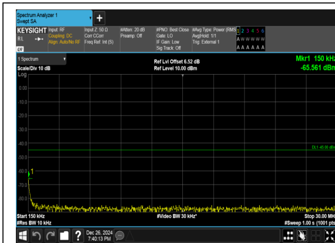
Band41-5MHz-16QAM-39675-25RB#0-0.15~30-PASS
