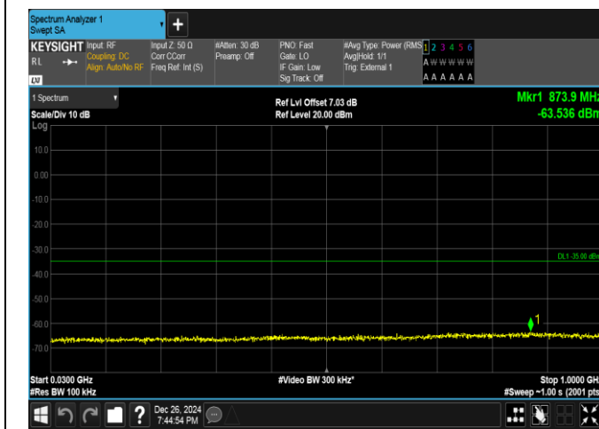
Band41-5MHz-QPSK-40620-1RB#24-30~1000-PASS
