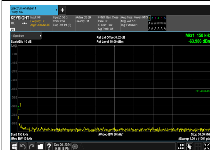
Band41-10MHz-QPSK-39700-1RB#49-0.15~30-PASS
