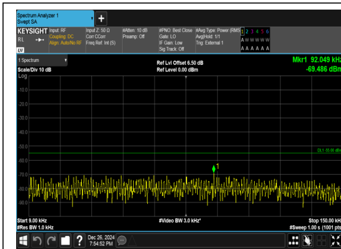
Band41-5MHz-16QAM-41565-1RB#24-0.009~0.15-PASS
