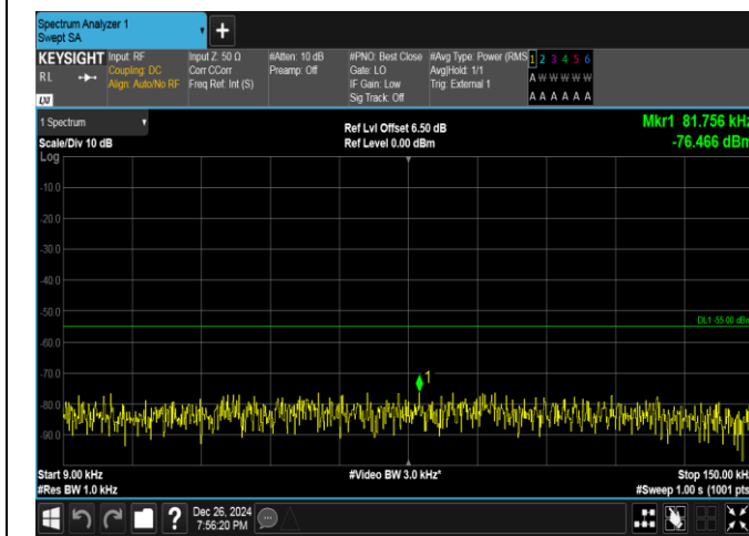
Band41-5MHz-QPSK-41565-25RB#0-0.009~0.15-PASS
