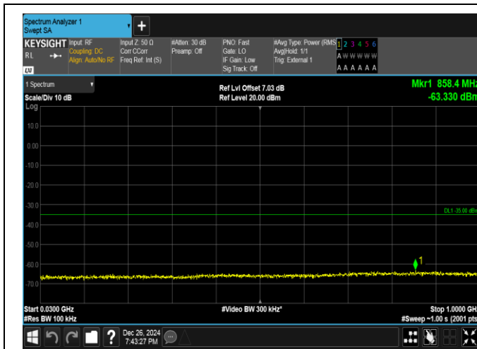
Band41-5MHz-16QAM-40620-1RB#0-30~1000-PASS
