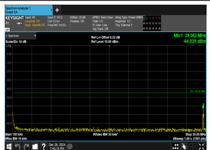
Band41-5MHz-16QAM-40620-1RB#0-0.15~30-PASS
