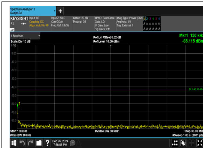
Band41-5MHz-16QAM-41565-25RB#0-0.15~30-PASS
