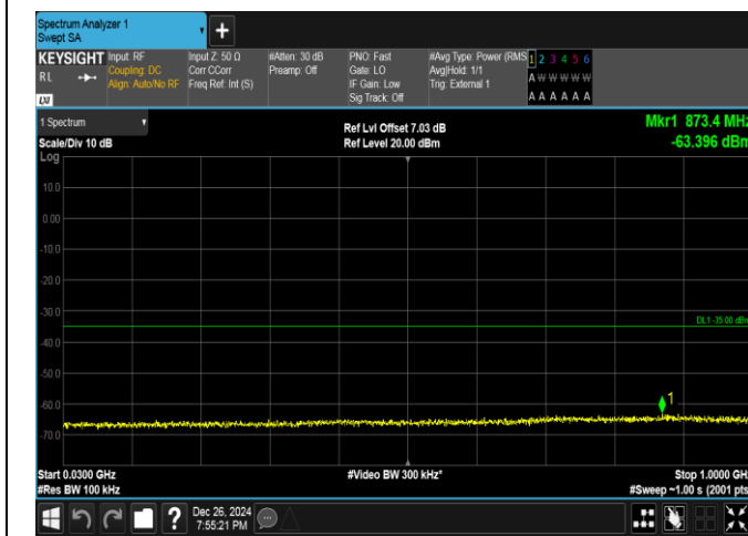
Band41-5MHz-16QAM-41565-1RB#24-30~1000-PASS
