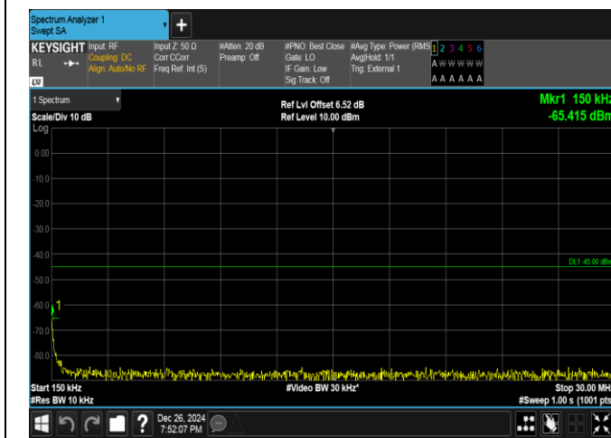
Band41-5MHz-16QAM-41565-1RB#0-0.15~30-PASS
