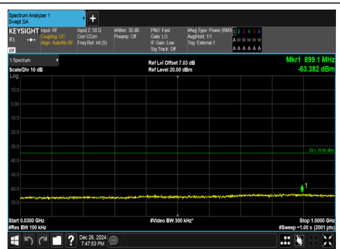
Band41-5MHz-QPSK-40620-25RB#0-30~1000-PASS
