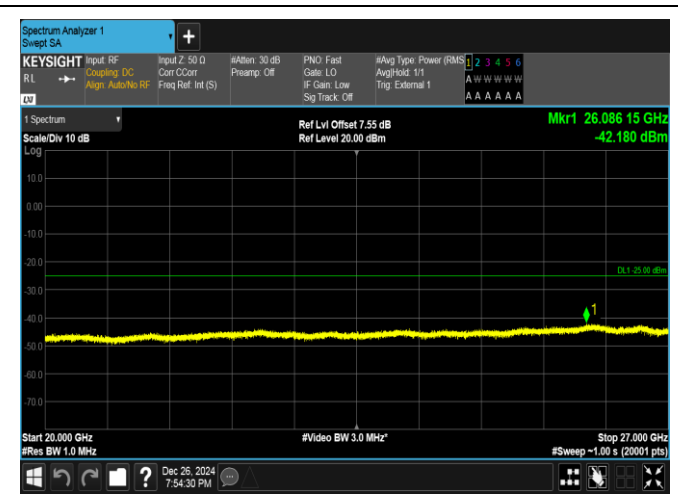
Band41-5MHz-QPSK-41565-1RB#24-20000~27000-PASS
