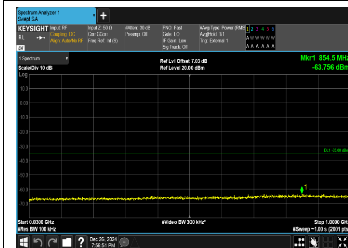
Band41-5MHz-QPSK-41565-25RB#0-30~1000-PASS
