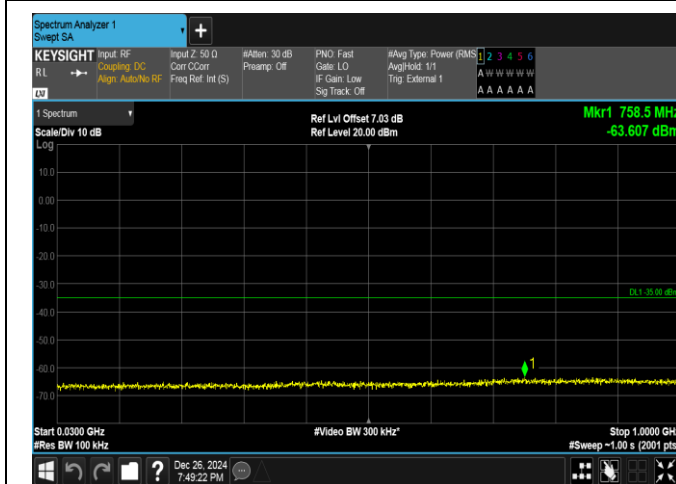
Band41-5MHz-16QAM-40620-25RB#0-30~1000-PASS
