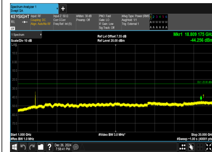
Band41-5MHz-16QAM-41565-25RB#0-1000~20000-PASS
