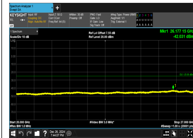
Band41-5MHz-16QAM-40620-1RB#0-20000~27000-PASS
