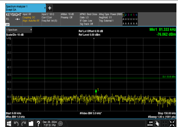
Band41-5MHz-16QAM-41565-25RB#0-0.009~0.15-PASS
