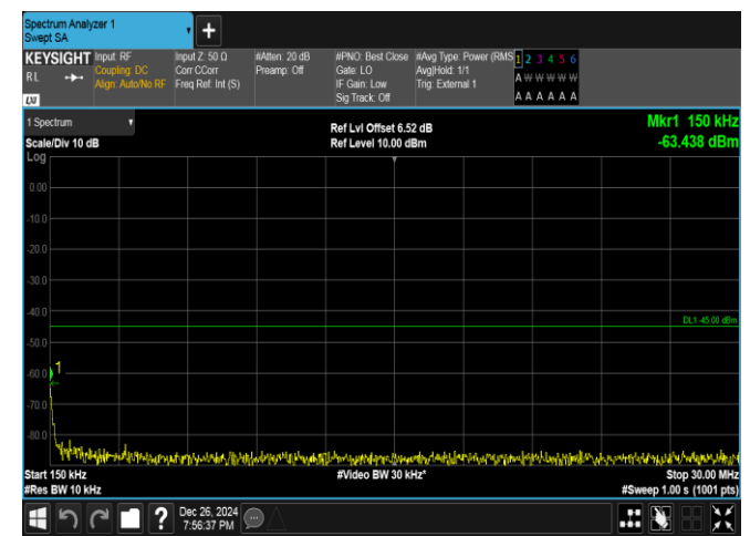
Band41-5MHz-QPSK-41565-25RB#0-0.15~30-PASS
