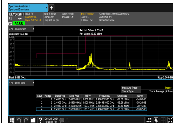
Band41-10MHz-QPSK-39700-1RB#0-PASS
