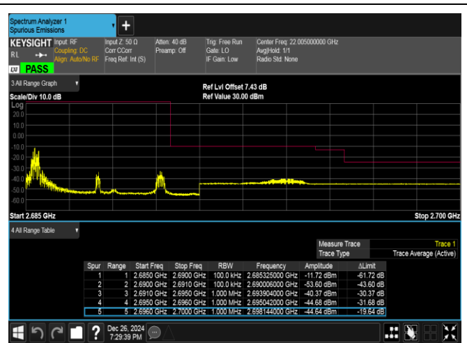
Band41-5MHz-16QAM-41565-1RB#0-PASS
