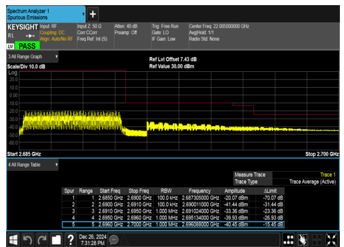
Band41-5MHz-QPSK-41565-25RB#0-PASS
