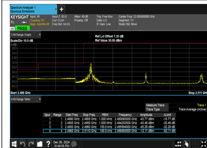
Band41-15MHz-QPSK-39725-1RB#0-PASS
