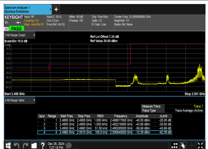
Band41-5MHz-16QAM-39675-1RB#24-PASS
