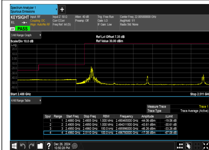
Band41-15MHz-16QAM-39725-1RB#0-PASS
