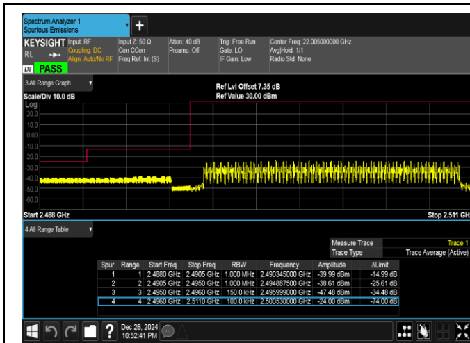
Band41-15MHz-16QAM-39725-75RB#0-PASS
