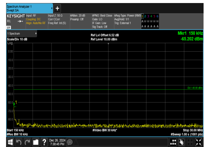
Band41-5MHz-QPSK-39675-25RB#0-0.15~30-PASS
