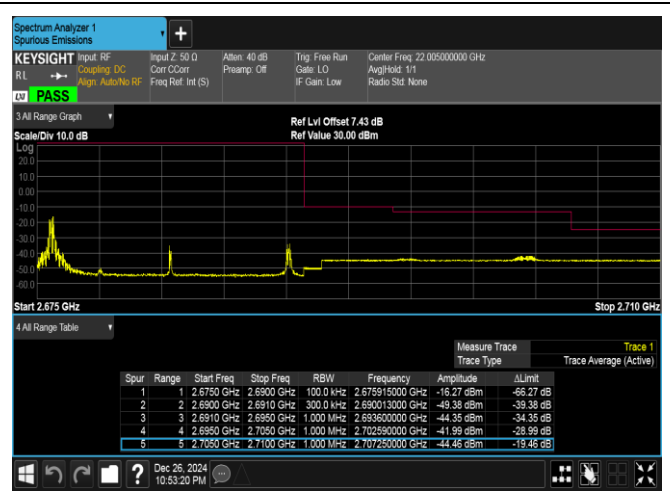
Band41-15MHz-QPSK-41515-1RB#0-PASS
