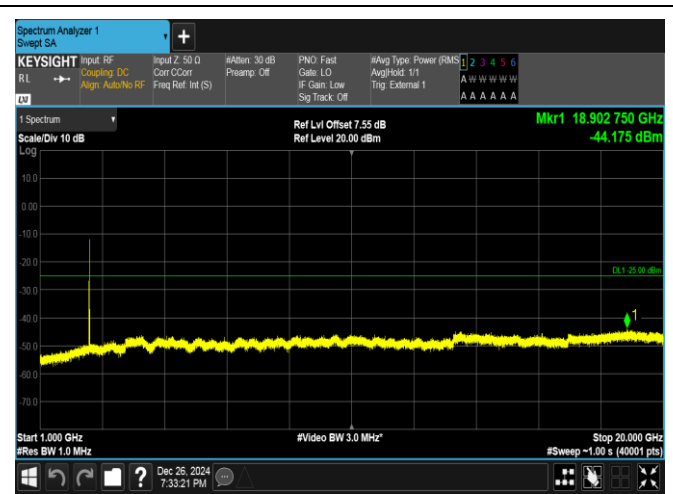
Band41-5MHz-QPSK-39675-1RB#0-1000~20000-PASS
