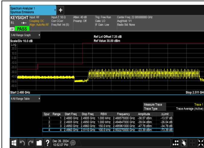
Band41-15MHz-QPSK-39725-75RB#0-PASS
