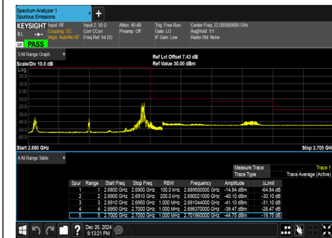
Band41-10MHz-16QAM-41540-1RB#49-PASS
