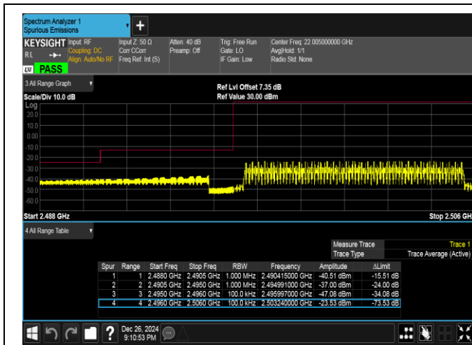
Band41-10MHz-16QAM-39700-50RB#0-PASS
