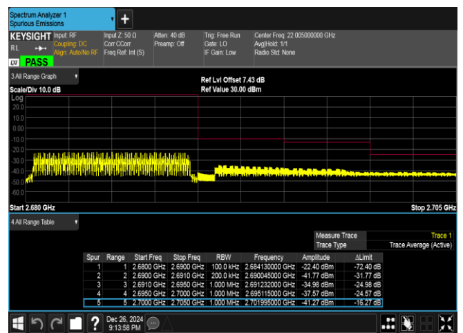
Band41-10MHz-QPSK-41540-50RB#0-PASS
