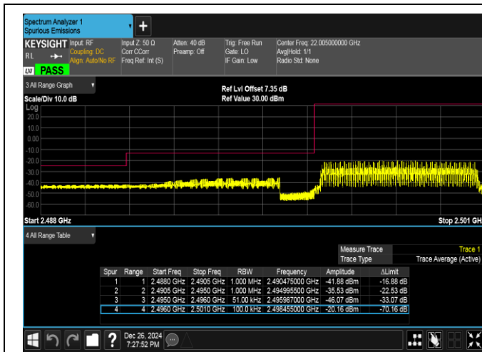
Band41-5MHz-QPSK-39675-25RB#0-PASS
