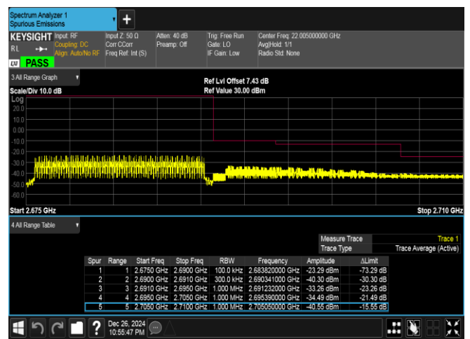
Band41-15MHz-QPSK-41515-75RB#0-PASS
