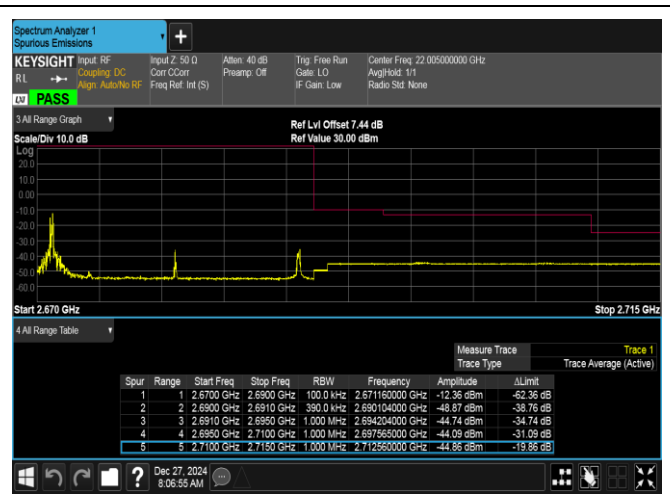
Band41-20MHz-16QAM-41490-1RB#0-PASS
