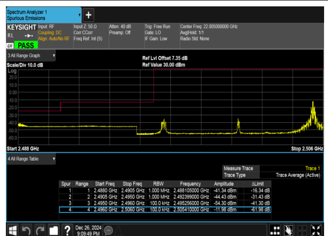
Band41-10MHz-16QAM-39700-1RB#49-PASS
