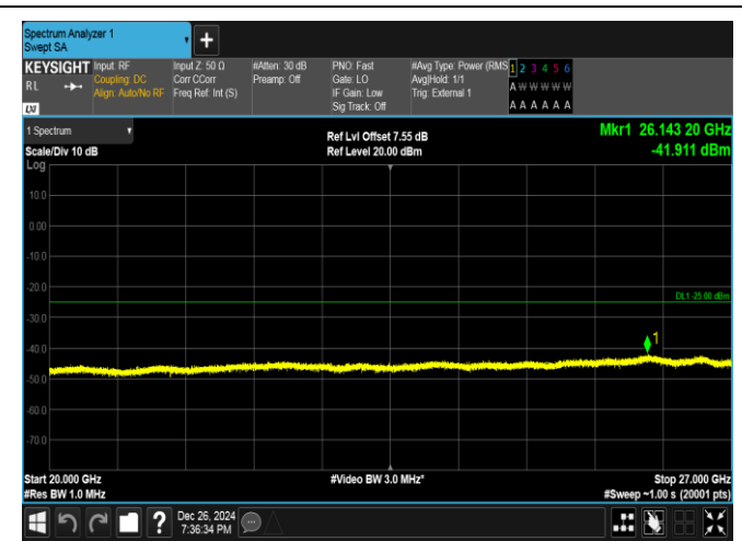
Band41-5MHz-QPSK-39675-1RB#24-20000~27000-PASS
