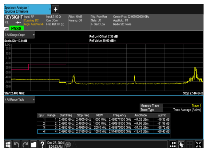
Band41-20MHz-16QAM-39750-1RB#99-PASS
