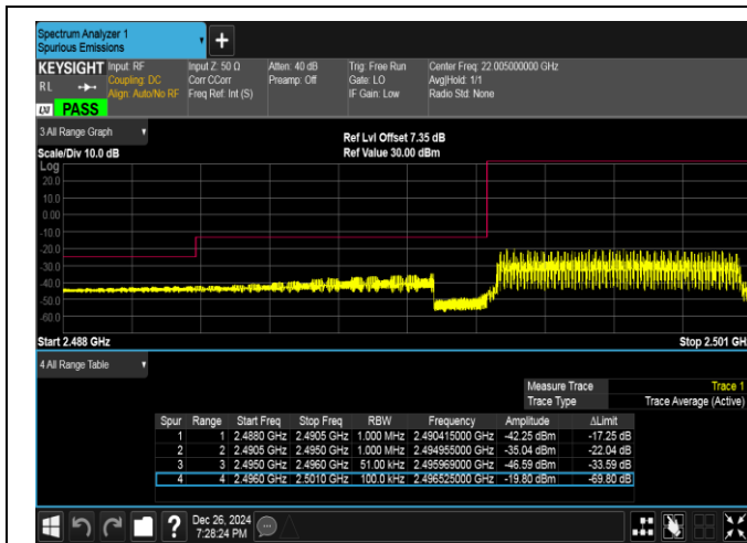
Band41-5MHz-16QAM-39675-25RB#0-PASS
