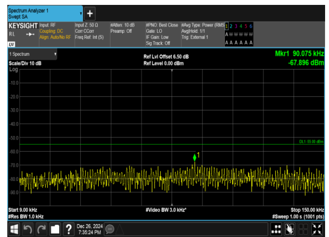
Band41-5MHz-QPSK-39675-1RB#24-0.009~0.15-PASS
