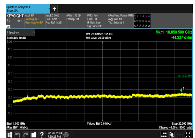
Band41-5MHz-QPSK-39675-25RB#0-1000~20000-PASS
