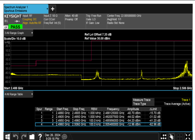
Band41-10MHz-QPSK-39700-1RB#49-PASS
