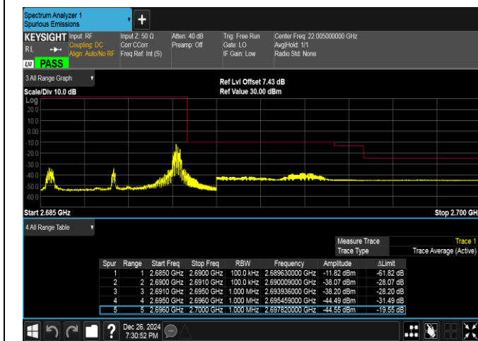
Band41-5MHz-16QAM-41565-1RB#24-PASS
