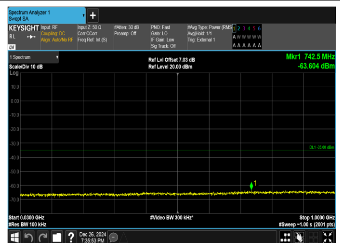
Band41-5MHz-QPSK-39675-1RB#24-30~1000-PASS
