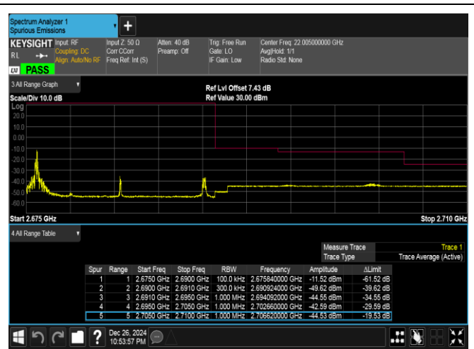
Band41-15MHz-16QAM-41515-1RB#0-PASS
