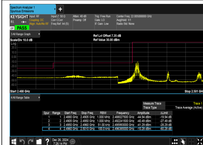
Band41-5MHz-16QAM-39675-1RB#0-PASS
