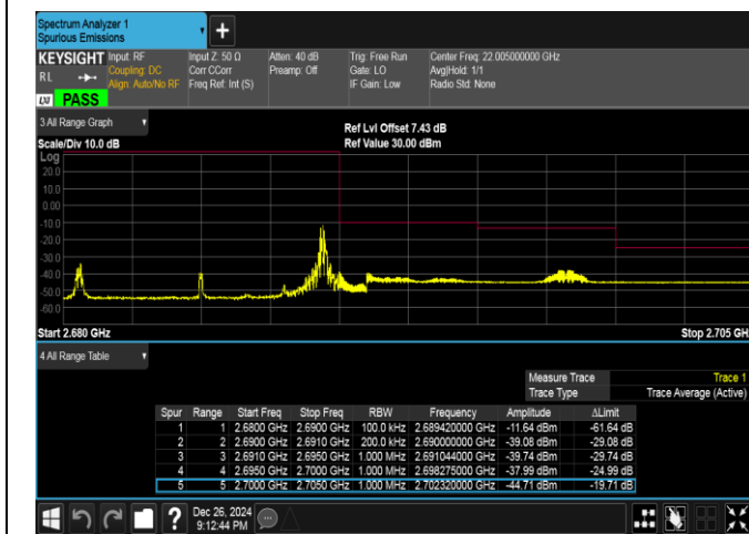
Band41-10MHz-QPSK-41540-1RB#49-PASS
