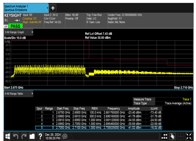
Band41-15MHz-16QAM-41515-75RB#0-PASS
