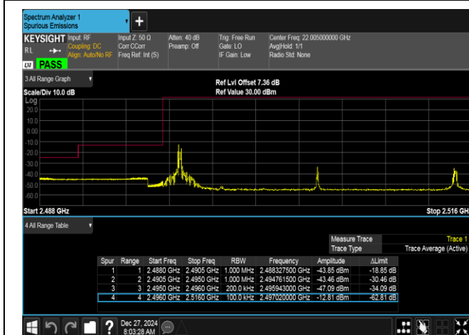
Band41-20MHz-16QAM-39750-1RB#0-PASS
