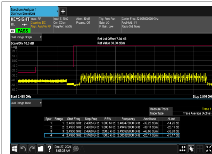
Band41-20MHz-16QAM-39750-100RB#0-PASS
