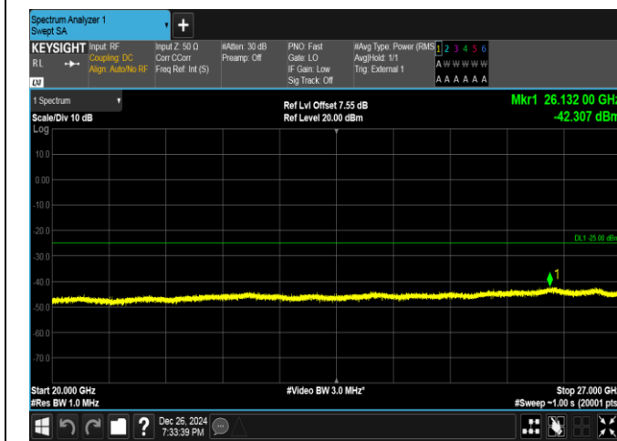
Band41-5MHz-QPSK-39675-1RB#0-20000~27000-PASS
