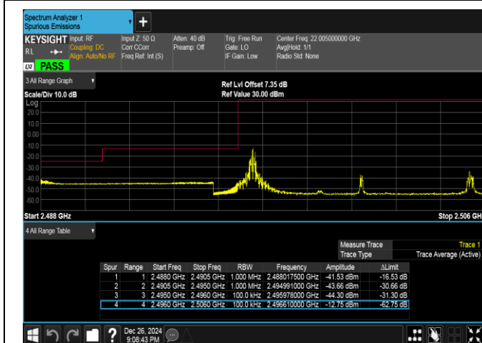
Band41-10MHz-16QAM-39700-1RB#0-PASS
