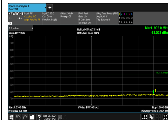
Band41-5MHz-QPSK-39675-25RB#0-30~1000-PASS
