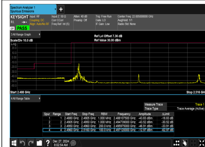
Band41-20MHz-QPSK-39750-1RB#0-PASS
