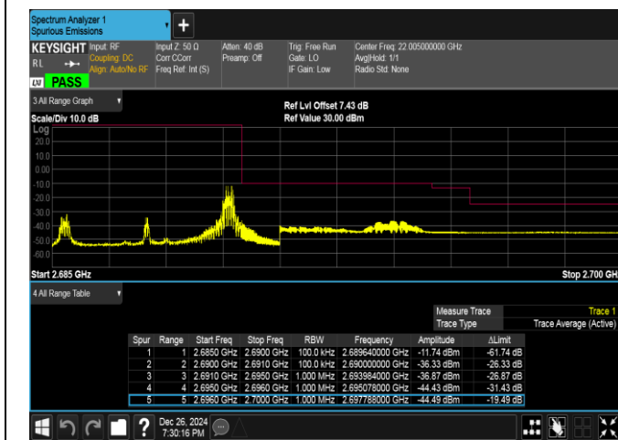
Band41-5MHz-QPSK-41565-1RB#24-PASS
