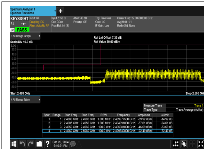
Band41-10MHz-QPSK-39700-50RB#0-PASS
