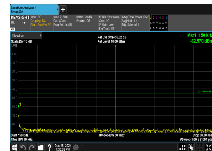
Band41-5MHz-QPSK-39675-1RB#24-0.15~30-PASS
