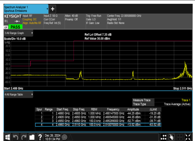
Band41-15MHz-16QAM-39725-1RB#74-PASS
