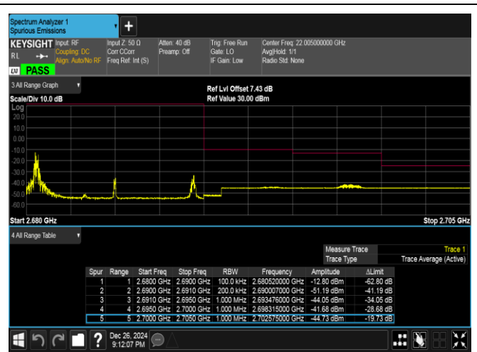
Band41-10MHz-16QAM-41540-1RB#0-PASS
