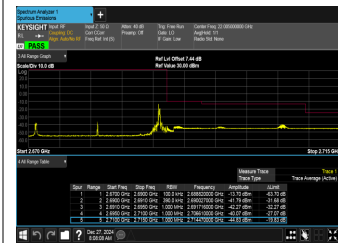
Band41-20MHz-16QAM-41490-1RB#99-PASS
