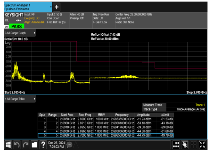
Band41-5MHz-QPSK-41565-1RB#0-PASS
