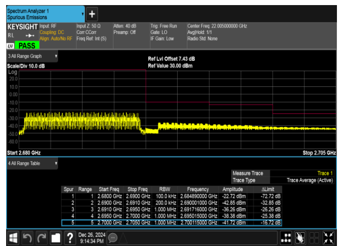
Band41-10MHz-16QAM-41540-50RB#0-PASS
