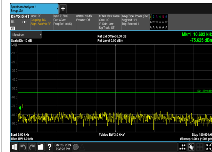
Band41-5MHz-QPSK-39675-25RB#0-0.009~0.15-PASS
