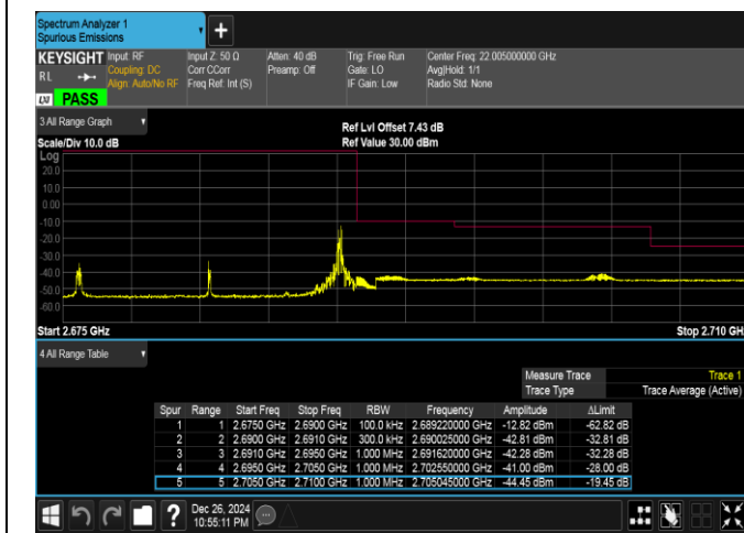
Band41-15MHz-16QAM-41515-1RB#74-PASS
