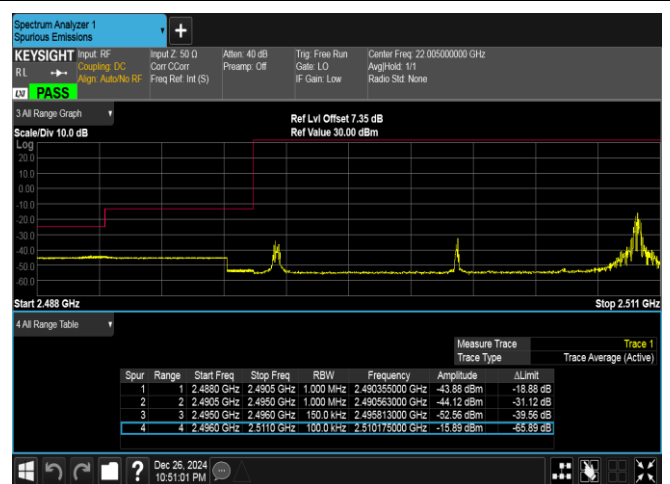
Band41-15MHz-QPSK-39725-1RB#74-PASS
