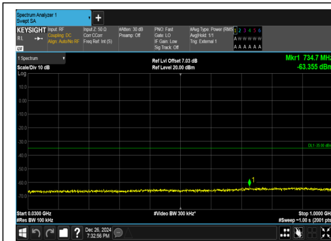
Band41-5MHz-QPSK-39675-1RB#0-30~1000-PASS
