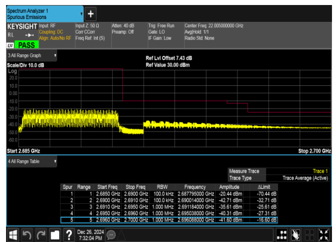
Band41-5MHz-16QAM-41565-25RB#0-PASS
