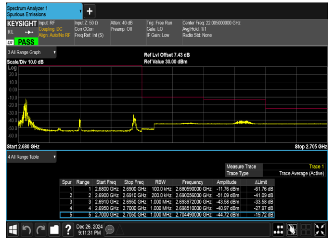
Band41-10MHz-QPSK-41540-1RB#0-PASS
