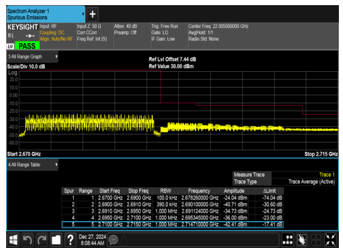
Band41-20MHz-QPSK-41490-100RB#0-PASS
