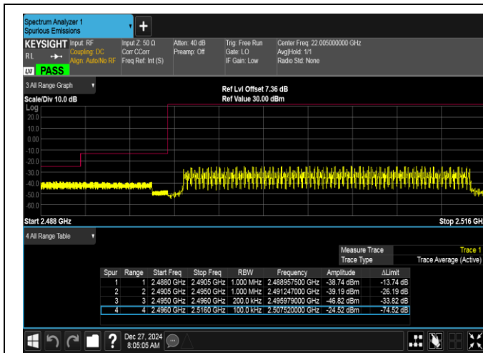
Band41-20MHz-QPSK-39750-100RB#0-PASS
