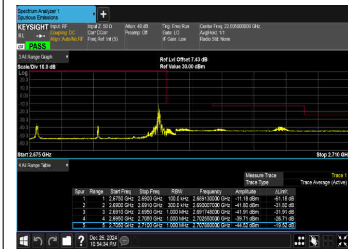
Band41-15MHz-QPSK-41515-1RB#74-PASS
