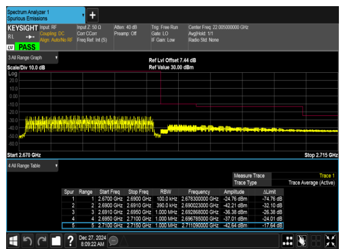
Band41-20MHz-16QAM-41490-100RB#0-PASS
