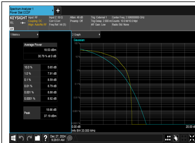
Band41-20MHz-16QAM-39750-1RB#0-PASS
