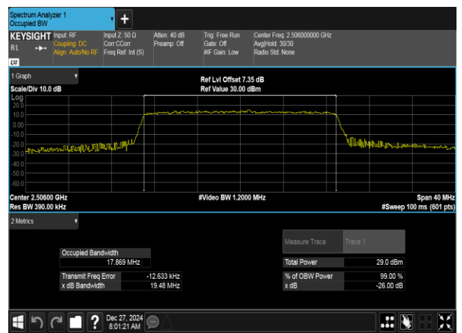
Band41-20MHz-16QAM-39750-100RB#0-PASS
