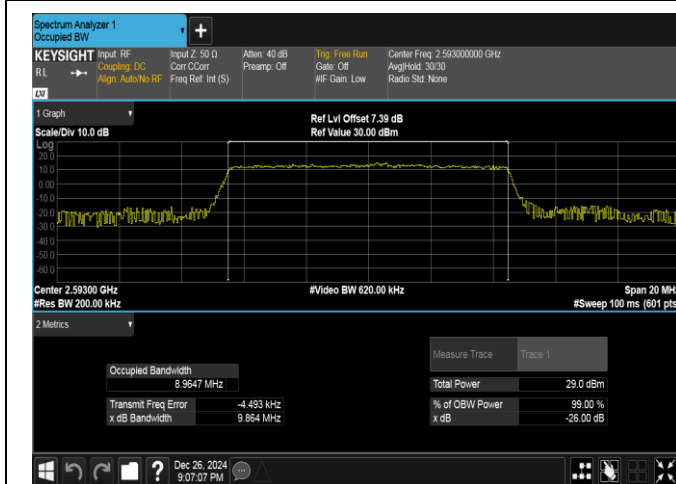
Band41-10MHz-16QAM-40620-50RB#0-PASS
