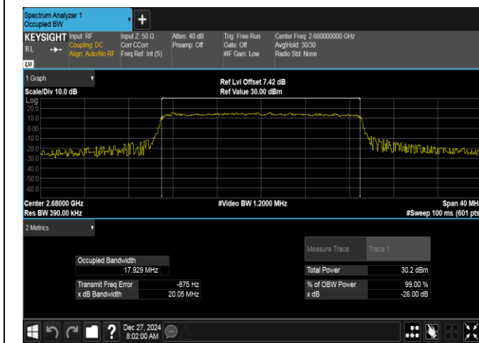
Band41-20MHz-QPSK-41490-100RB#0-PASS
