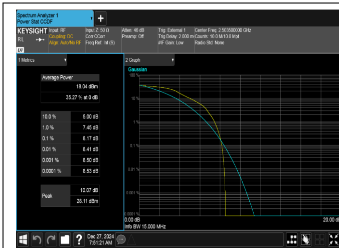
Band41-15MHz-QPSK-39725-1RB#0-PASS
