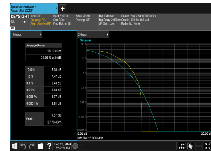
Band41-15MHz-QPSK-40620-1RB#0-PASS
