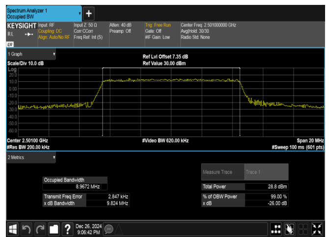
Band41-10MHz-16QAM-39700-50RB#0-PASS
