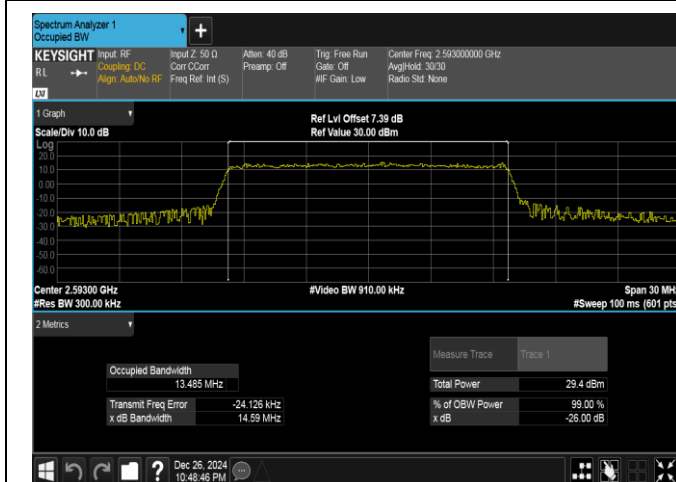
Band41-15MHz-16QAM-40620-75RB#0-PASS
