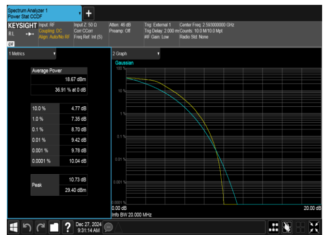
Band41-20MHz-QPSK-40620-100RB#0-PASS
