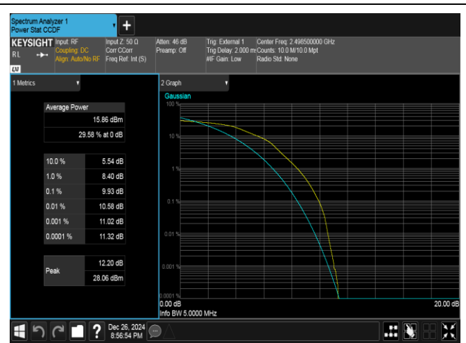
Band41-5MHz-16QAM-39675-25RB#0-PASS
