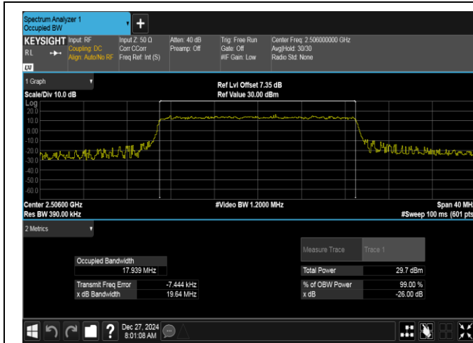
Band41-20MHz-QPSK-39750-100RB#0-PASS
