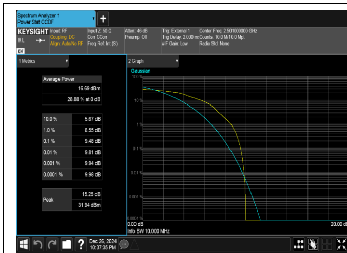
Band41-10MHz-16QAM-39700-1RB#0-PASS
