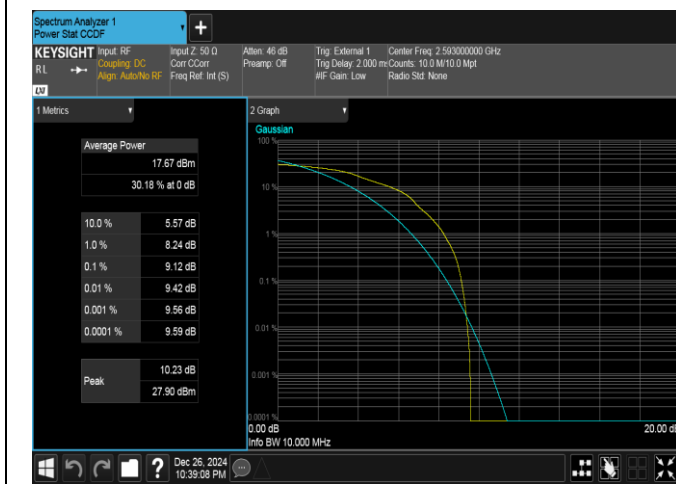
Band41-10MHz-16QAM-40620-1RB#0-PASS
