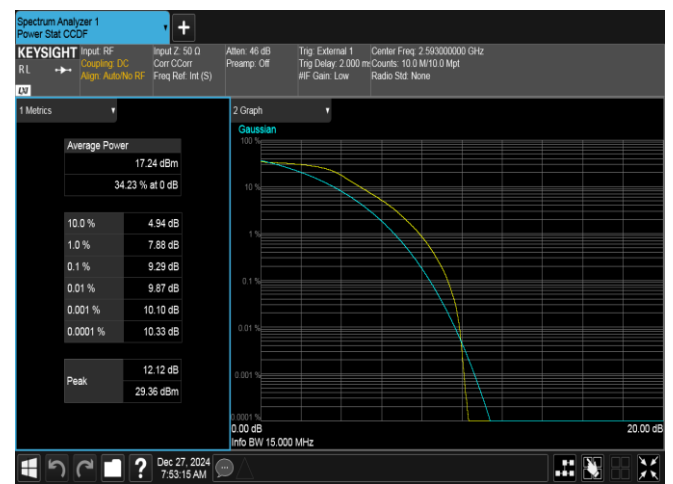
Band41-15MHz-QPSK-40620-75RB#0-PASS
