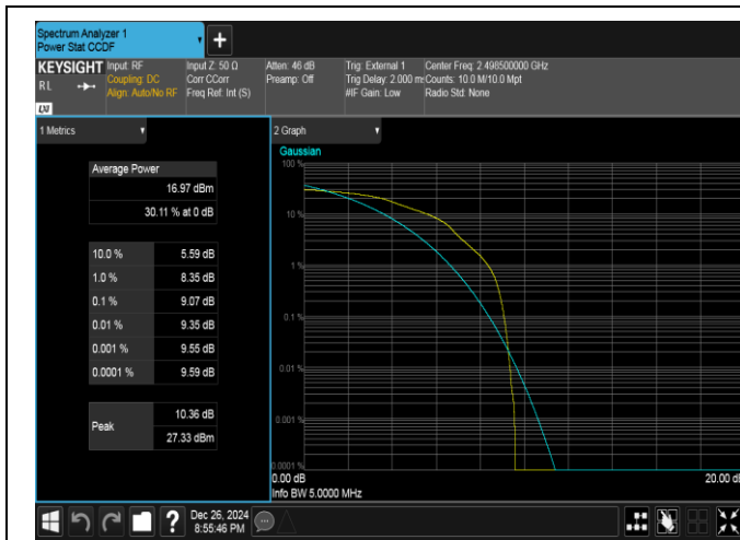
Band41-5MHz-16QAM-39675-1RB#0-PASS
