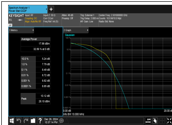
Band41-10MHz-QPSK-39700-1RB#0-PASS
