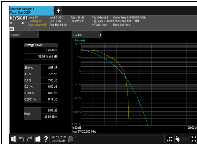
Band41-20MHz-QPSK-39750-1RB#0-PASS
