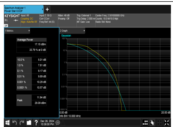
Band41-10MHz-QPSK-39700-50RB#0-PASS
