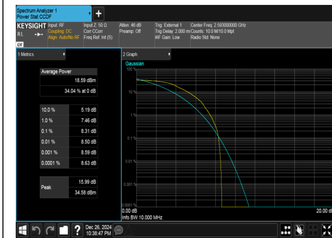
Band41-10MHz-QPSK-40620-1RB#0-PASS
