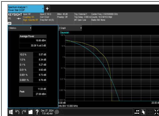
Band41-15MHz-16QAM-39725-1RB#0-PASS
