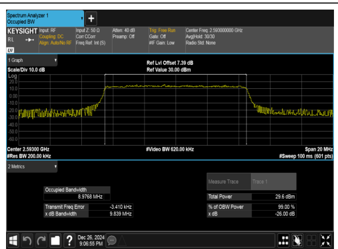
Band41-10MHz-QPSK-40620-50RB#0-PASS
