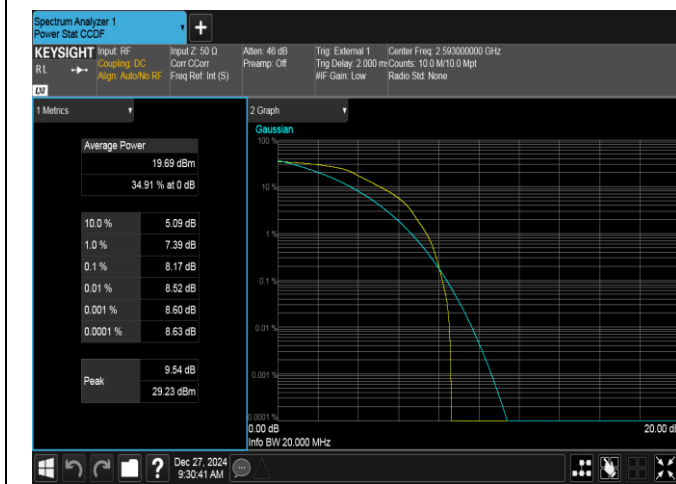
Band41-20MHz-QPSK-40620-1RB#0-PASS
