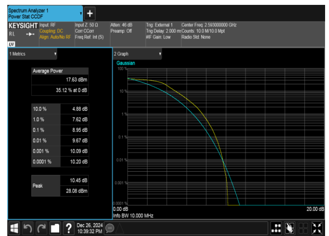
Band41-10MHz-QPSK-40620-50RB#0-PASS
