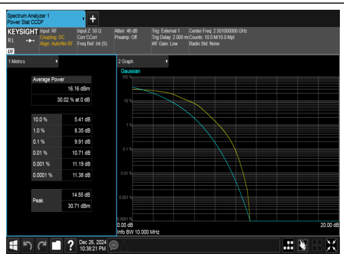
Band41-10MHz-16QAM-39700-50RB#0-PASS
