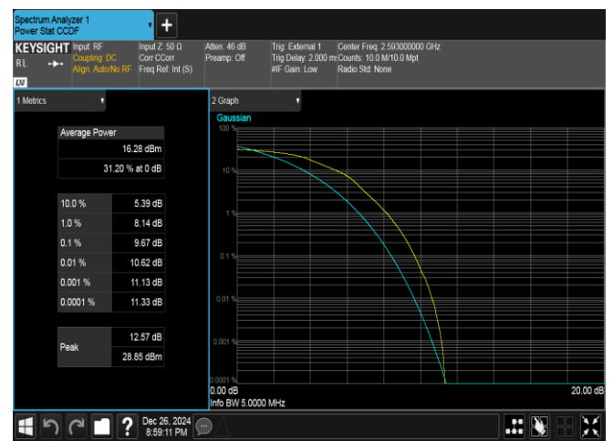
Band41-5MHz-16QAM-40620-25RB#0-PASS
