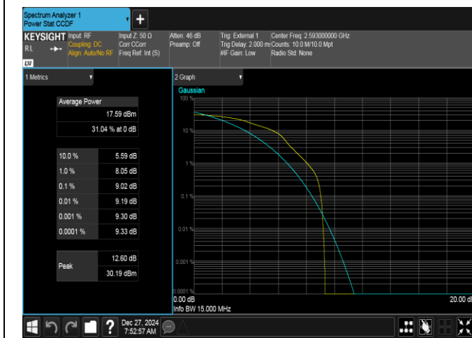
Band41-15MHz-16QAM-40620-1RB#0-PASS
