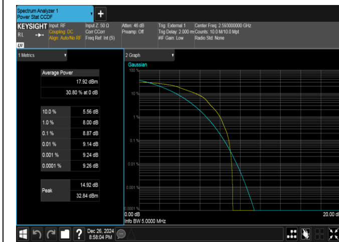
Band41-5MHz-16QAM-40620-1RB#0-PASS
