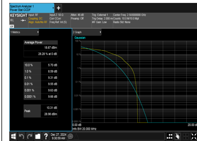
Band41-20MHz-16QAM-40620-1RB#0-PASS
