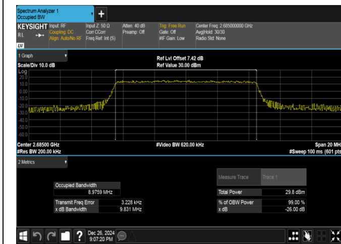
Band41-10MHz-QPSK-41540-50RB#0-PASS
