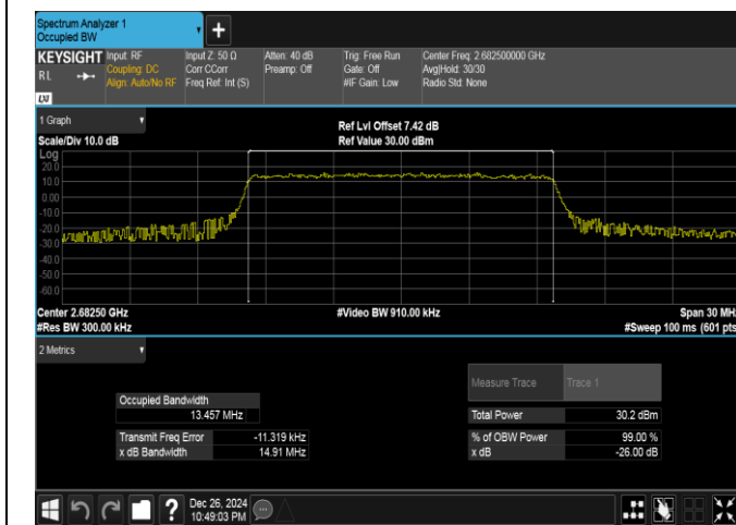
Band41-15MHz-QPSK-41515-75RB#0-PASS
