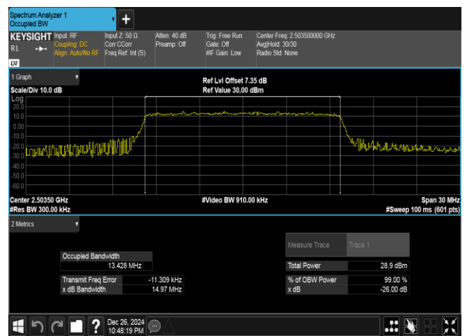
Band41-15MHz-16QAM-39725-75RB#0-PASS
