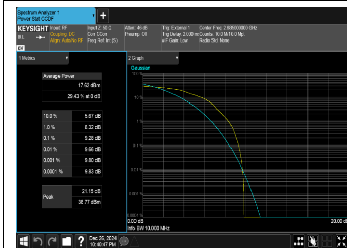
Band41-10MHz-16QAM-41540-1RB#0-PASS
