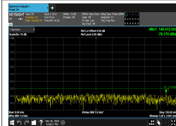
Band40(2350-2360)-5MHz-QPSK-39225-25RB#0-0.009~0.15-PASS
