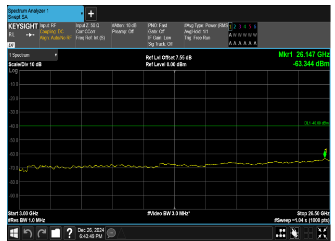
Band40(2350-2360)-5MHz-16QAM-39200-1RB#24-3000~26500-PASS
