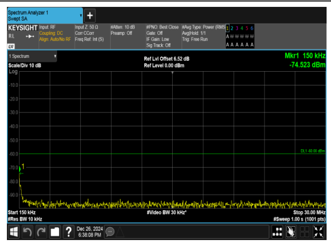
Band40(2350-2360)-5MHz-16QAM-39175-1RB#24-0.15~30-PASS
