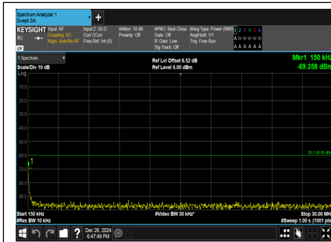
Band40(2350-2360)-5MHz-QPSK-39225-1RB#24-0.15~30-PASS
