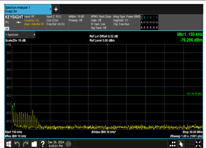
Band40(2350-2360)-5MHz-16QAM-39200-25RB#0-0.15~30-PASS
