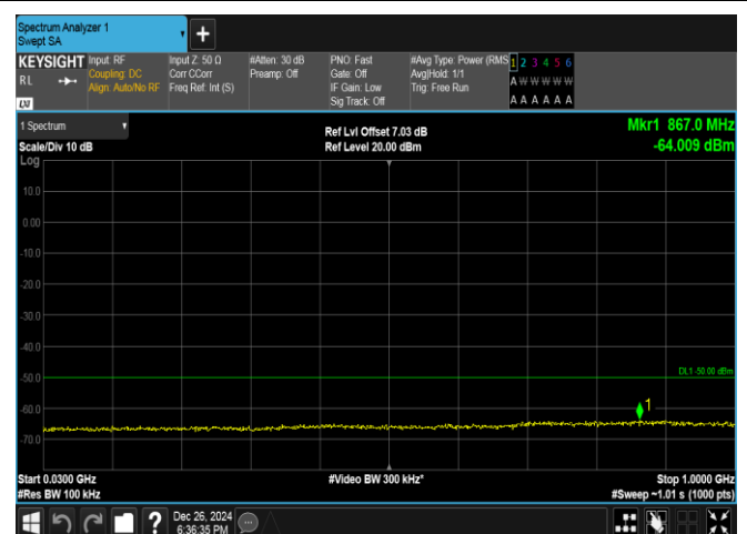
Band40(2350-2360)-5MHz-16QAM-39175-1RB#0-30~1000-PASS
