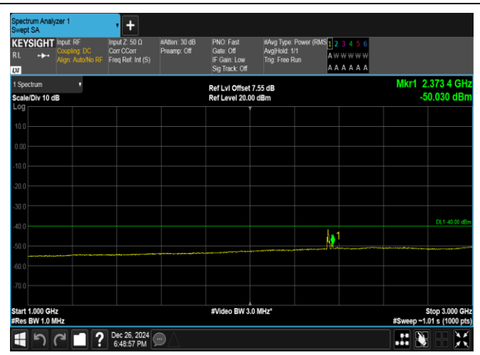
Band40(2350-2360)-5MHz-16QAM-39225-1RB#24-1000~3000-PASS
