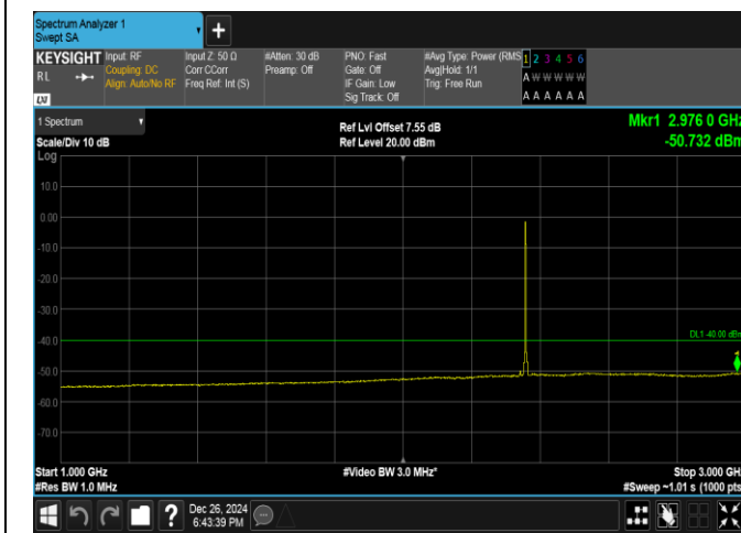
Band40(2350-2360)-5MHz-16QAM-39200-1RB#24-1000~3000-PASS
