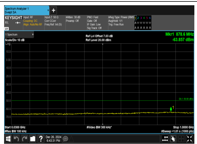
Band40(2350-2360)-5MHz-16QAM-39200-1RB#24-30~1000-PASS
