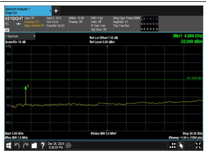
Band40(2350-2360)-5MHz-16QAM-39175-1RB#0-3000~26500-PASS
