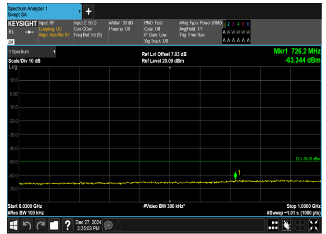
Band40(2350-2360)-10MHz-QPSK-39200-1RB#49-30~1000-PASS
