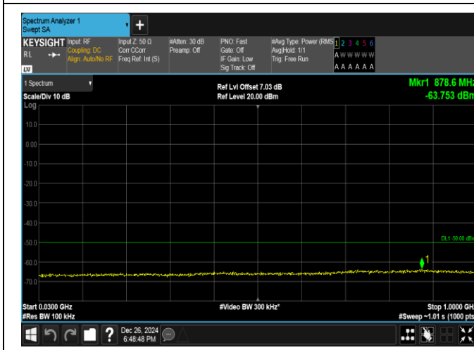
Band40(2350-2360)-5MHz-16QAM-39225-1RB#24-30~1000-PASS
