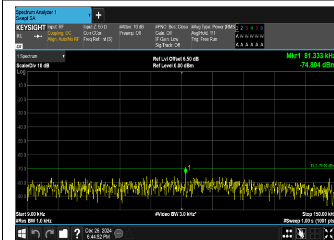
Band40(2350-2360)-5MHz-16QAM-39200-25RB#0-0.009~0.15-PASS
