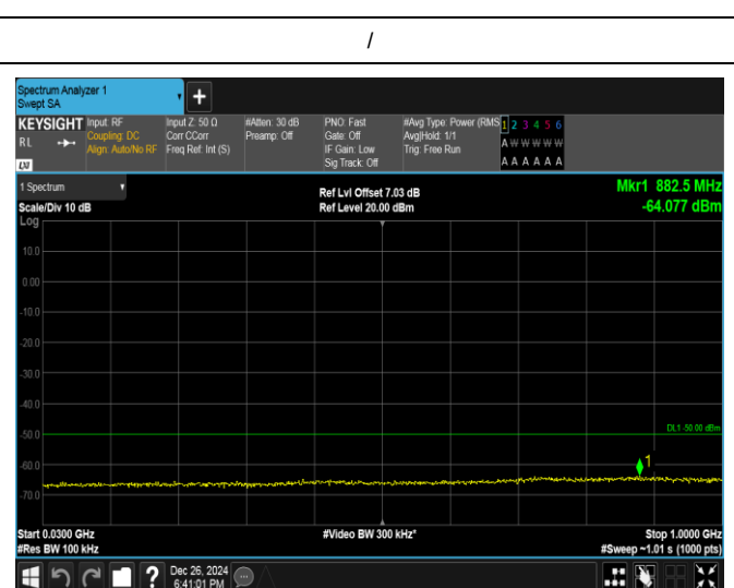
Band40(2350-2360)-5MHz-QPSK-39200-1RB#0-30~1000-PASS
