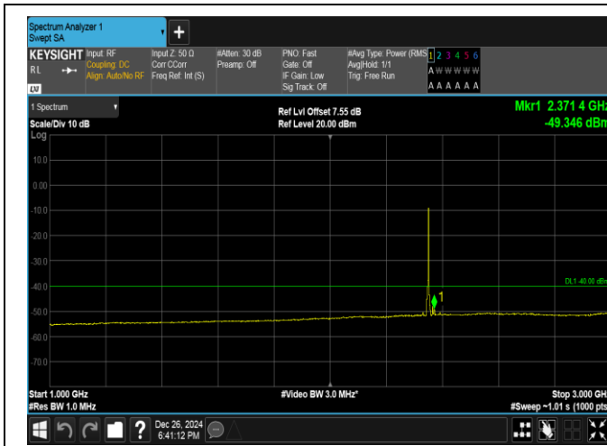
Band40(2350-2360)-5MHz-QPSK-39200-1RB#0-1000-3000-PASS
