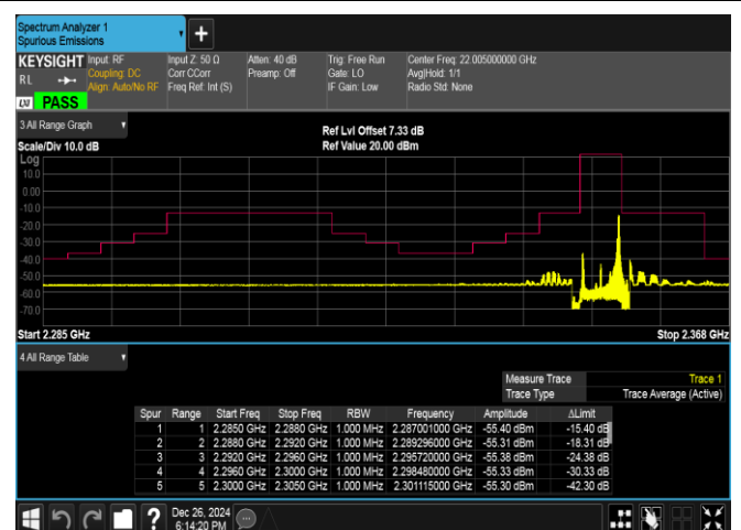
Band40(2350-2360)-5MHz-16QAM-39175-1RB#24-PASS
