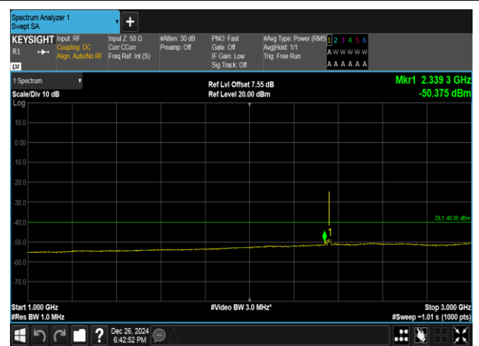
Band40(2350-2360)-5MHz-QPSK-39200-1RB#24-1000-3000-PASS
