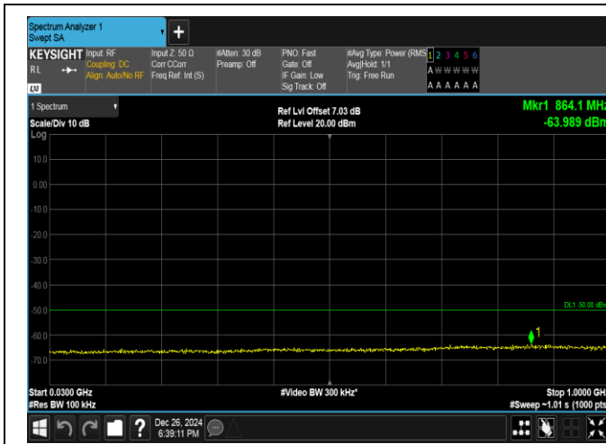
Band40(2350-2360)-5MHz-QPSK-39175-25RB#0-30~1000-PASS
