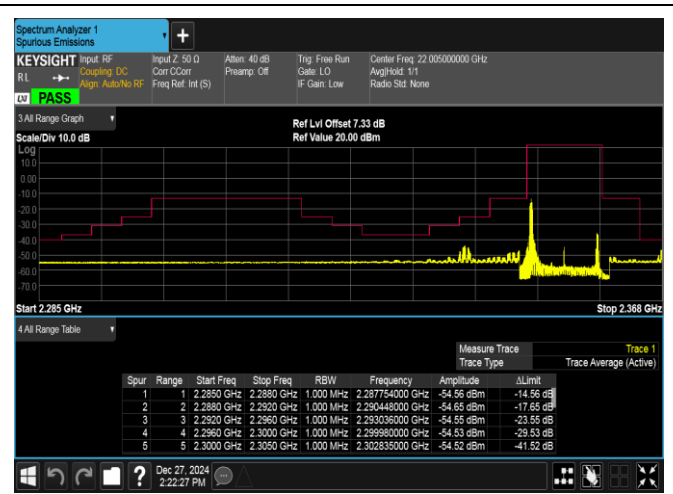
Band40(2350-2360)-10MHz-16QAM-39200-1RB#0-PASS
