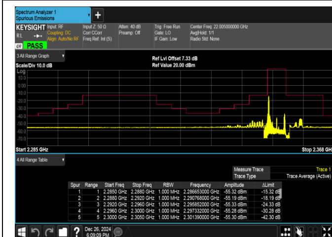
Band40(2350-2360)-5MHz-16QAM-39175-1RB#0-PASS
