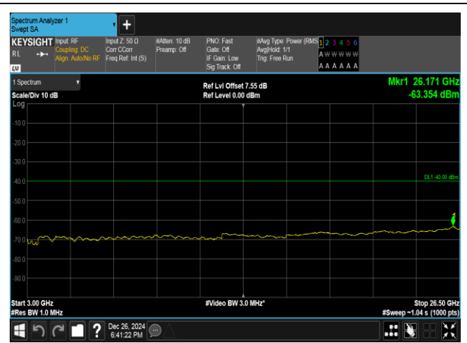
Band40(2350-2360)-5MHz-QPSK-39200-1RB#0-3000-26500-PASS
