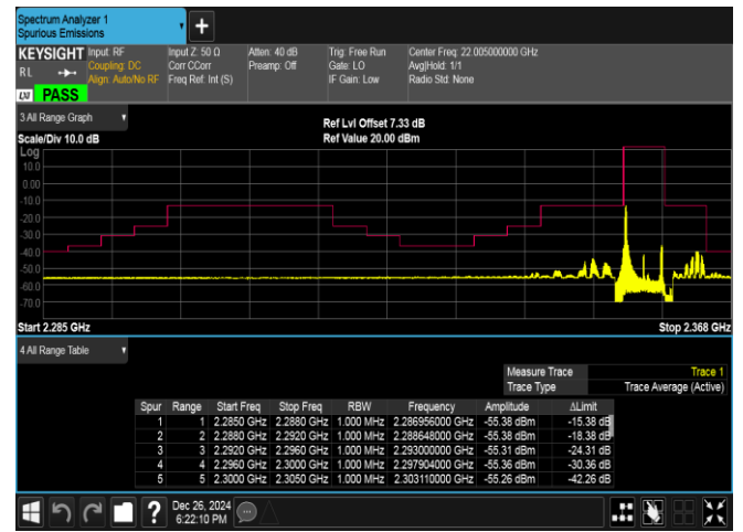
Band40(2350-2360)-5MHz-QPSK-39225-1RB#0-PASS
