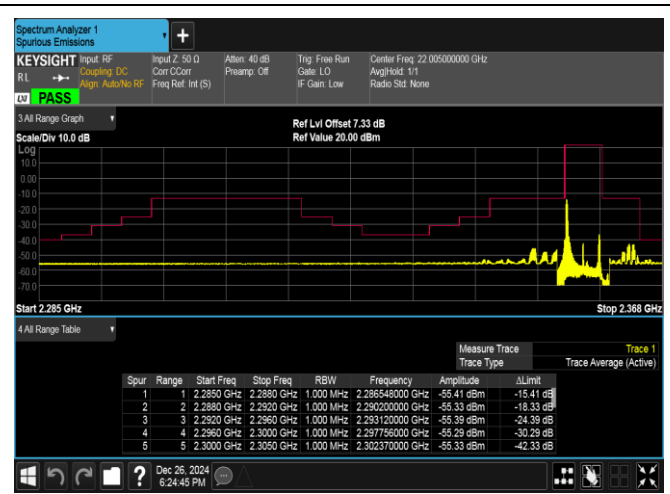
Band40(2350-2360)-5MHz-16QAM-39225-1RB#0-PASS
