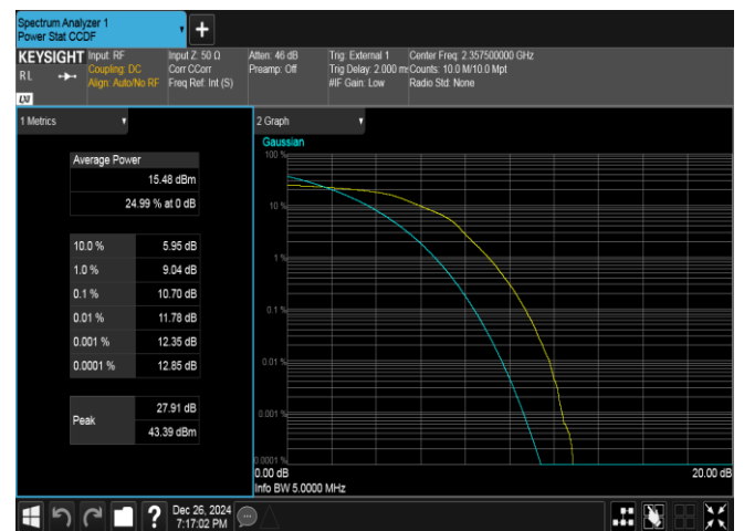
Band40(2350-2360)-5MHz-16QAM-39225-25RB#0-PASS
