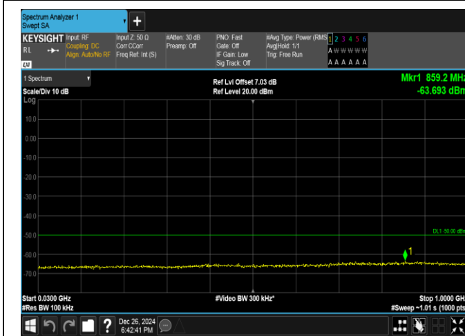
Band40(2350-2360)-5MHz-QPSK-39200-1RB#24-30-1000-PASS
