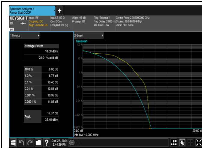
Band40(2350-2360)-10MHz-QPSK-39200-1RB#0-PASS
