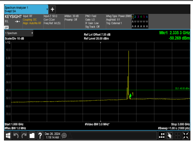
Band40(2305-2315)-10MHz-16QAM-38750-1RB#49-1000~3000-PASS
