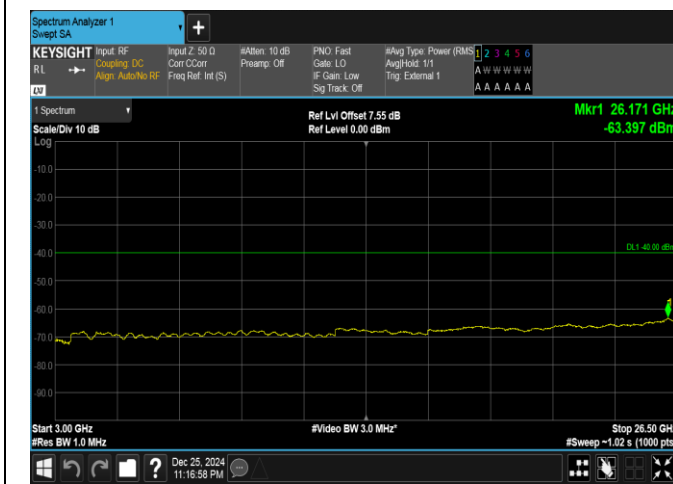
Band40(2305-2315)-5MHz-QPSK-38775-25RB#0-3000~26500-PASS
