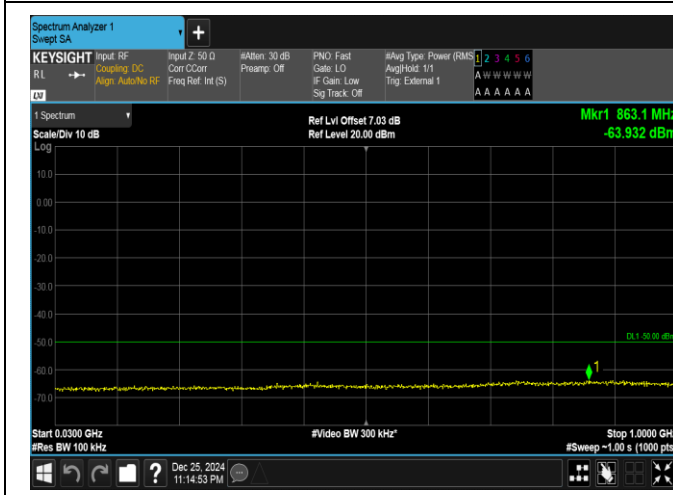
Band40(2305-2315)-5MHz-16QAM-38775-1RB#24-30~1000-PASS
