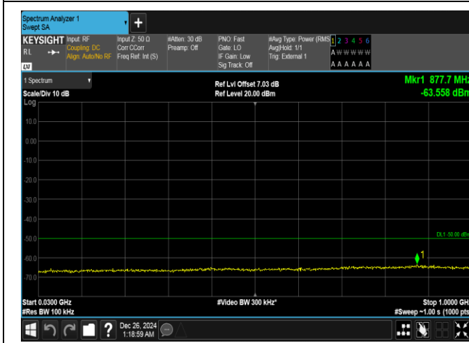
Band40(2305-2315)-10MHz-16QAM-38750-1RB#49-30~1000-PASS
