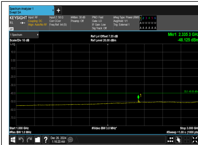
Band40(2305-2315)-10MHz-16QAM-38750-1RB#0-1000~3000-PASS
