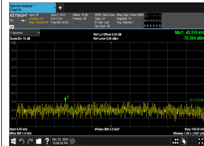
Band40(2305-2315)-5MHz-16QAM-38725-1RB#24-0.009~0.15-PASS
