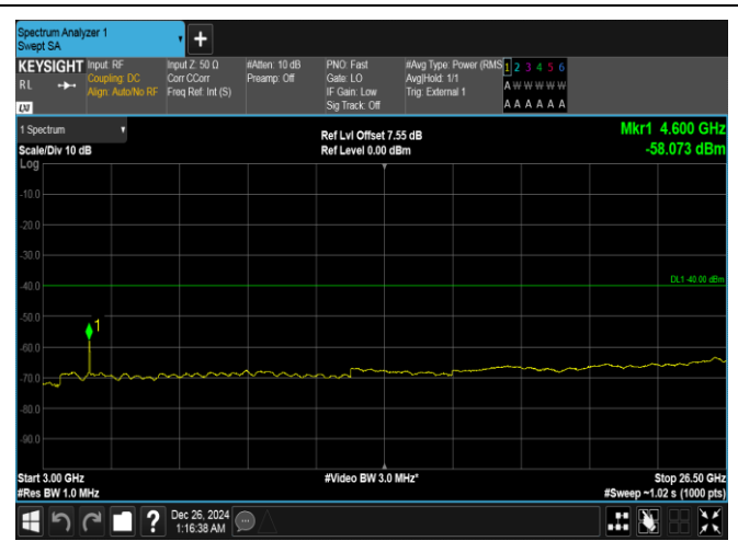
Band40(2305-2315)-10MHz-16QAM-38750-1RB#0-3000~26500-PASS
