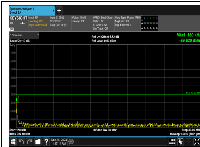
Band40(2305-2315)-10MHz-QPSK-38750-1RB#49-0.15~30-PASS
