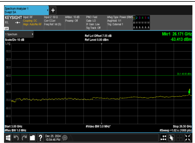
Band40(2305-2315)-5MHz-16QAM-38725-1RB#0-3000~26500-PASS
