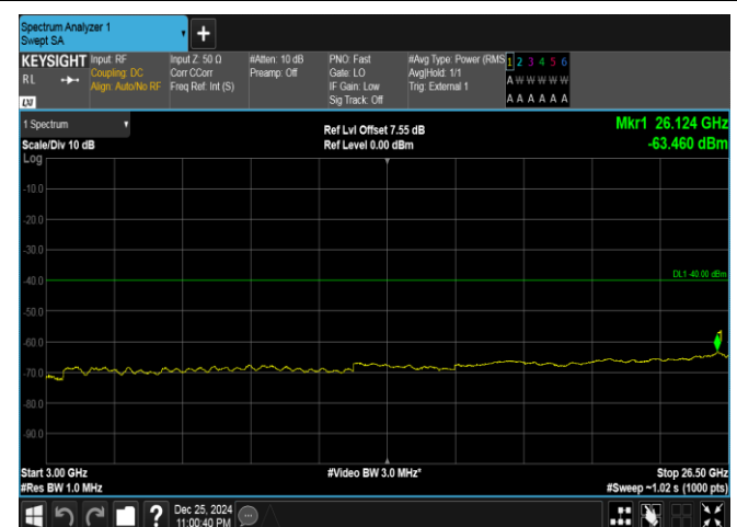
Band40(2305-2315)-5MHz-16QAM-38725-25RB#0-3000~26500-PASS
