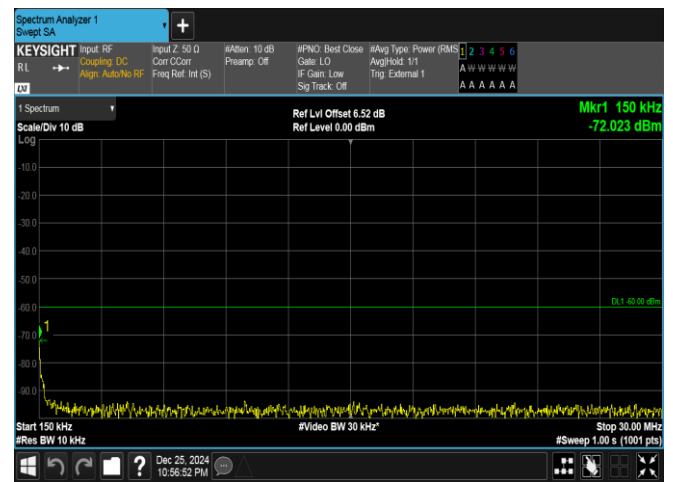
Band40(2305-2315)-5MHz-16QAM-38725-1RB#24-0.15~30-PASS
