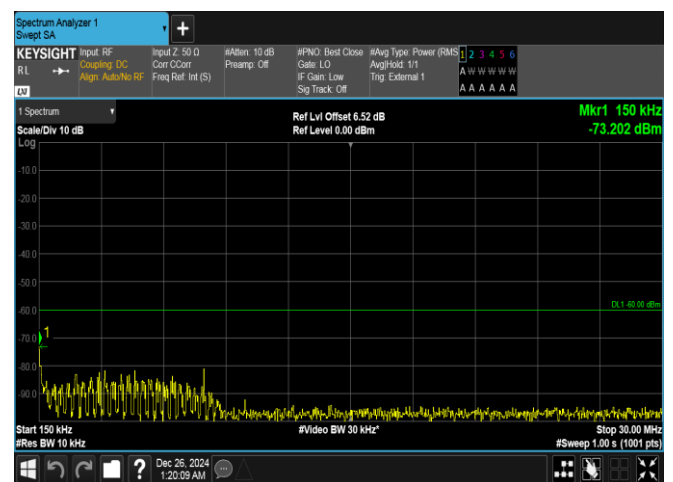
Band40(2305-2315)-10MHz-QPSK-38750-50RB#0-0.15~30-PASS
