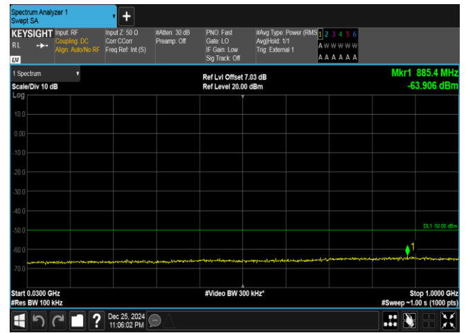
Band40(2305-2315)-5MHz-16QAM-38750-1RB#24-30~1000-PASS
