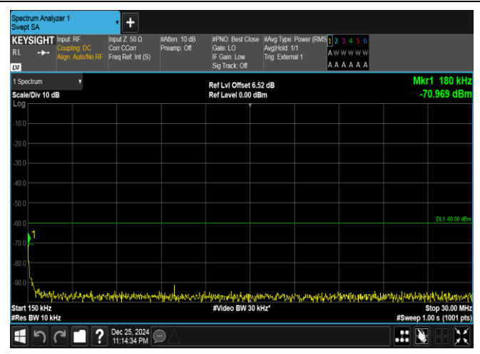
Band40(2305-2315)-5MHz-16QAM-38775-1RB#24-0.15~30-PASS
