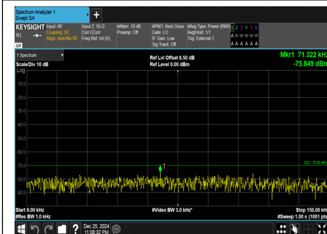
Band40(2305-2315)-5MHz-16QAM-38750-25RB#0-0.009~0.15-PASS
