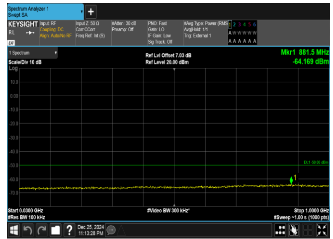
Band40(2305-2315)-5MHz-QPSK-38775-1RB#24-30~1000-PASS
