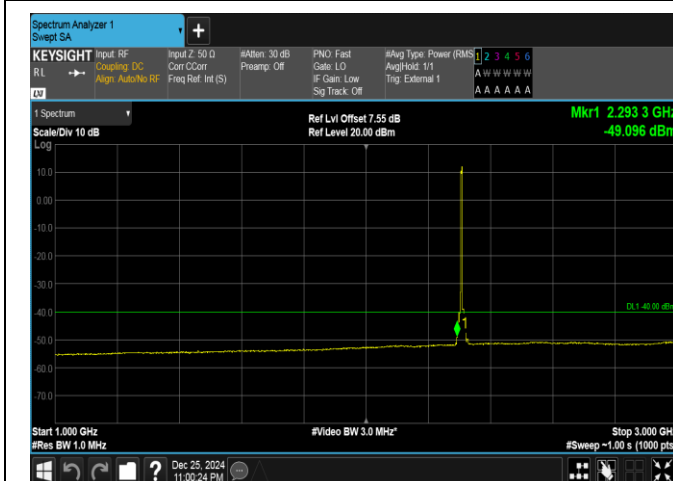
Band40(2305-2315)-5MHz-16QAM-38725-25RB#0-1000~3000-PASS
