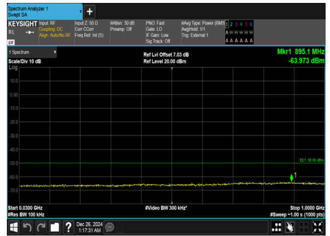
Band40(2305-2315)-10MHz-QPSK-38750-1RB#49-30~1000-PASS
