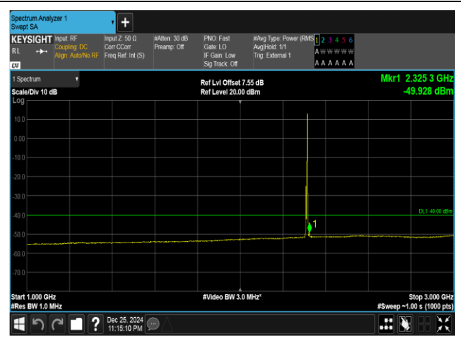
Band40(2305-2315)-5MHz-16QAM-38775-1RB#24-1000~3000-PASS
