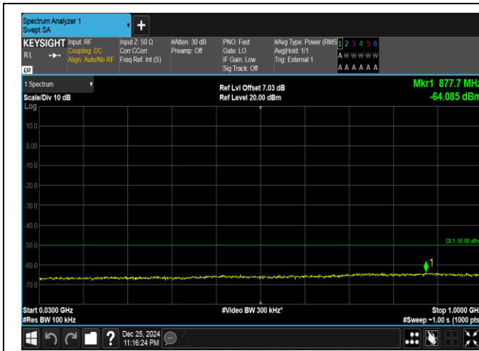
Band40(2305-2315)-5MHz-QPSK-38775-25RB#0-30~1000-PASS
