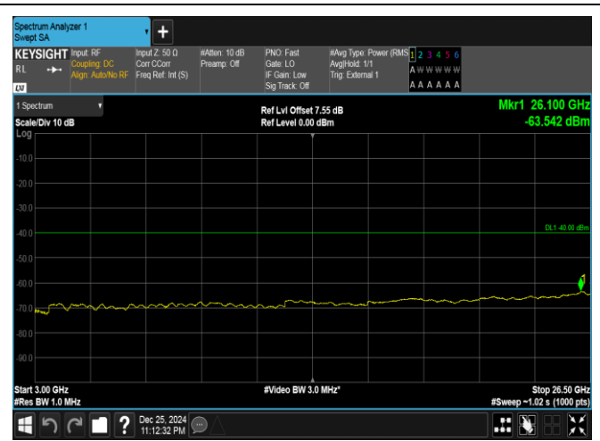
Band40(2305-2315)-5MHz-16QAM-38775-1RB#0-3000~26500-PASS
