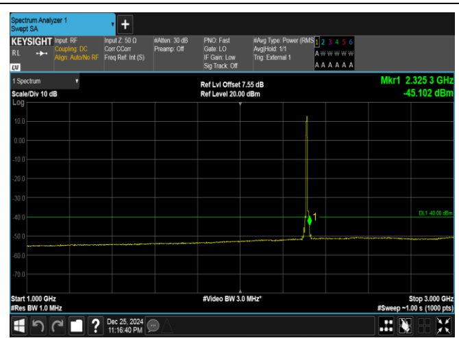
Band40(2305-2315)-5MHz-QPSK-38775-25RB#0-1000~3000-PASS
