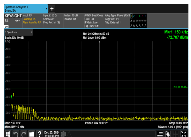
Band40(2305-2315)-5MHz-16QAM-38750-25RB#0-0.15~30-PASS
