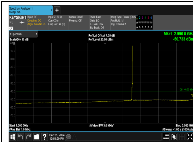
Band40(2305-2315)-5MHz-16QAM-38725-1RB#0-1000~3000-PASS
