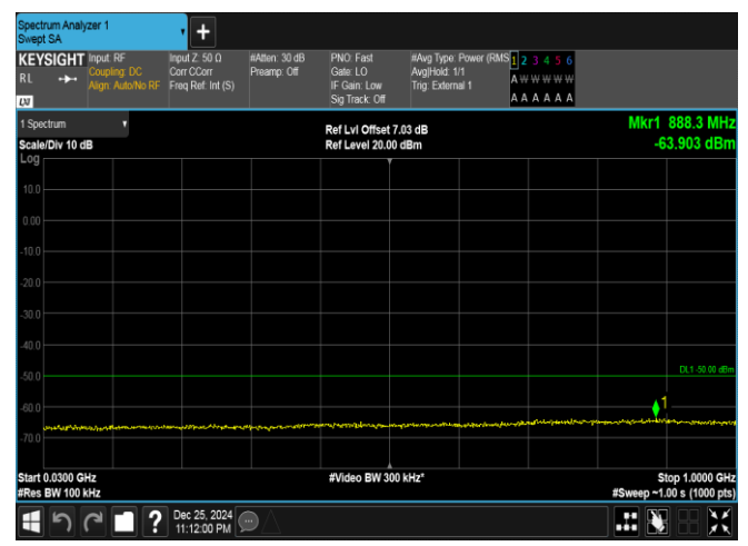
Band40(2305-2315)-5MHz-16QAM-38775-1RB#0-30~1000-PASS
