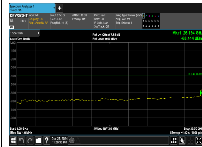
Band40(2305-2315)-5MHz-16QAM-38750-25RB#0-3000~26500-PASS
