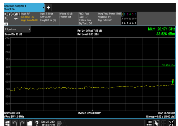
Band40(2305-2315)-5MHz-QPSK-38750-25RB#0-3000~26500-PASS
