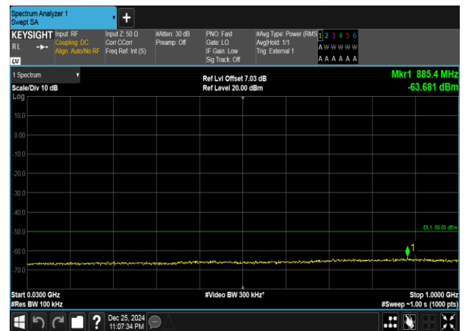
Band40(2305-2315)-5MHz-QPSK-38750-25RB#0-30~1000-PASS
