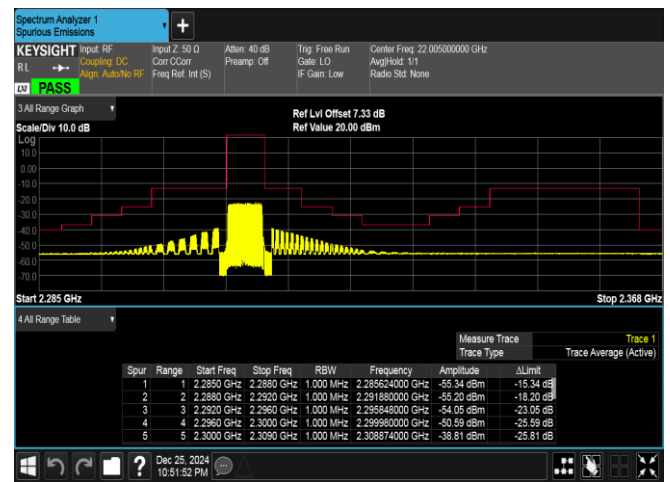
Band40(2305-2315)-5MHz-16QAM-38775-25RB#0-PASS
