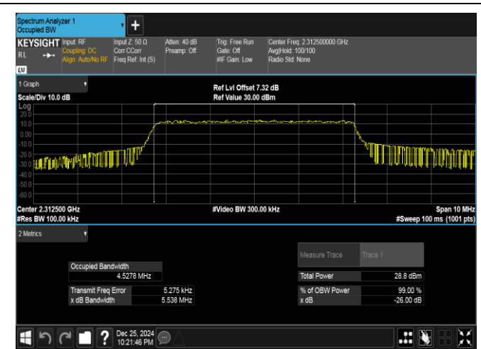
Band40(2305-2315)-5MHz-16QAM-38775-25RB#0-PASS
