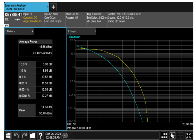
Band40(2305-2315)-5MHz-16QAM-38725-25RB#0-PASS
