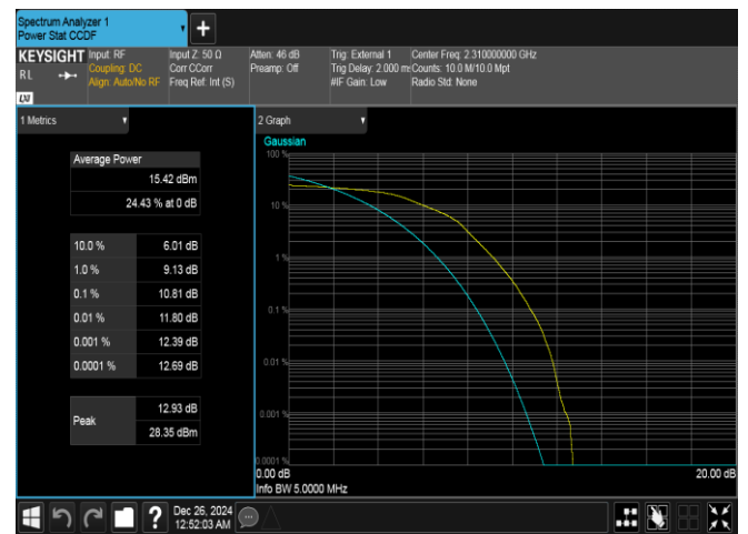
Band40(2305-2315)-5MHz-16QAM-38750-25RB#0-PASS
