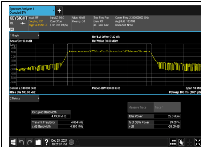
Band40(2305-2315)-5MHz-16QAM-38750-25RB#0-PASS
