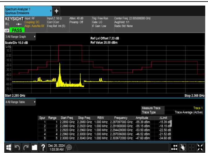
Band40(2305-2315)-10MHz-16QAM-38750-1RB#0-PASS
