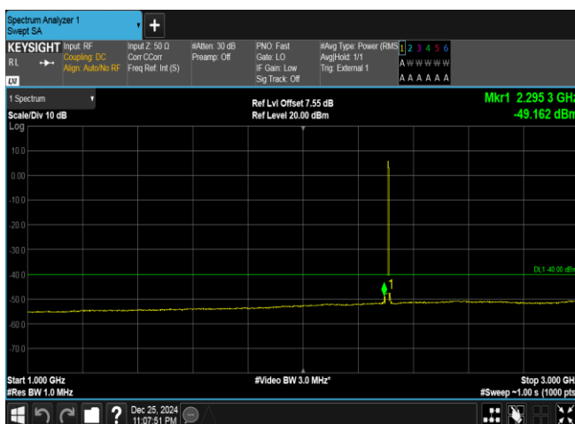
Band40(2305-2315)-5MHz-QPSK-38750-25RB#0-1000~3000-PASS
