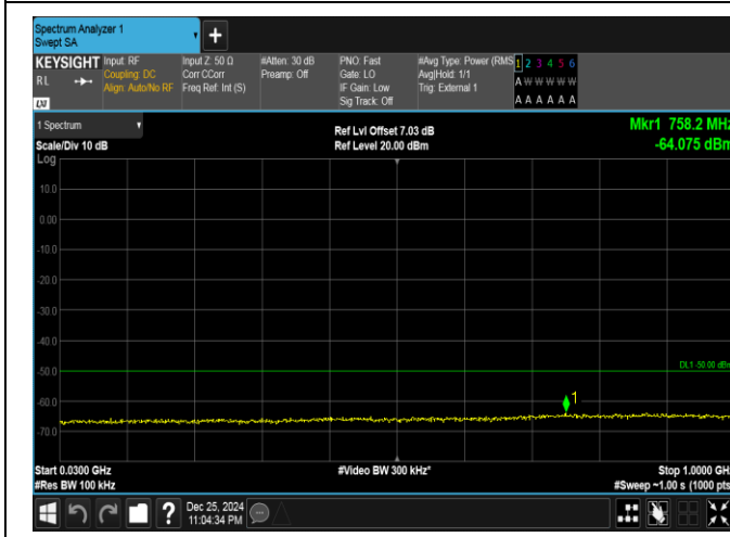
Band40(2305-2315)-5MHz-QPSK-38750-1RB#24-30-1000-PASS
