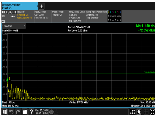
Band40(2305-2315)-5MHz-QPSK-38750-25RB#0-0.15~30-PASS
