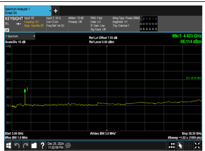
Band40(2305-2315)-5MHz-QPSK-38750-1RB#0-3000-26500-PASS
