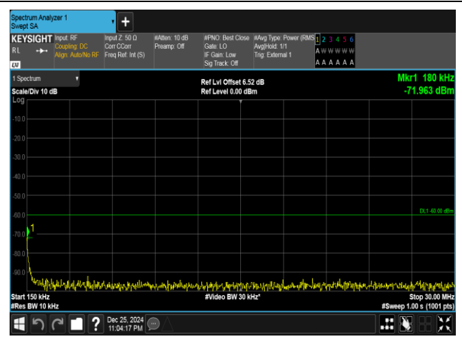
Band40(2305-2315)-5MHz-QPSK-38750-1RB#24-0.15-30-PASS
