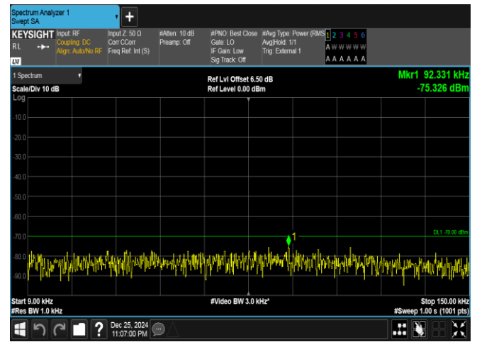
Band40(2305-2315)-5MHz-QPSK-38750-25RB#0-0.009~0.15-PASS
