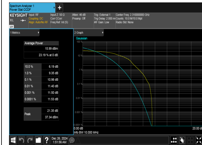
Band40(2305-2315)-10MHz-16QAM-38750-1RB#0-PASS
