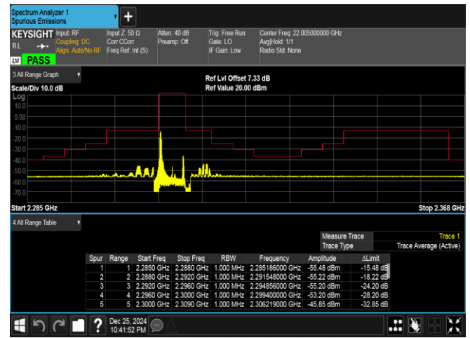
Band40(2305-2315)-5MHz-16QAM-38775-1RB#0-PASS
