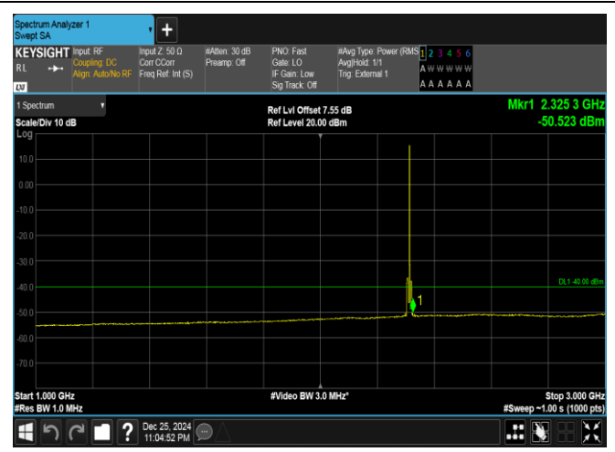
Band40(2305-2315)-5MHz-QPSK-38750-1RB#24-1000-3000-PASS
