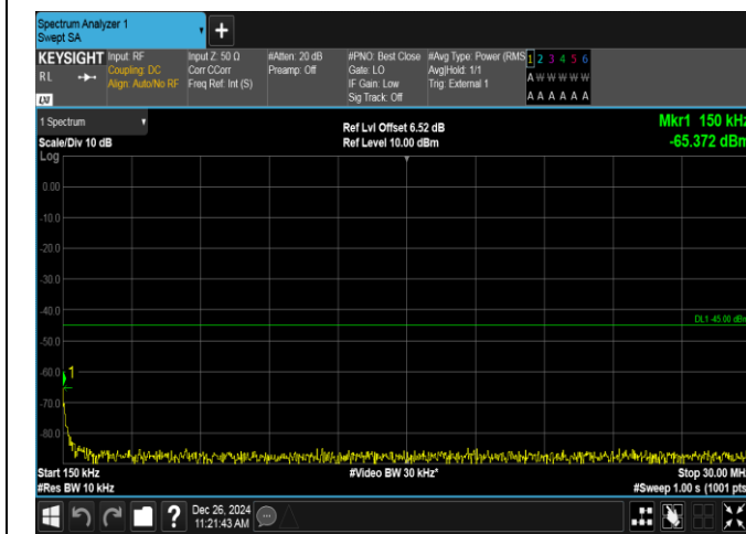
Band38-20MHz-16QAM-38150-1RB#0-0.15~30-PASS
