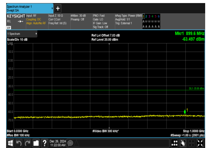
Band38-20MHz-16QAM-38150-1RB#0-30~1000-PASS
