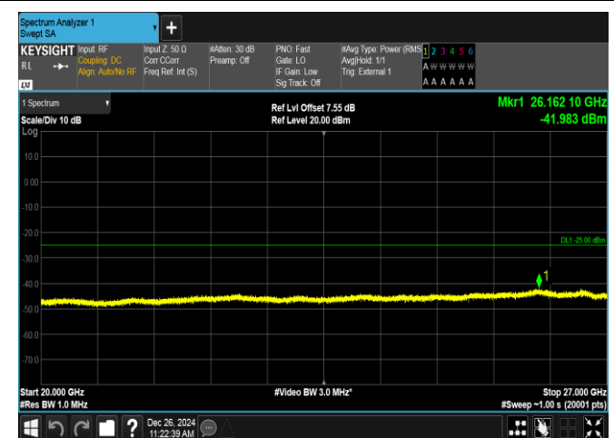
Band38-20MHz-16QAM-38150-1RB#0-20000~27000-PASS
