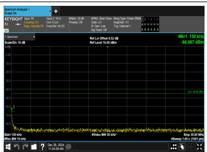
Band38-20MHz-16QAM-38150-1RB#99-0.15~30-PASS
