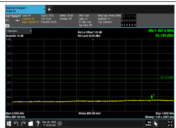
Band38-20MHz-16QAM-37850-100RB#0-30~1000-PASS
