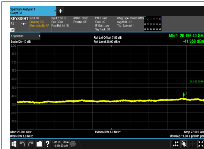
Band38-20MHz-16QAM-38000-100RB#0-20000~27000-PASS
