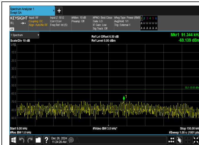
Band38-20MHz-16QAM-38150-1RB#99-0.009~0.15-PASS
