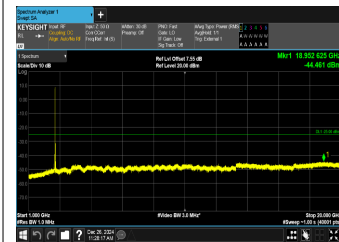
Band38-20MHz-16QAM-38150-100RB#0-1000~20000-PASS
