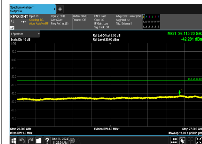
Band38-20MHz-16QAM-38150-1RB#99-20000~27000-PASS
