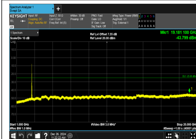
Band38-20MHz-16QAM-38150-1RB#0-1000~20000-PASS
