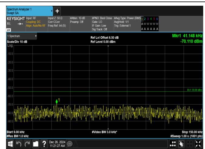
Band38-20MHz-16QAM-38150-1RB#0-0.009~0.15-PASS
