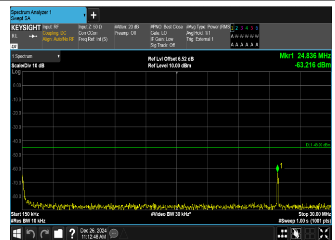
Band38-20MHz-16QAM-38000-1RB#0-0.15~30-PASS
