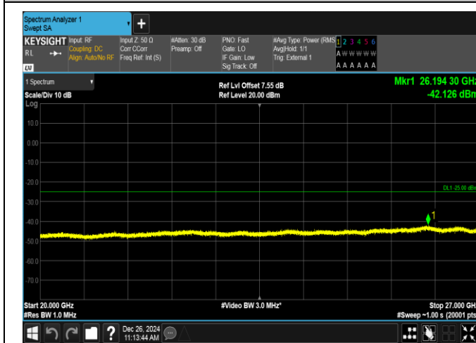
Band38-20MHz-16QAM-38000-1RB#0-20000~27000-PASS
