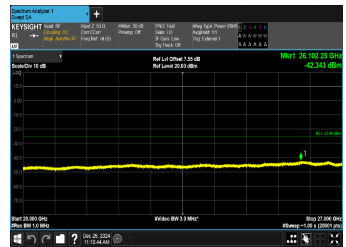
Band38-20MHz-16QAM-37850-100RB#0-20000~27000-PASS
