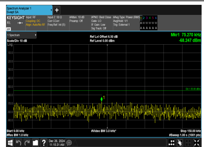
Band38-20MHz-16QAM-38000-1RB#99-0.009~0.15-PASS
