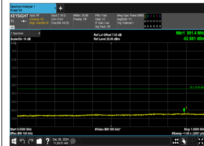
Band38-20MHz-16QAM-38150-1RB#99-30~1000-PASS
