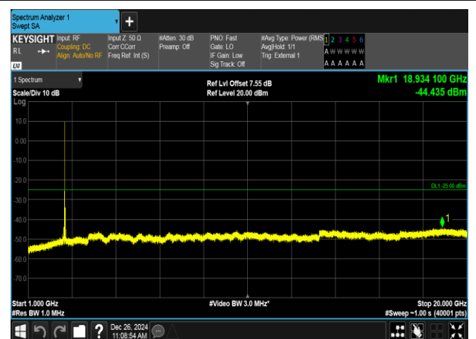
Band38-20MHz-QPSK-37850-100RB#0-1000~20000-PASS
