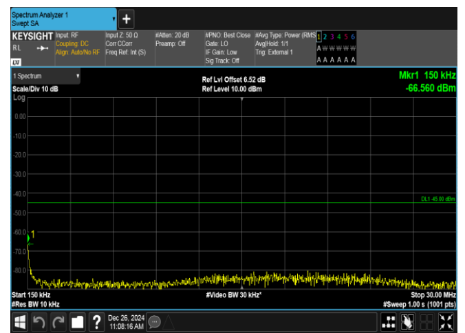
Band38-20MHz-QPSK-37850-100RB#0-0.15~30-PASS
