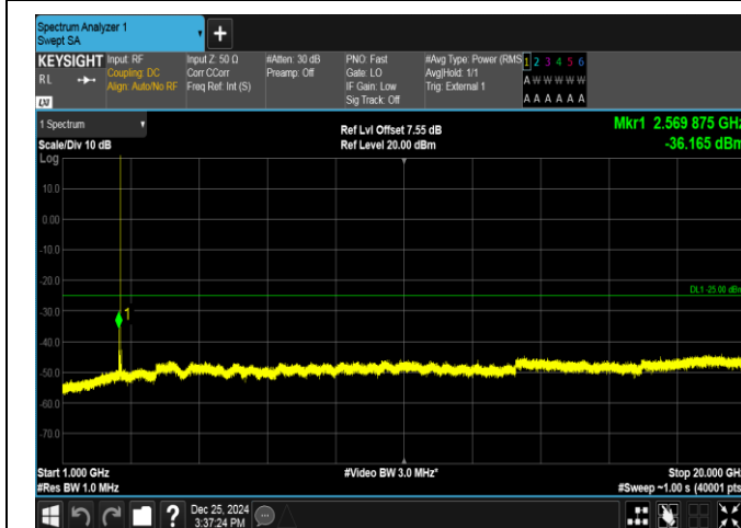
Band38-15MHz-16QAM-38175-1RB#0-1000~20000-PASS
