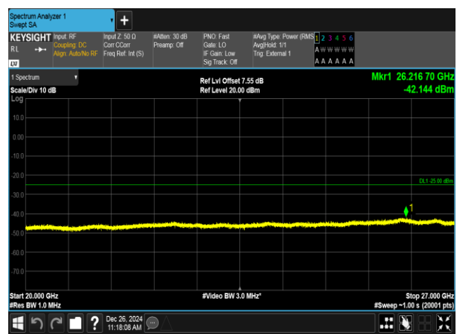
Band38-20MHz-QPSK-38000-100RB#0-20000~27000-PASS
