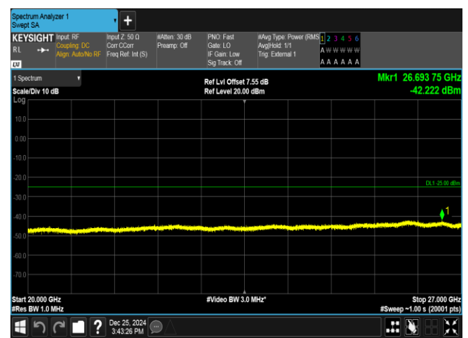
Band38-15MHz-16QAM-38175-75RB#0-20000~27000-PASS
