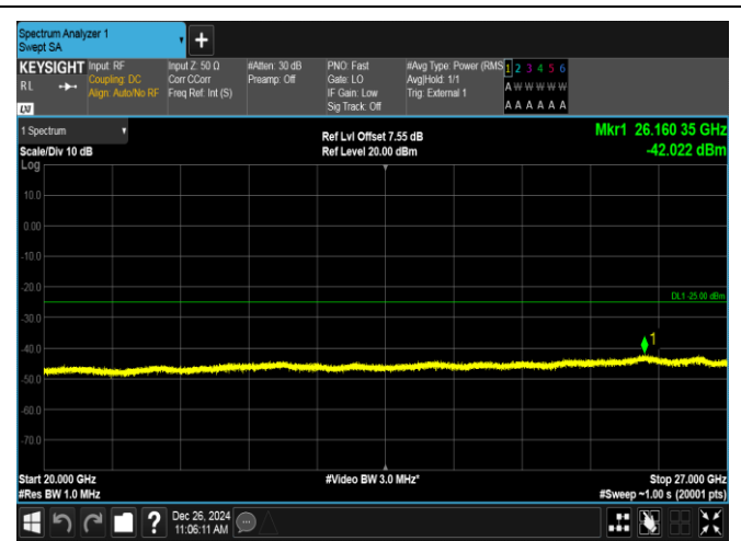
Band38-20MHz-QPSK-37850-1RB#99-20000~27000-PASS
