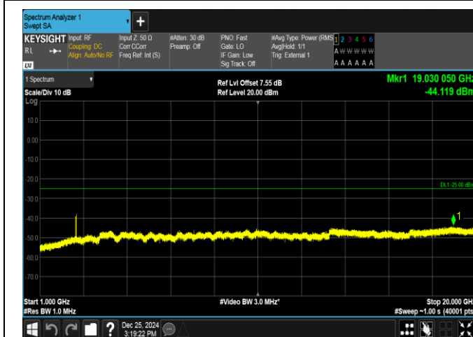
Band38-15MHz-16QAM-37825-1RB#0-1000~20000-PASS
