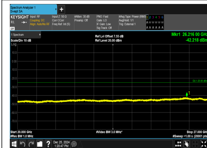
Band38-10MHz-16QAM-38200-1RB#49-20000~27000-PASS
