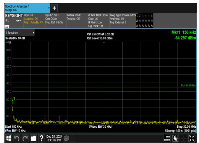
Band38-15MHz-QPSK-38175-75RB#0-0.15~30-PASS
