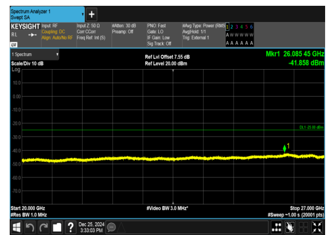
Band38-15MHz-QPSK-38000-75RB#0-20000~27000-PASS
