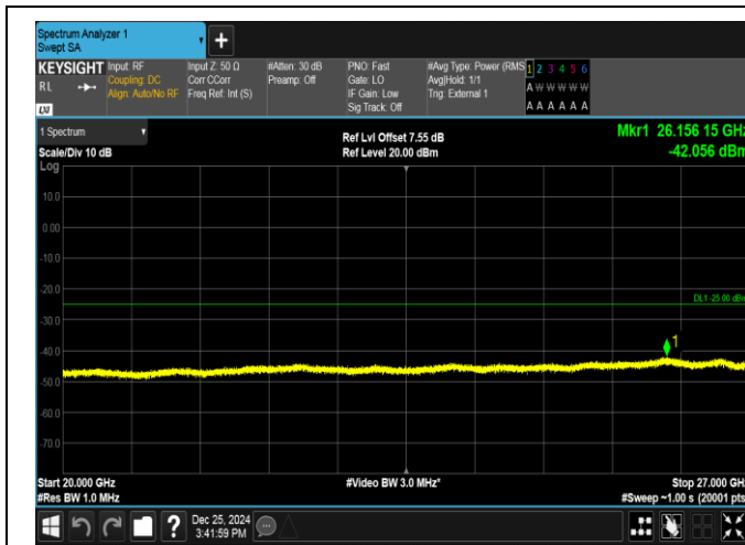
Band38-15MHz-QPSK-38175-75RB#0-20000~27000-PASS
