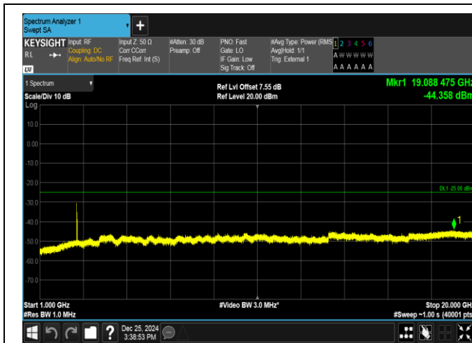
Band38-15MHz-QPSK-38175-1RB#74-1000~20000-PASS
