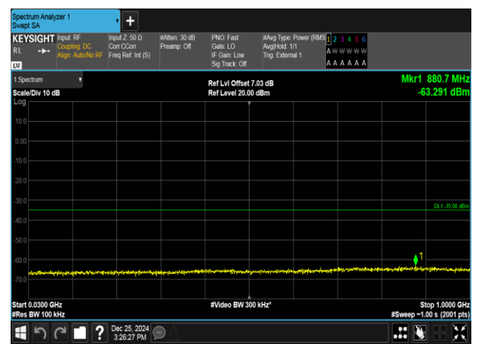
Band38-15MHz-QPSK-38000-1RB#0-30~1000-PASS
