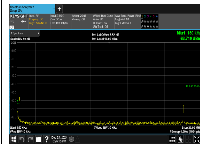
Band38-15MHz-QPSK-38000-1RB#0-0.15~30-PASS
