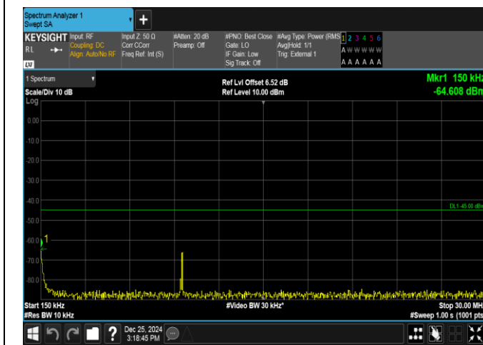
Band38-15MHz-16QAM-37825-1RB#0-0.15~30-PASS
