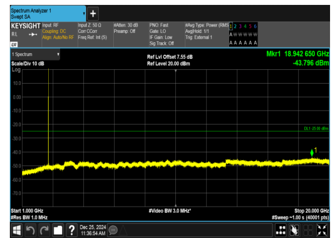
Band38-5MHz-16QAM-38225-1RB#24-1000~20000-PASS
