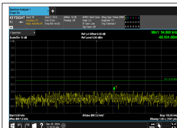
Band38-5MHz-OPSK-38000-1RB#24-0.009~0.15-PASS
