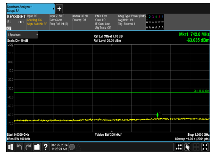
Band38-5MHz-QPSK-38000-1RB#0-30~1000-PASS
