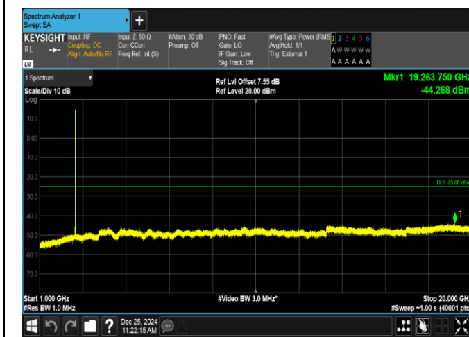
Band38-5MHz-16QAM-37775-25RB#0-1000~20000-PASS
