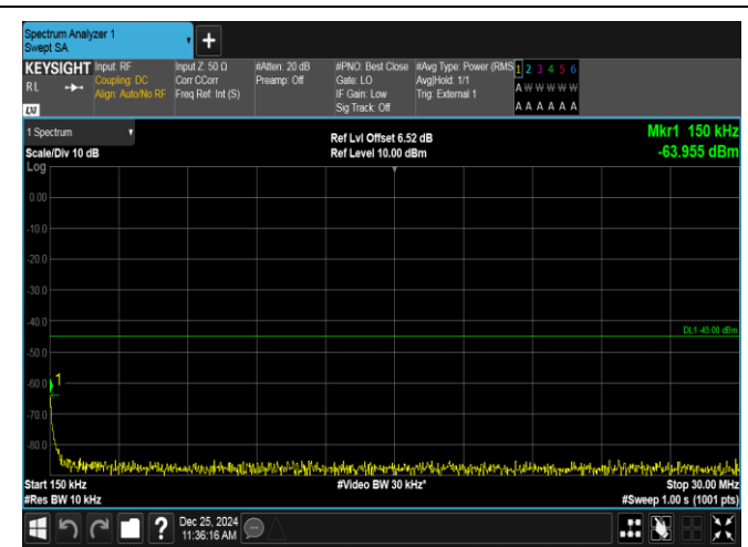
Band38-5MHz-16QAM-38225-1RB#24-0.15~30-PASS
