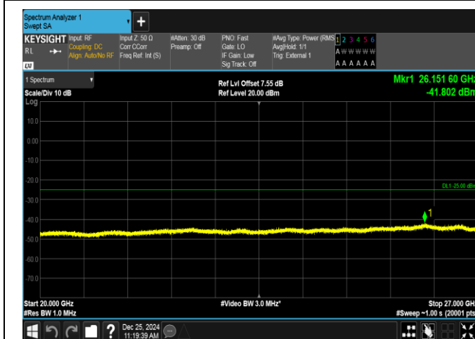
Band38-5MHz-16QAM-37775-1RB#24-20000~27000-PASS
