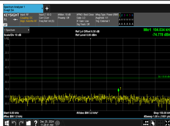
Band38-5MHz-QPSK-38000-25RB#0-0.009~0.15-PASS
