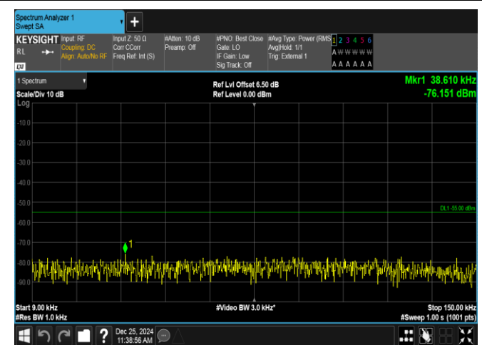
Band38-5MHz-16QAM-38225-25RB#0-0.009~0.15-PASS
