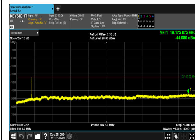
Band38-5MHz-16QAM-37775-1RB#0-1000~20000-PASS
