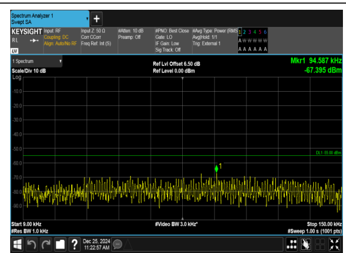
Band38-5MHz-QPSK-38000-1RB#0-0.009~0.15-PASS
