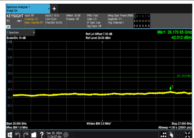
Band38-5MHz-QPSK-38000-1RB#0-20000~27000-PASS
