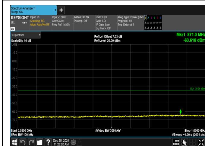
Band38-5MHz-OPSK-38000-1RB#24-30~1000-PASS
