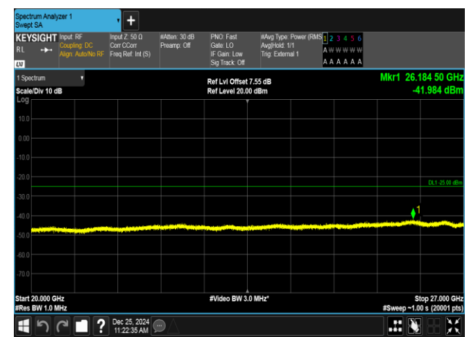
Band38-5MHz-16QAM-37775-25RB#0-20000~27000-PASS
