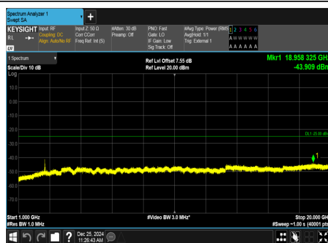
Band38-5MHz-OPSK-38000-1RB#24-1000~20000-PASS
