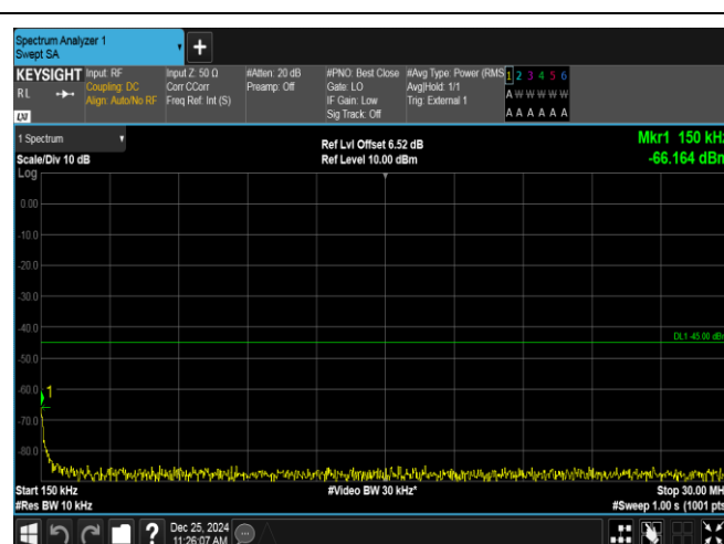
Band38-5MHz-OPSK-38000-1RB#24-0.15~30-PASS
