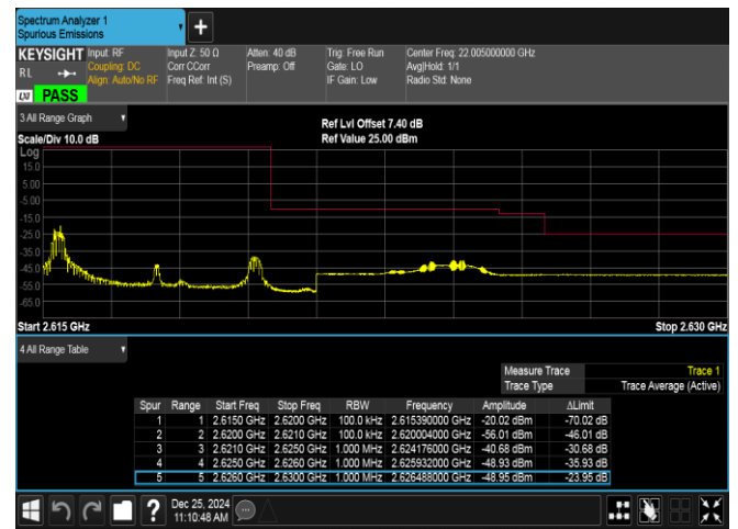
Band38-5MHz-QPSK-38225-1RB#0-PASS
